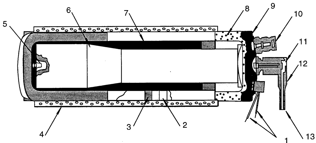
FIGURE 16. DISASSEMBLED GENERATOR
