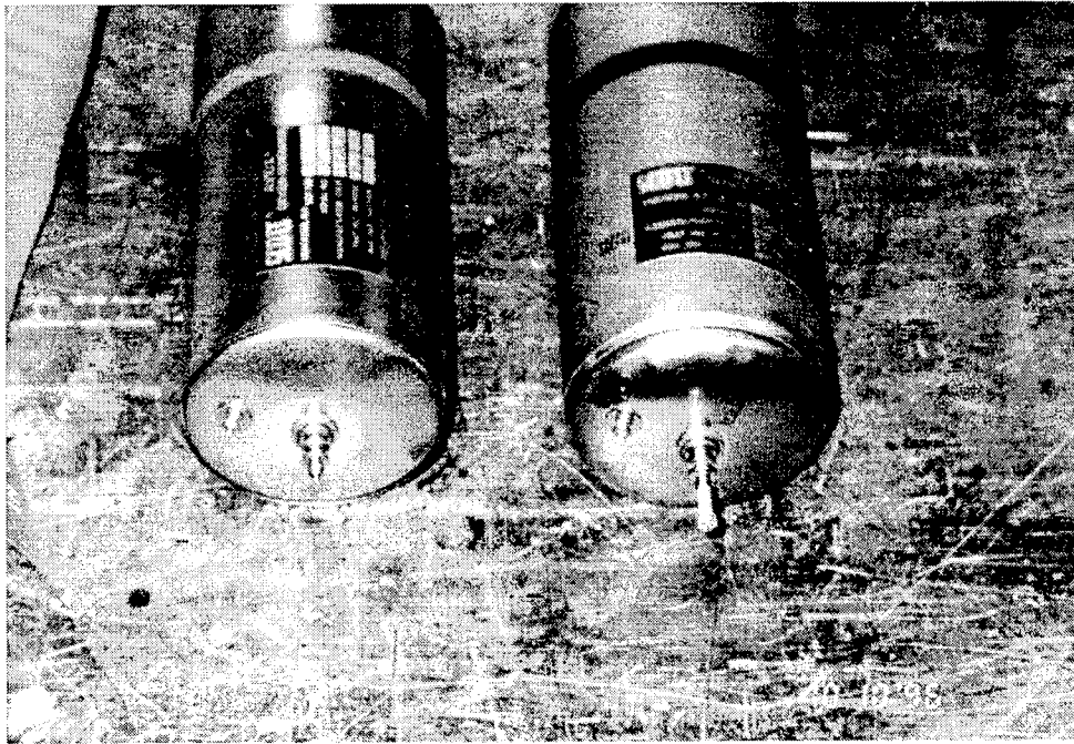
FIGURE 5. GENERATORS OVERPRESSURIZED AFTER PLUGGING THE OUTLETS AND ACTIVATED
