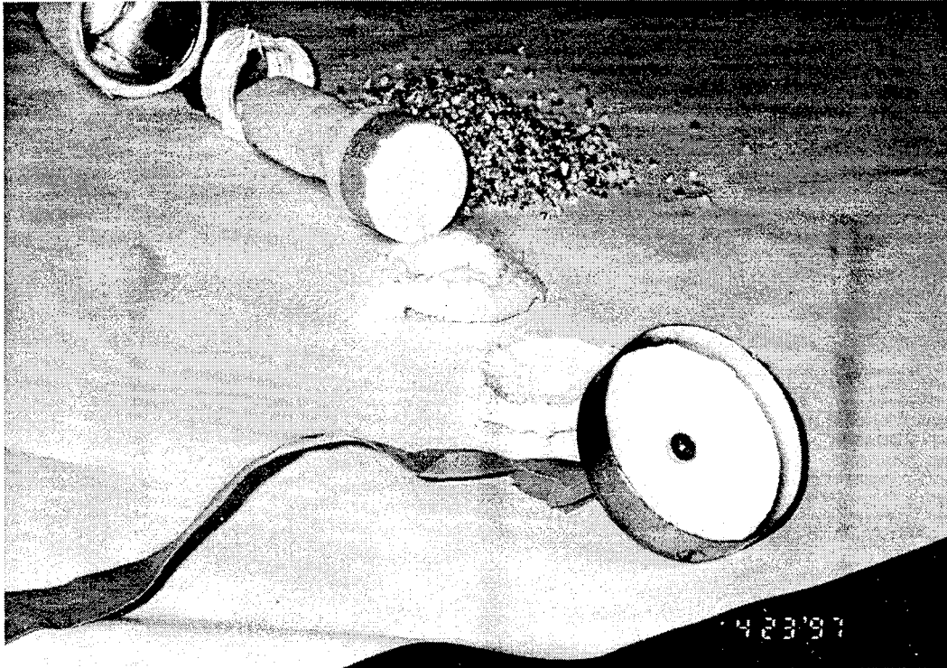
FIGURE 16. DISASSEMBLED GENERATOR
