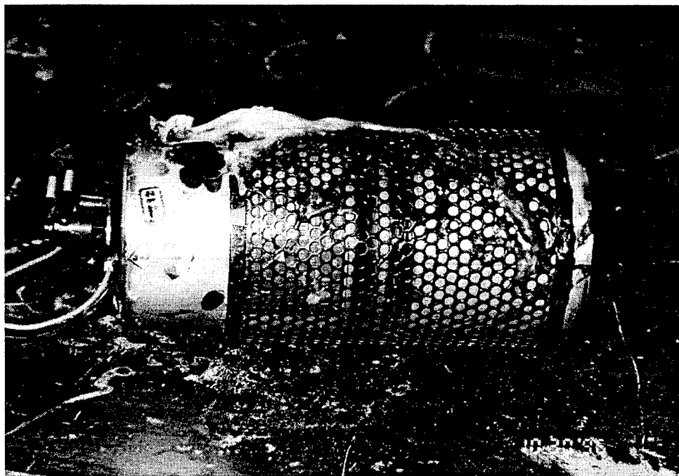
FIGURE 15. ELECTRICALLY ACTIVATED GENERATOR WITH HEAT SHIELD AND MELTED BUBBLE PLASTIC
