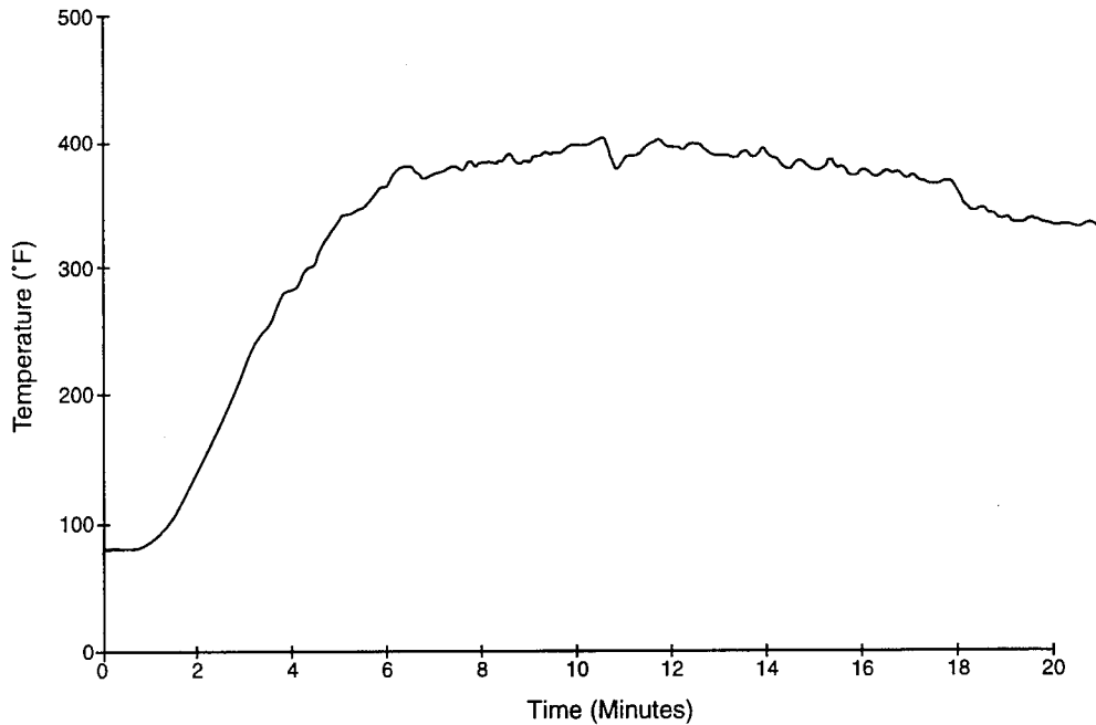
FIGURE 10. RESULTS OF THE SPOT-WELDED GENERATOR TEST
