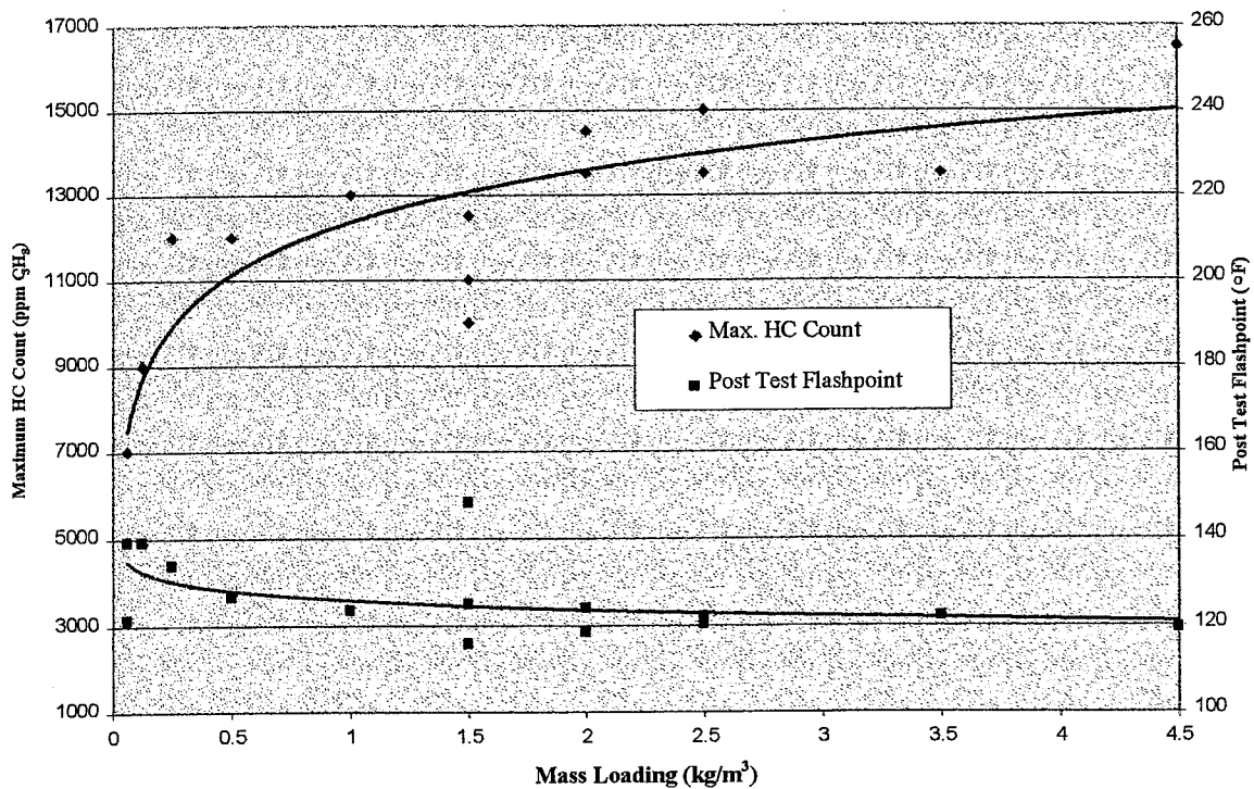
FIGURE 3. MAXIMUM HYDROCARBON COUNT (ppm C 3 H 8 ) AND POSTTEST FLASHPOINT (°F) AS A FUNCTION OF MASS LOADING
