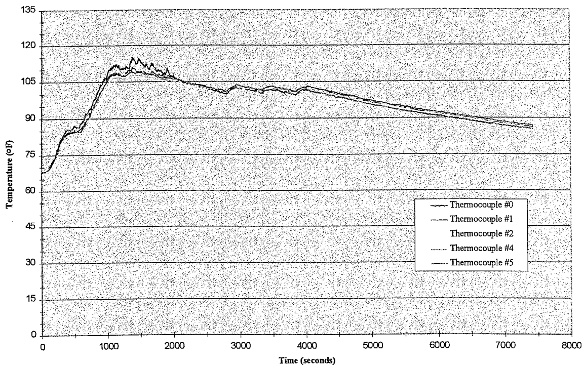
FIGURE 5. TYPICAL ULLAGE TEMPERATURE (°F) PROFILES
