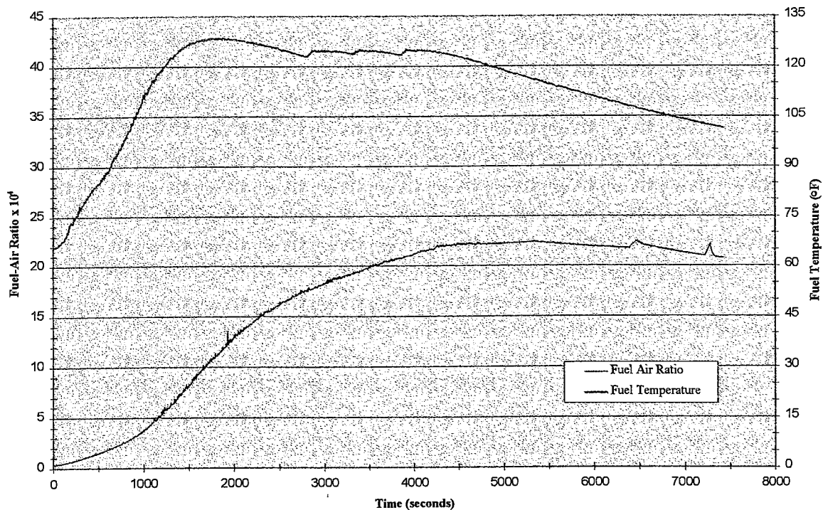
FIGURE 4. TYPICAL FUEL AIR RATIO AND FUEL TEMPERATURE (°F) PROFILES
