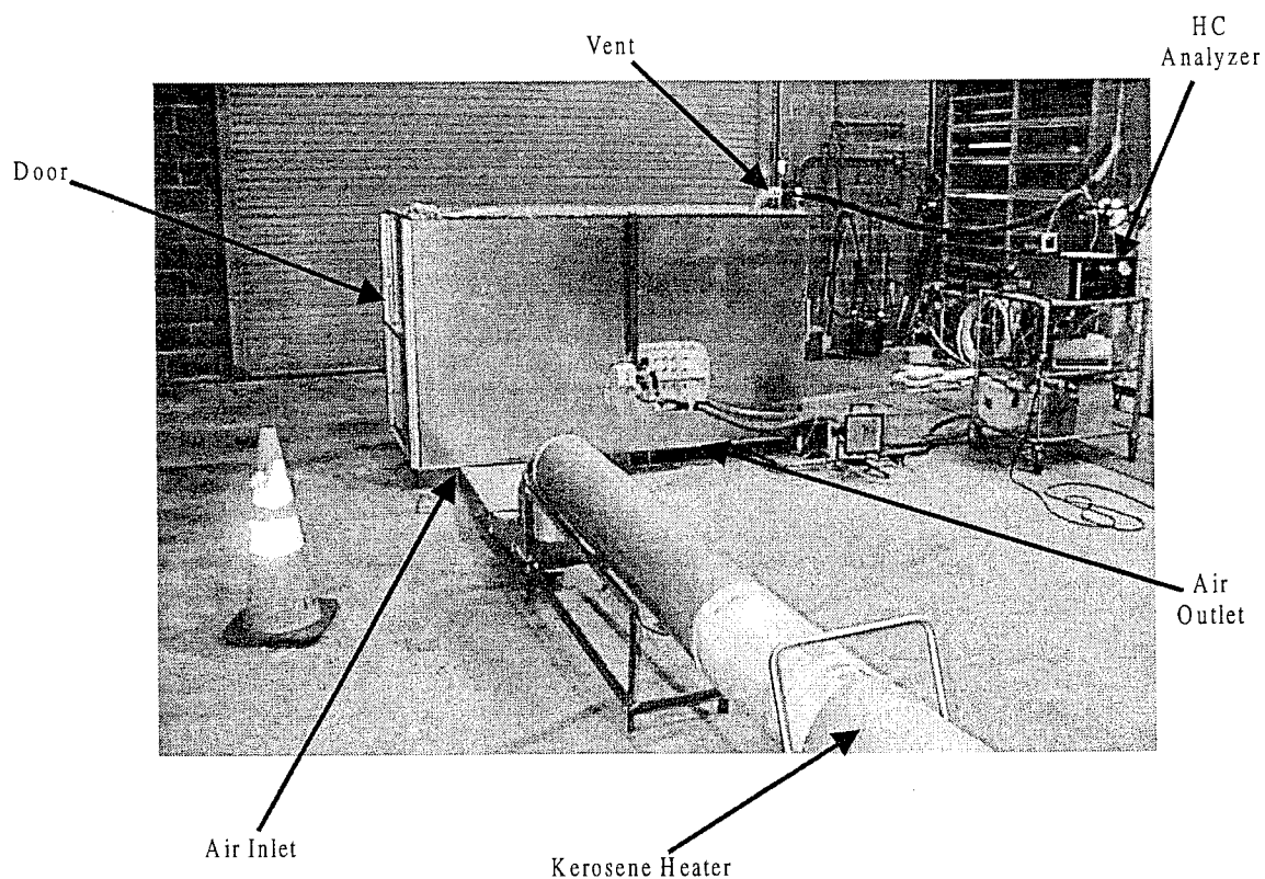
FIGURE 1. TEST SETUP
