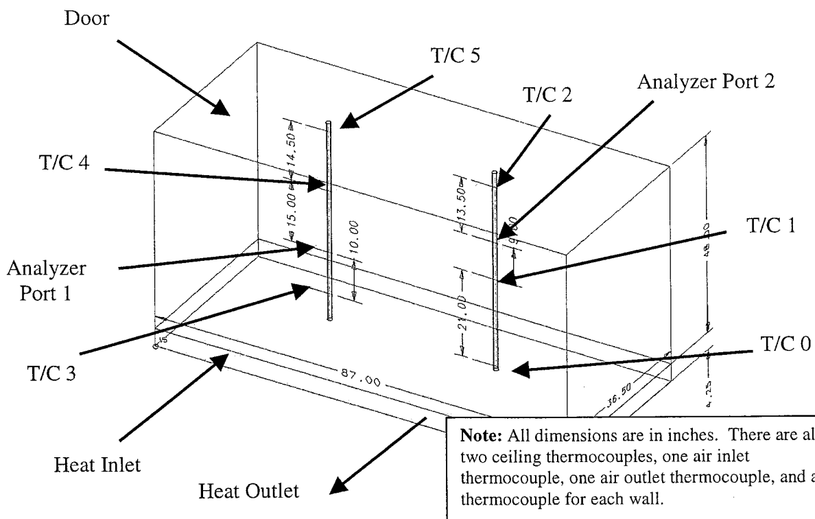
FIGURE 2. THERMOCOUPLE AND ANALYZER PORT LOCATIONS
