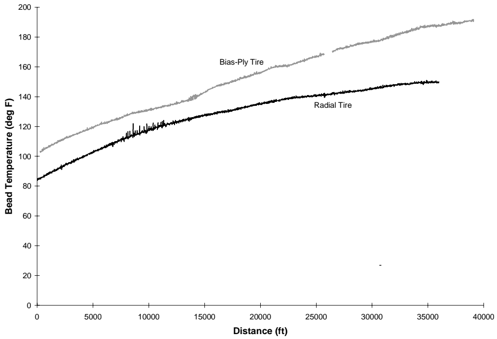
FIGURE 4. RADIAL AND BIAS-PLY TIRE HEATING DURING 10-MPH TAXI WITH 24,000-LB TIRE LOAD
