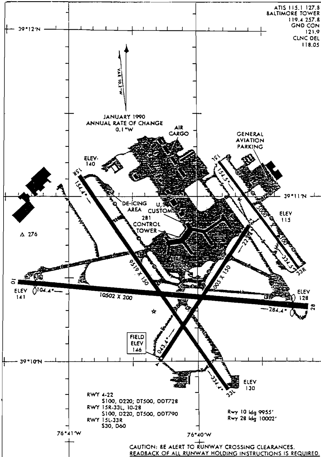
FIGURE 3. DIAGRAM—BALTIMORE-WASHINGTON INTERNATIONAL AIRPORT (BWI), MARYLAND
