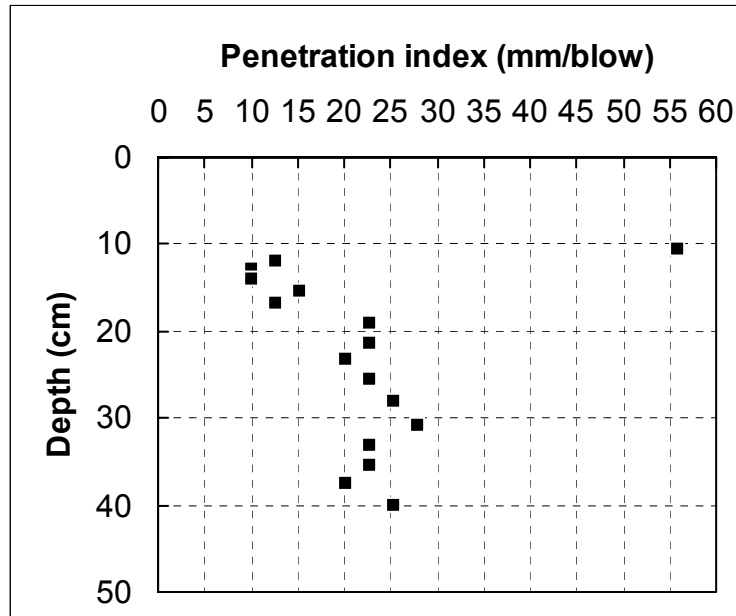
Figure 3.30 Log of DCPT for the site of US35 in Knox, IN (Station: 2+150, Test No. 1)
