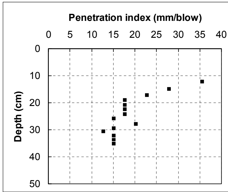
Figure 3.23 Log of DCPT for the site of I-80/I-94 in Gary, IN (Station: 342+000, Test No. 5)
