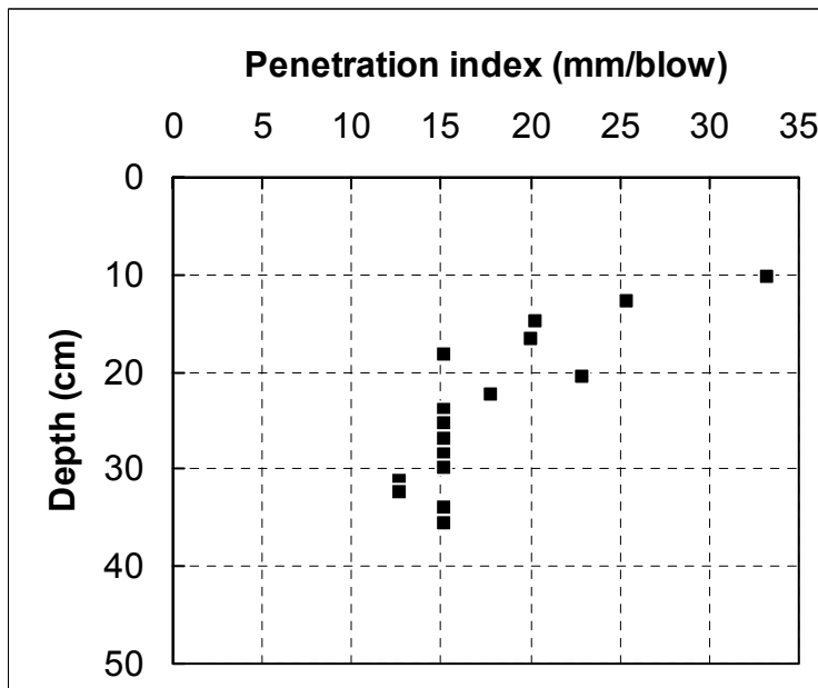
Figure 3.22 Log of DCPT for the site of I-80/I-94 in Gary, IN (Station: 342+000, Test No. 4)
