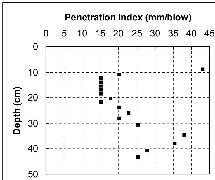
Figure 3.31 Log of DCPT for the site of US35 in Knox, IN (Station: 2+150, Test No. 2)
