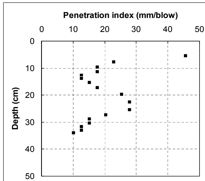
Figure 3.43 Log of DCPT for the site of Lindberg Road in West Lafayette, IN (Station: 1+211, Test No. 3)
