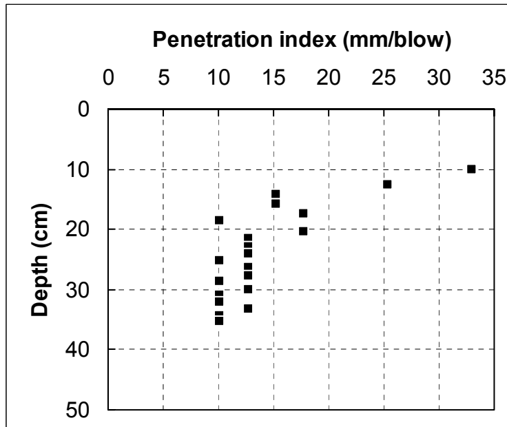
Figure 3.21 Log of DCPT for the site of I-80/I-94 in Gary, IN (Station: 342+000, Test No. 3)
