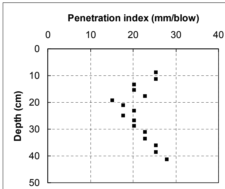
Figure 3.33 Log of DCPT for the site of US35 in Knox, IN (Station: 2+150, Test No. 4)
