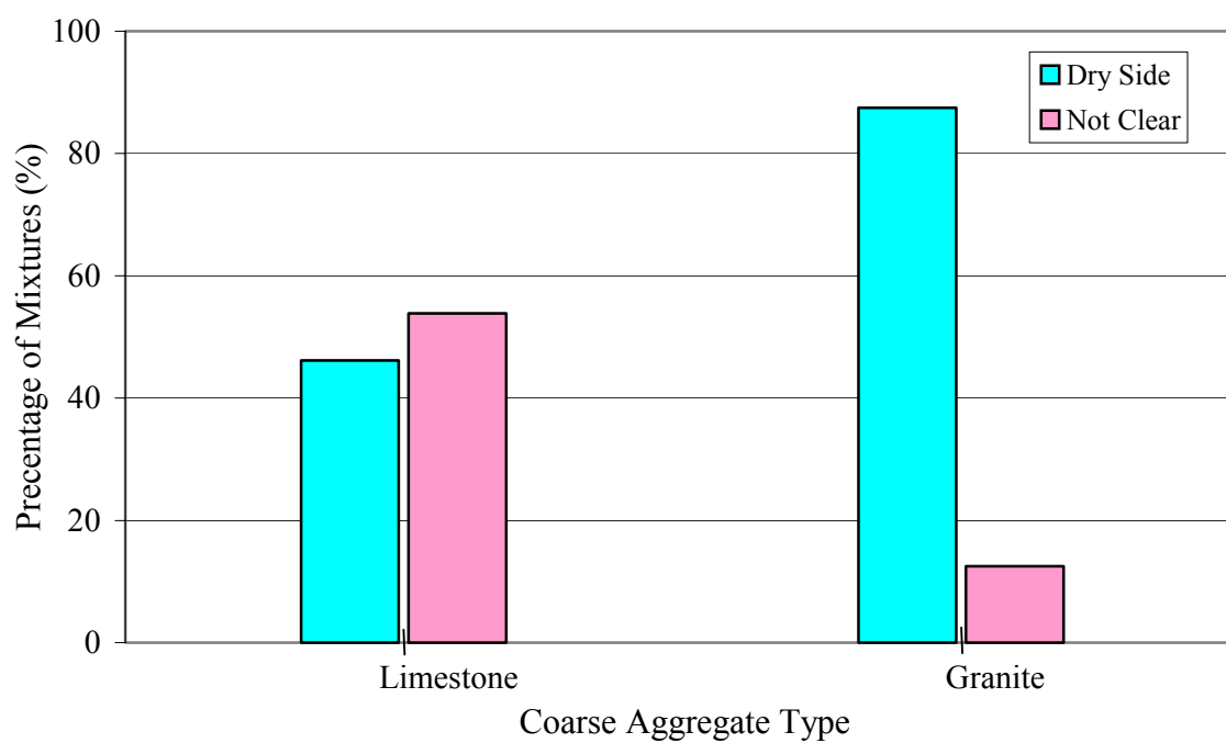
Figure 9.12 Effect of Coarse Aggregate Type on Location of Design AC on VMA Curve at N_{\text{design}} Gyration.
