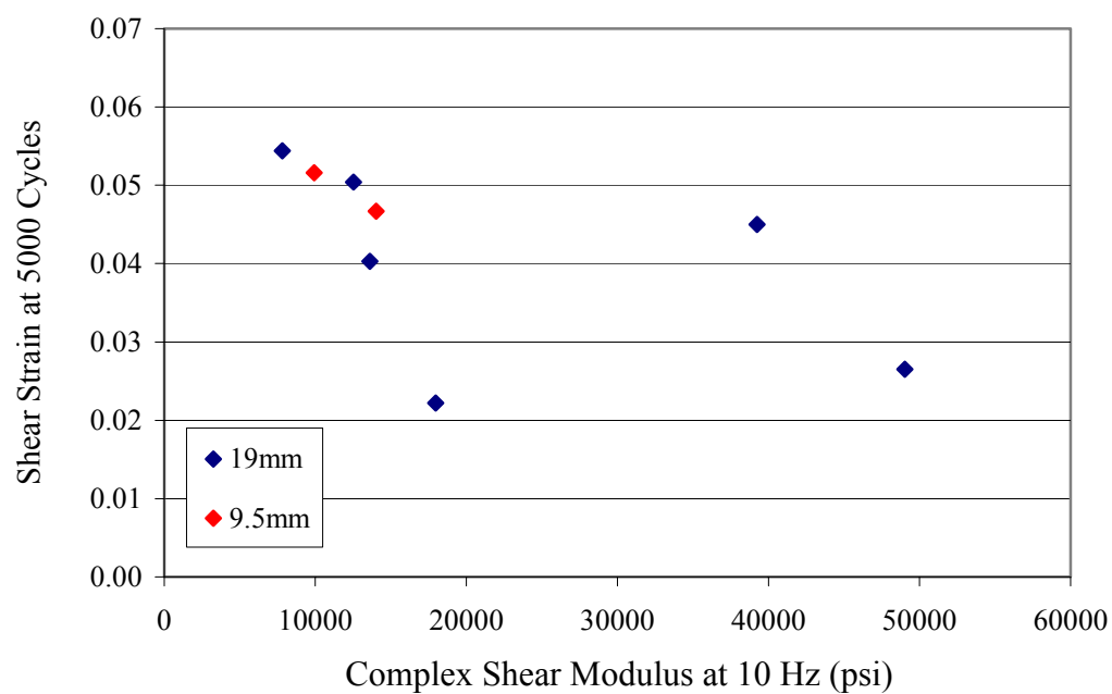
Figure 7.50 Scatter Plot of RSCH and FSCH Test Results for FMFC Specimens (50 0 C).
