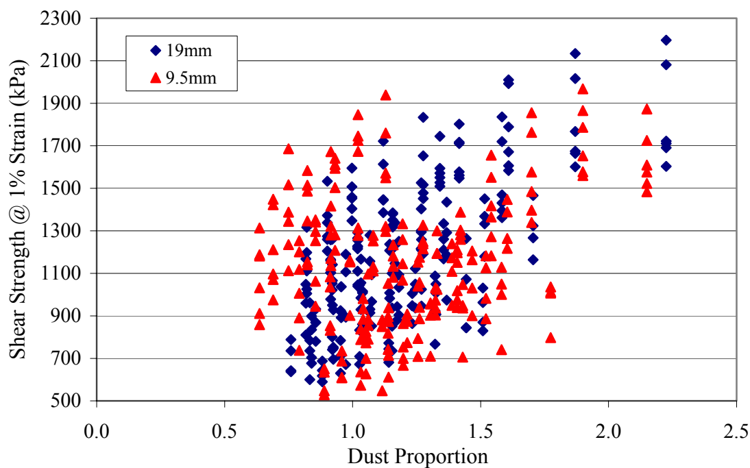
Figure 9.62 Effect of Dust Proportion on Triaxial Test Results.
