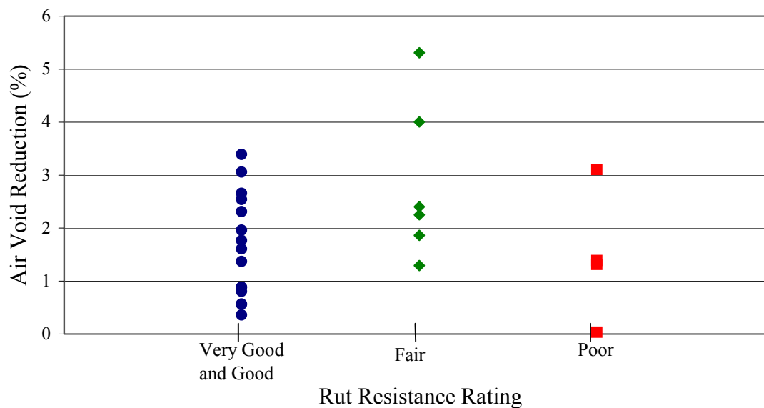
Figure 4.30 Scatter Plot of Reduction in Air Void and Rut Resistance Rating
