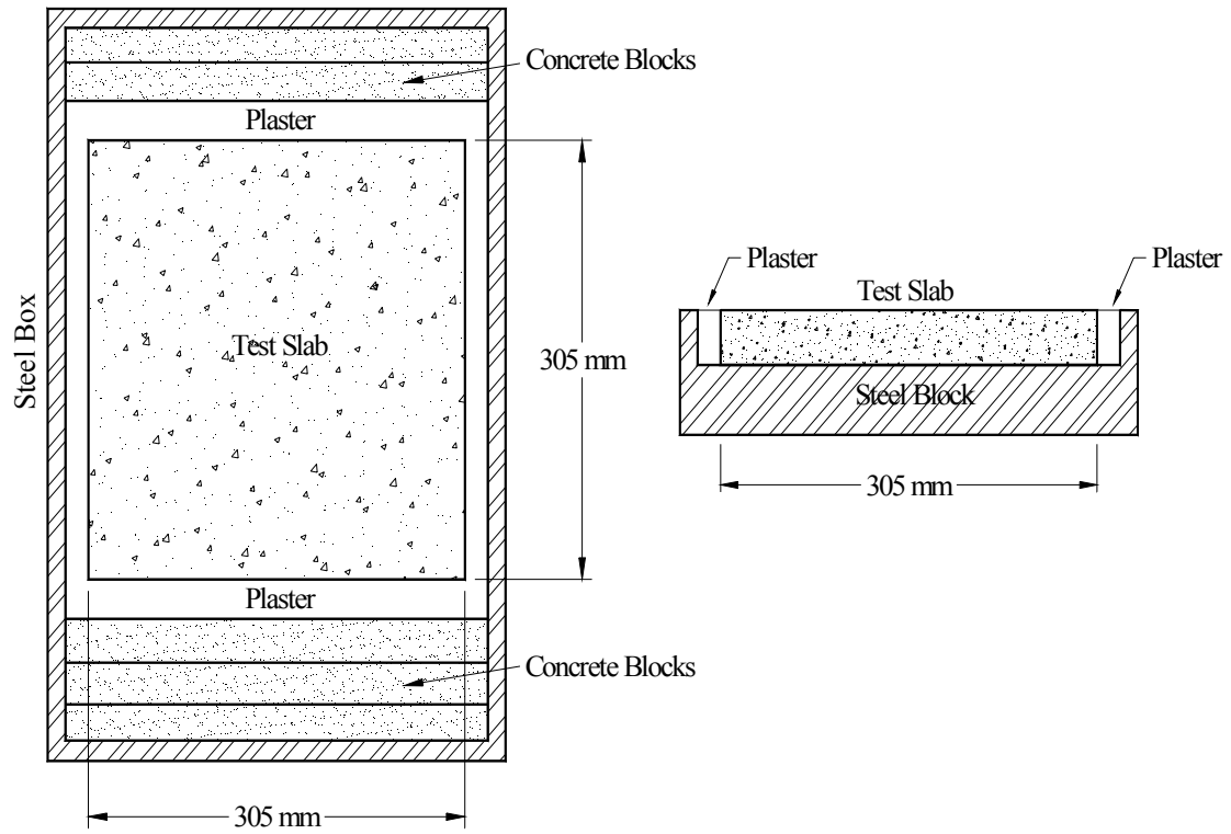
Figure 5.3 Schematic of Sample Mounting Box.
