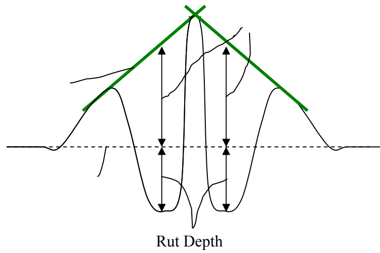
Figure 4.5 Definition of Rutting Components without Wander.
