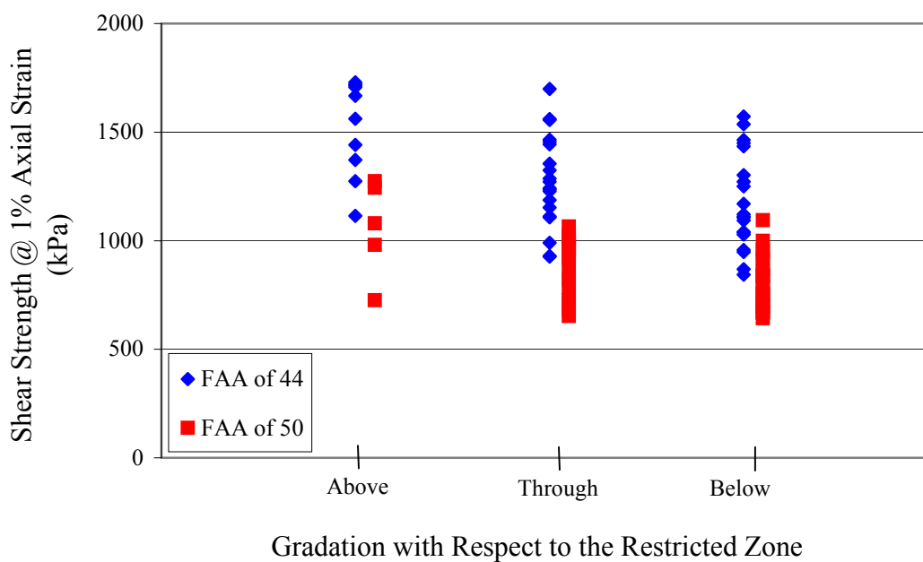
Figure 9.42 Effect of Gradation on Triaxial Test Results.
