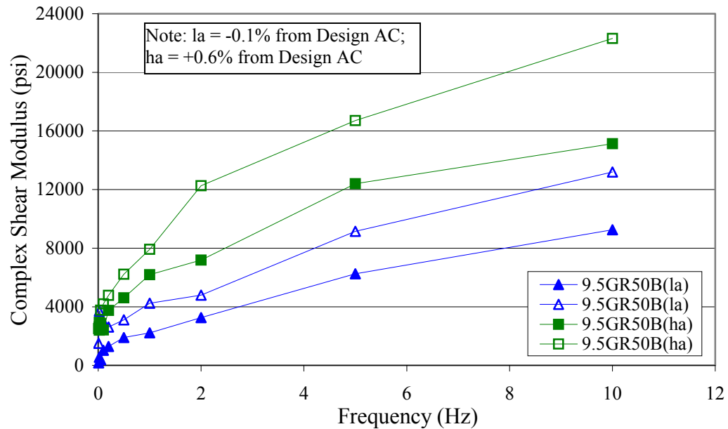
Figure 7.9 Frequency Sweep Test at Constant Height Result for 9.5mm Granite with FAA of 50 and Gradations Plotting Below The Restricted Zone FMFC Specimens (50°C).
