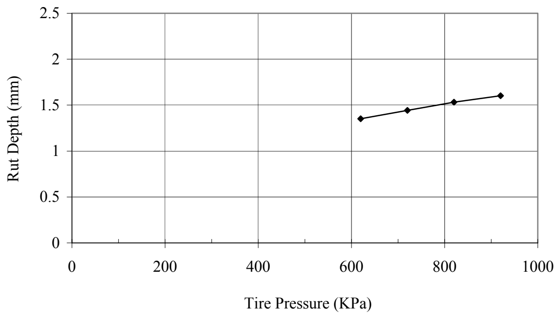
Figure 8.22 Modeling Tire Inflation Pressure Effect for PURWheel Tests.
