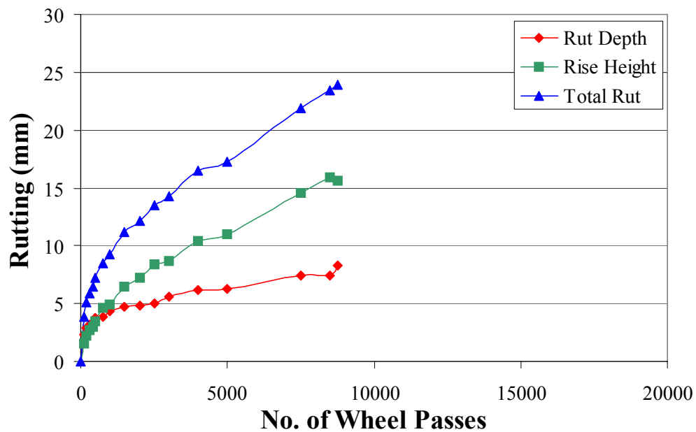
Figure C. 2 No Wander Rutting for 19 mm Limestone with FAA of 39, Gradation Plotting Below The Restricted Zone, High Density Lane.
