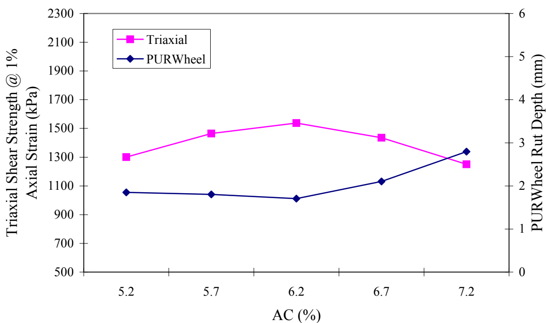
Figure 6.21 Triaxial Shear Strength and PURWheel Rut Depth of 9.5mm Limestone with FAA of 44 and Gradation Plotting Below the Restricted Zone Mixture.
