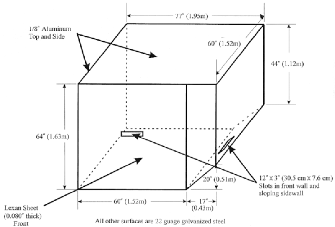
FIGURE 5. LD-3 CONTAINER
