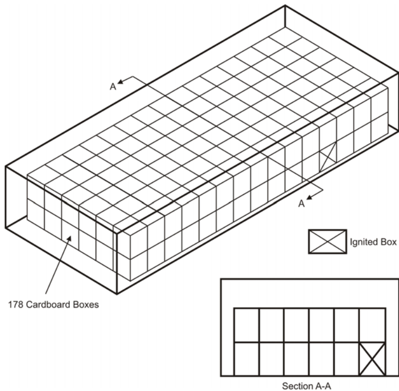
FIGURE 2. BULK-LOAD FIRE TEST SETUP
