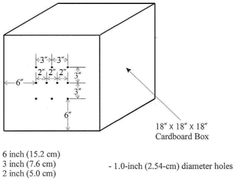
FIGURE 3. IGNITER BOX
