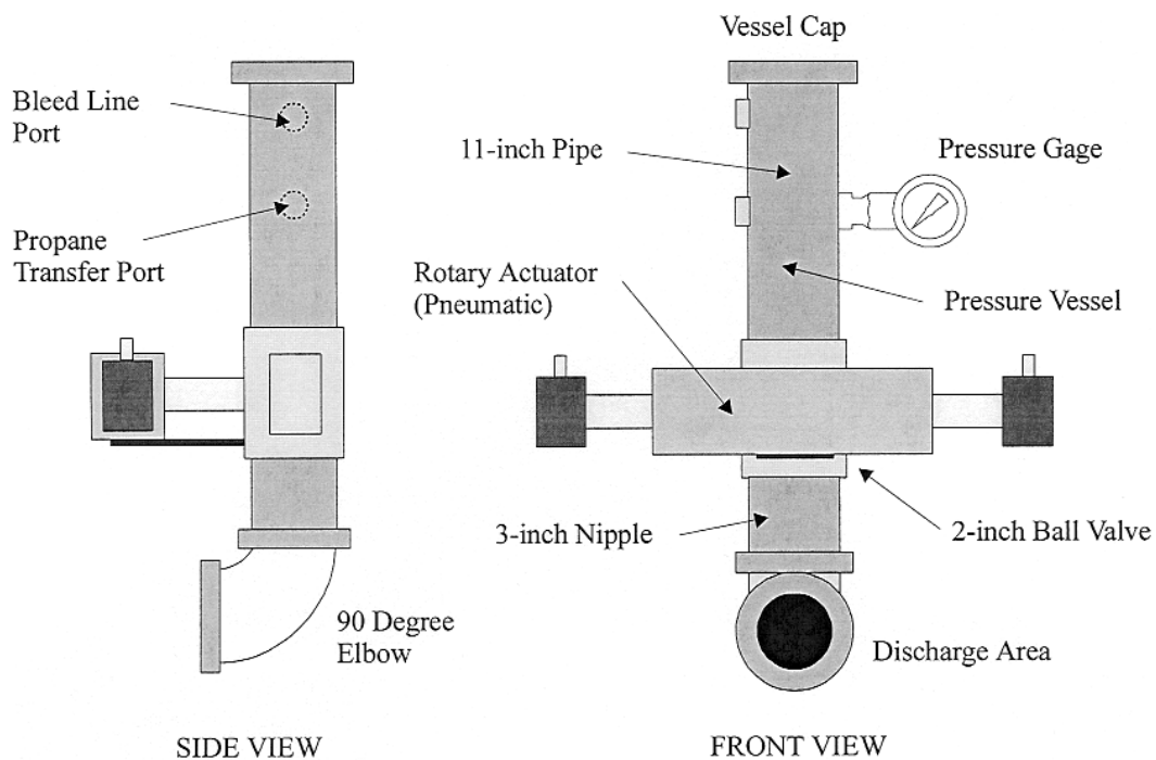
FIGURE 8. SCHEMATIC OF AEROSOL EXPLOSION SIMULATOR
