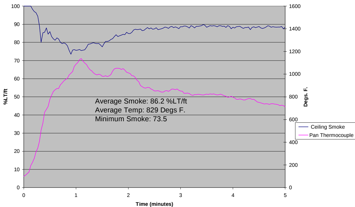
FIGURE 5. SAMPLE JP8 SMOKE DENSITY DATA
