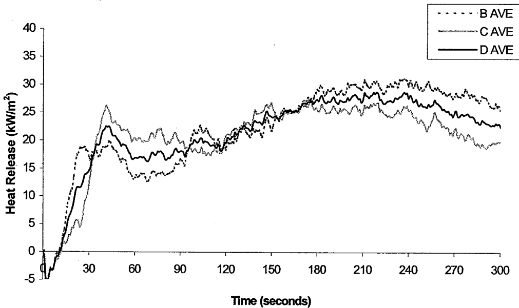
FIGURE 5. HEAT RELEASE AVERAGE (POINT-BY-POINT) OF PANELS B, C, AND D
