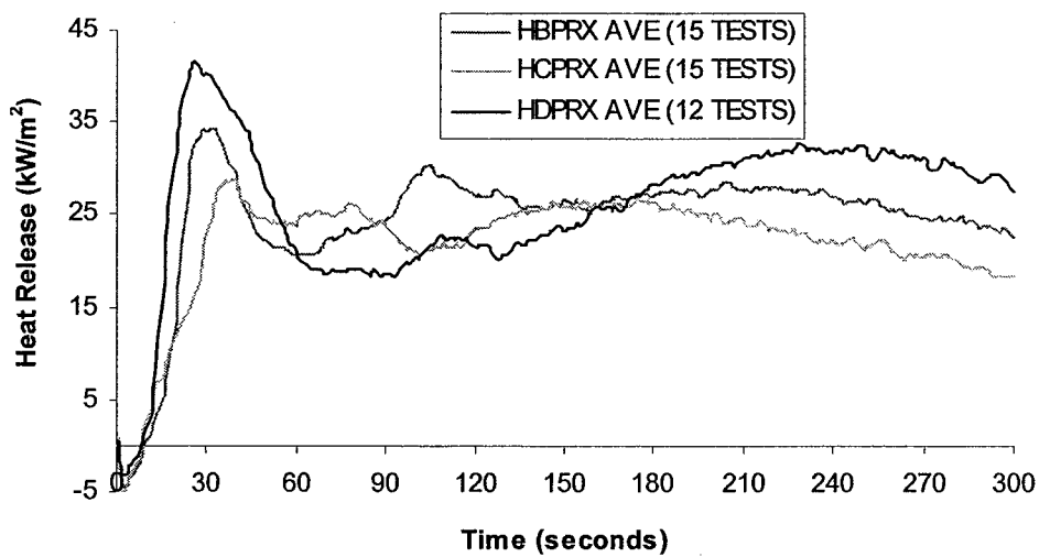
FIGURE 7. HEAT RELEASE AVERAGE (POINT-BY-POINT)—COMPARISON OF PANELS B, C, AND D FINISHED WITH PAINT R
