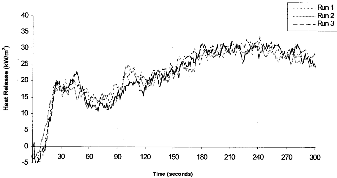
FIGURE 2. PANEL B HEAT RELEASE RESULTS (Bare panel)
