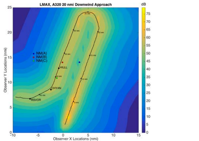
Figure 21. A320 approach procedure to Runway 22L at Boston Logan Airport with calculated maximum noise level contours overlaid for the as-flown speed profile.
