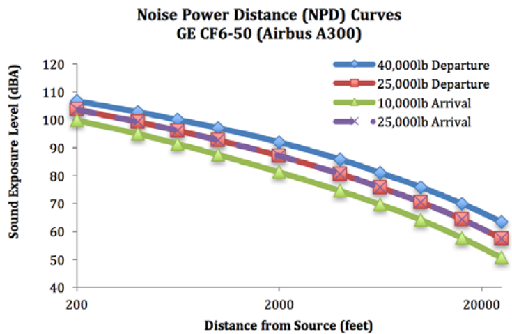
Figure 1. Sample Noise Power Distance (NPD) Curves
