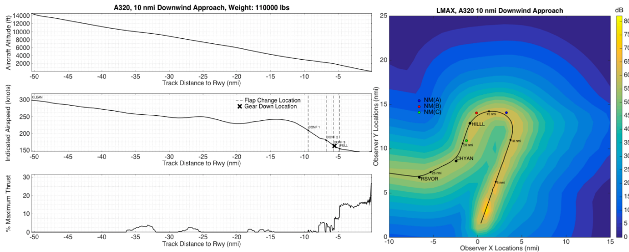
Figure 8. A320 Standard Downwind Approach Flight Profile (left) and Lmax Contour (right)
