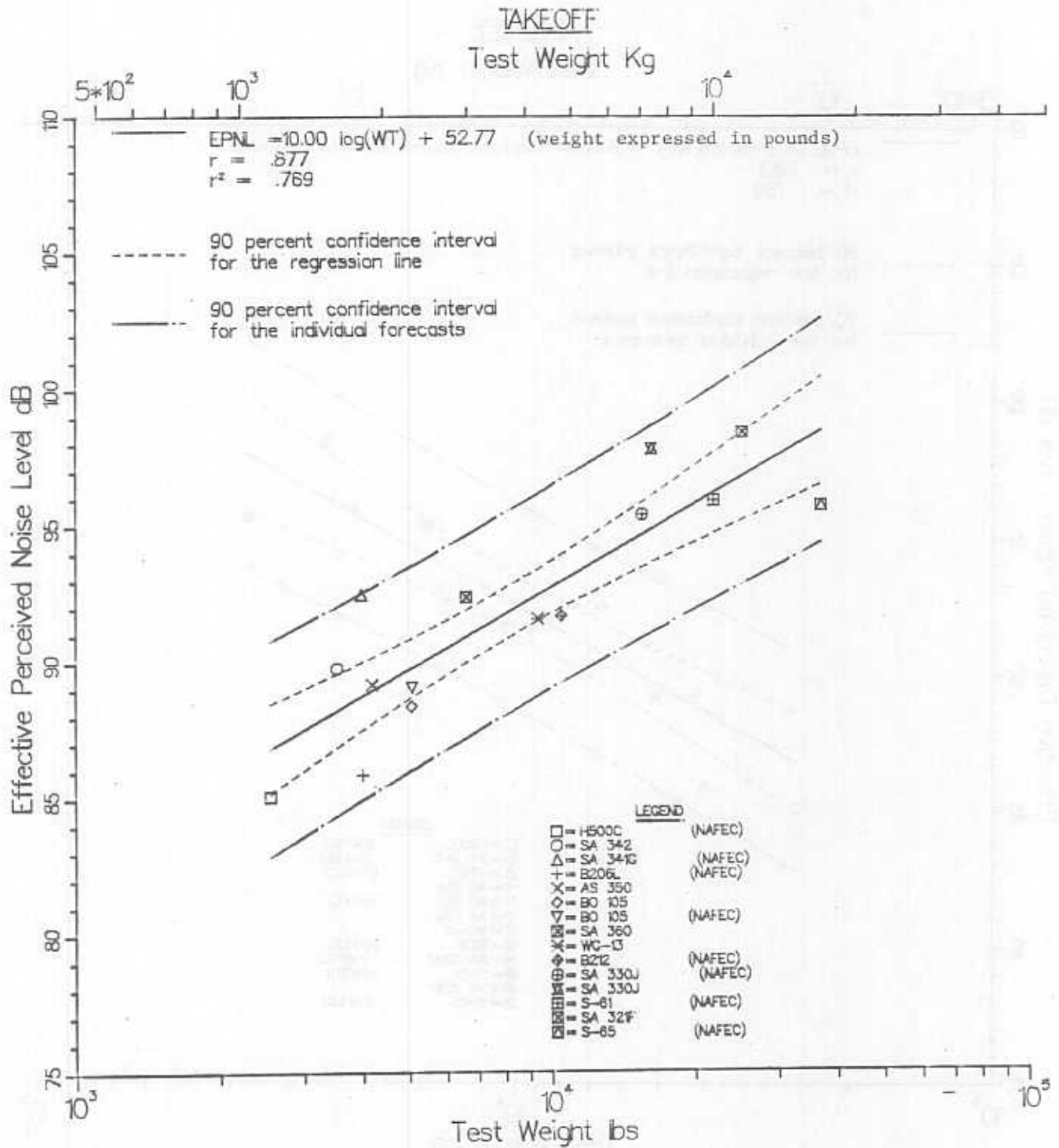
Figure 5.2.2 NAFEC TEST DATA (+) DATA SET 2 CONFIDENCE INTERVAL ANALYSIS
