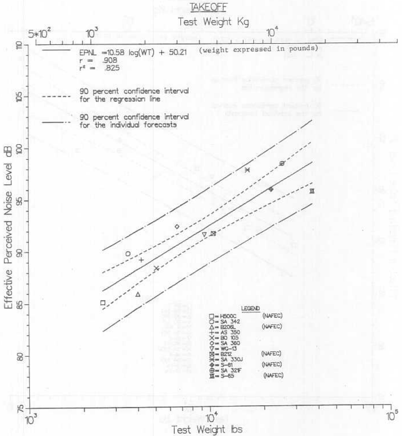
Figure 5.2.4 NAFEC TEST DATA (+) DATA SET 2 (-) NAFEC REPEATS CONFIDENCE INTERVAL ANALYSIS
