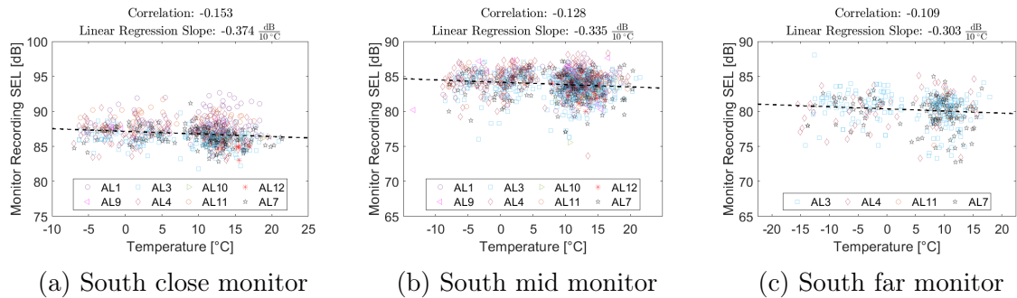
Figure 4-27: Temperature Impact on Noise from Departing A320 Aircraft
