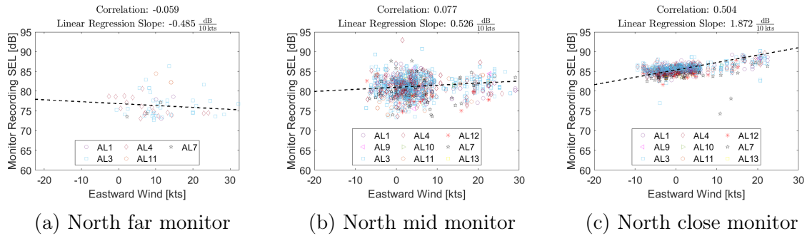
Figure 4-53: Eastward Wind (Crosswind) Impact on Noise from Arriving A320 Aircraft
