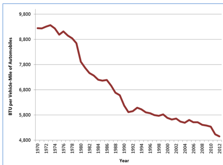
Exhibit 5-3: ORNL Historical Highway Automobile Energy Intensities Data
