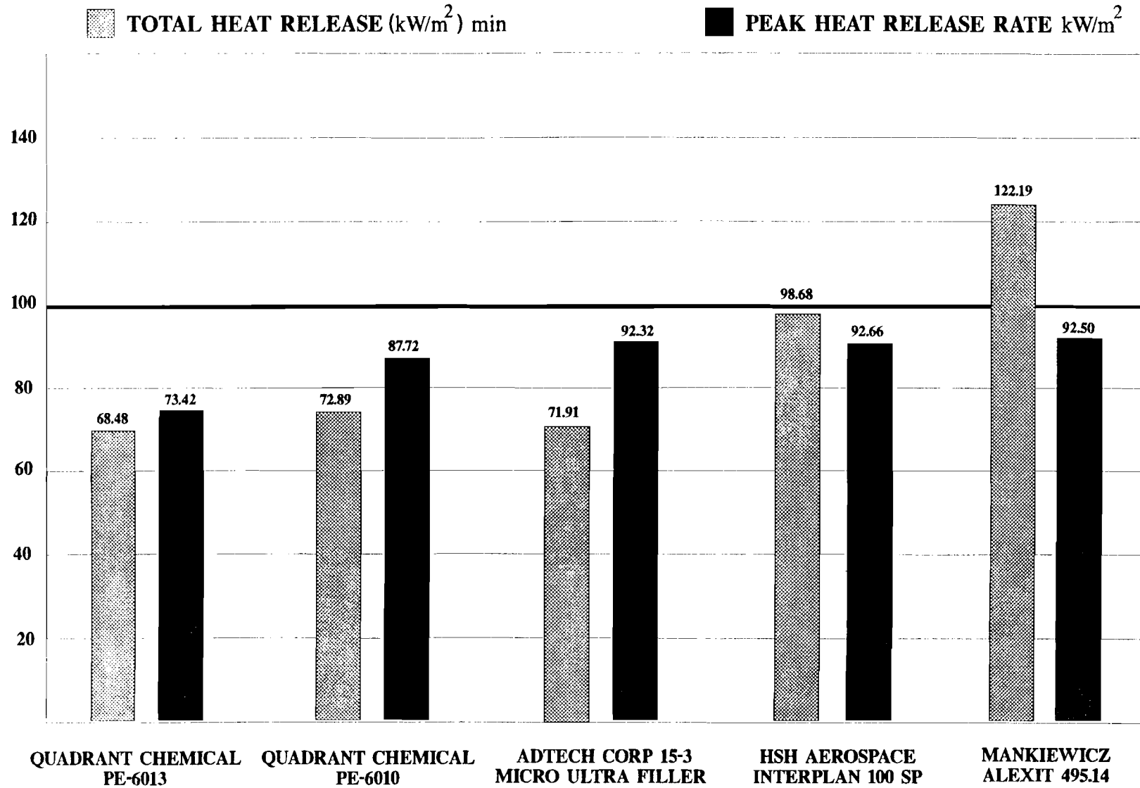
FIGURE 17. SPATULA FILLER TEST RESULTS (0.250 IN.)
