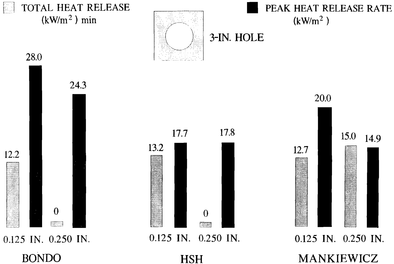
FIGURE 12. SPATULA FILLER TESTS USING STAINLESS STEEL PLATES WITH 3-INCH-DIAMETER HOLES
