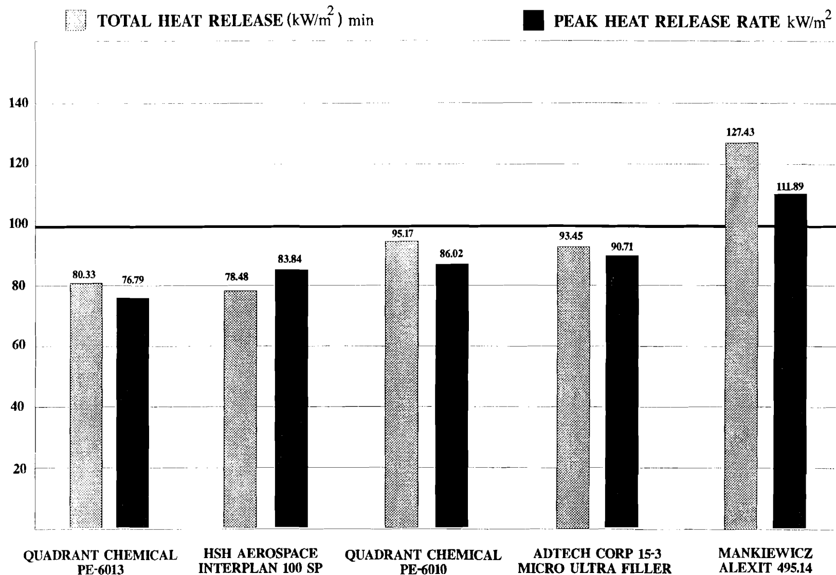
FIGURE 16. SPATULA FILLER TEST RESULTS (0.125 IN.)
