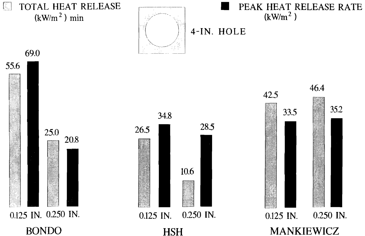
FIGURE 13. SPATULA FILLER TESTS USING STAINLESS STEEL PLATES WITH 4-INCH DIAMETER HOLES
