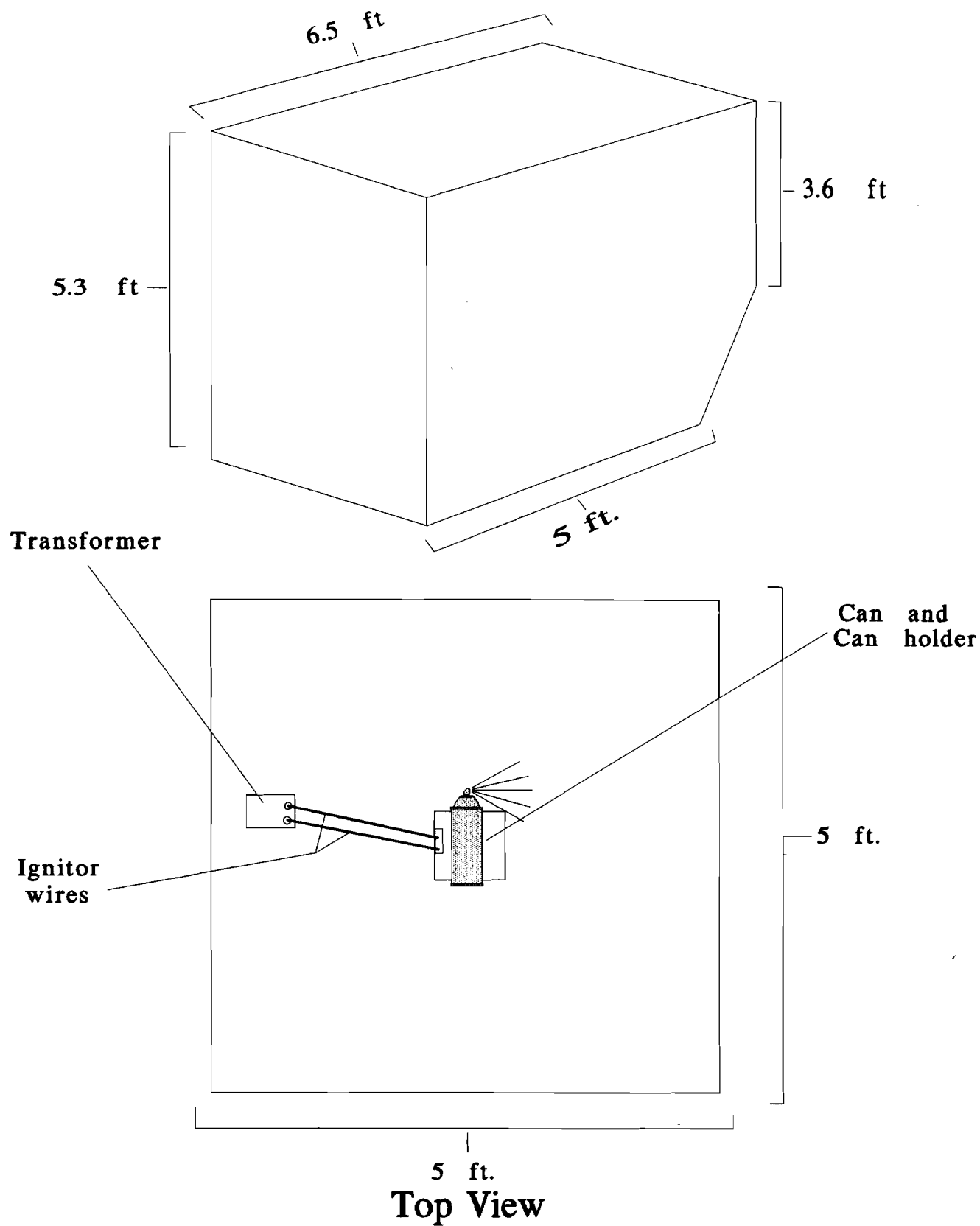
FIGURE 2. LD-3 CONTAINER
