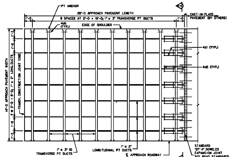
PLAN VIEW SHOWING POST-TENSIONING DUCTS TRANSVERSELY AND LONGITUDINALLY
