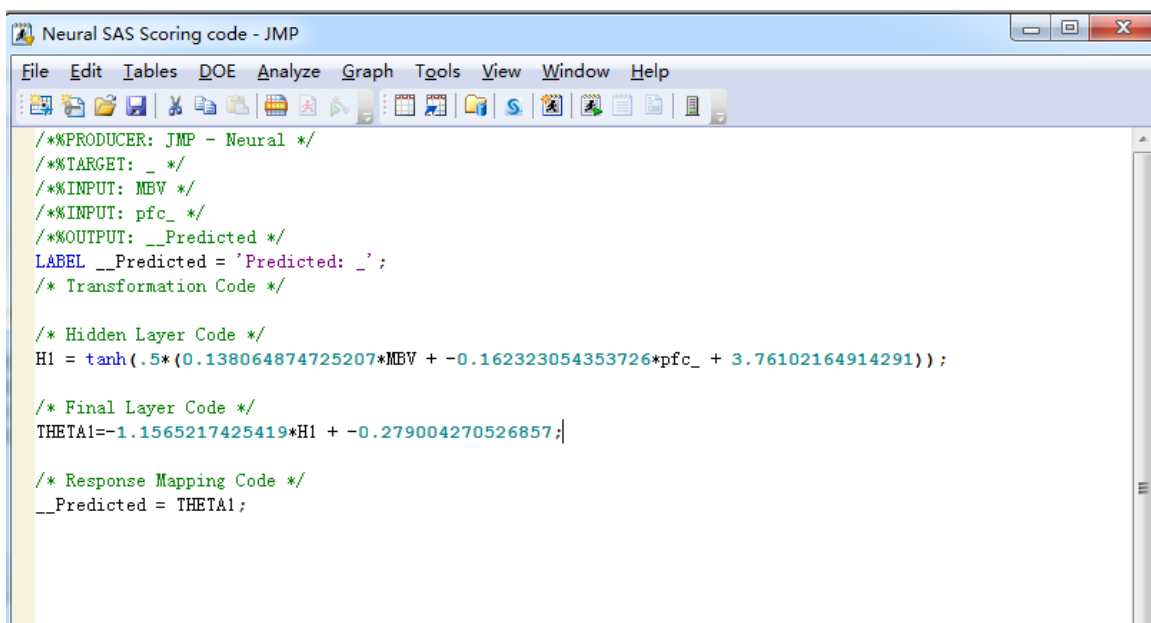
Figure M-6 Make SAS DATA Step
