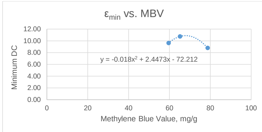
Figure 7-9 the correlation between MBV and \varepsilon_{min} for the three soil samples
