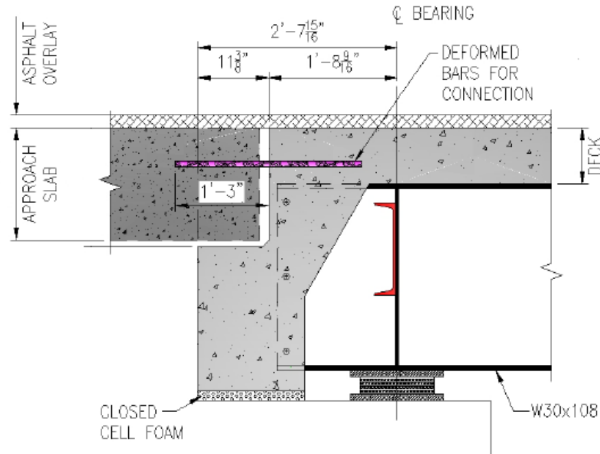
Figure 11-3 Design details of JPrCP BAS – bridge deck connection [66]
