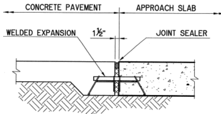
Figure 11-10 BAS – pavement expansion joint detail in Oklahoma [2]
