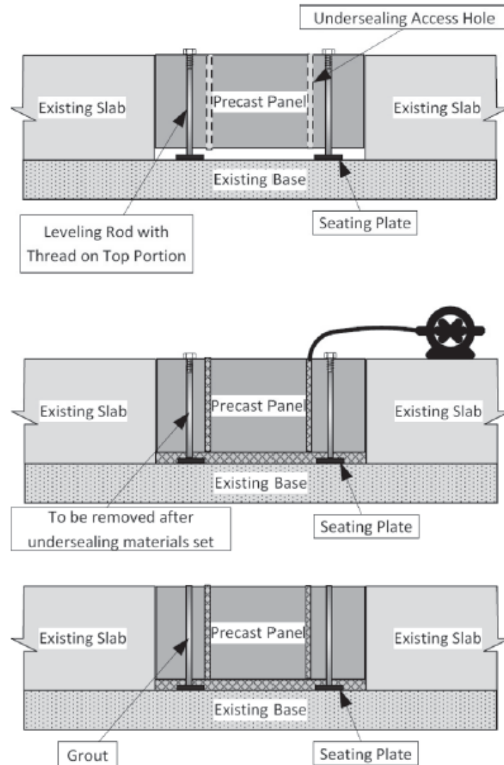
Figure 4-3 Threaded setting bolts installation option [10]
