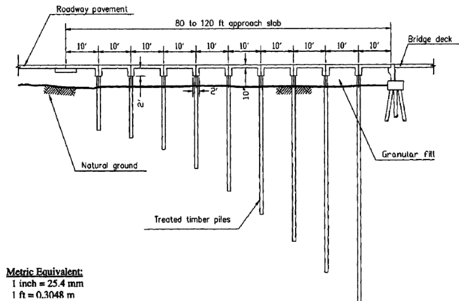
Figure 5-42 Column-supported BASs [96]
