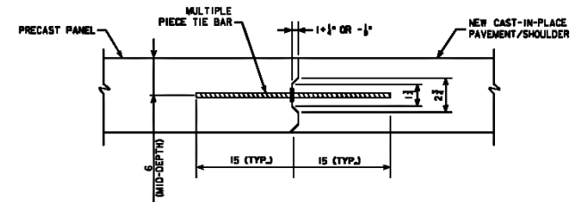
KEYWAY DIMENSIONS LONGITUDINAL JOINTS AT ENDS OF PRECAST PANELS
