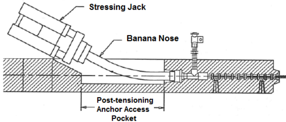
Figure 3-11 Stressing ram with a “banana nose” [22]
