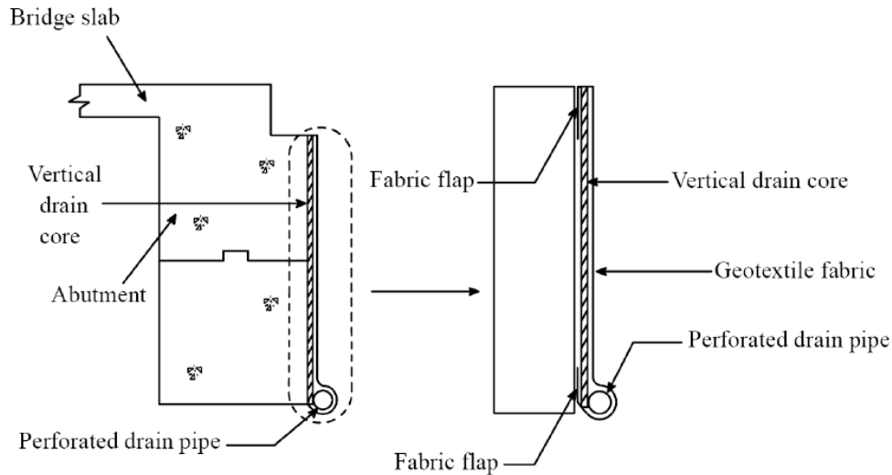
Figure 5-34 Schematic diagram of the use of vertical drain behind abutment [8]
