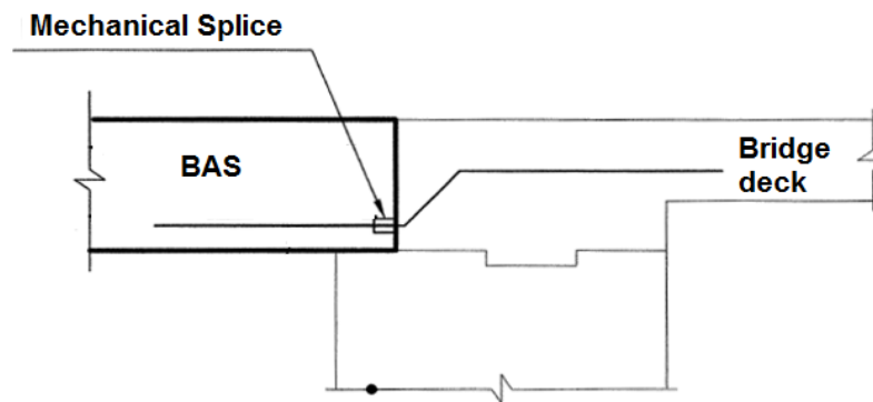
Figure 5-18 Standard design detail for the paving notch connection in Oklahoma [2]
