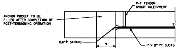
POST-TENSION ANCHORAGE DETAIL FOR DEAD END OF STRANDS
