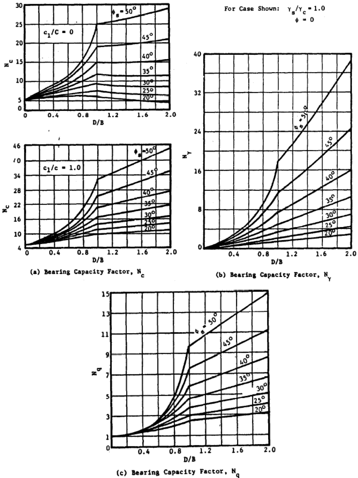
Figure 15-10 Bearing capacity factors for stone column treated soil [118]
