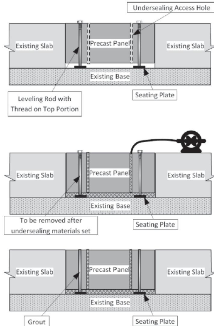
Figure 12-4 Threaded setting bolts installation option [10]
