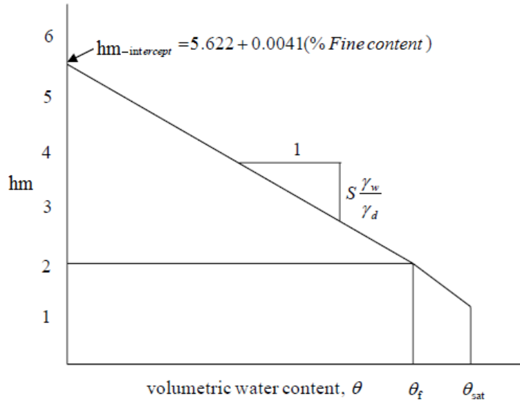
Figure 16-3 The SWCC of a clay soil [144]
