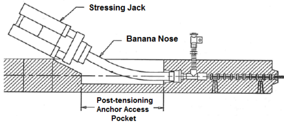
Figure 9-11 Stressing ram with a “banana nose” [22]
