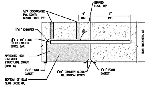
SECTION B-B STANDARD PRECAST TO PRECAST TRANSVERSE TIE
