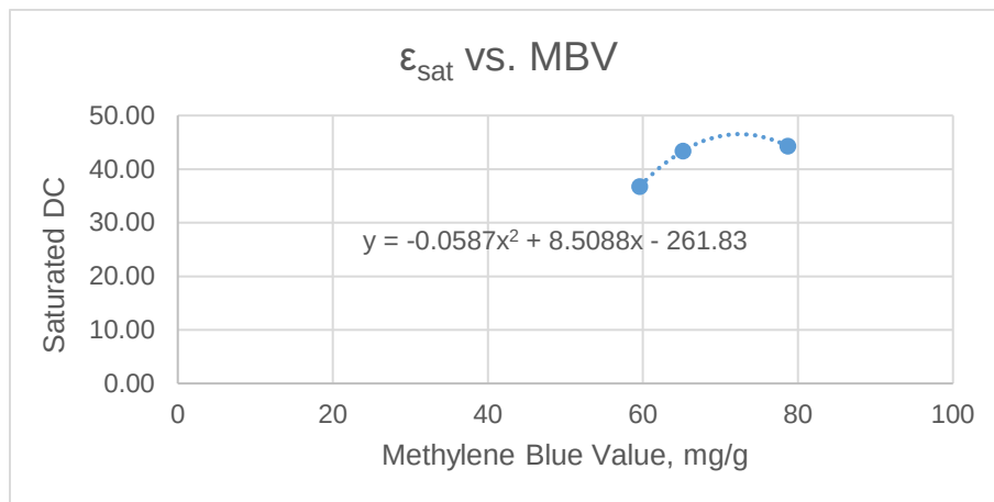
Figure 16-10 the correlation between MBV and \varepsilon_{sat} for the three soil samples
