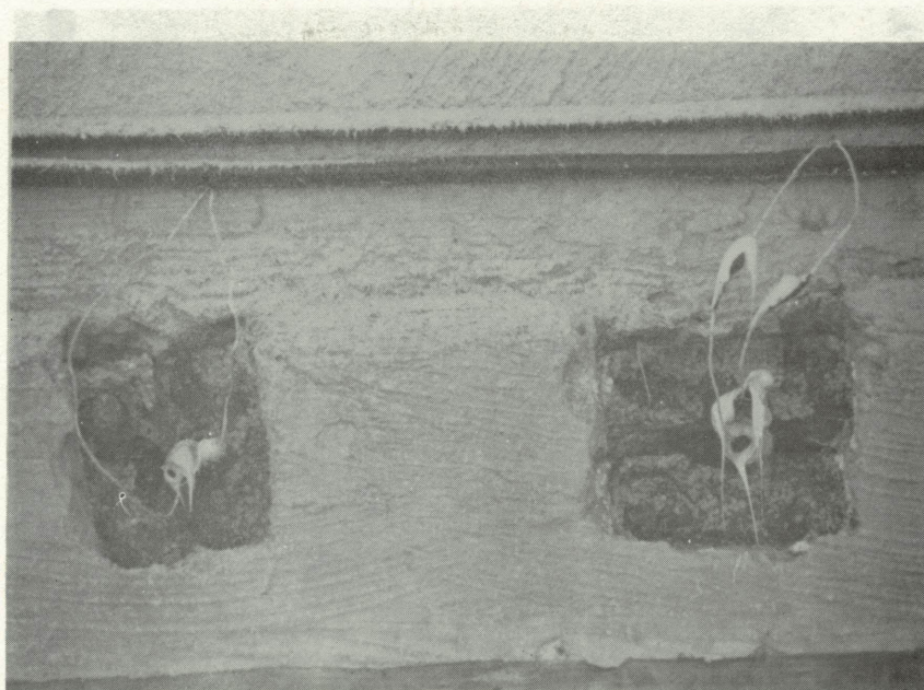
Figure 25: Direct electrical connections to a resistance measurement cell are insulated with caulking material. (A measurement cell consists of two copper conductors and two coated rebars).
