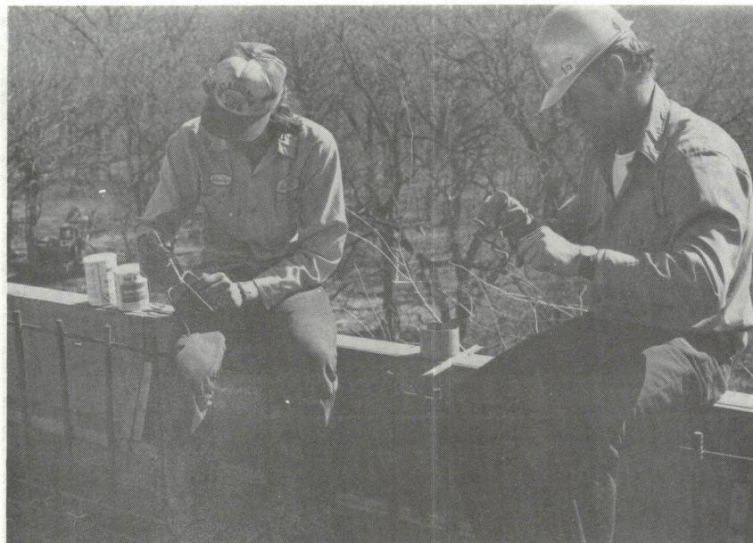
Figure 12: The contractor paints additional chairs with epoxy resin after running out of coated chairs.
