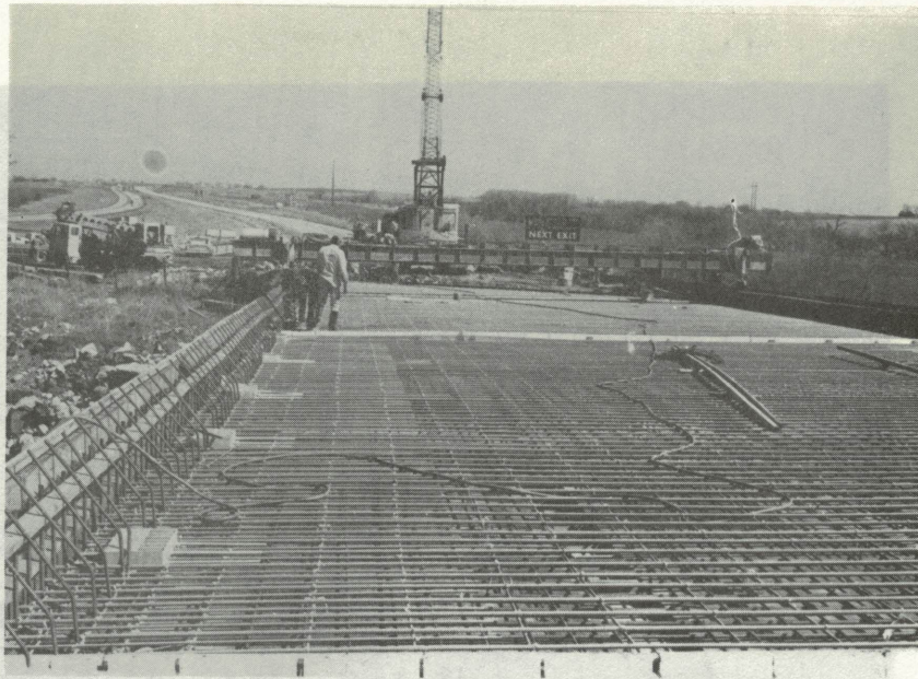
Figure 9: Overall view of the site while concrete was being poured.
