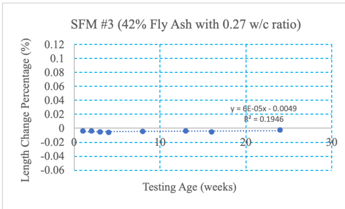
Figure 46. Length change test results for SFM #3
