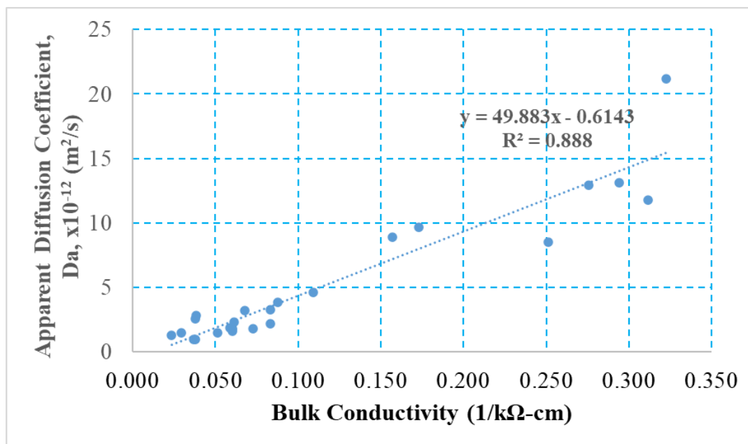
Figure 55. Correlation Between Bulk Conductivity and Apparent Diffusion Coefficient ( D_a )
