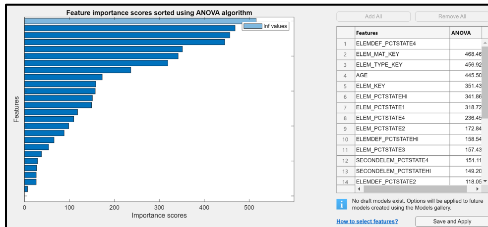
Figure 5.41. ANOVA feature ranking result for Deck Model 7.
