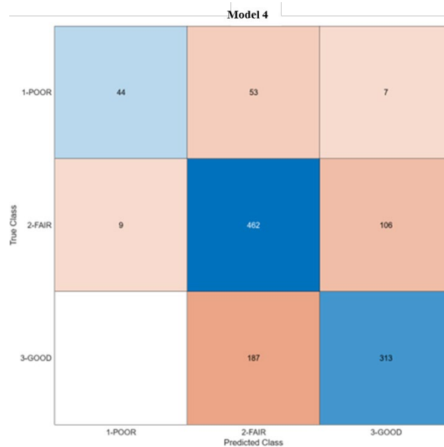
Figure 5.96. Culvert Model 4: Ensemble Classifier (69.3%) Performance, Number of Observations.
