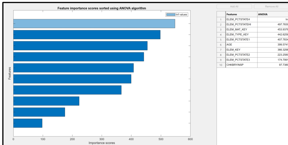
Figure 5.23. ANOVA feature ranking result for Deck Model1.
