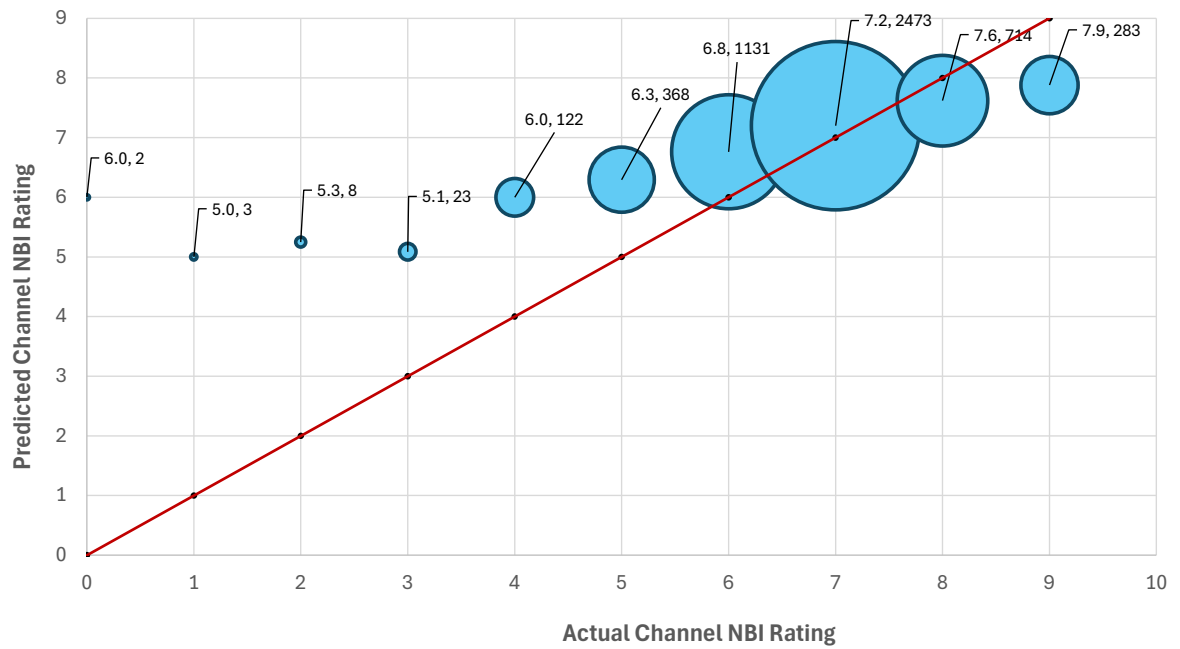
Figure 5.18. Mean predicted Channel NBI Ratings relative to the actual Ratings (showing no. of bridges).
