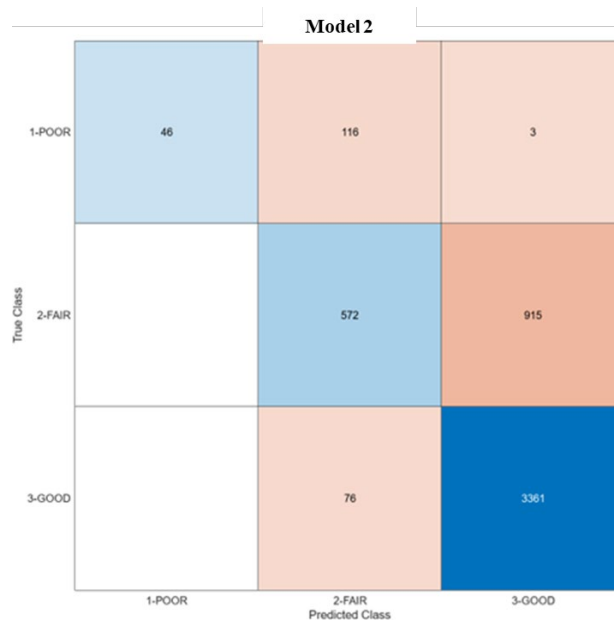
Figure 5.84. Channel Model 2: Decision Tree Classifier (78.2%) Performance, Number of Observations
