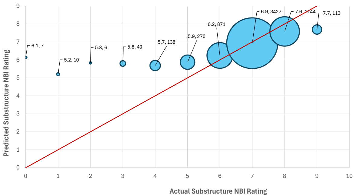
Figure 5.12. Mean predicted Substructure NBI Ratings relative to the actual Ratings (showing no. of bridges).
