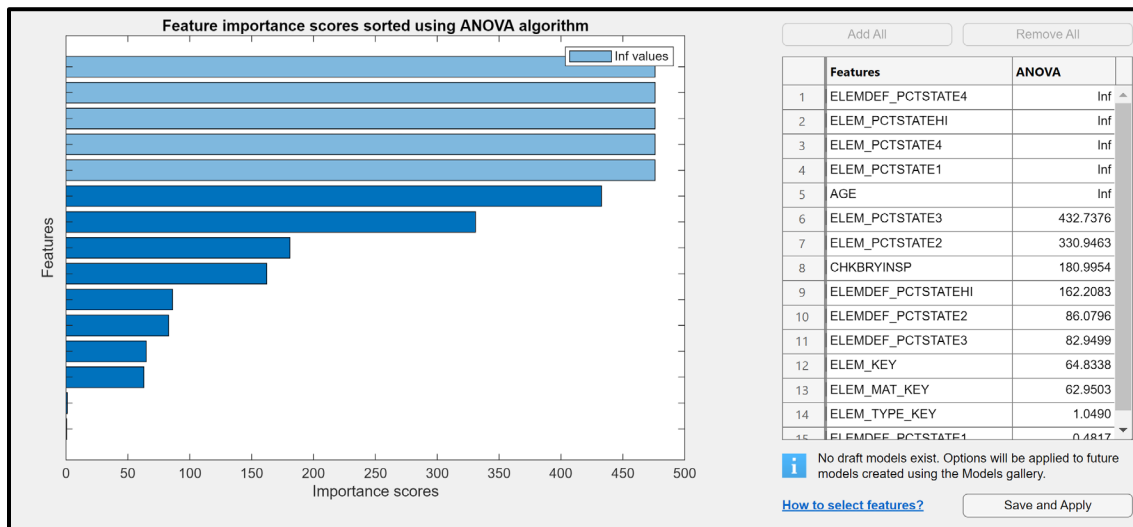
Figure 5.74. ANOVA feature ranking result for Substructure Model 5.
