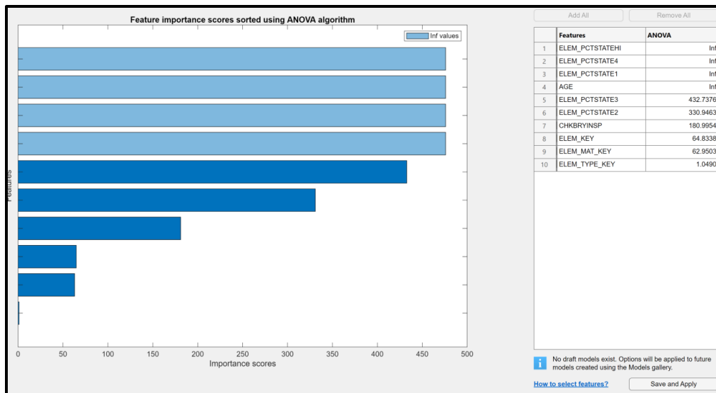
Figure 5.62. ANOVA feature ranking result for Substructure Model 1.
