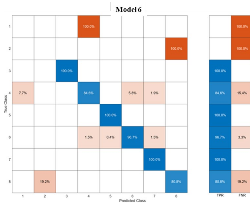
Figure 5.76. Substructure Model 6: Ensemble Classifier (96.1%) Performance, True Positive Rates (TPR), False Negative Rates (FNR)
