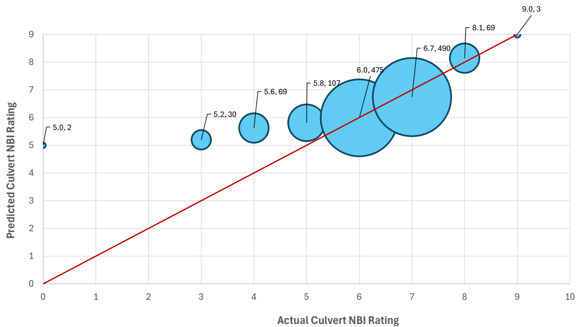
Figure B13. Means of age-based predicted Culvert NBI rating and number of bridges at each actual rating.
