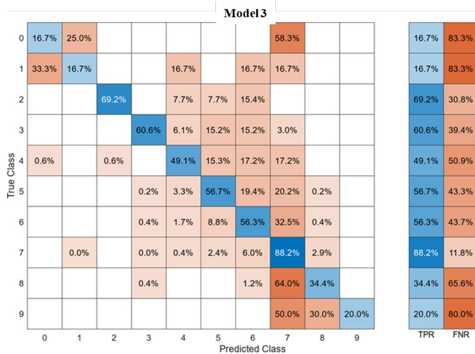
Figure 5.52. Superstructure Model 3: Ensemble Classifier (71.5%) Performance, True Positive Rates (TPR), False Negative Rates (FNR)
