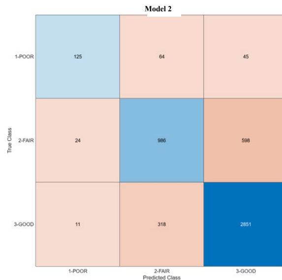
Figure 5.24. Deck Model 2: Ensemble, Bagging Trees Classifier (78.9 %) Performance, Number of Observations
