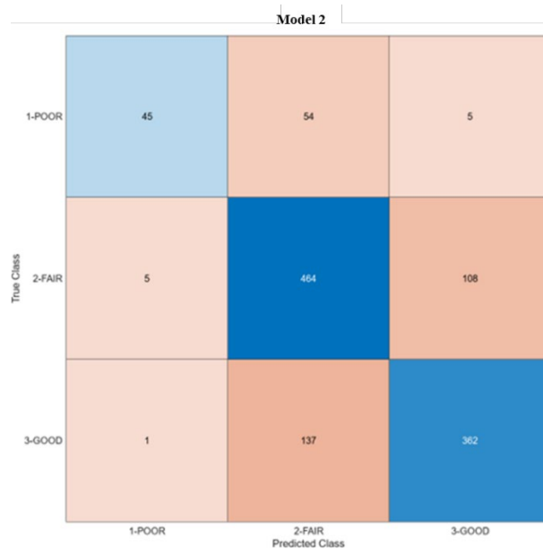
Figure 5.90. Culvert Model 2: Efficient Logistic Regression Classifier (73.8%) Performance, Number of Observations
