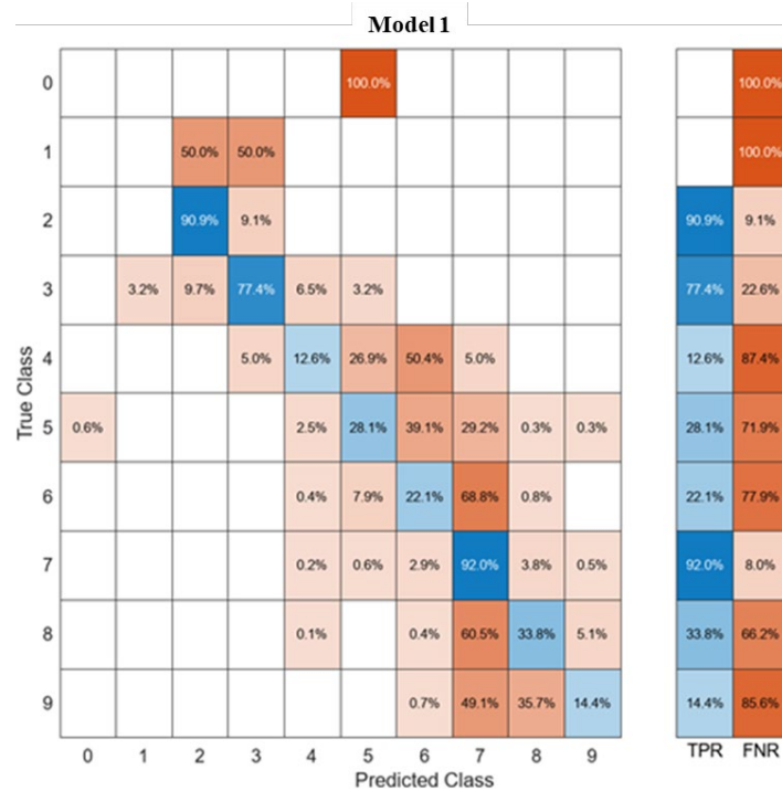
Figure 5.82. Channel Model 1: Ensemble Classifier (57.9%) Performance, True Positive Rates (TPR), False Negative Rates (FNR)
