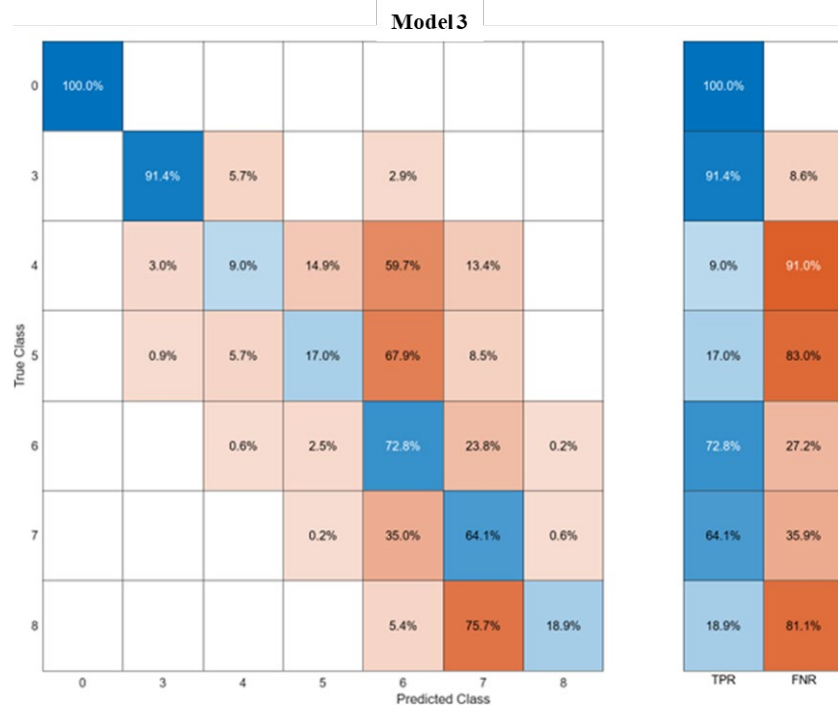
Figure 5.94. Culvert Model 3: Ensemble Classifier (59.7 %) Performance, True Positive Rates (TPR), False Negative Rates (FNR)
