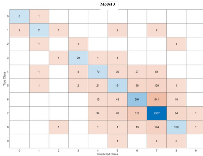
Figure 5.27. Deck Model 3: Ensemble, Bagging Trees Classifier (65.7%) Performance, Number of Observations
