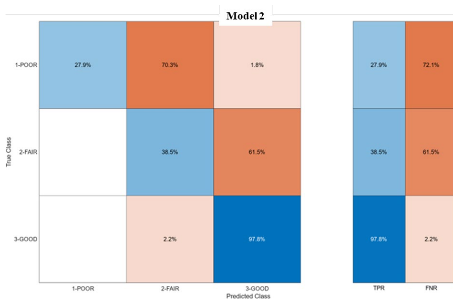
Figure 5.85. Channel Model 2: Decision Tree Classifier (78.2%) Performance, True Positive Rates (TPR), False Negative Rates (FNR).
