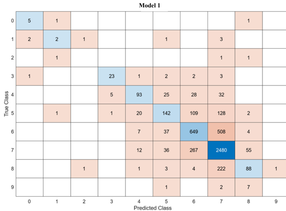
Figure 5.21. Deck Model 1: Ensemble, Bagging Trees Classifier (69.3 %) Performance, Number of Observations.
