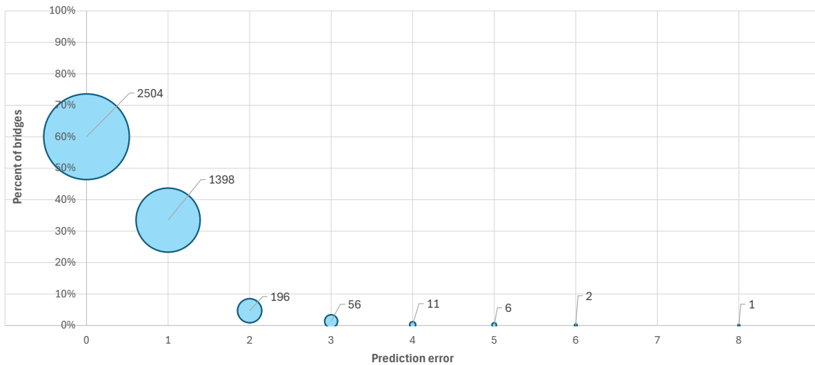
Figure 5.11. Variation in prediction errors for Superstructure NBI Ratings (showing no. of bridges).
