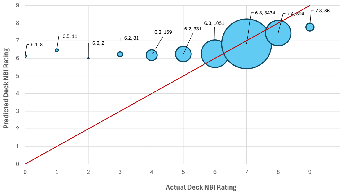
Figure 5.3. Predicted Deck NBI Ratings relative to the actual Ratings (showing no. of bridges).
