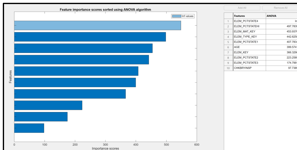
Figure 5.32. ANOVA feature ranking result for Deck Model 4.
