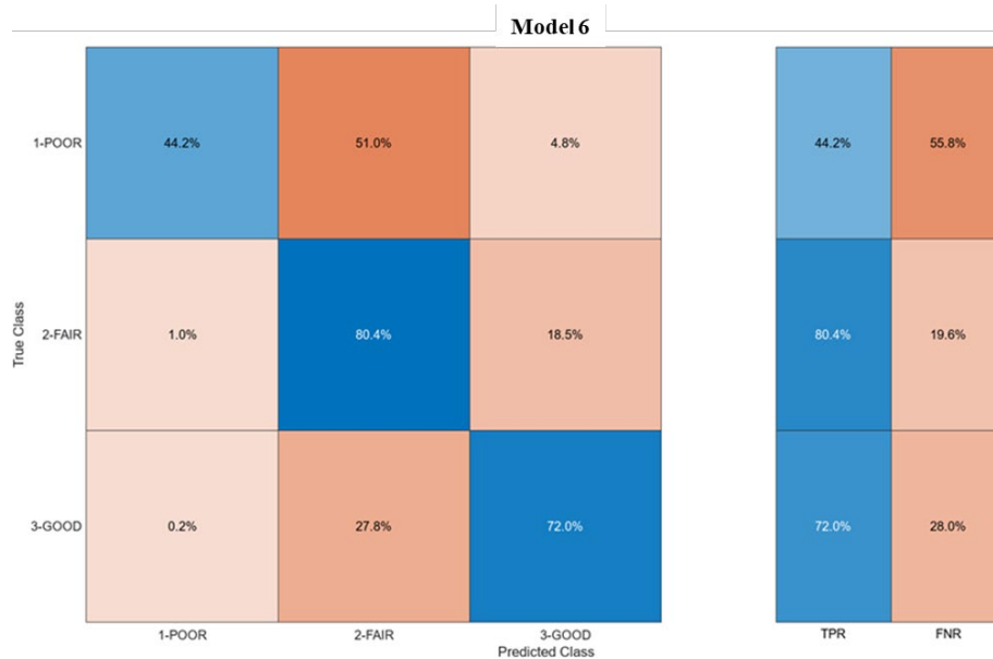
Figure 5.103. Culvert Model 6: Ensemble Classifier (73.7%) Performance, True Positive Rates (TPR), False Negative Rates (FNR).
