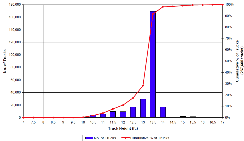
Figure 4.26. Truck height histogram for Interstate Florida roadways (Sobanjo and Thompson 2004).
