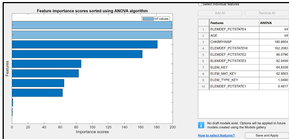
Figure 5.68. ANOVA feature ranking result for Substructure Model 3.
