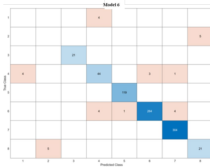
Figure 5.75. Substructure Model 6: Ensemble Classifier (96.1%) Performance, Number of Observations
