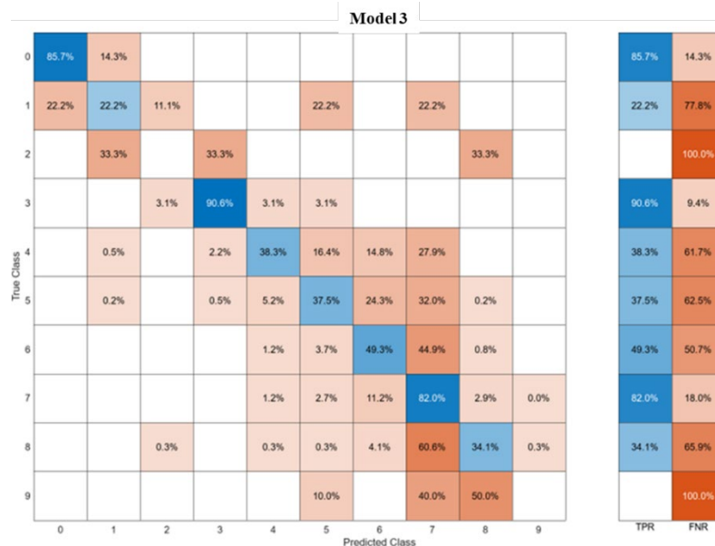
Figure 5.28. Deck Model 3: Ensemble, Bagging Trees Classifier (65.7%) Performance, True Positive Rates (TPR), False Negative Rates (FNR)
