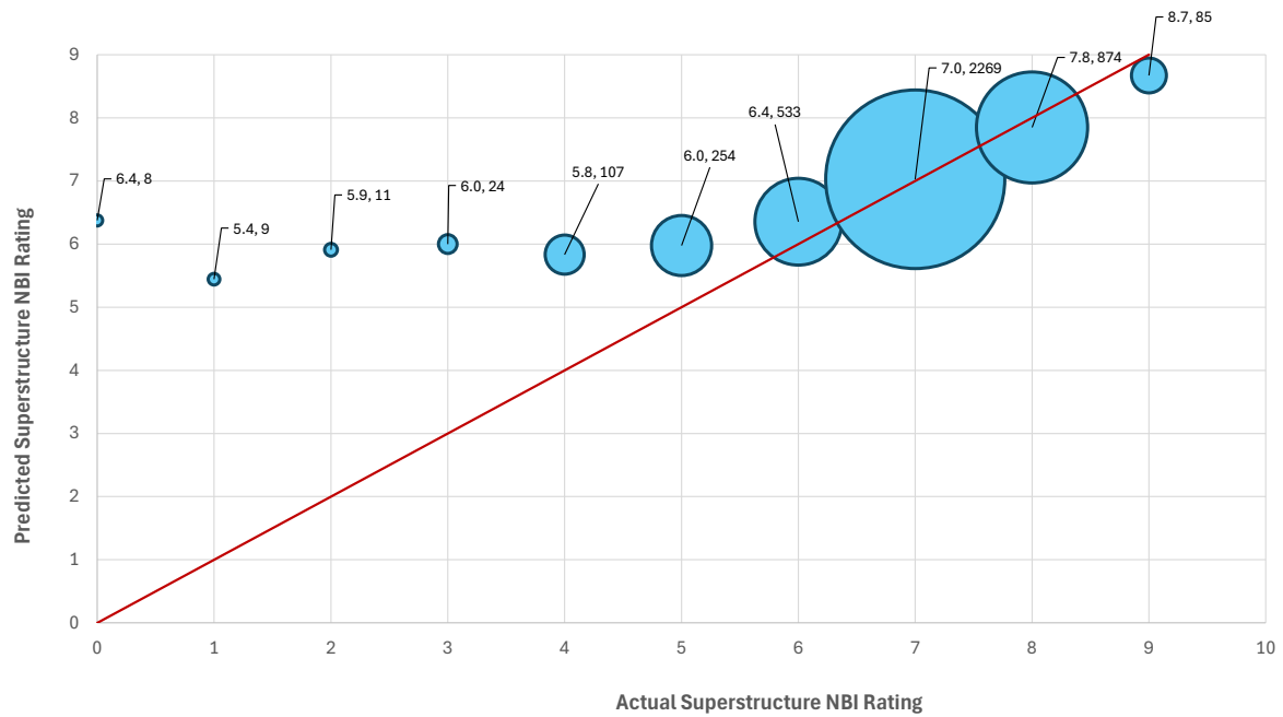
Figure 5.9. Mean predicted Superstructure NBI Ratings relative to the actual Ratings (showing no. of bridges).
