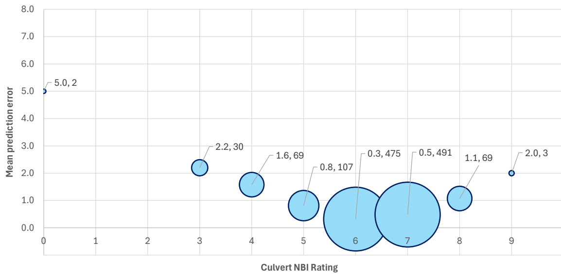
Figure 5.16. Variation in mean prediction errors at each Culvert NBI Rating (showing no. of bridges).
