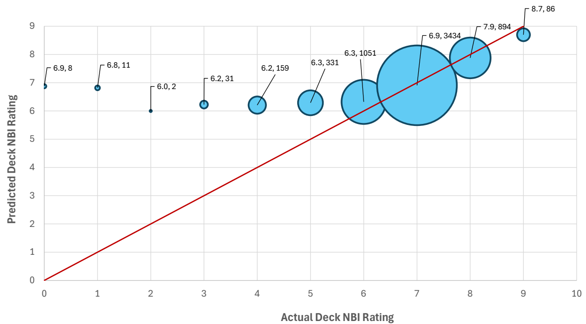
Figure 5.8. . Age-based predicted Deck NBI Ratings relative to the actual Ratings (showing no. of bridges).
