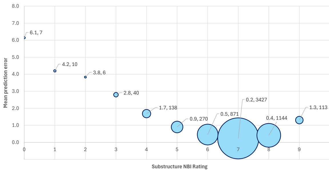
Figure 5.13. Variation in mean prediction errors at each Substructure NBI Rating (showing no. of bridges).
