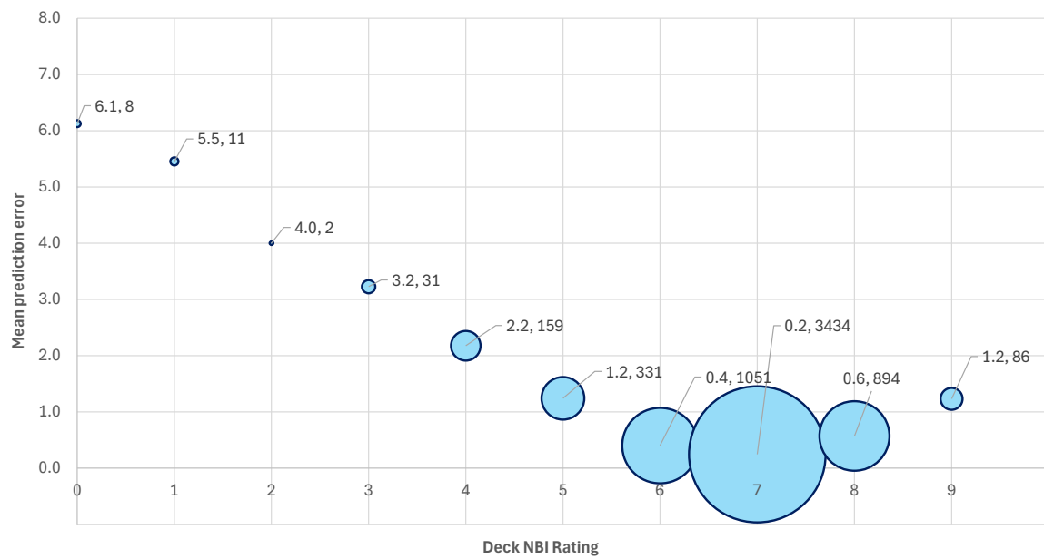
Figure 5.4. Mean prediction errors at each Deck NBI Rating (showing no. of bridges).
