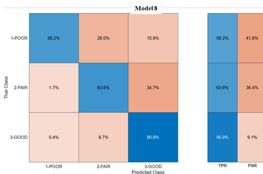
Figure 5.43. Deck Model 8: Ensemble, Bagging Trees Classifier (81.9 %) Performance, True Positive Rates (TPR), False Negative Rates (FNR)
