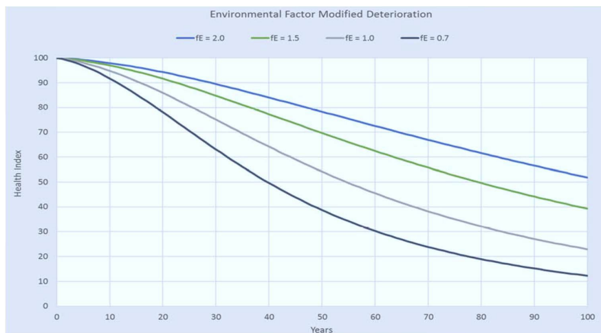
Figure 3.1. Modification of bridge deterioration based on environmental factors (NJDOT 2015).
