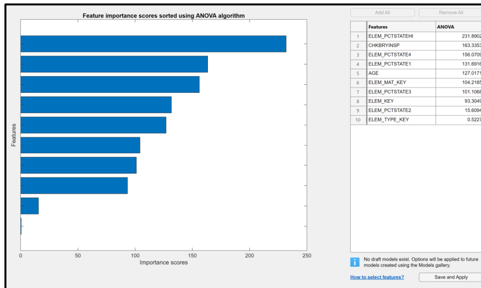
Figure 5.92. ANOVA feature ranking result for Culvert Model 2.
