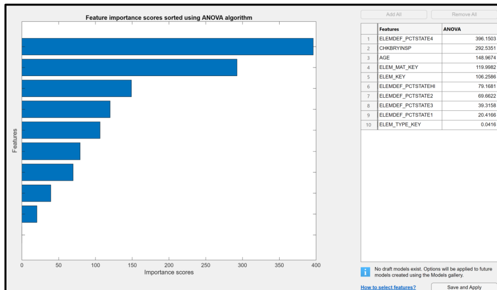
Figure 5.95. ANOVA feature ranking result for Culvert Model 3.
