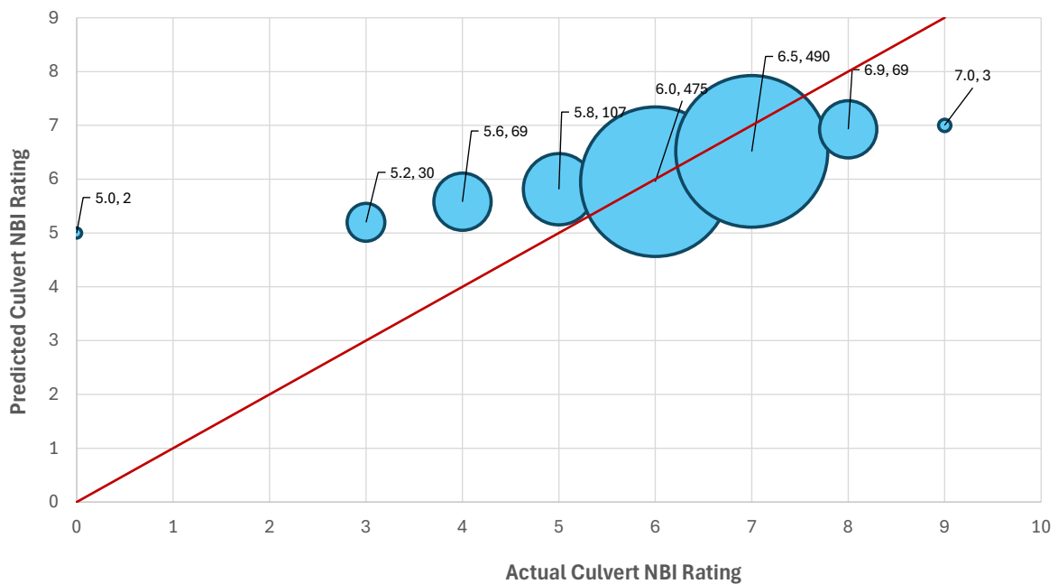
Figure 5.15. Mean predicted Culvert NBI Ratings relative to the actual Ratings (showing no. of bridges).
