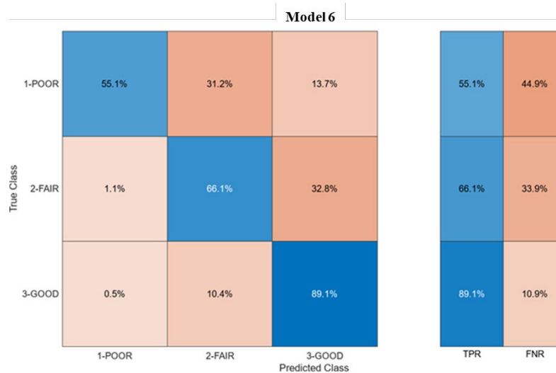
Figure 5.37. Deck Model 6: Ensemble, Bagging Trees Classifier (80.1%) Performance, True Positive Rates (TPR), False Negative Rates (FNR)
