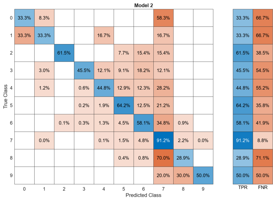
Figure 5.49. Superstructure Model 2: Ensemble Classifier (74%) Performance, True Positive Rates (TPR), False Negative Rates (FNR)
