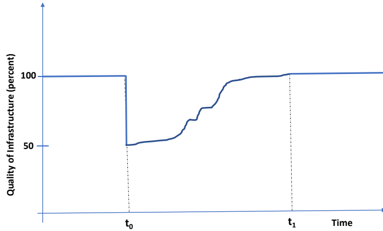
Figure 4.2. Measure of seismic resilience—conceptual definition (Bruneau et al. 2003).
