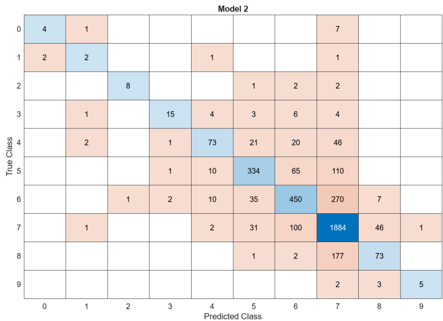
Figure 5.48. Superstructure Model 2: Ensemble Classifier (74%) Performance, Number of Observations
