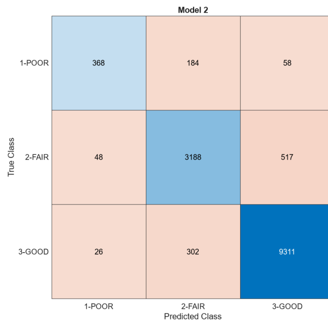
Figure 5.63. Substructure Model 2: Ensemble Classifier (91.9 %) Performance, Number of Observations
