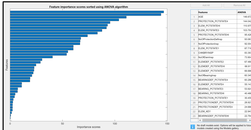
Figure 5.56. ANOVA feature ranking result for Superstructure Model 4.
