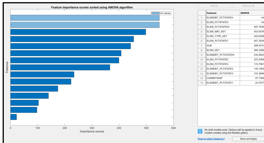
Figure 5.35. ANOVA feature ranking result for Deck Model 5.
