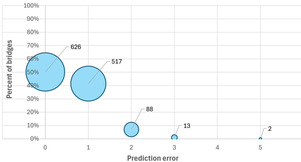
Figure 5.17. Variation in prediction errors for Culvert NBI Ratings (showing no. of bridges).
