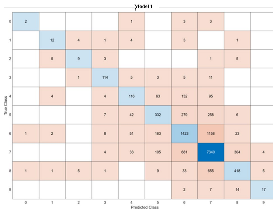
Figure 5.60. Substructure Model 1: Ensemble Classifier (69.9 %) Performance, Number of Observations
