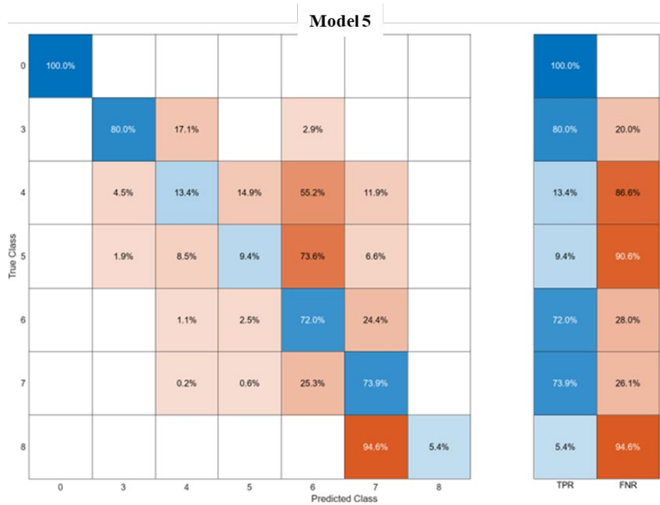
Figure 5.100. Culvert Model 5: Ensemble Classifier (62 %) Performance, True Positive Rates (TPR), False Negative Rates (FNR).
