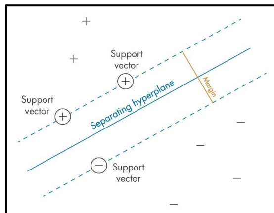
Figure 5.2. Demonstration of the SVM algorithm: defining the “margin” between classes.
