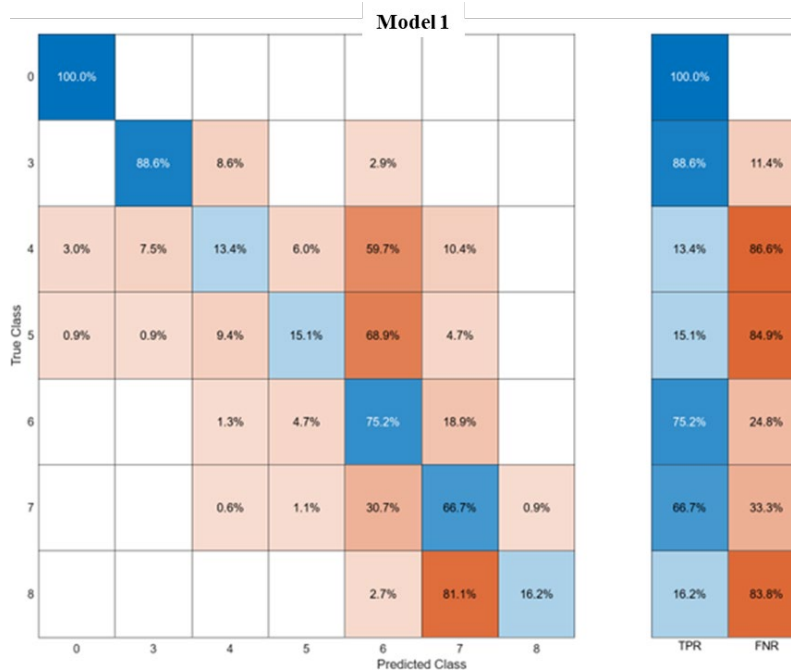
Figure 5.88. Culvert Model 1: Neural Network Classifier (61.6%) Performance, True Positive Rates (TPR), False Negative Rates (FNR)
