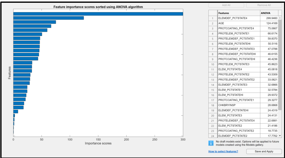
Figure 5.77. ANOVA feature ranking result for Substructure Model 6.
