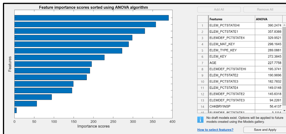
Figure 5.38. ANOVA feature ranking result for Deck Model 6.
