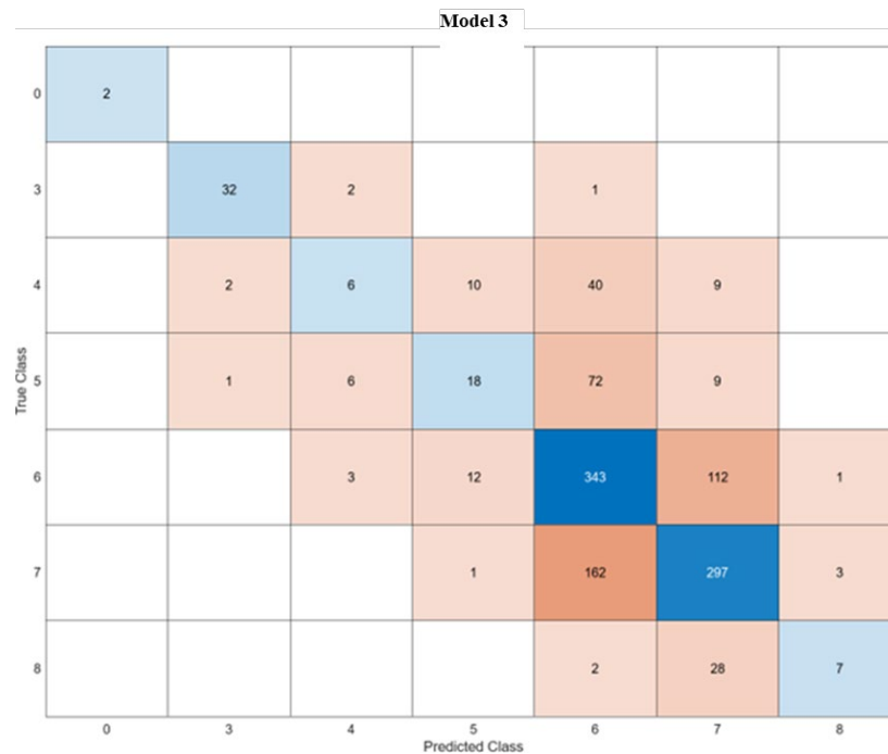
Figure 5.93. Culvert Model 3: Ensemble Classifier (59.7 %) Performance, Number of Observations.
