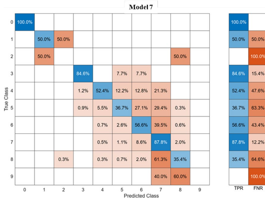
Figure 5.40. Deck Model 7: Ensemble, Bagging Trees Classifier (71.8 %) Performance, True Positive Rates (TPR), False Negative Rates (FNR)
