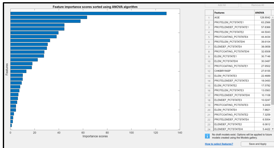
Figure 5.80. ANOVA feature ranking result for Substructure Model 7.
