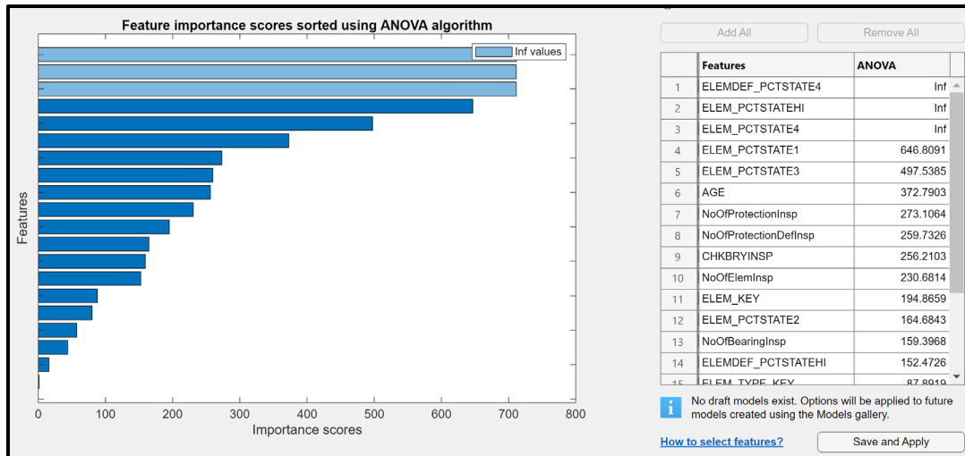
Figure 5.59. ANOVA feature ranking result for Superstructure Model 5.
