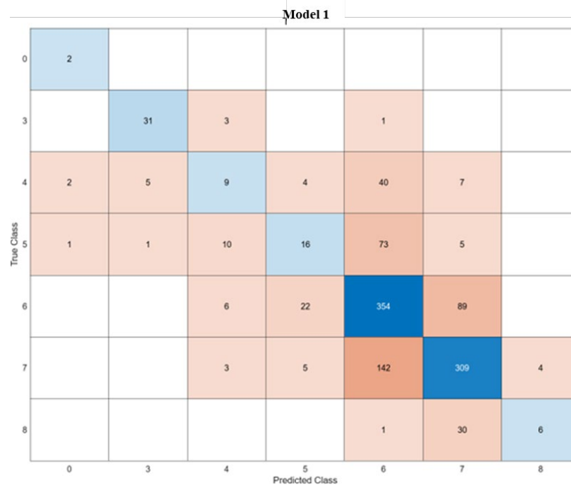
Figure 5.87. Culvert Model 1: Neural Network Classifier (61.6%) Performance, Number of Observations
