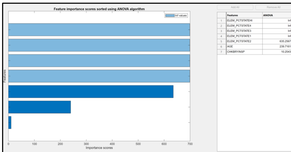
Figure 5.83. ANOVA feature ranking result for Channel Model 1.
