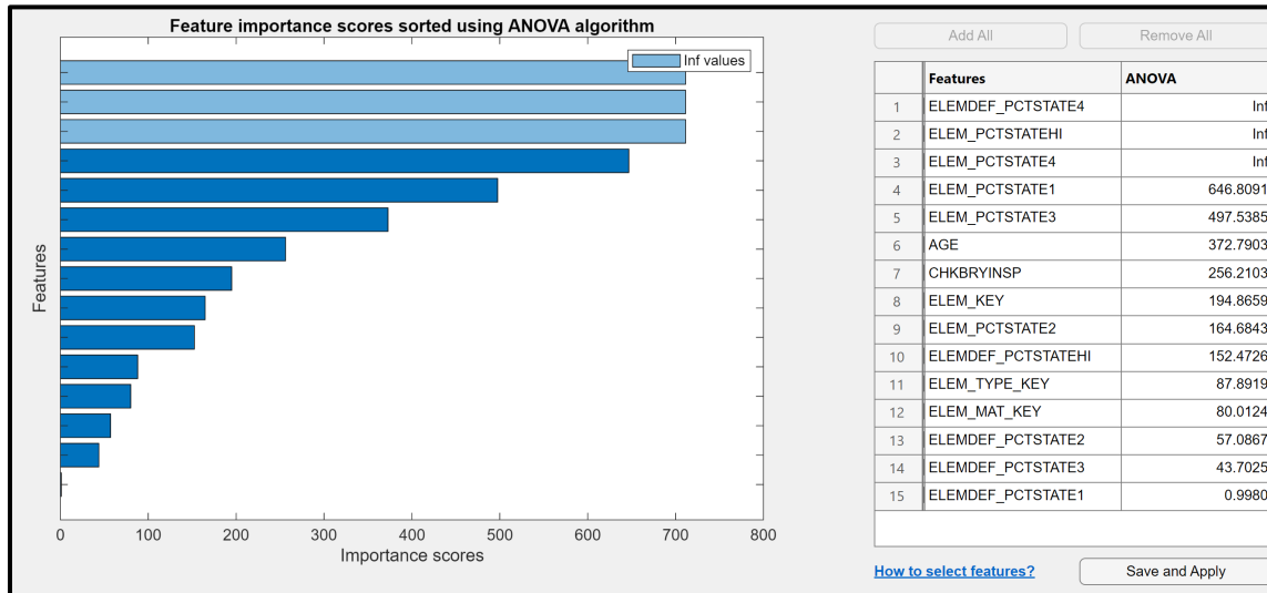
Figure 5.47. ANOVA feature ranking result for Superstructure Model 1.
