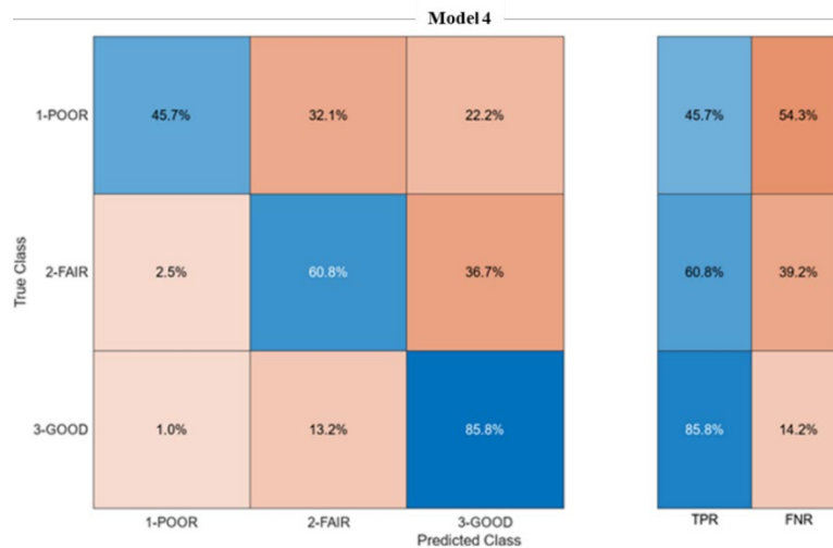
Figure 5.31. Deck Model 4: Ensemble, Bagging Trees Classifier (75.9%) Performance, True Positive Rates (TPR), False Negative Rates (FNR)
