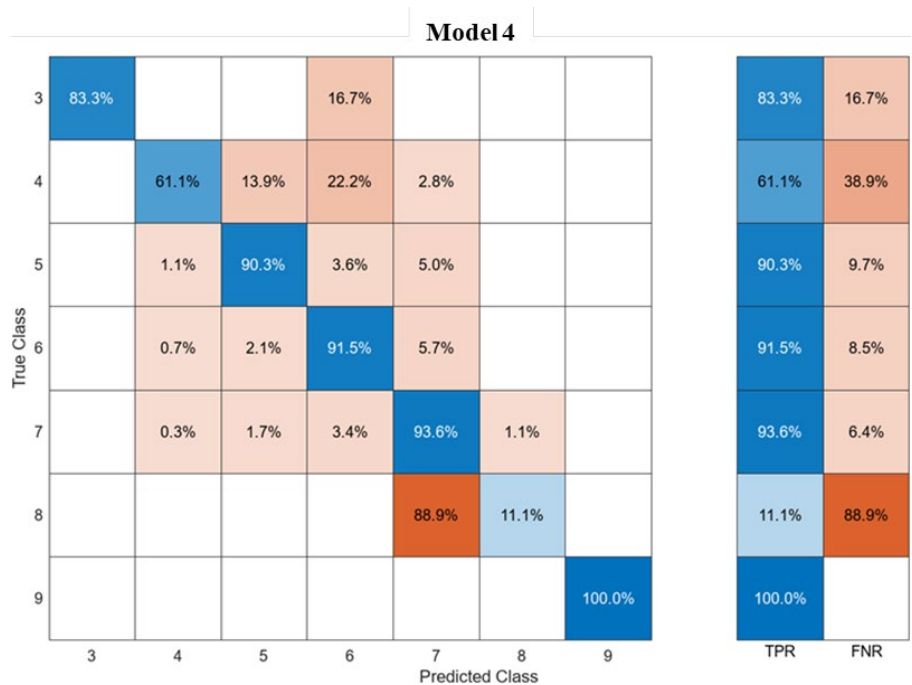
Figure 5.55. Superstructure Model 4: Ensemble Classifier (89.2%) Performance, True Positive Rates (TPR), False Negative Rates (FNR)
