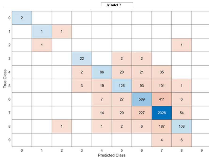
Figure 5.39. Deck Model 7: Ensemble, Bagging Trees Classifier (71.8 %) Performance, Number of Observations
