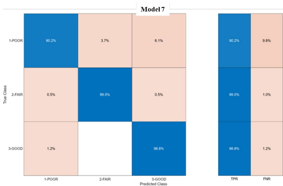
Figure 5.79. Substructure Model 7: Ensemble Classifier (98 %) Performance, True Positive Rates (TPR), False Negative Rates (FNR)
