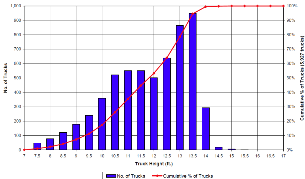
Figure 4.27. Truck height histogram for Non-Interstate Florida roadways (Sobanjo and Thompson 2004).
