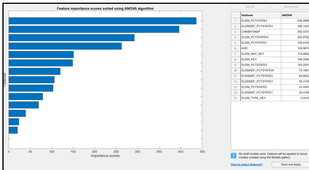
Figure 5.101. ANOVA feature ranking result for Culvert Model 5.
