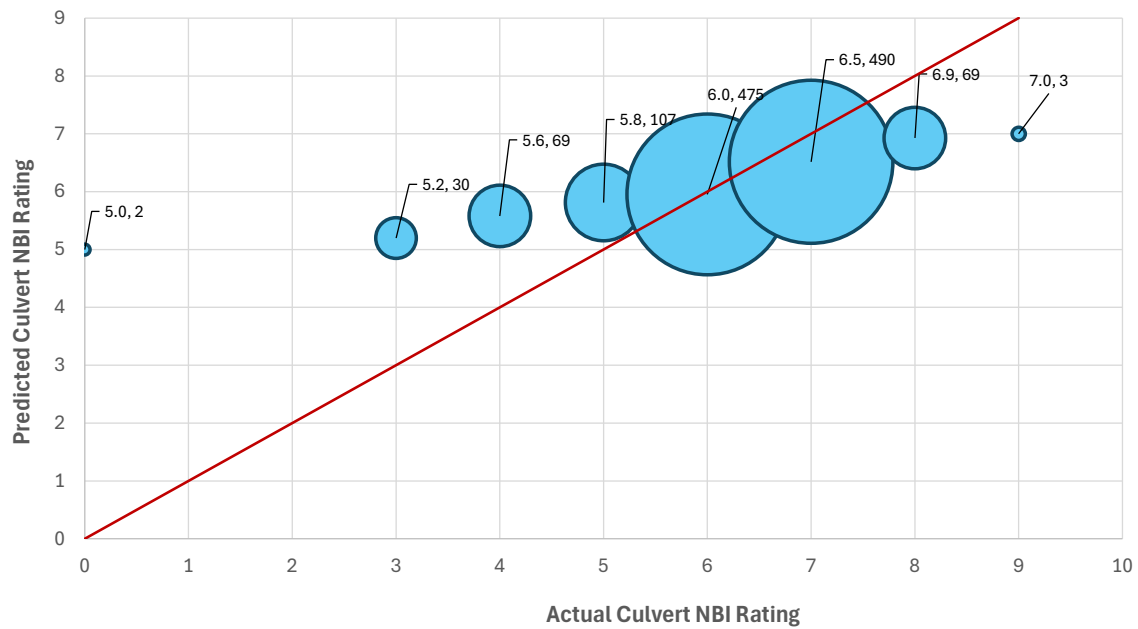
Figure B12. Means of predicted Culvert NBI rating and number of bridges at each actual rating.
