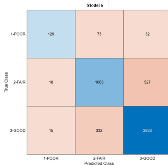
Figure 5.36. Deck Model 6: Ensemble, Bagging Trees Classifier (80.1%) Performance, Number of Observations
