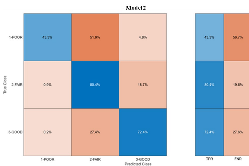
Figure 5.91. Culvert Model 2: Efficient Logistic Regression Classifier (73.8%) Performance, True Positive Rates (TPR), False Negative Rates (FNR).
