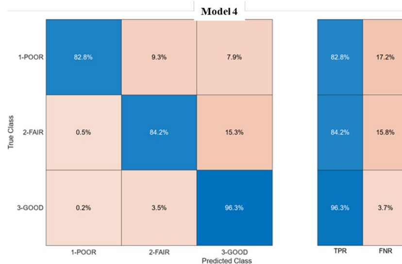
Figure 5.70. Substructure Model 4: Ensemble Classifier (92.5 %) Performance, True Positive Rates (TPR), False Negative Rates (FNR)
