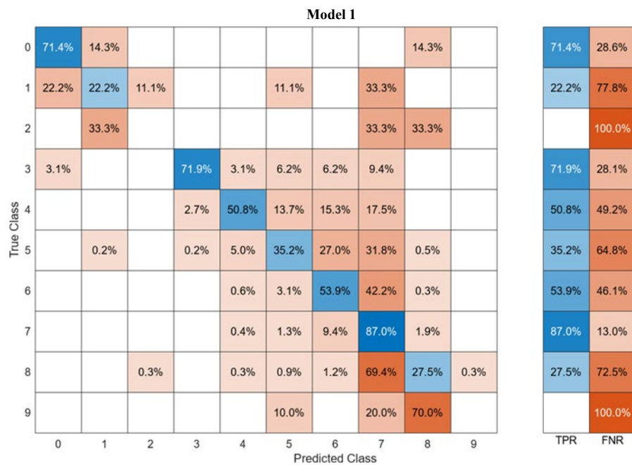
Figure 5.22. Deck Model 1: Ensemble, Bagging Trees Classifier (69.3%) Performance, True Positive Rates (TPR), False Negative Rates (FNR).
