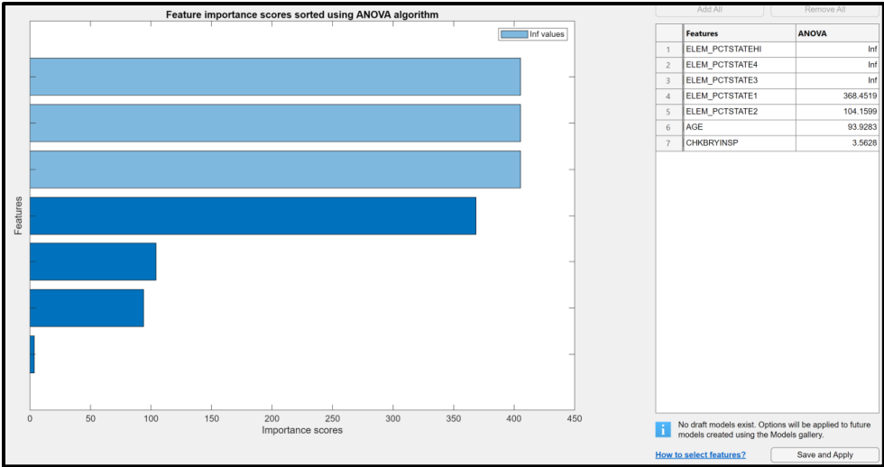
Figure 5.86. ANOVA feature ranking result for Channel Model 2.
