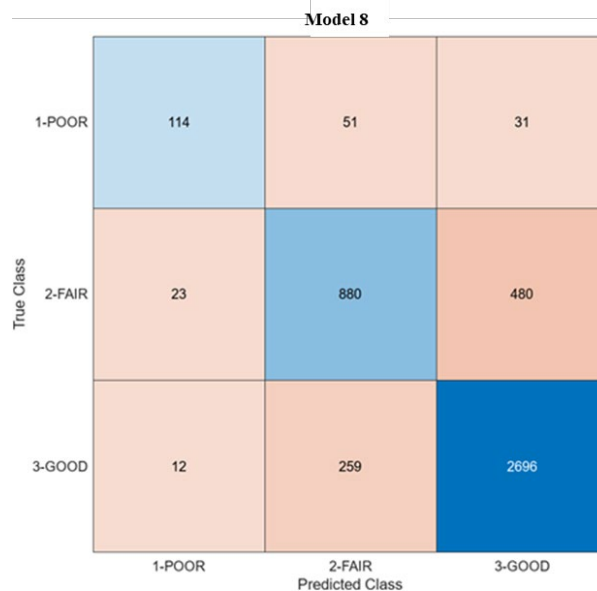
Figure 5.42. Deck Model 8: Ensemble, Bagging Trees Classifier (81.9 %) Performance, Number of Observations
