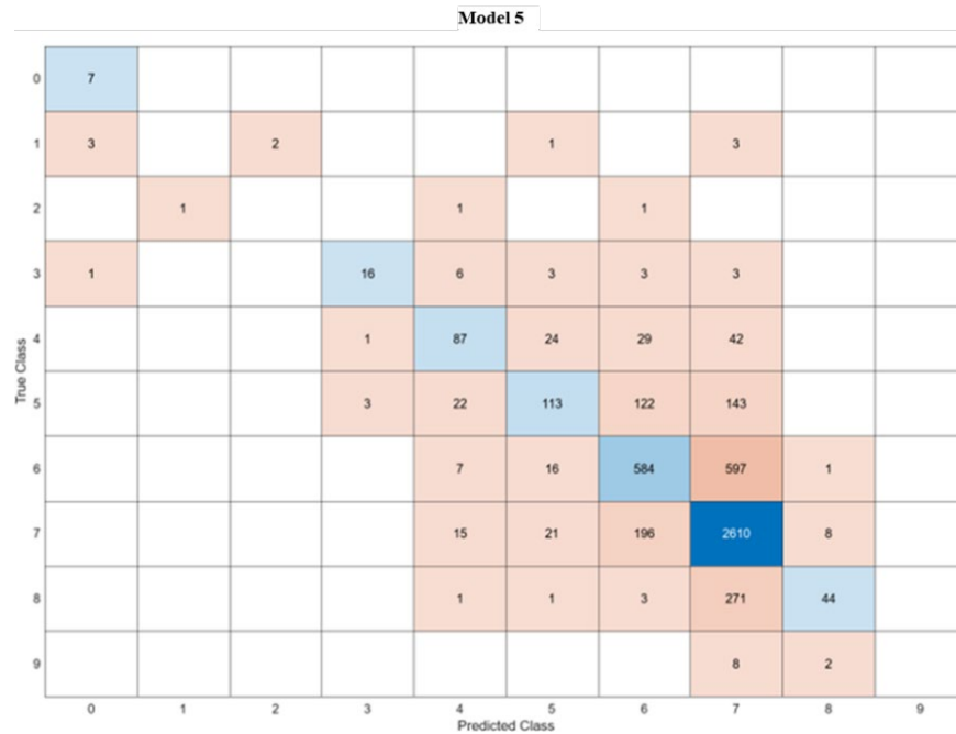
Figure 5.33. Deck Model 5: Ensemble, Bagging Trees Classifier (68.9%) Performance, Number of Observations
