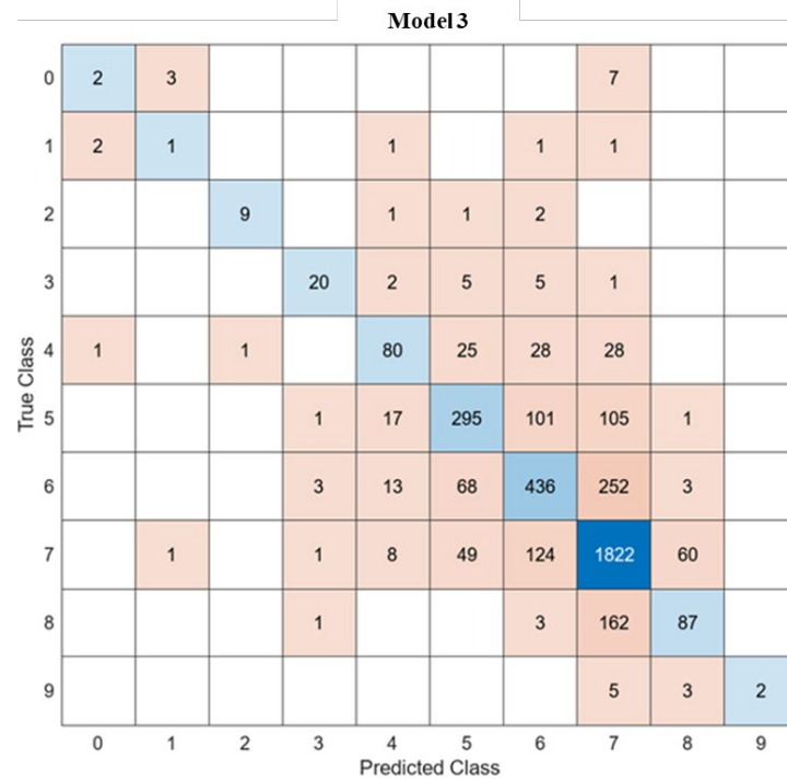
Figure 5.51. Superstructure Model 3: Ensemble Classifier (71.5%) Performance, Number of Observations
