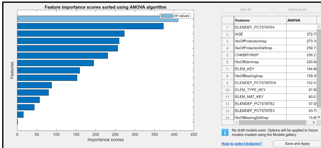
Figure 5.50. ANOVA feature ranking result for Superstructure Model 2.
