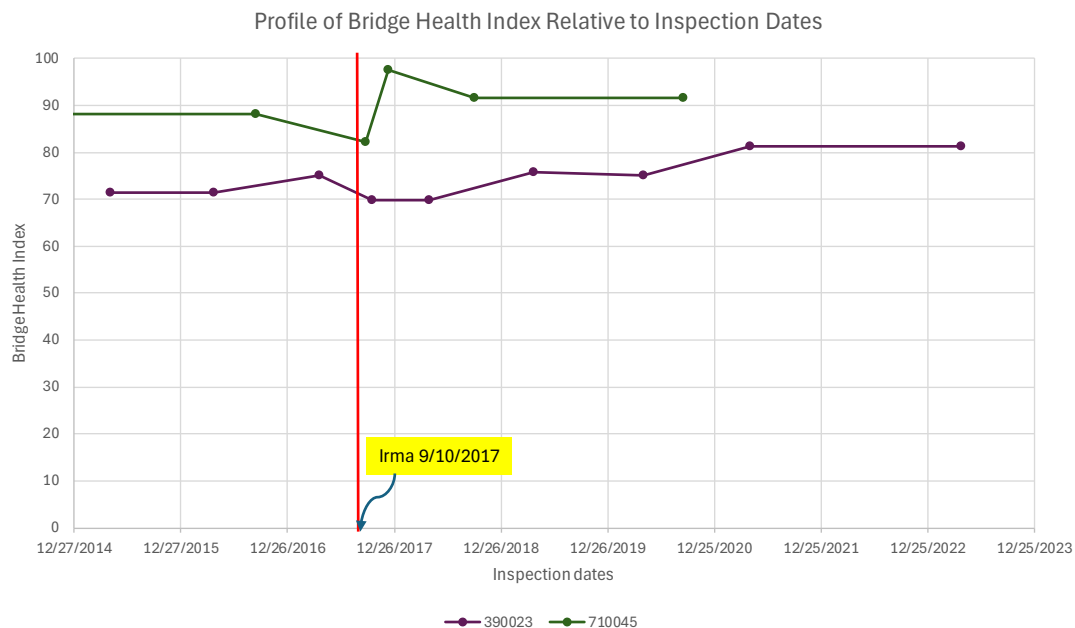
Figure 4.5. Bridge Health Index's variation with time.
