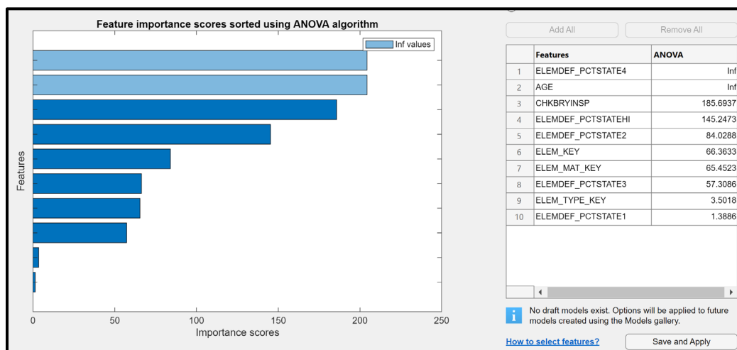
Figure 5.71. ANOVA feature ranking result for Substructure Model 4.
