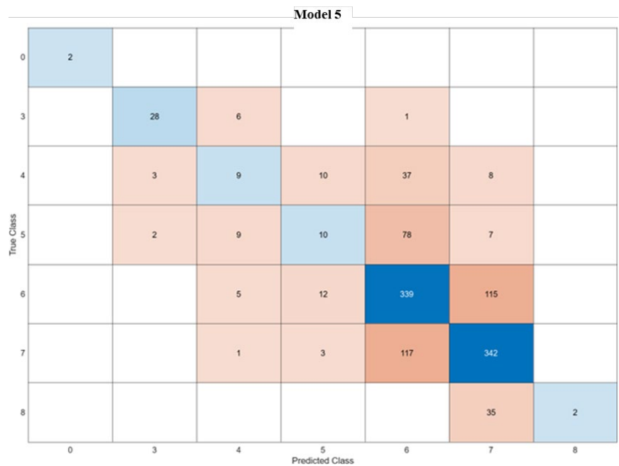
Figure 5.99. Culvert Model 5: Ensemble Classifier (62 %) Performance, Number of Observations.
