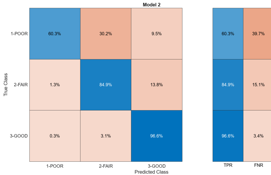
Figure 5.64. Substructure Model 2: Ensemble Classifier (91.9%) Performance, True Positive Rates (TPR), False Negative Rates (FNR)
