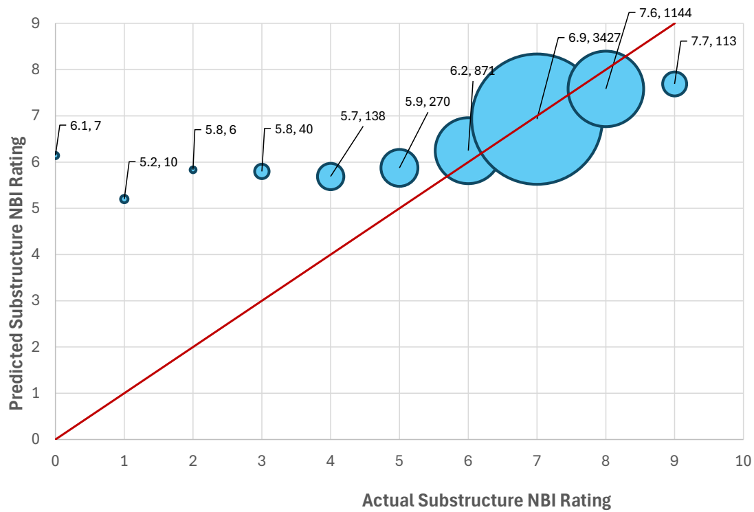
Figure B10. Means of predicted Substructure NBI rating and number of bridges at each actual rating.
