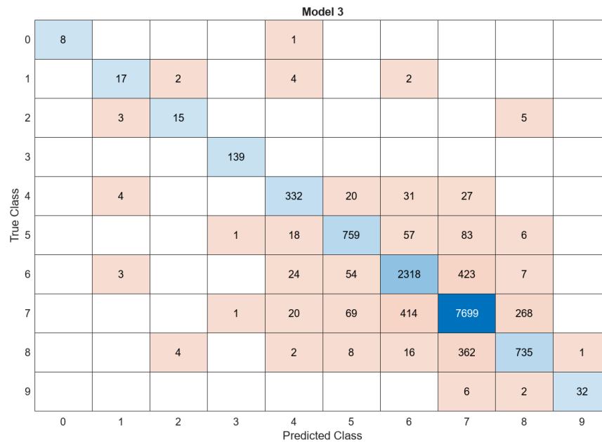
Figure 5.66. Substructure Model 3: Ensemble Classifier (86.1 %) Performance, Number of Observations
