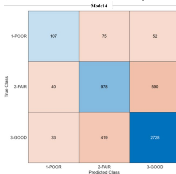
Figure 5.30. Deck Model 4: Ensemble, Bagging Trees Classifier (75.9%) Performance, Number of Observations
