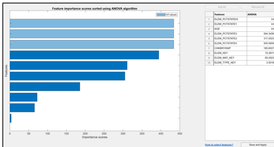
Figure 5.65. ANOVA feature ranking result for Substructure Model 2.
