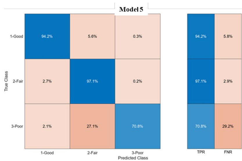
Figure 5.58. Superstructure Model 5: Ensemble, Bagging Trees Classifier (94.7 %) Performance, True Positive Rates (TPR), False Negative Rates (FNR)
