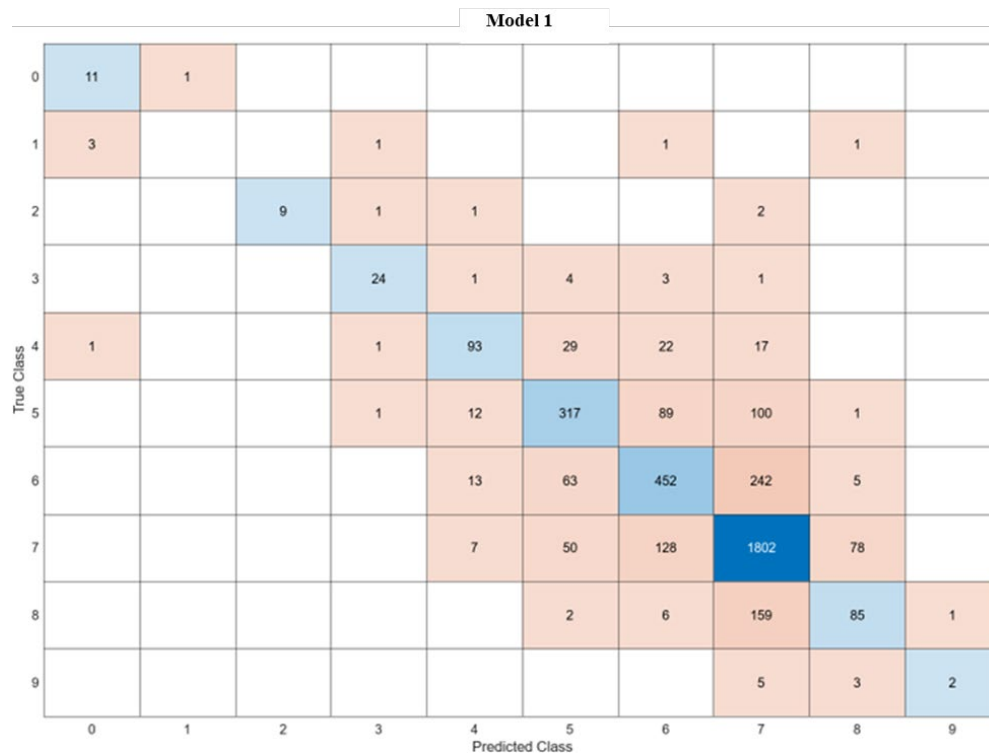
Figure 5.45. Superstructure Model 1: Ensemble Classifier (72.6%) Performance, Number of Observations
