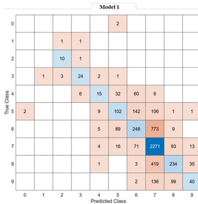
Figure 5.81. Channel Model 1: Ensemble Classifier (57.9%) Performance, Number of Observations
