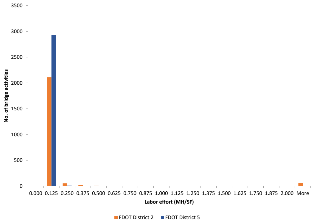
Figure 6.2. Labor effort per bridge deck area in Districts 2 & 5 for substructure maintenance and repair.
