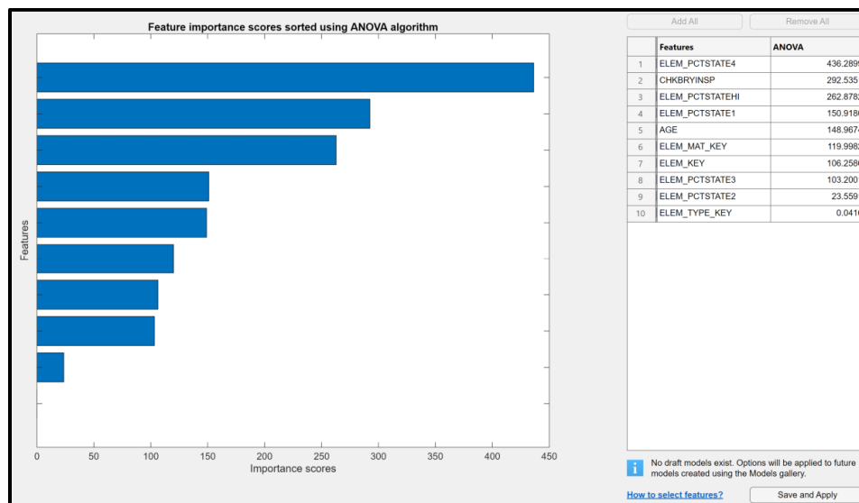
Figure 5.89. ANOVA feature ranking result for Culvert Model 1.
