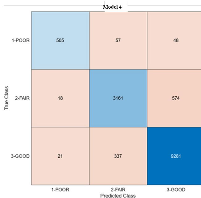
Figure 5.69. Substructure Model 4: Ensemble Classifier (92.5 %) Performance, Number of Observations
