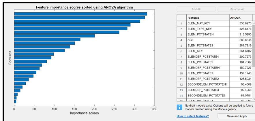
Figure 5.44. ANOVA feature ranking result for Deck Model 8.
