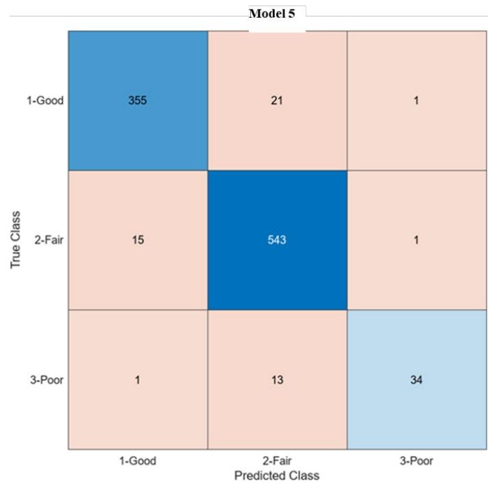
Figure 5.57. Superstructure Model 5: Ensemble, Bagging Trees Classifier (94.7 %) Performance, Number of Observations
