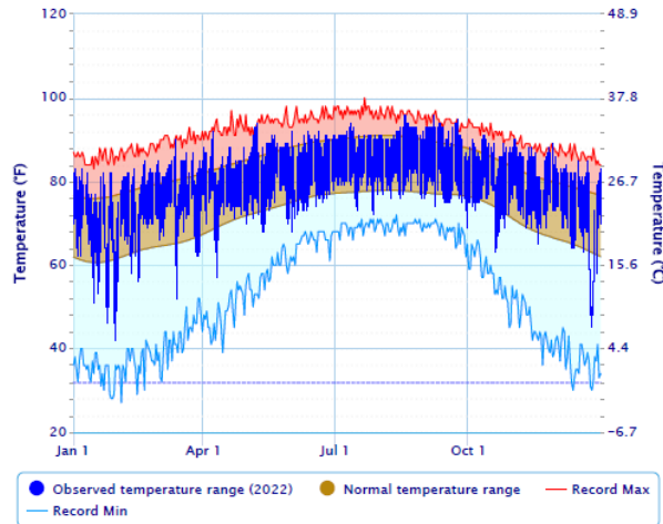
Figure 3.9. Variation in observed temperatures in Florida in 2022 (NOAA 2023).
