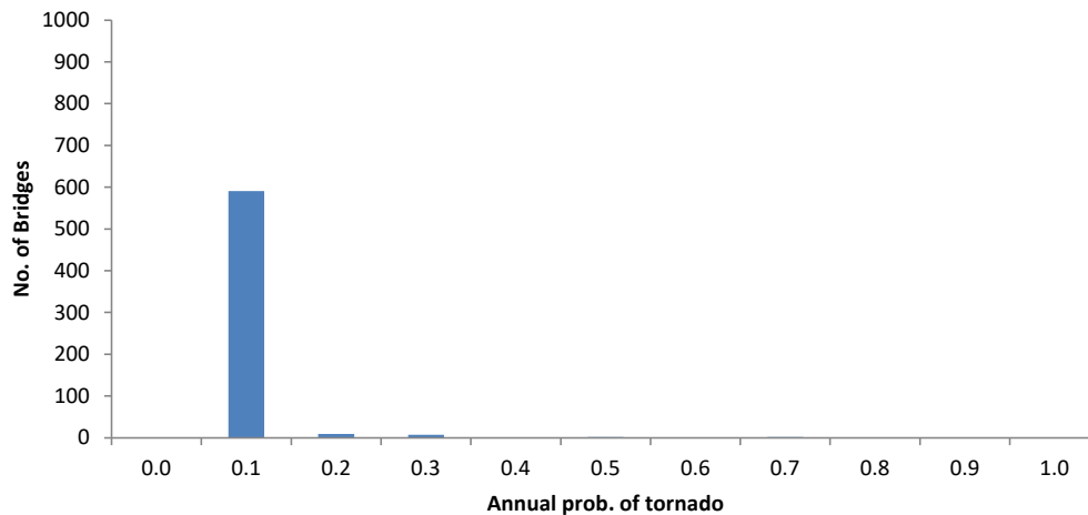
Figure 4.20. Estimated annual frequency of tornado occurrence on Florida state-maintained bridges.
