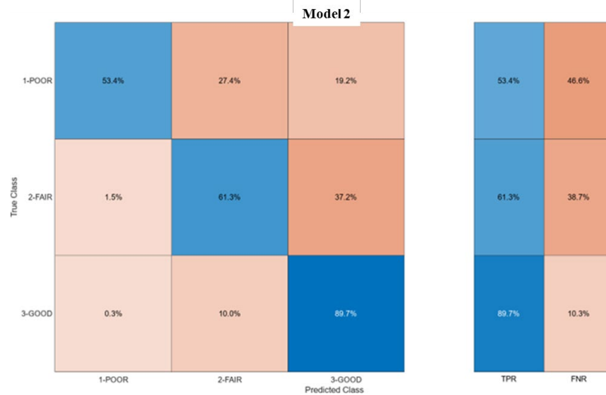
Figure 5.25. Deck Model 2: Ensemble, Bagging Trees Classifier (78.9%) Performance, True Positive Rates (TPR), False Negative Rates (FNR)
