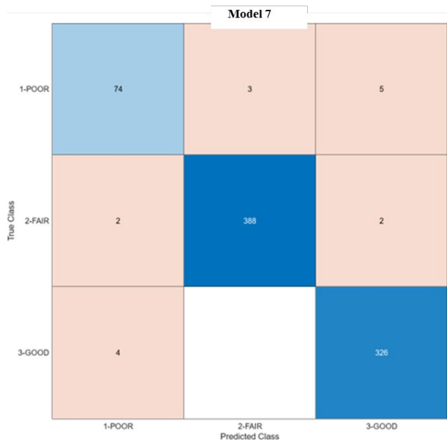
Figure 5.78. Substructure Model 7: Ensemble Classifier (98%) Performance, Number of Observations
