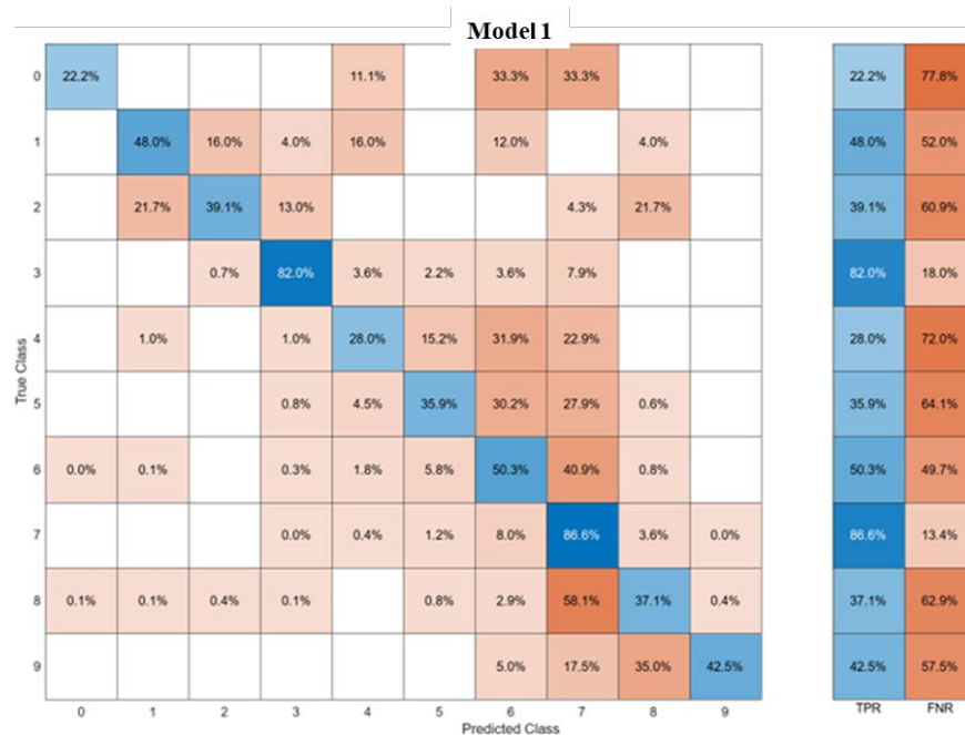
Figure 5.61. Substructure Model 1: Ensemble Classifier (69.9%) Performance, True Positive Rates (TPR), False Negative Rates (FNR)
