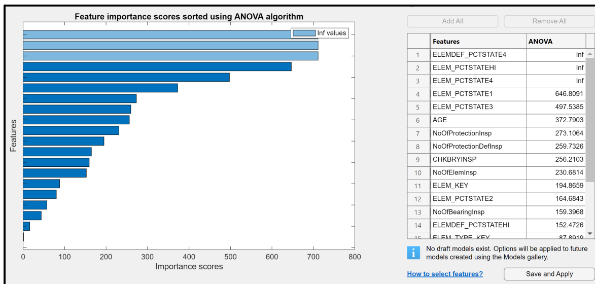
Figure 5.53. ANOVA feature ranking result for Superstructure Model 2.
