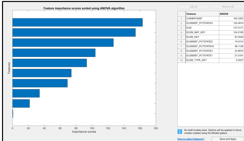
Figure 5.98. ANOVA feature ranking result for Culvert Model 4.
