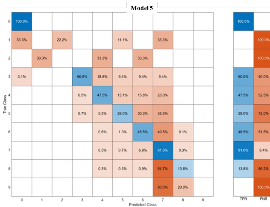
Figure 5.34. Deck Model 5: Ensemble, Bagging Trees Classifier (68.9%) Performance, True Positive Rates (TPR), False Negative Rates (FNR)
