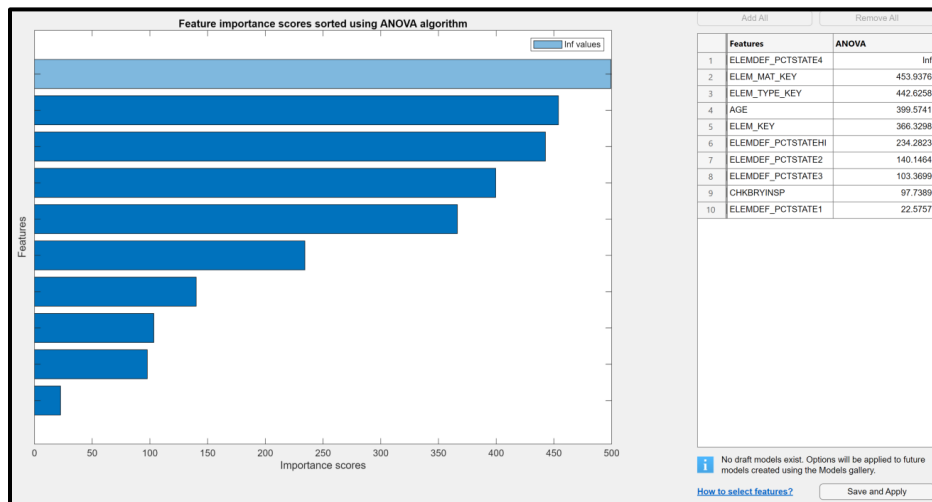
Figure 5.29. ANOVA feature ranking result for Deck Model 3.
