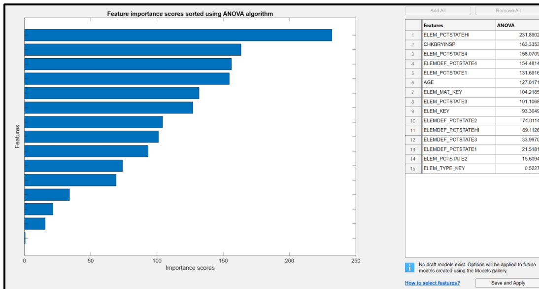
Figure 5.104. ANOVA feature ranking result for Culvert Model 6.
