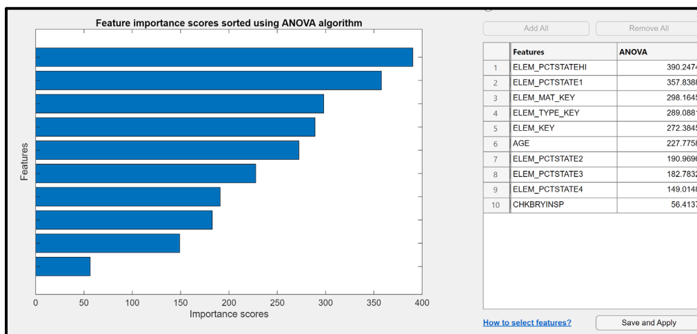
Figure 5.26. ANOVA feature ranking result for Deck Model 2.
