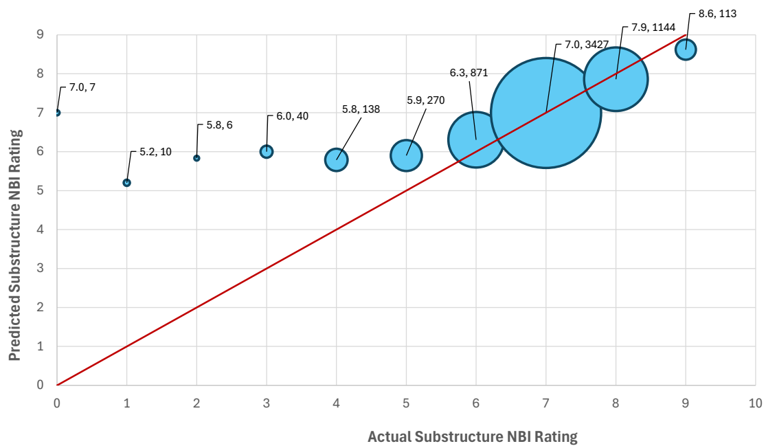
Figure B11. Means of age-based predicted Substructure NBI rating and number of bridges at each actual rating.
