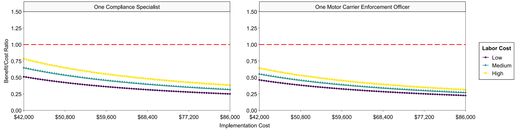
Figure 6.63: Benefit-Cost Results for Drive-Over Tire Measurement System at Cascade Locks POE (Evening Shift)
