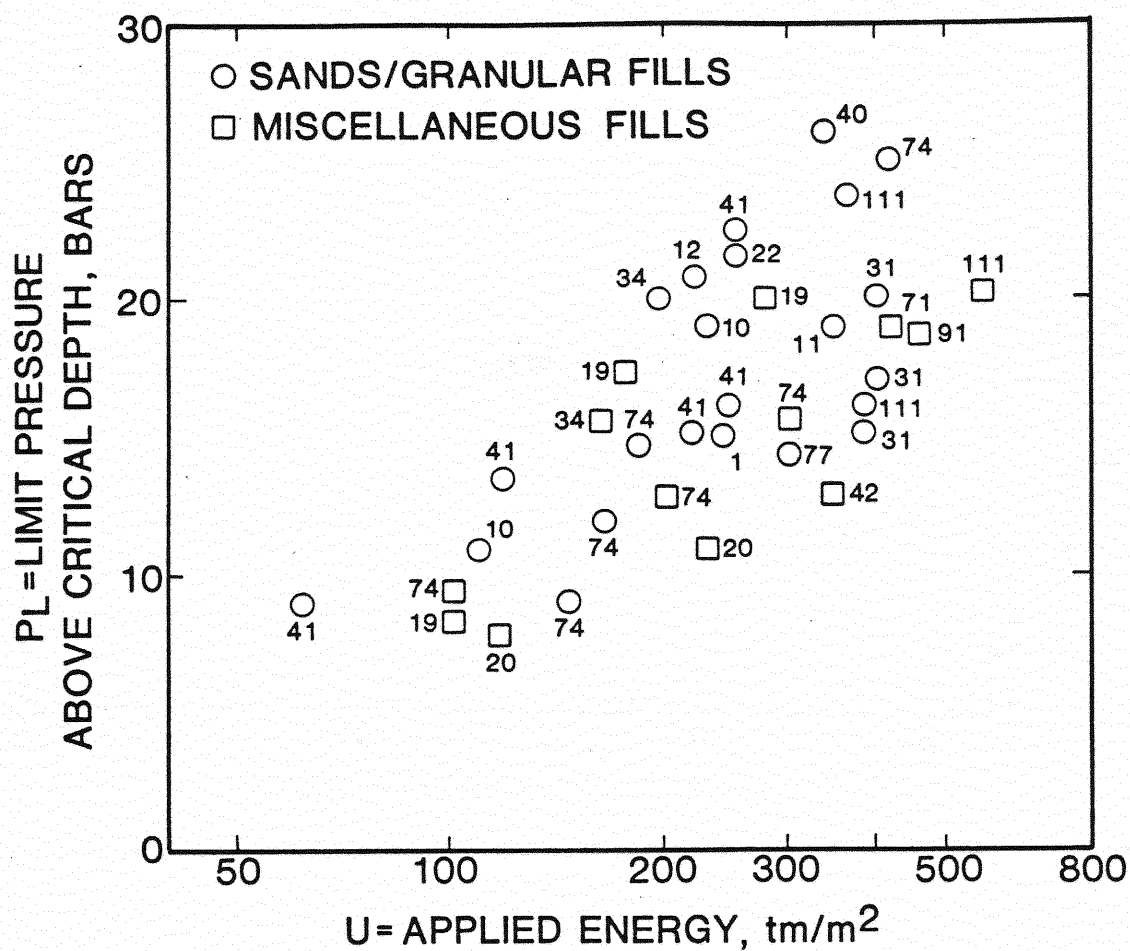
Figure 13. Observed Trend Between Limit Pressure and Applied Energy Level for Granular Soils (8)
