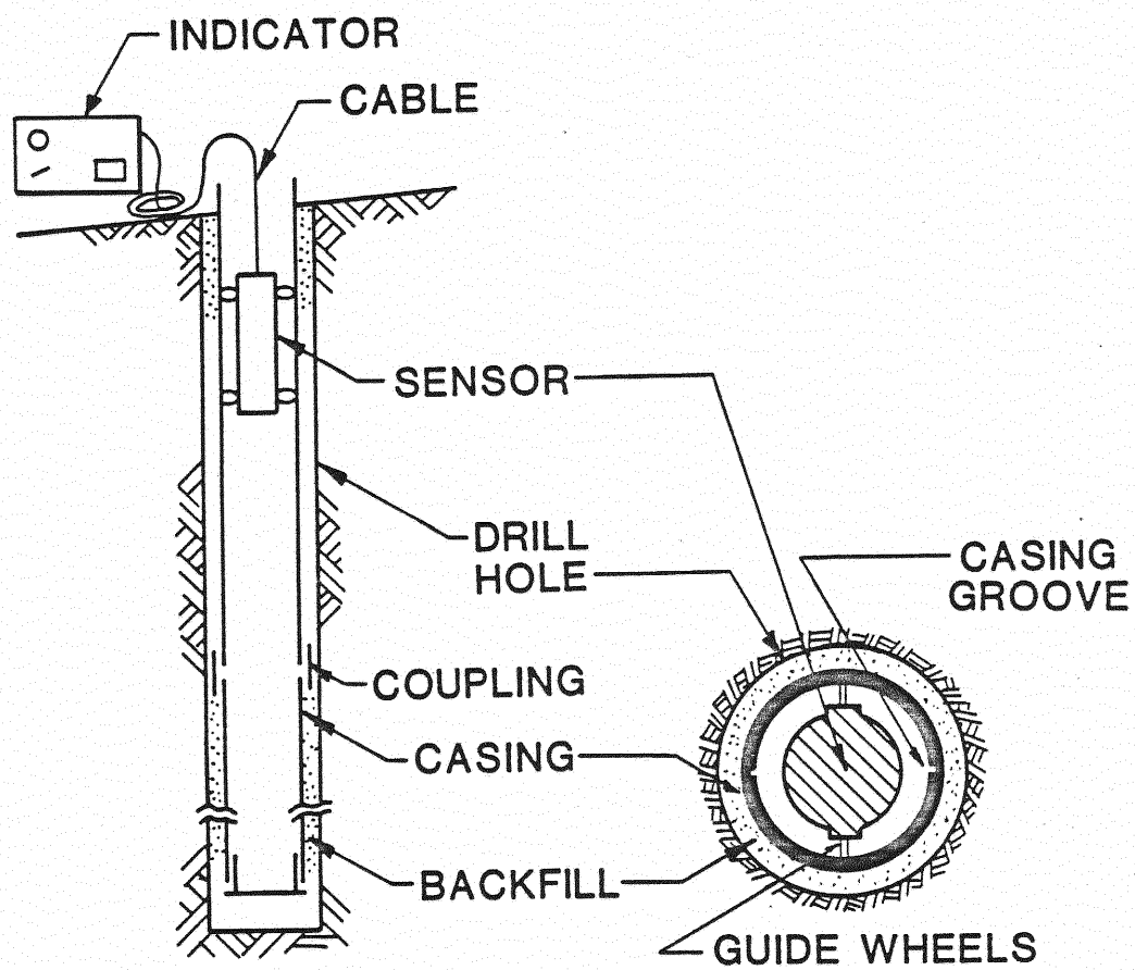
Figure 20. Inclinator Set-Up
