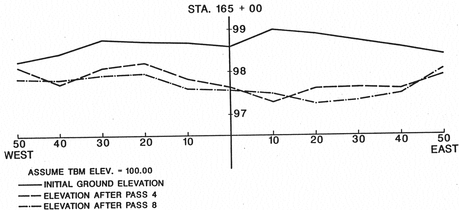
Figure 106. Post-Compaction Subsidence, Along CRL, Test Section No. 3
