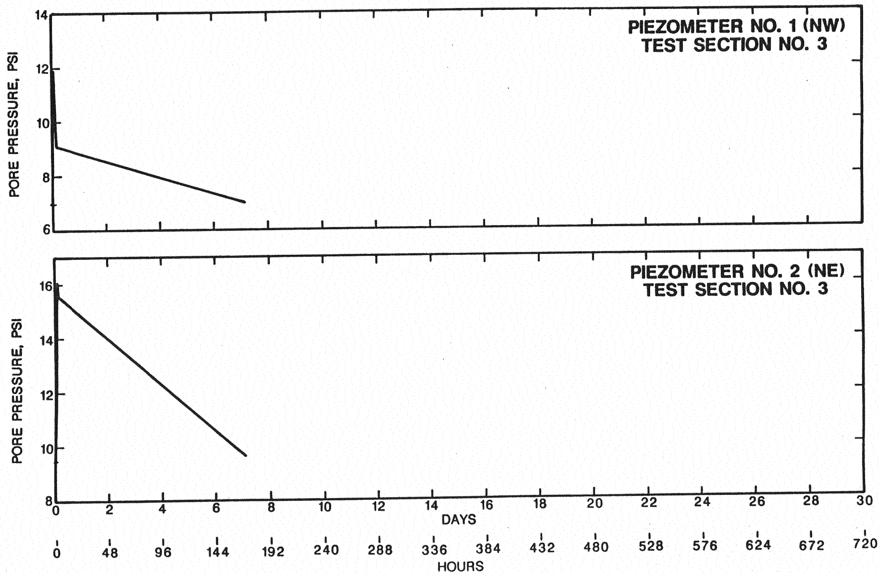
Figure 91. Long-Term Pore Pressure Dissipation (Piezometers 1 and 2), Test Section No. 3
