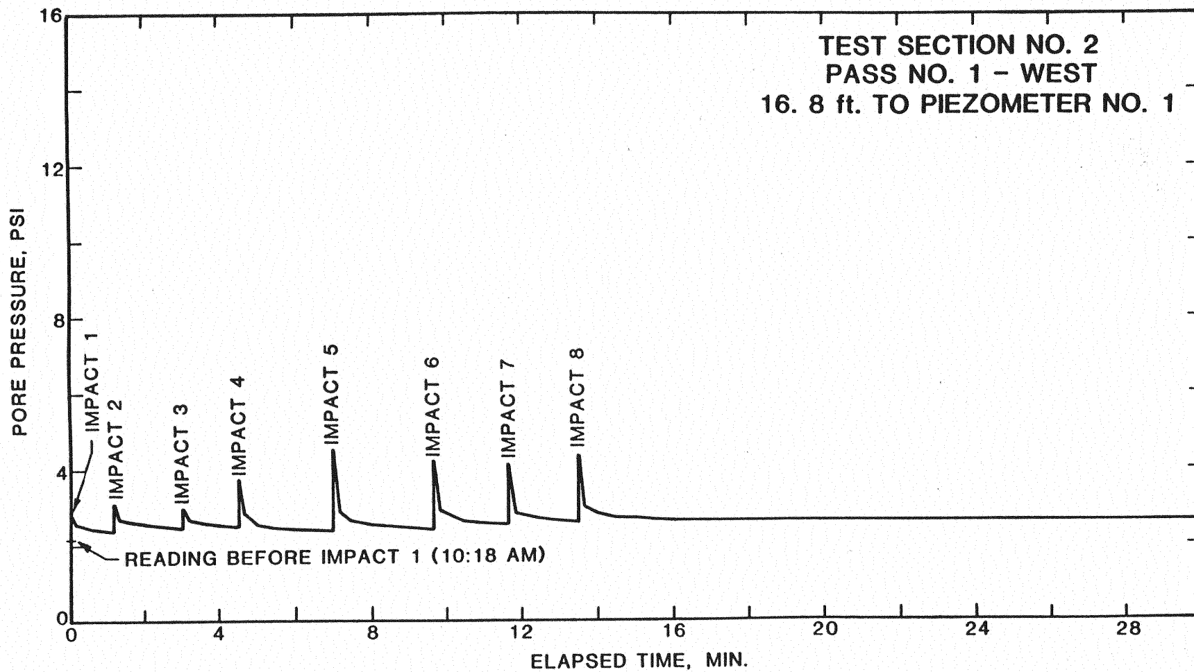
Figure 41. Piezometer Data, Pass No. 1 - West, Test Section No. 2
