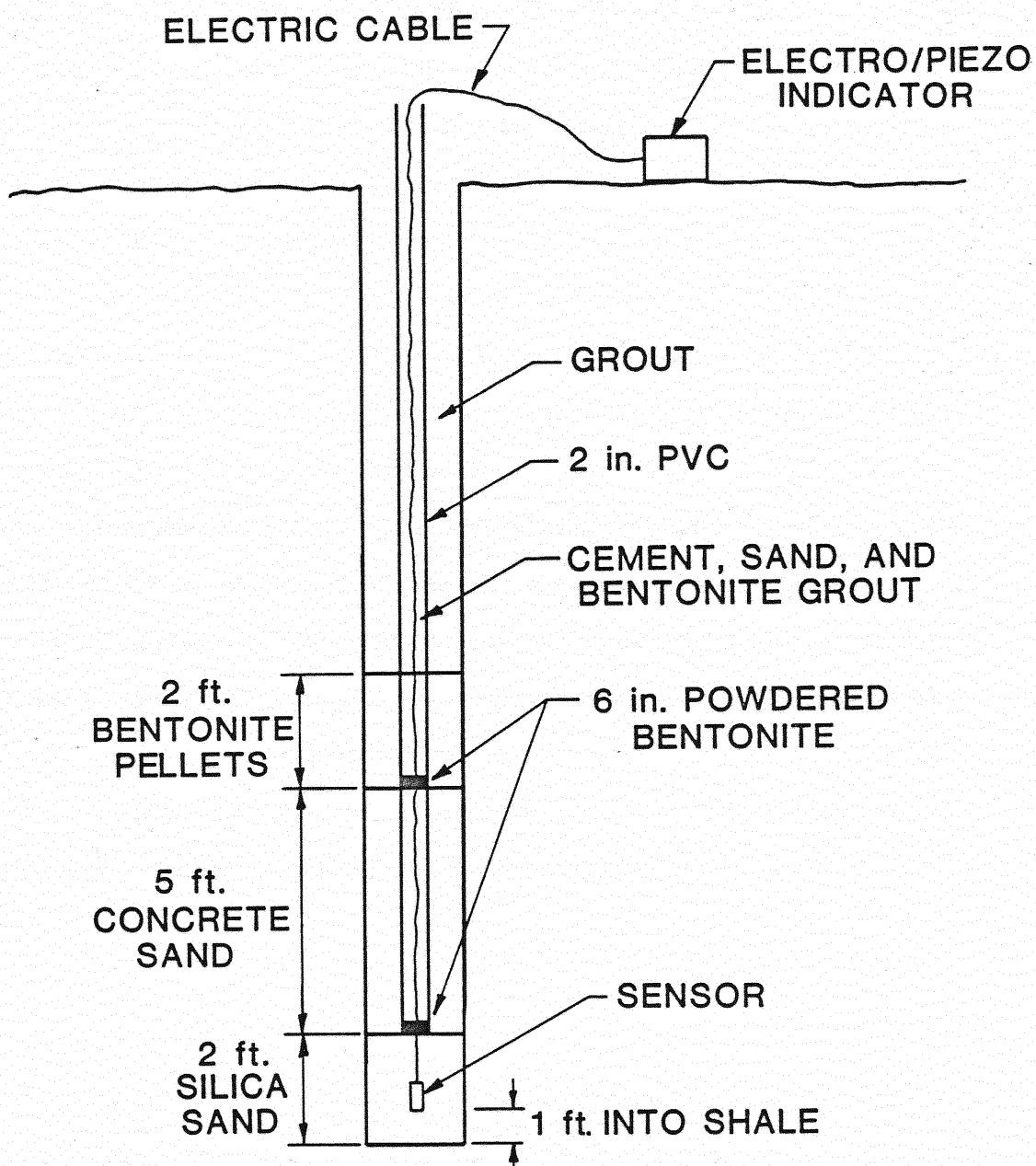
Figure 21. Piezometer Set-Up
