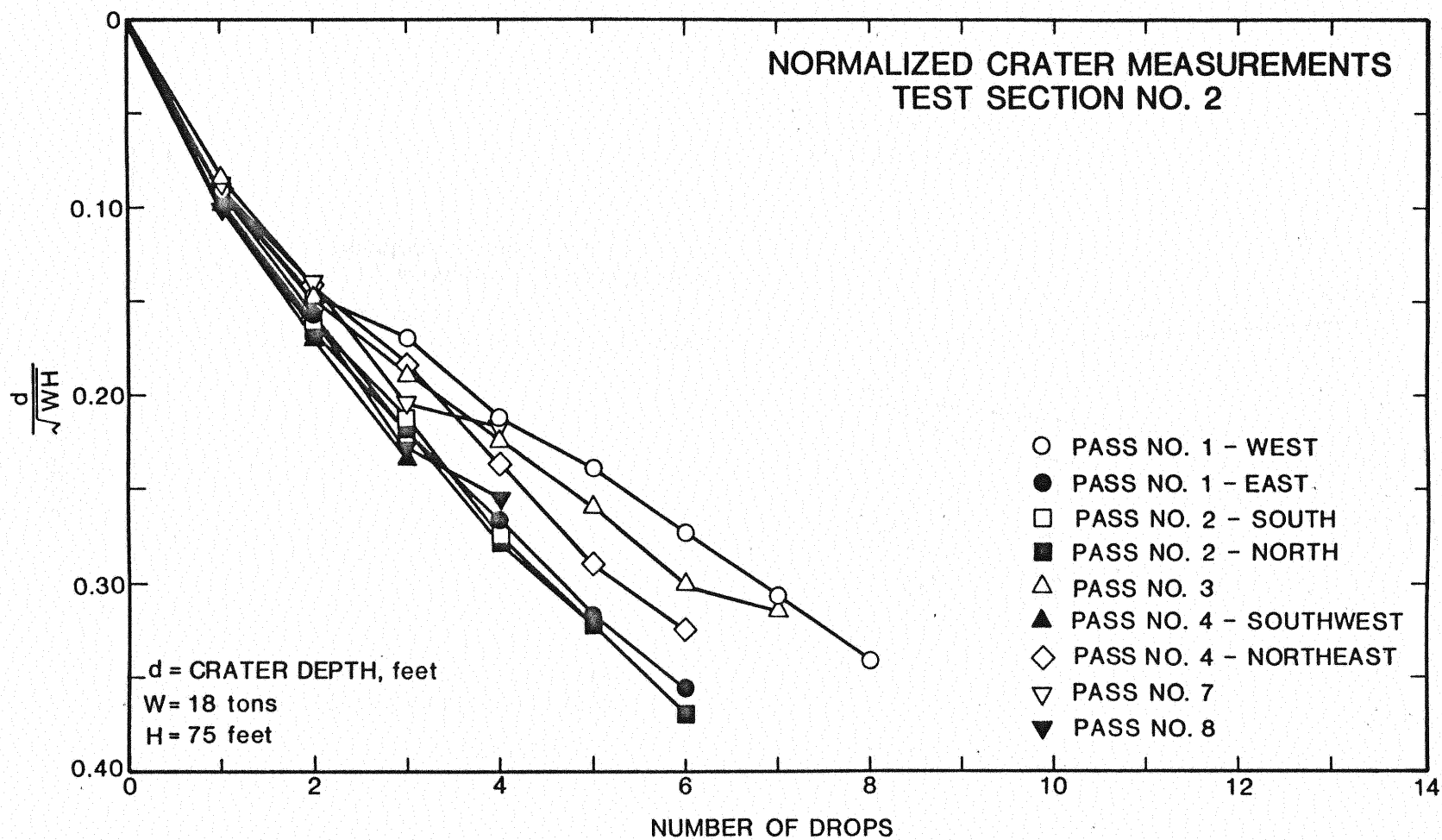
Figure 63. Normalized Crater Measurements, Test Section No. 2
