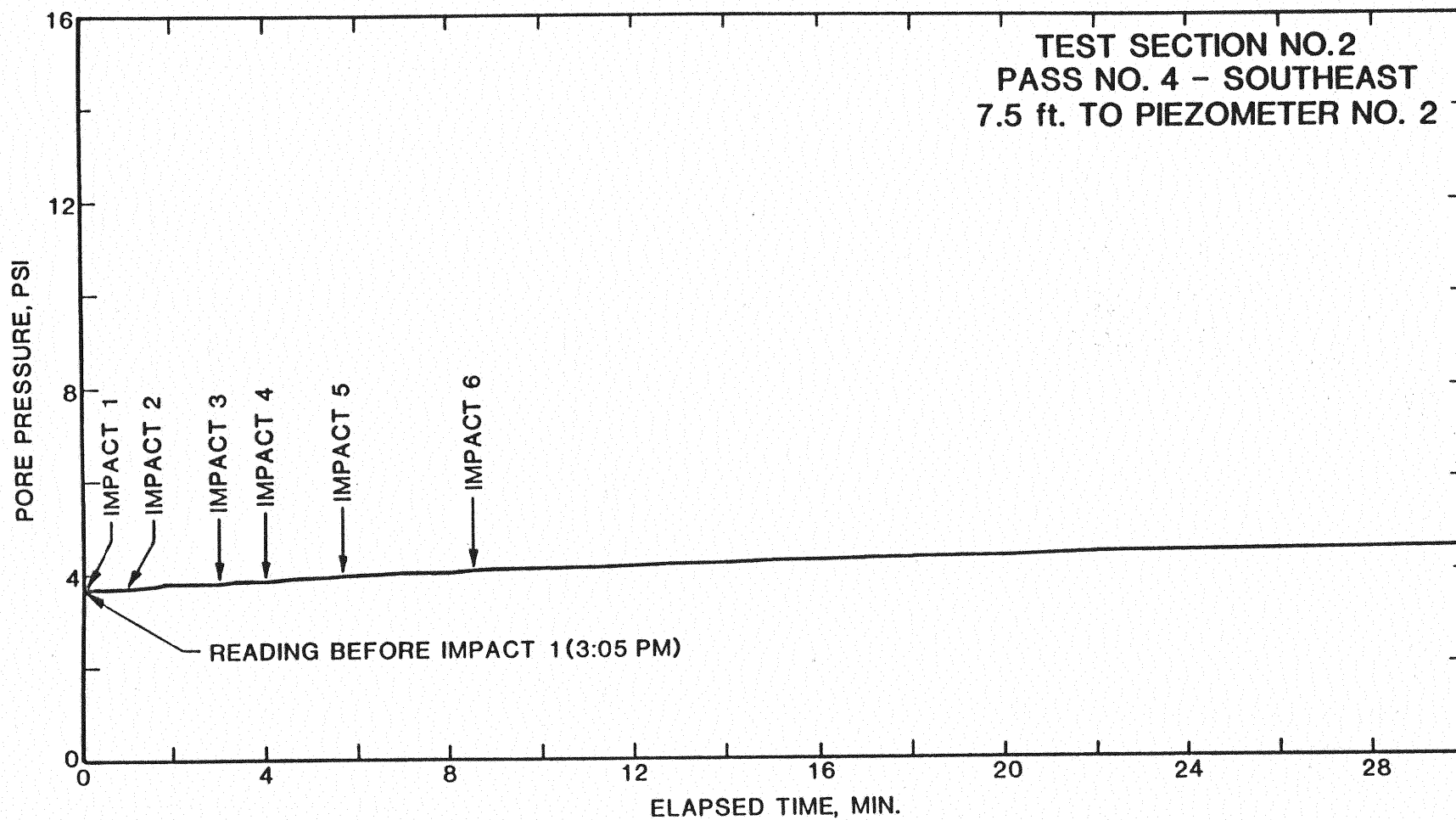
Figure 47. Piezometer Data, Pass No. 4 - Southeast, Test Section No. 2
