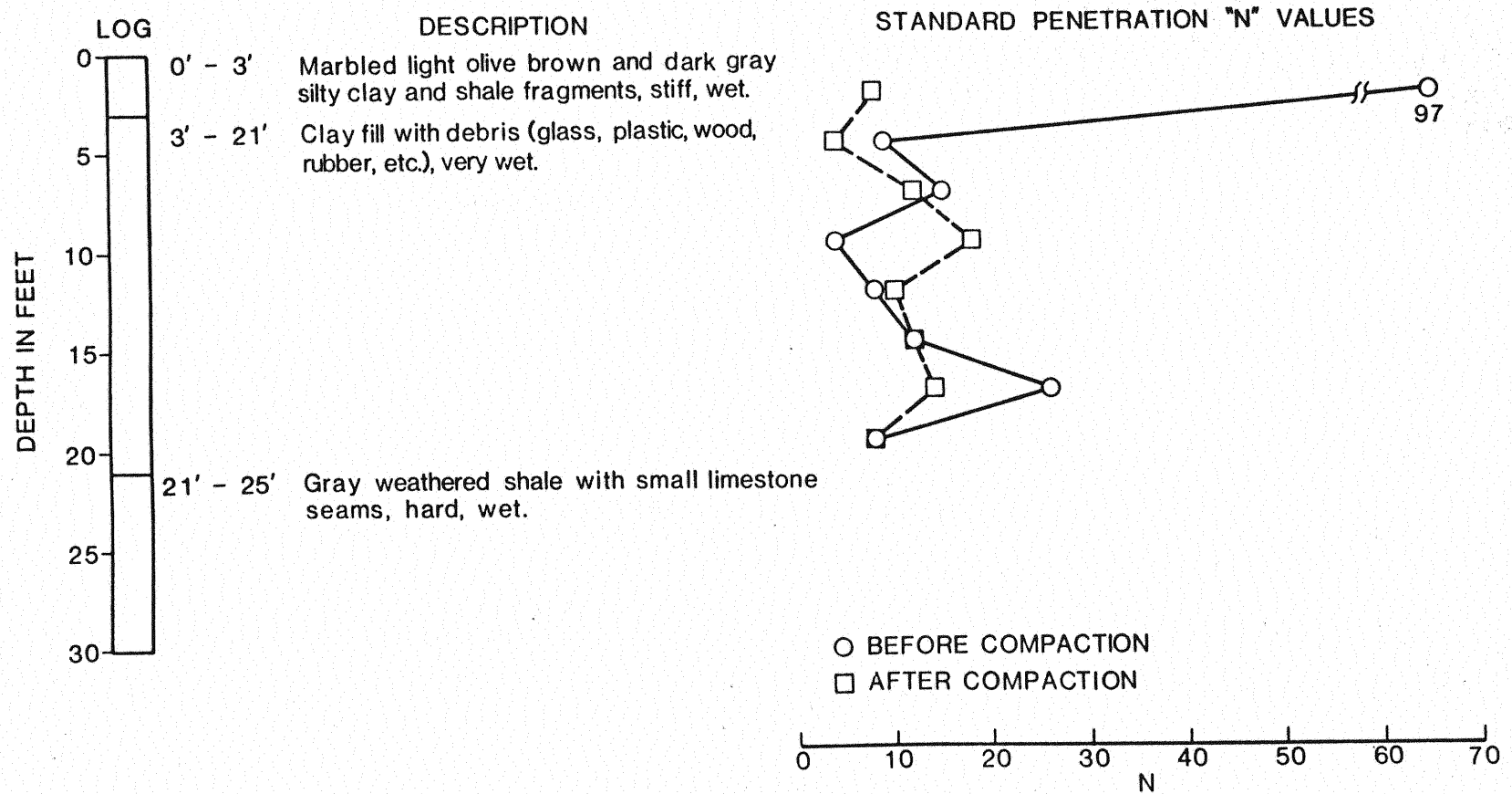
Figure 65. Standard Penetration Test Results, South of CRL, Test Section No. 2
