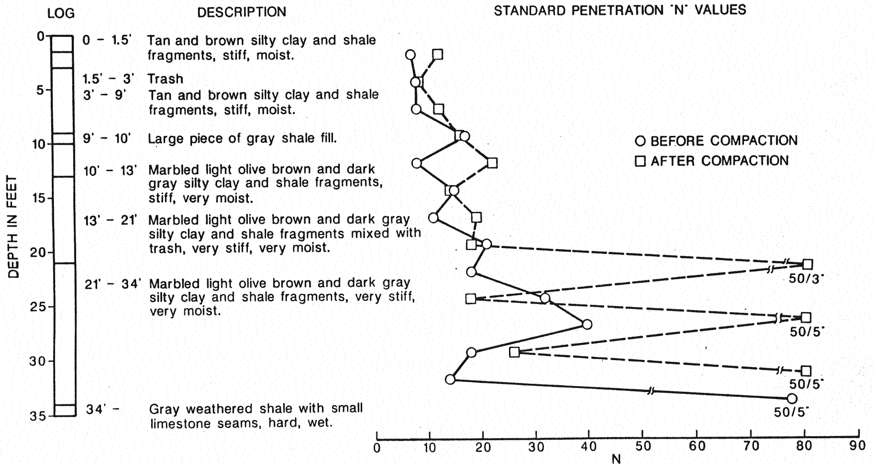
Figure 105. Standard Penetration Test Results, South of CRL, Test Section No. 3
