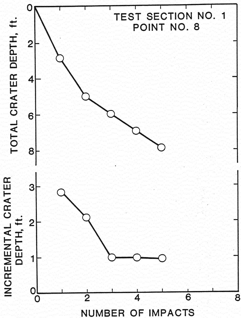
Figure 33. Crater Depth Versus Number of Impacts: Point No. 8, Test Section No. 1
