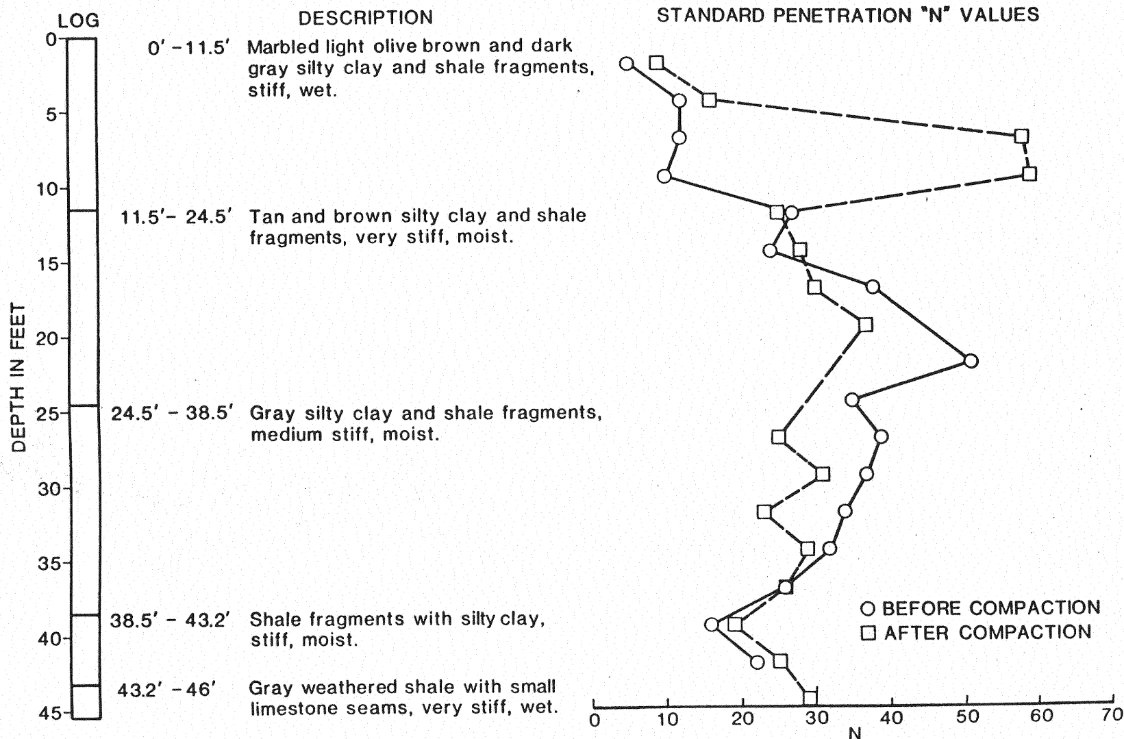
Figure 38. Standard Penetration Test Results, Along CRL, Test Section No. 1
