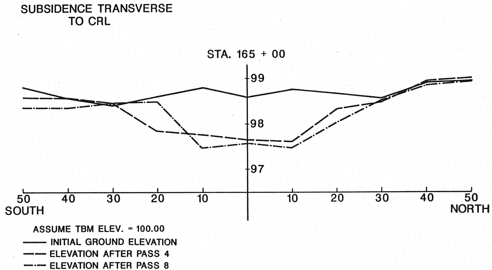
Figure 107. Post-Compaction Subsidence, Transverse to CRL, Test Section No. 3
