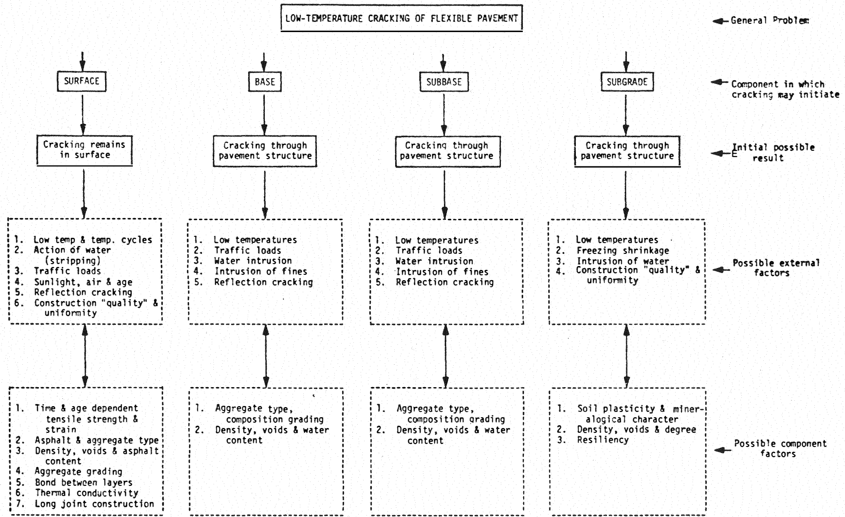
Figure 1. Factors of Possible Significance in Low-Temperature Cracking of Flexible Pavements (8)
