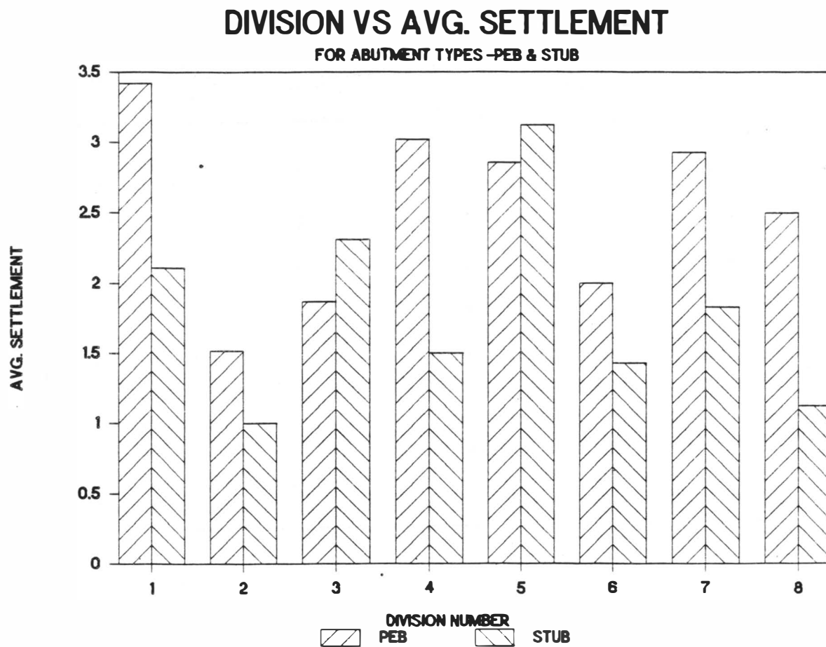
Fig. 5-8. Settlement vs. abutment type relationship.
