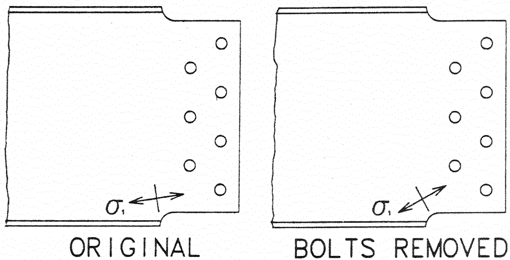
Figure 37. Comparison of Stresses in Original Detail to Stresses With Bolts Removed
