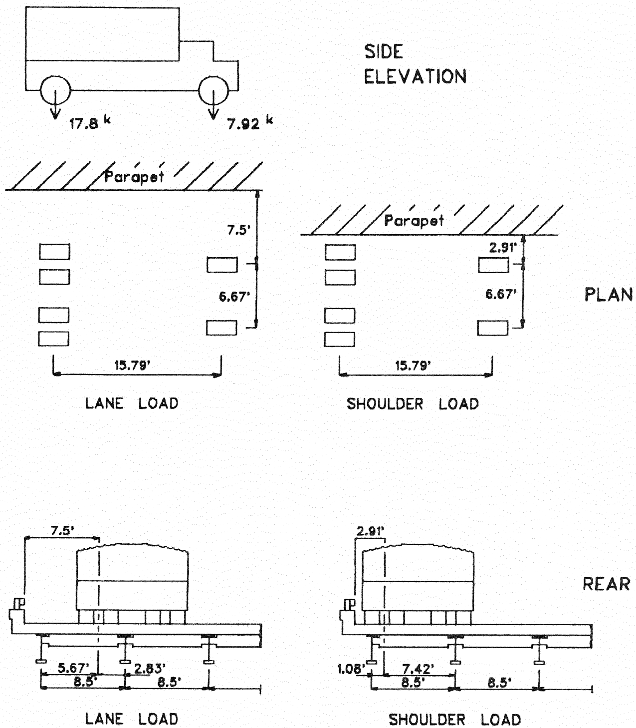
Figure 9. Tank Truck Used for Loading Bridge
