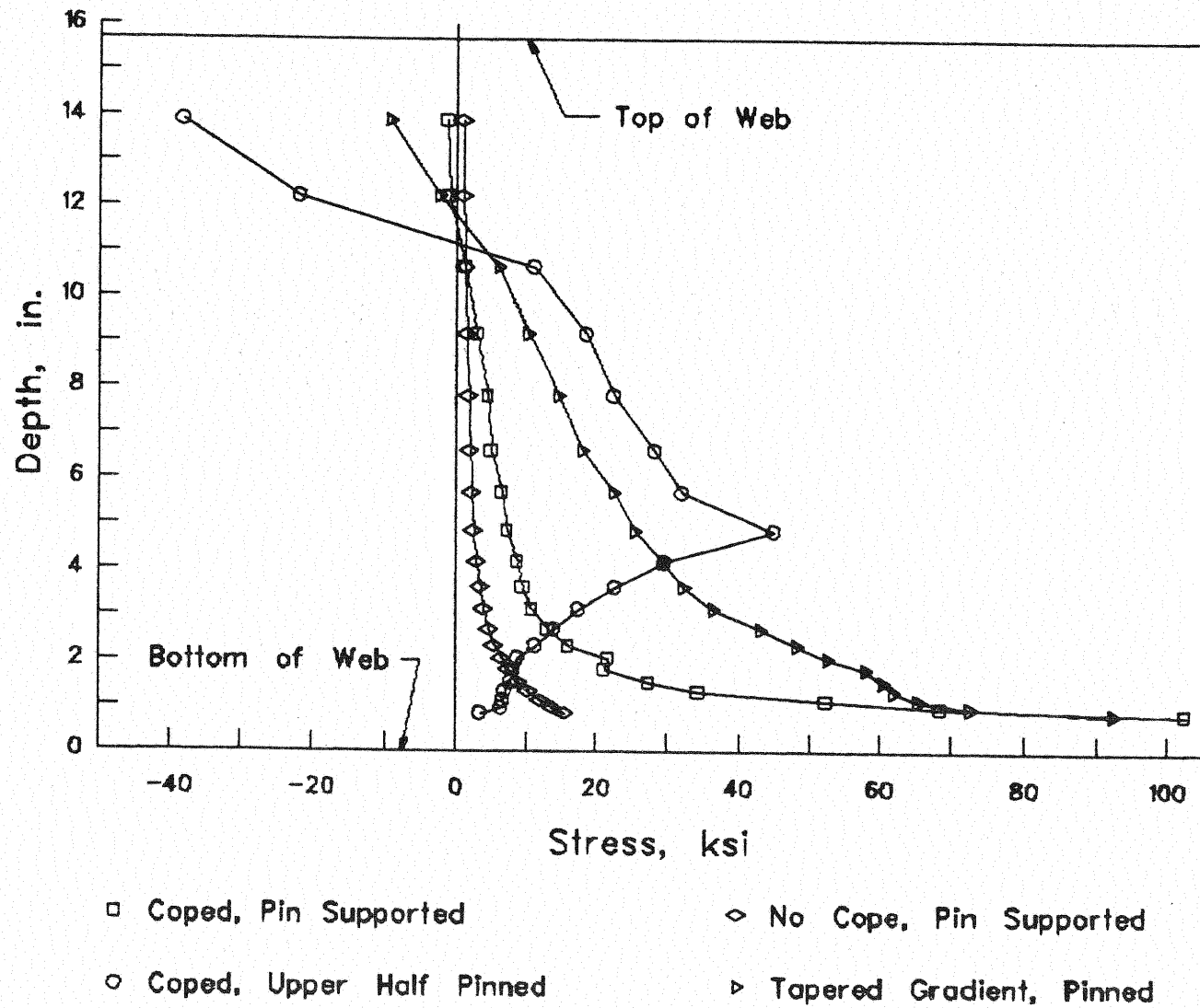
Figure 22. Stress Along Crack Line From Finite Element Analysis
