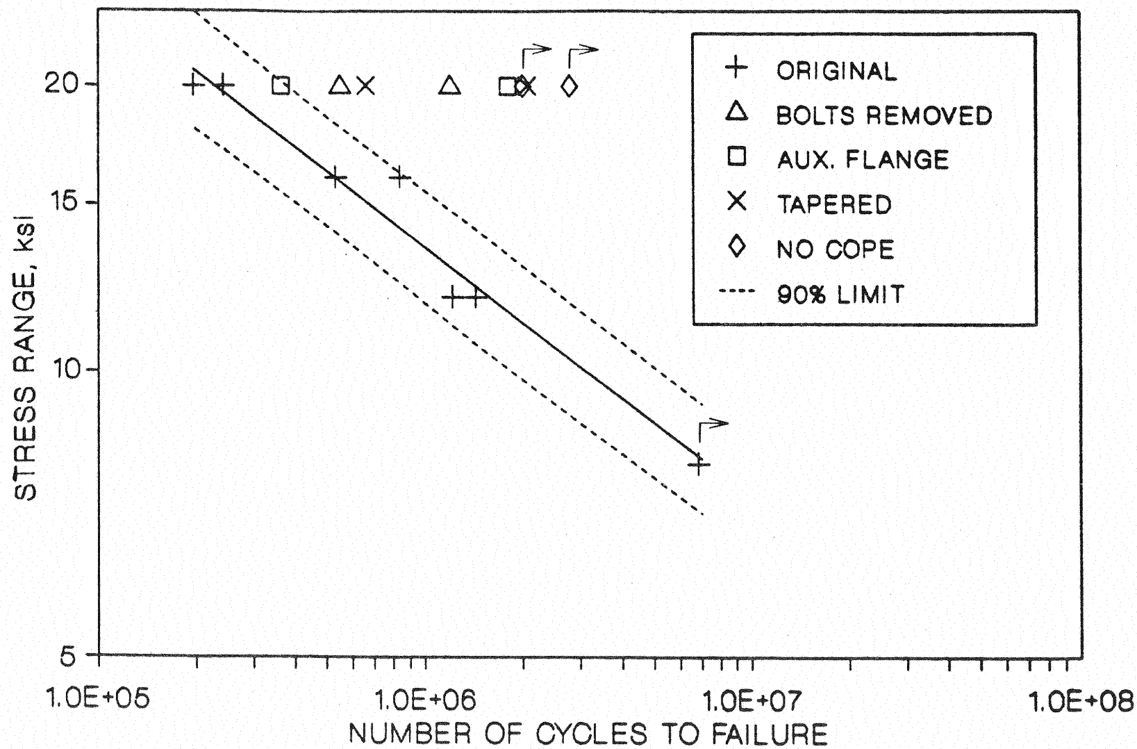
Figure 35. Fatigue Life of All Specimens
