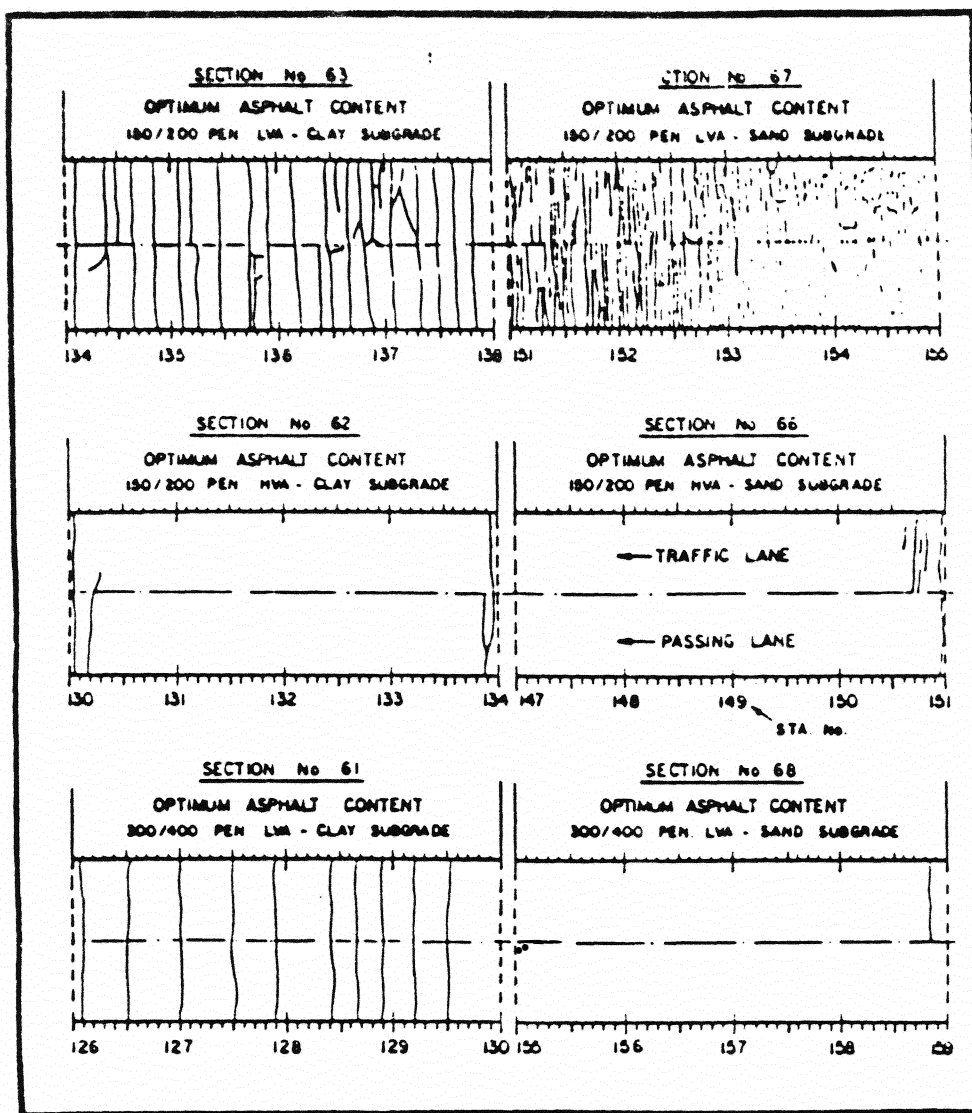
Figure 4. Example of Crack Survey Measurements at St. Anne Test Road [1]
