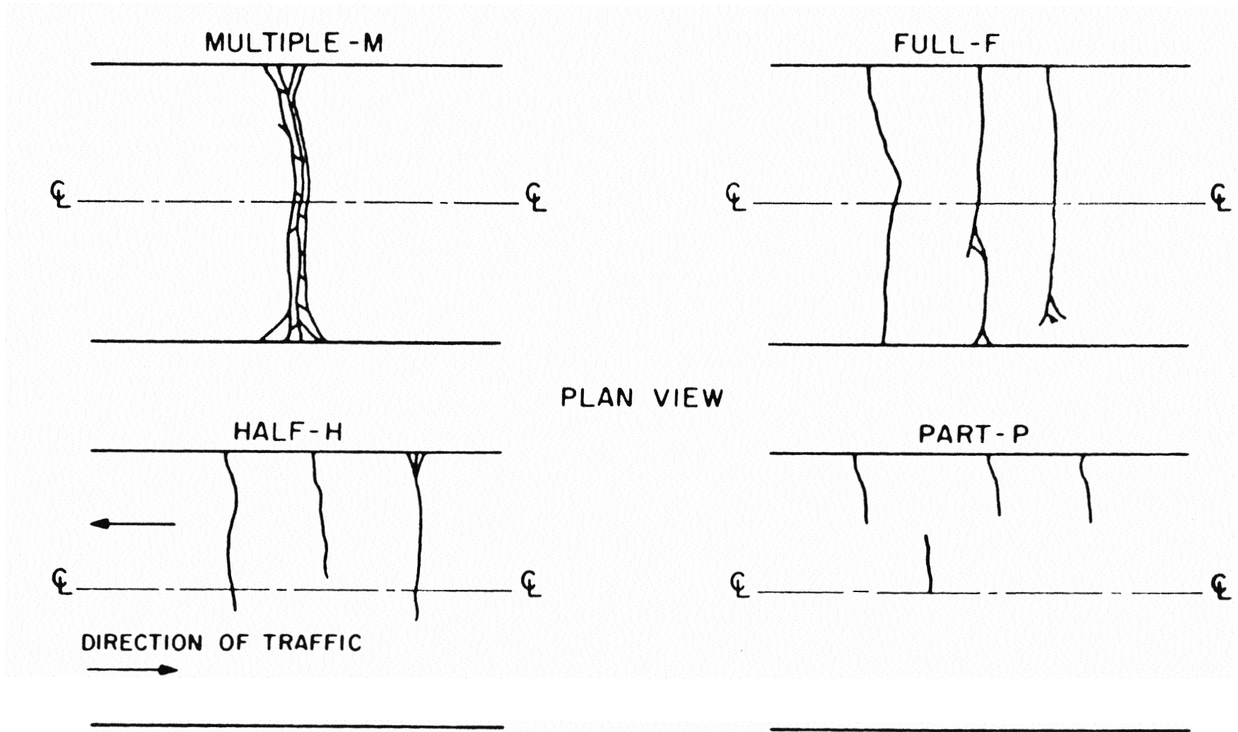
Figure 3. Different Types of Transverse Cracks [14]
