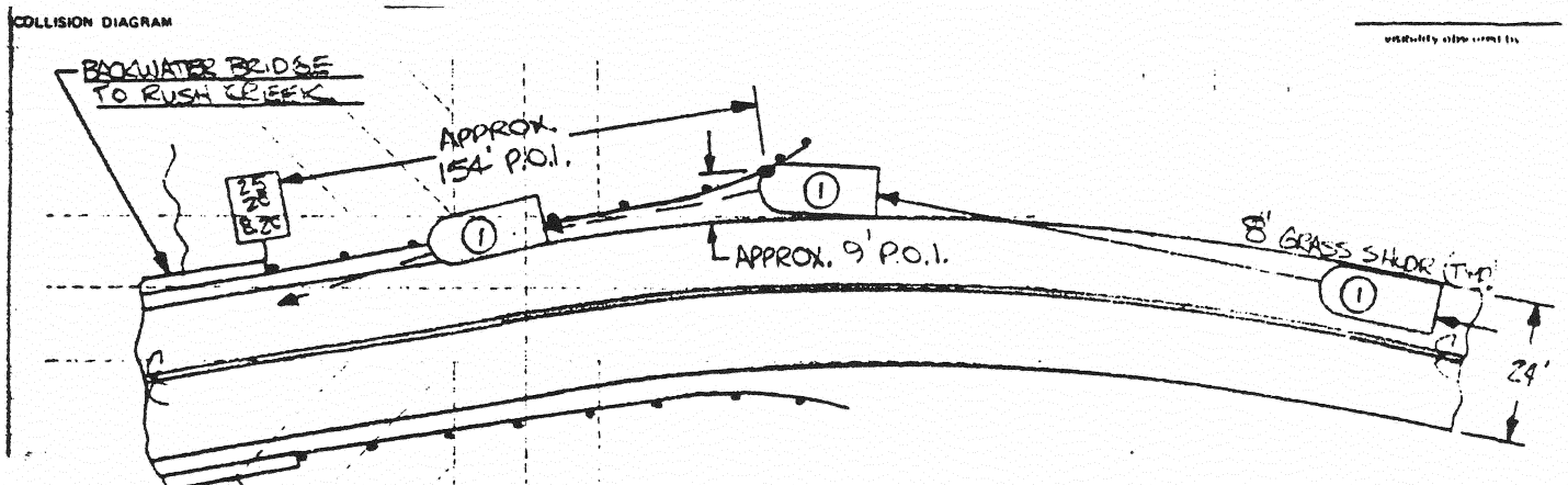
Questionable guardrail front end accident (DPS # 047714627)
