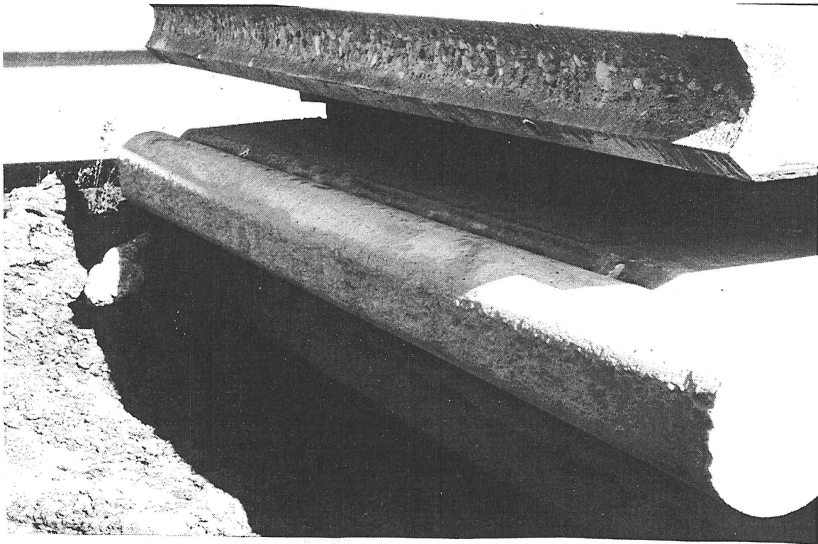
Figure 18. Sandblasted Joints.
