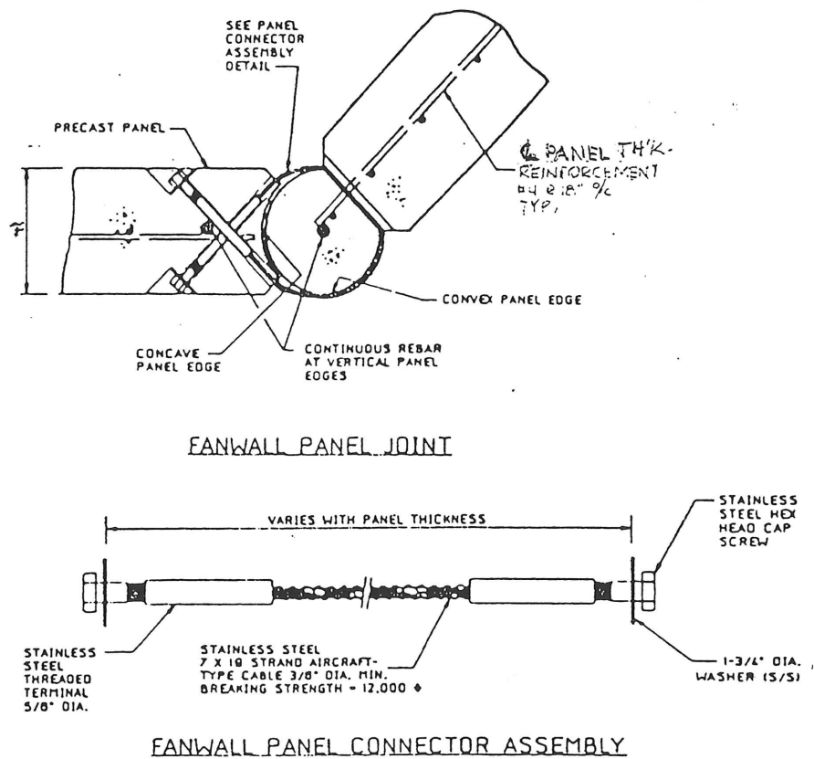
Figure 6. FANWALL Panel Joint and Connector Assembly.
