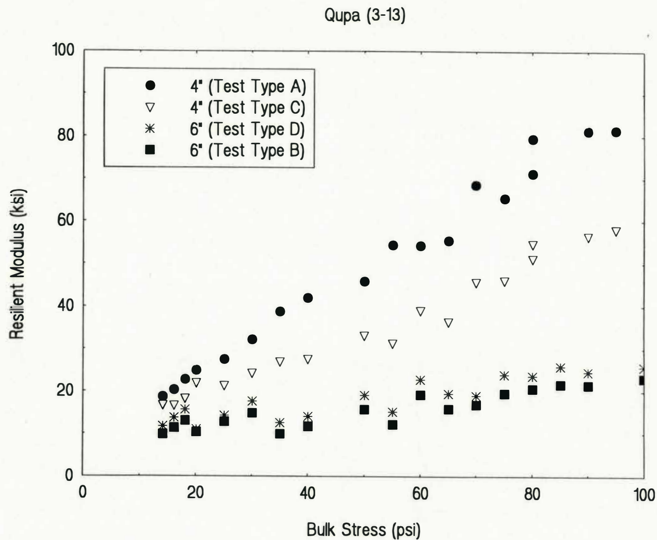
Fig. 3-13 Effects of the Compaction on the Resilient Moduli for 4" and 6" Specimens for the Aggregate from Creek County (Limestone)
