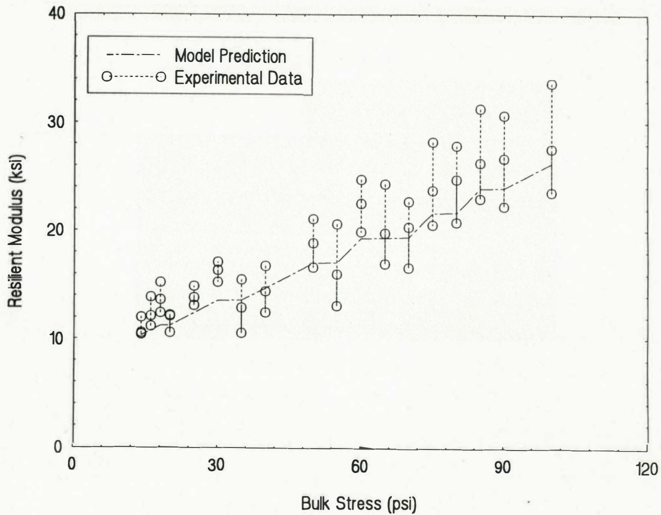
Fig. 4-3 Comparison of Model Prediction (Eq. 4-3) and Experimental Observed RM Values for Aggregate from Comanche County (Limestone)
