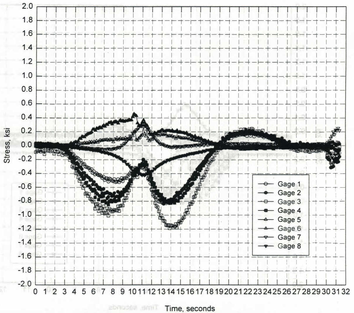
Figure 21. Truck Moving at 5 mph in Shoulder, from Measurements at Group 1 Location
