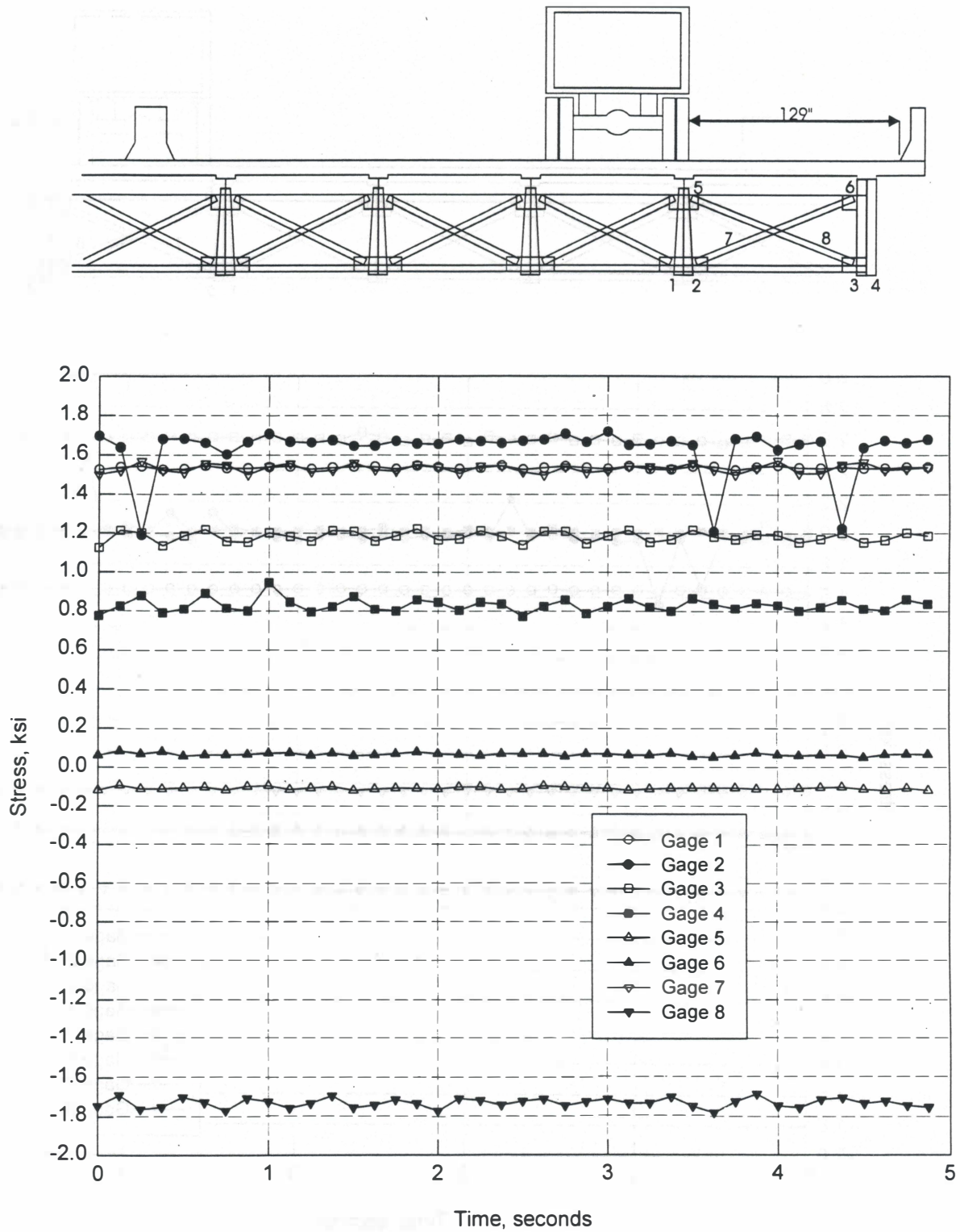
Figure 30. Truck Stationary in Right Lane, from Measurements at Group 3 Location
