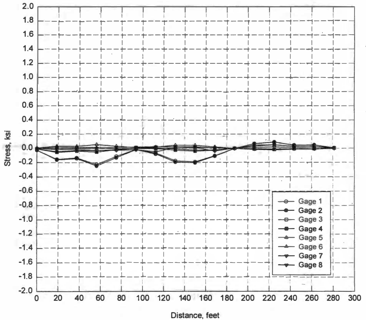
Figure 45. Truck Moving in Left Lane, Finite Element Analysis at Group 1 Location
