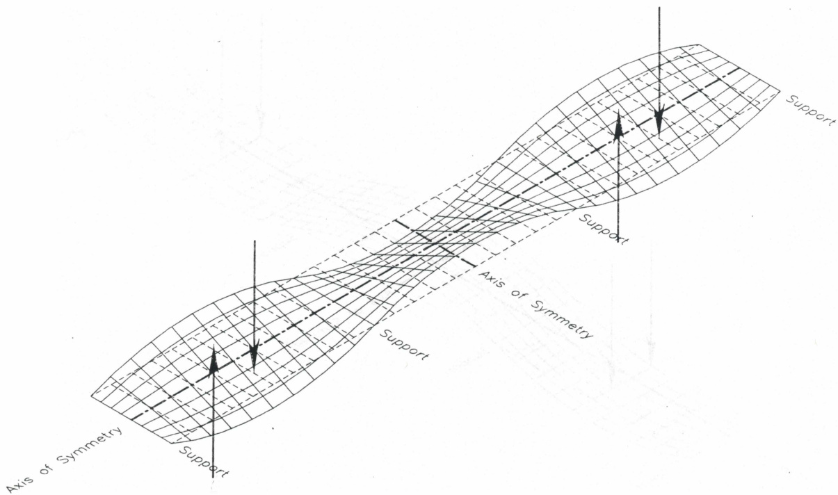
Figure 16. Symmetry of Loading in the Longitudinal Direction, Anti-symmetry of Loading in the Transverse Direction
