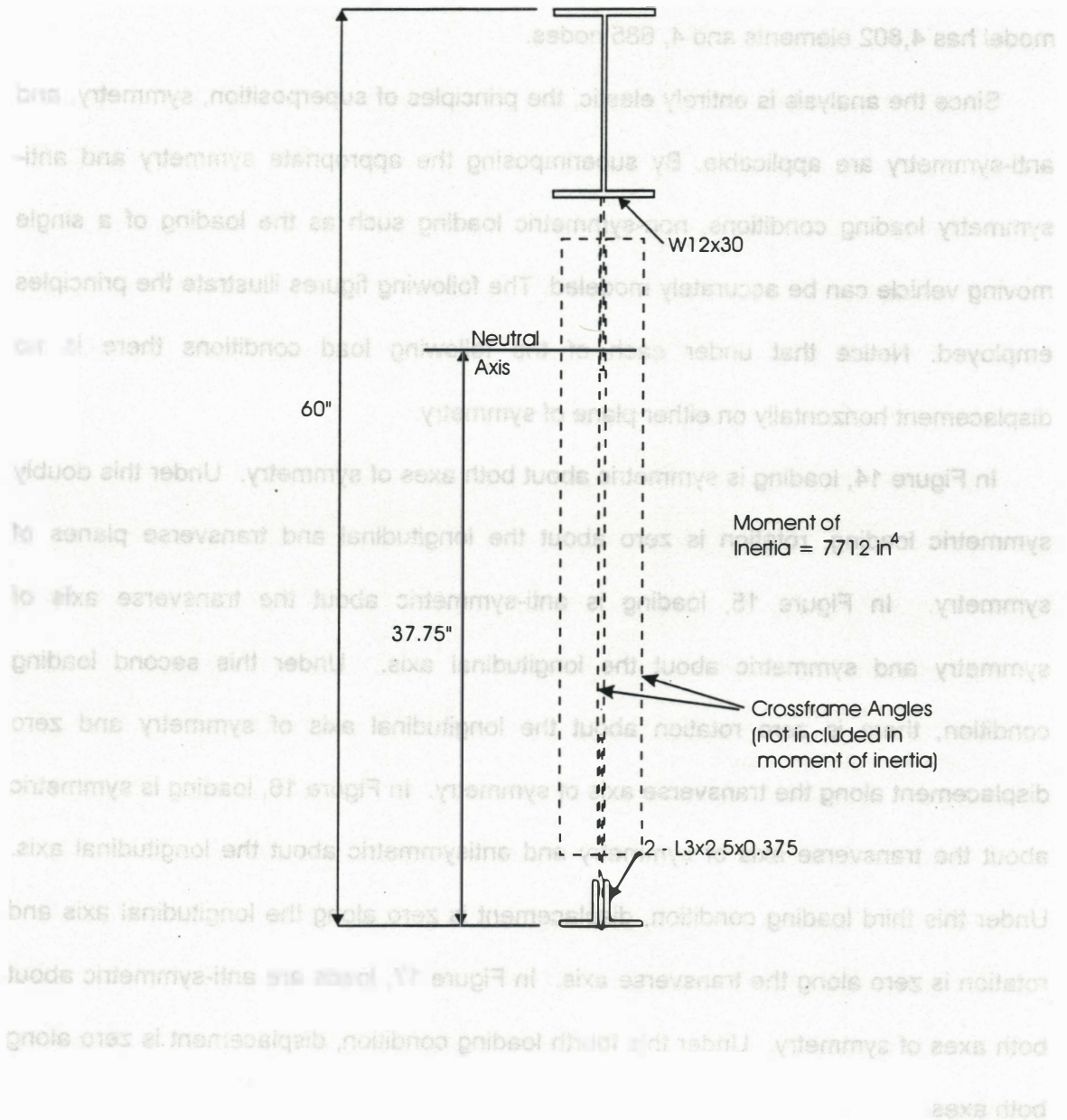
Figure 13. Crossframe Section Properties
