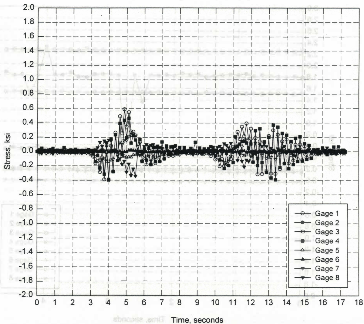
Figure 35. Truck Moving at 40 mph in Left Lane Followed by Tractor-Trailer, Without Gages 2 and 3
