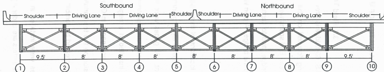
(b) Cross Section
