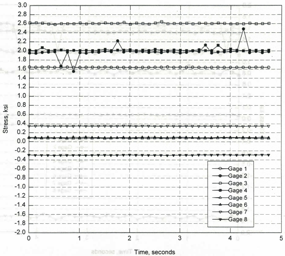
Figure 29. Stationary Truck in Shoulder, from Measurements at Group 3 Location
