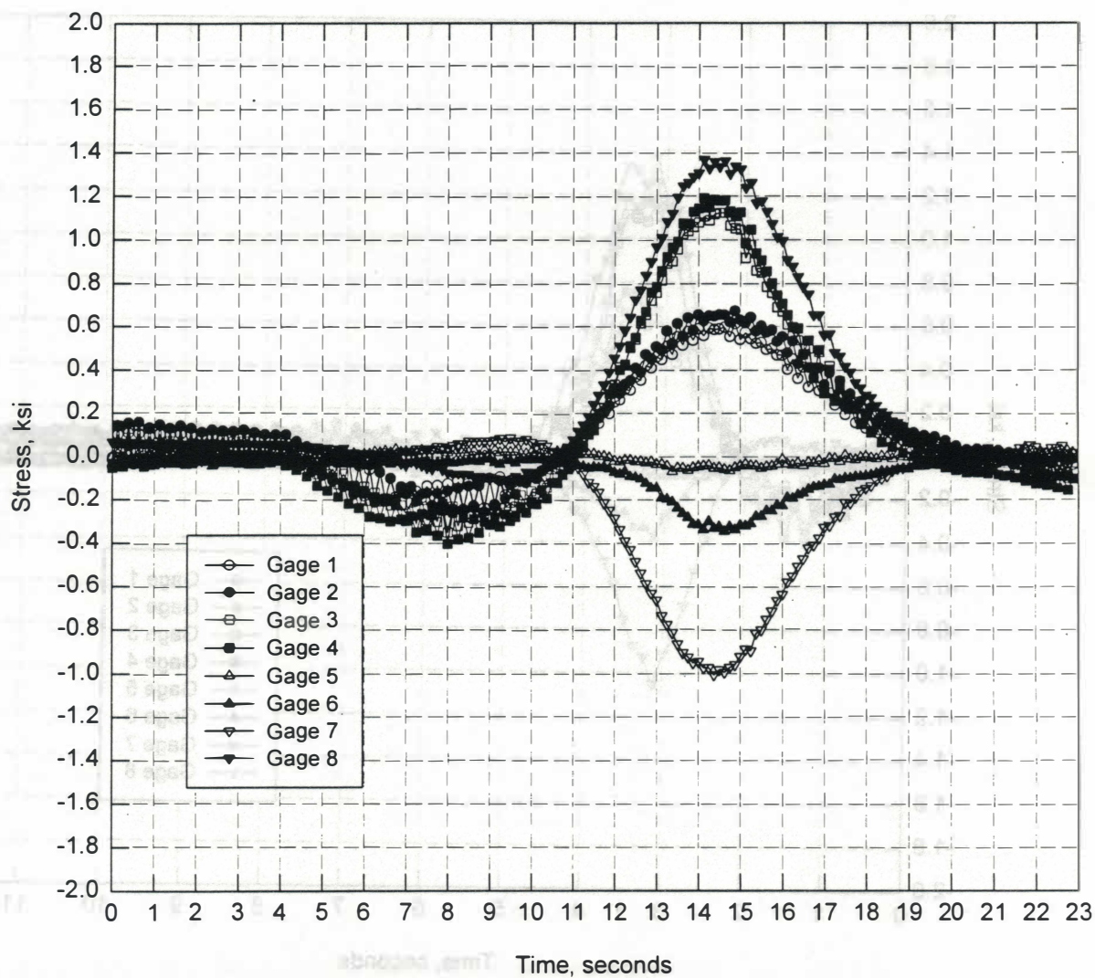
Figure 25. Truck Moving at 5 mph in Right Lane, from Measurements at Group 2 Location
