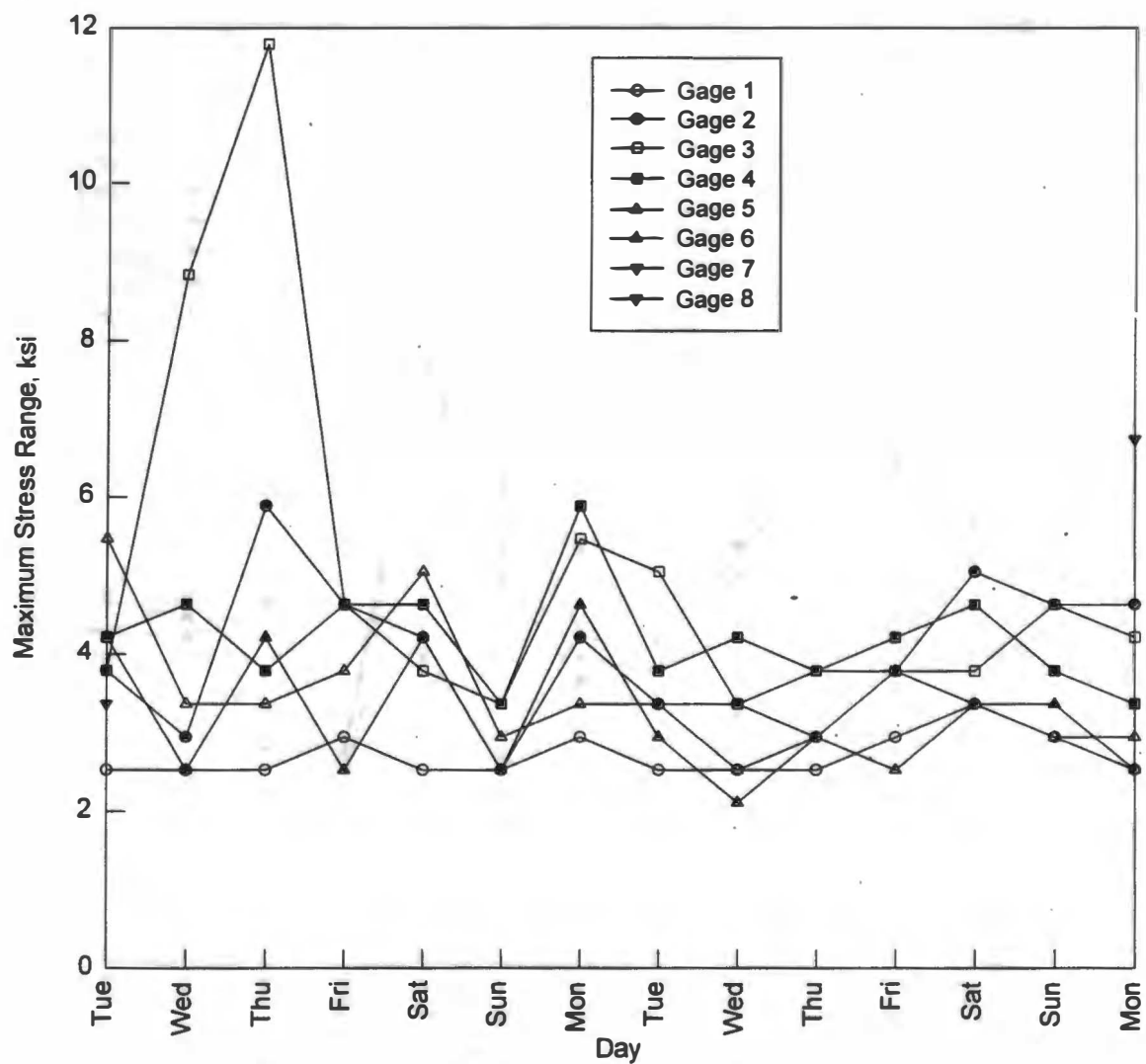
Figure 59. Maximum Stress Range Each Day Over a Two Week Period, Channels 7 and 8 Omitted
