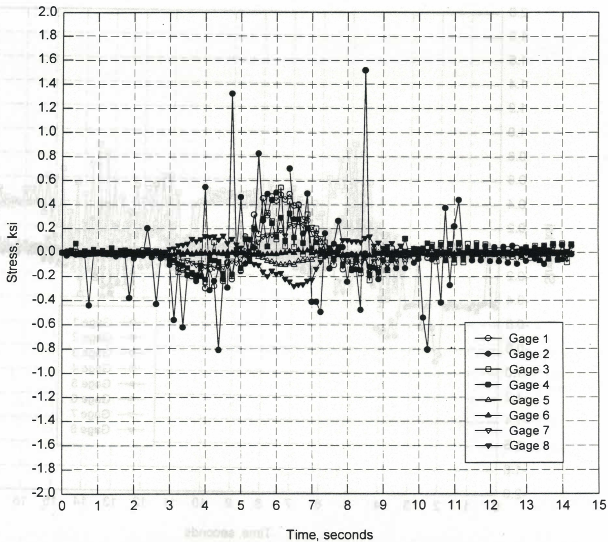
Figure 33. Truck Moving at 25 mph in Left Lane, from Measurements at Group 3 Location
