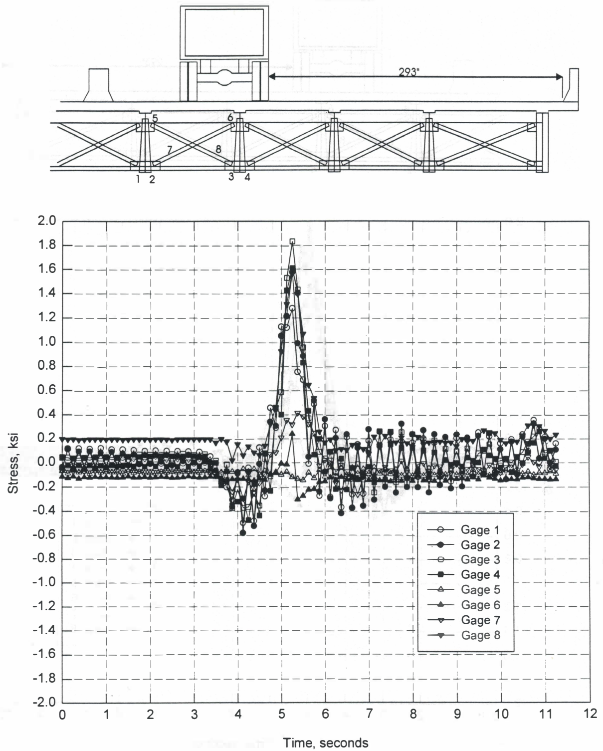
Figure 28. Truck Moving at 40 mph in Left Lane, from Measurements at Group 2 Location
