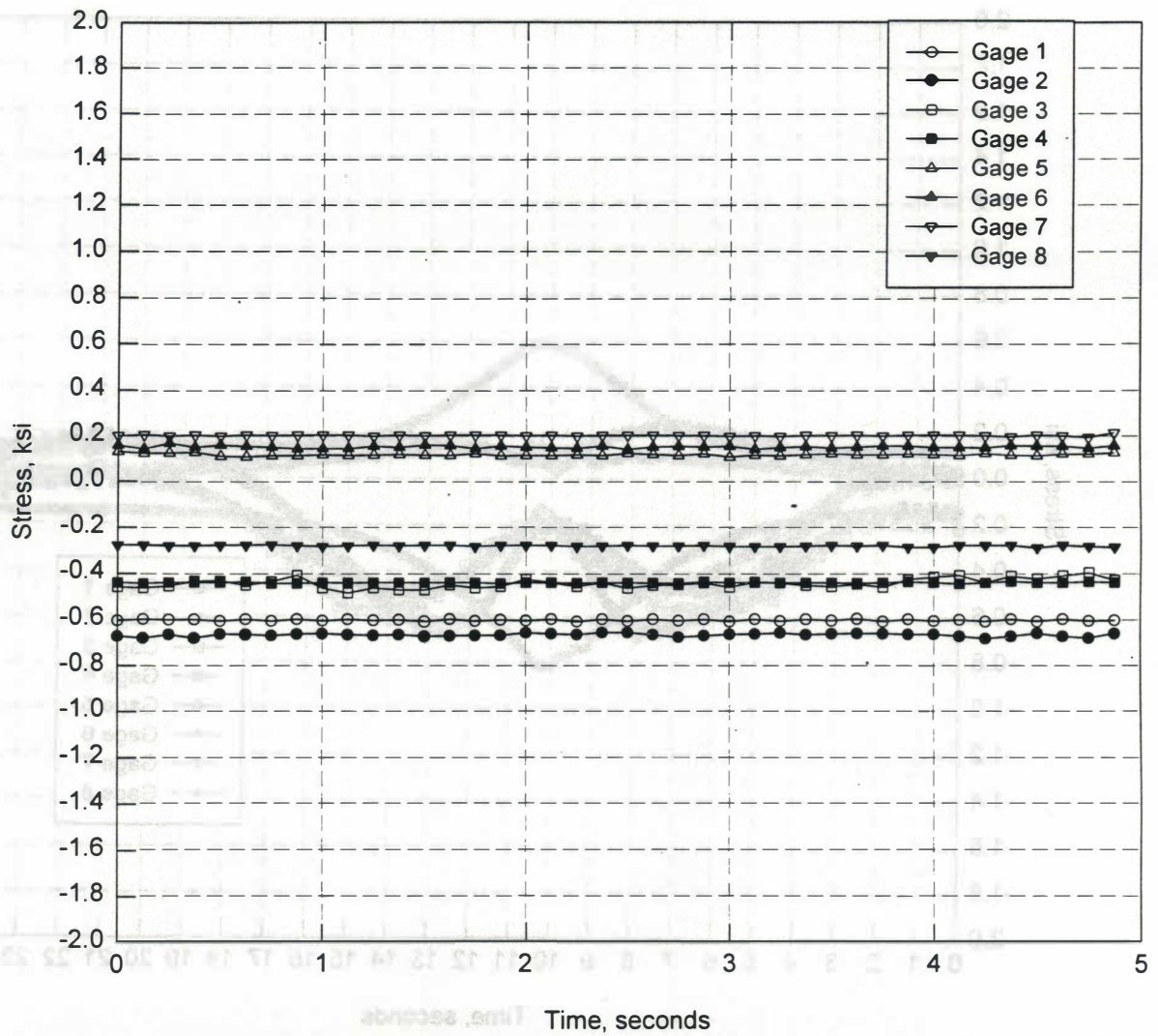
Figure 19. Stationary Truck in Right Lane, from Measurements at Group 1 Location
