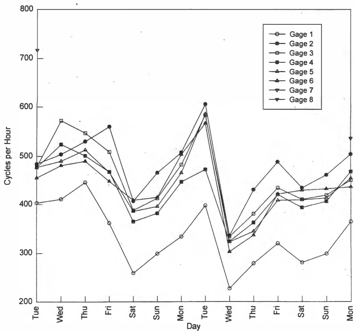
Figure 60. Cycles per Hour Each Day Over a Two Week Period, Channels 7 and 8 Omitted
