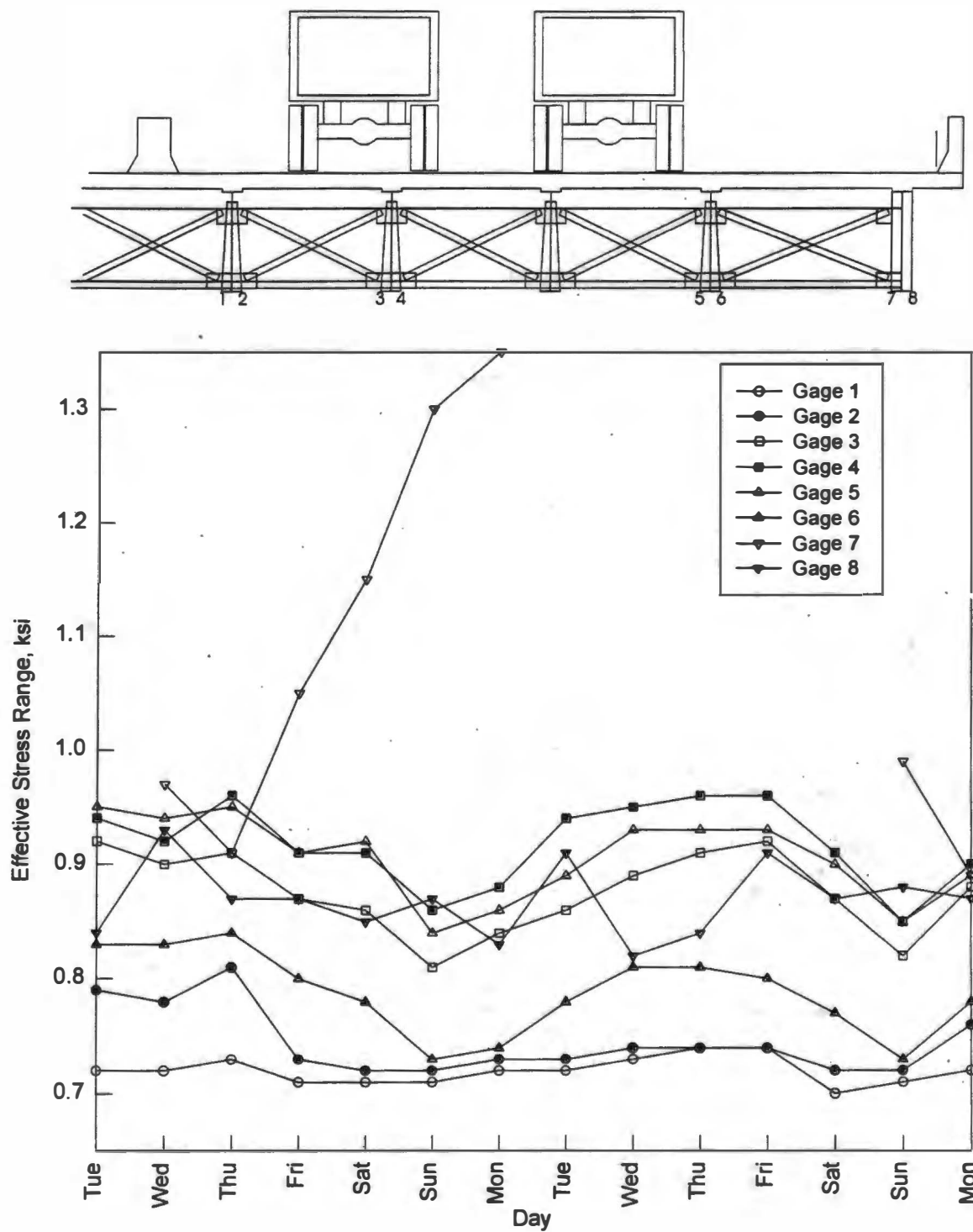
Figure 54. Effective Stress Ranges Over a Two Week Period
