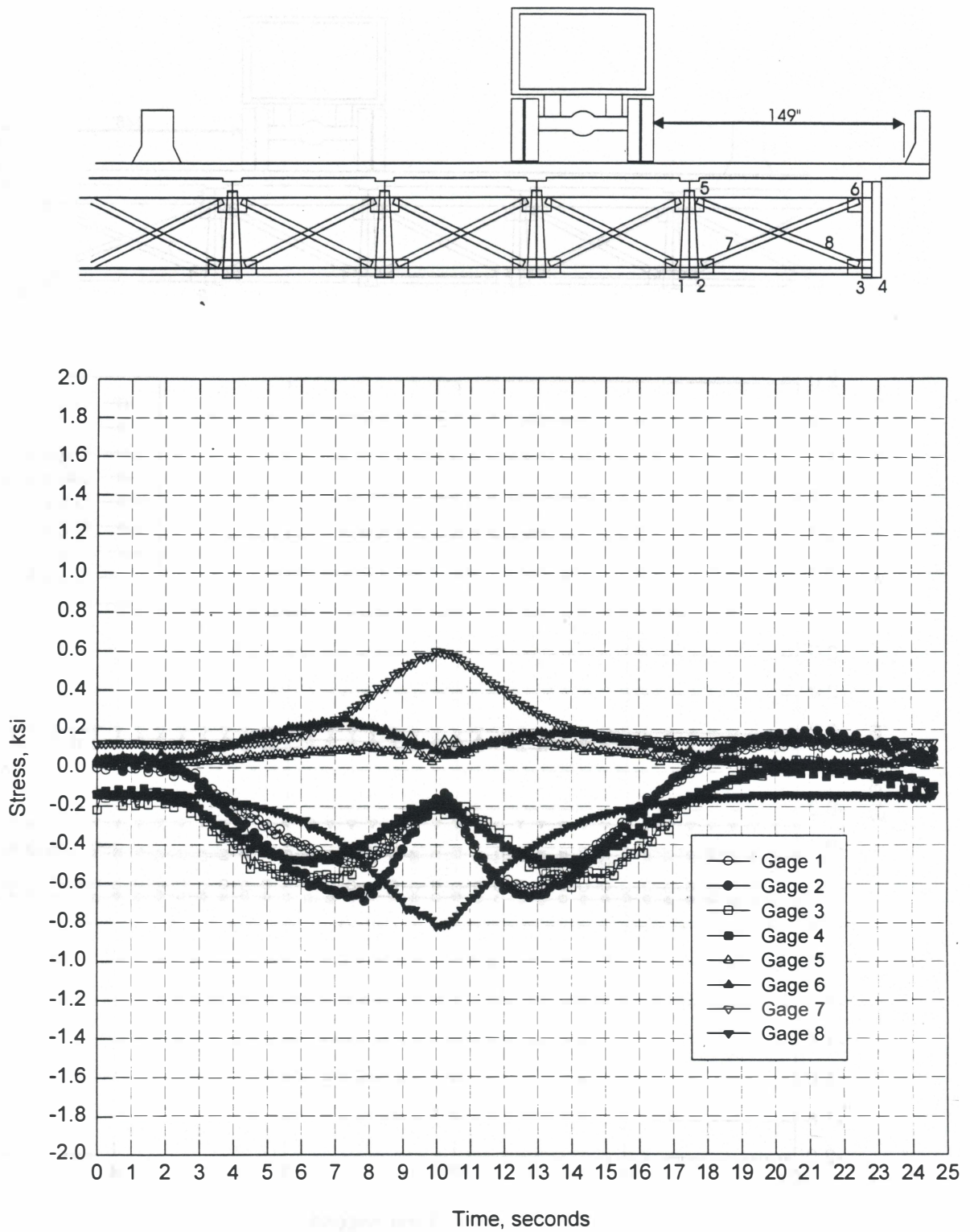
Figure 20. Truck Moving at 5 mph in Right Lane, from Measurements at Group 1 Location
