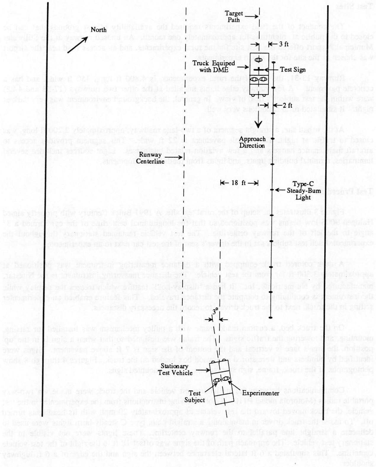
Figure 3. Setup of Rural Test Site
