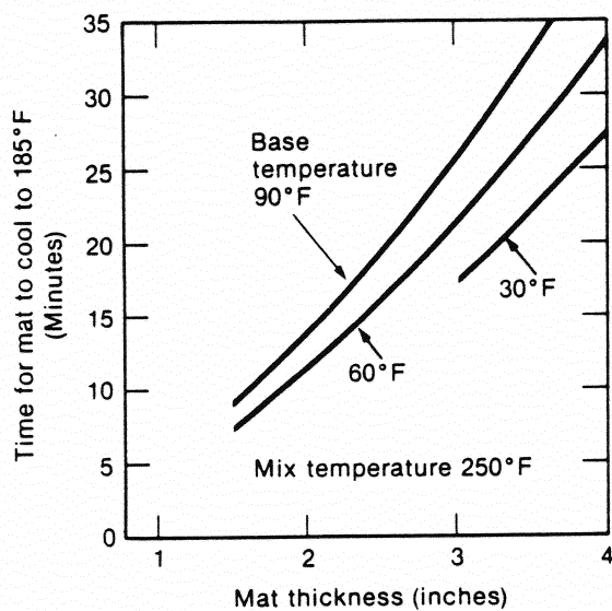
Times for asphalt to cool to 185°F.
