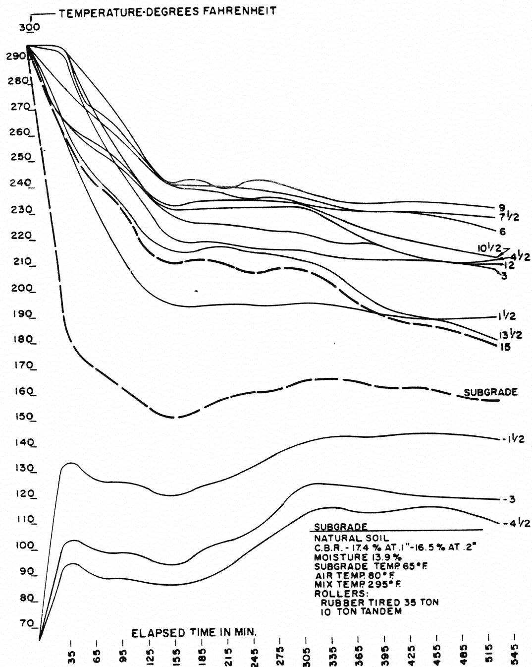
Fig. 2-10 Cooling Temperatures During Application of Hot Plant Mix Stabilized Base (Single Lift 15 inches Compacted Thickness) [Beagle, 1966]
