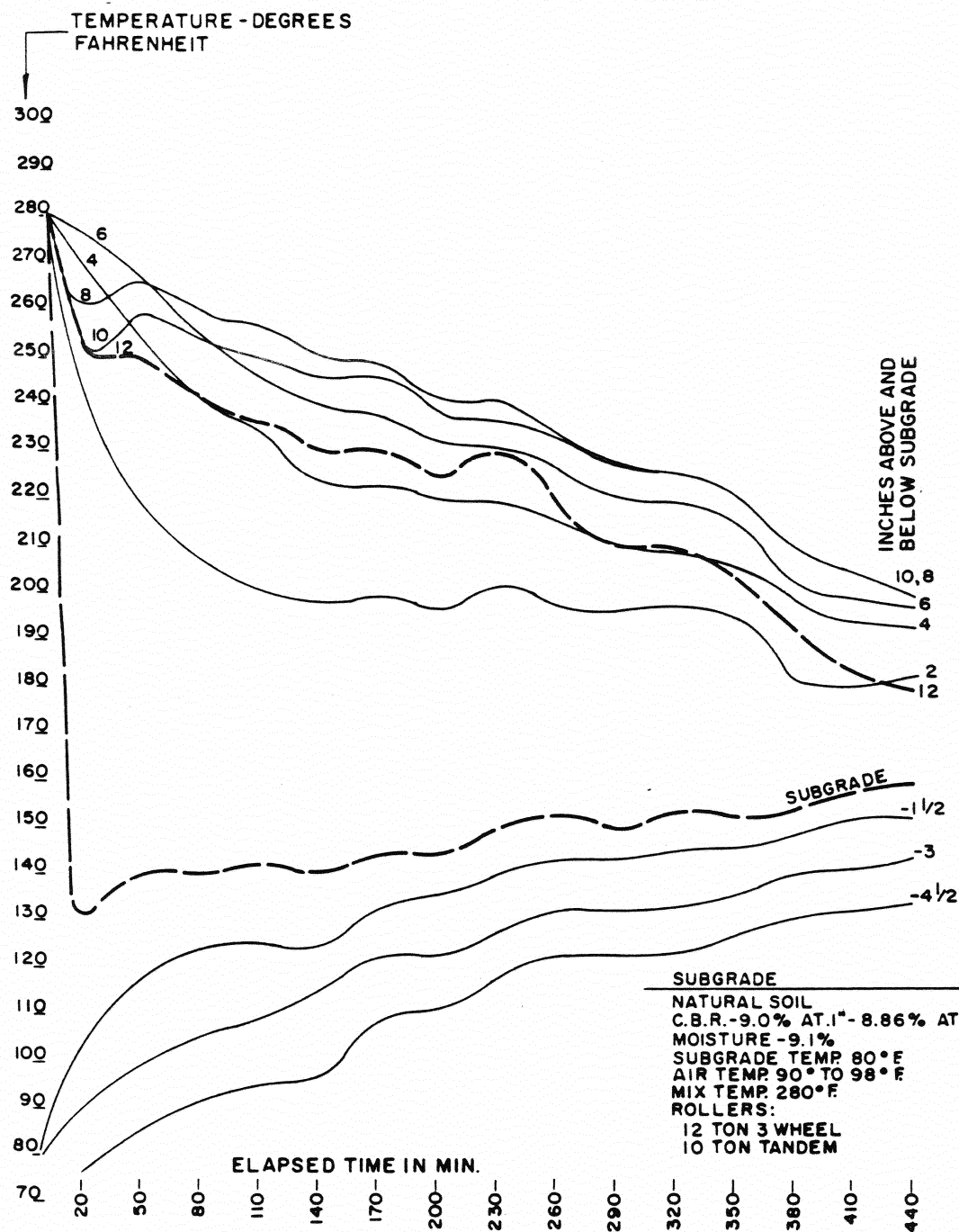
Fig. 2-9 Cooling Temperatures During Application of Hot Plant Mix Stabilized Base (Single Lift 12 inches Compacted Thickness) [Beagle, 1966]
