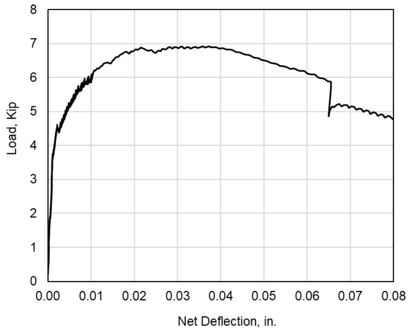
Figure C.1: Load versus Deflection for A-1
