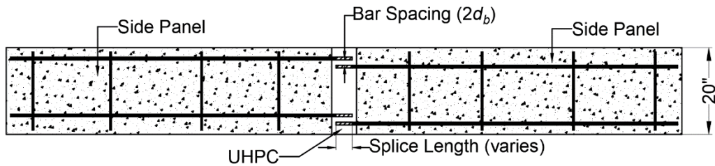
Figure 2.23: Bars Spliced in Compression Region Plan View
