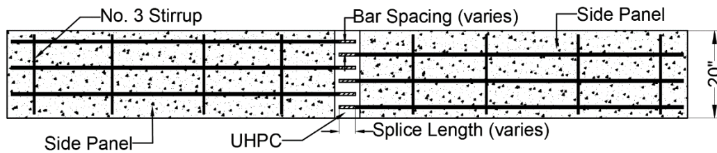
Figure 2.22: Test Splices Plan View
