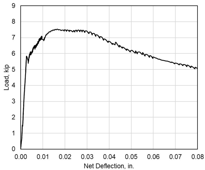
Figure C.6: Load versus Deflection for A-6
