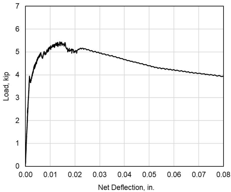
Figure C.2: Load versus Deflection for A-2
