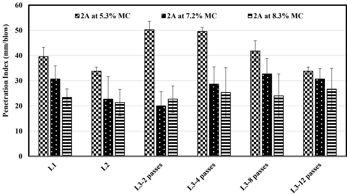
Figure 102. Penetration index of 2A material at various moisture contents tested in the Pit.
