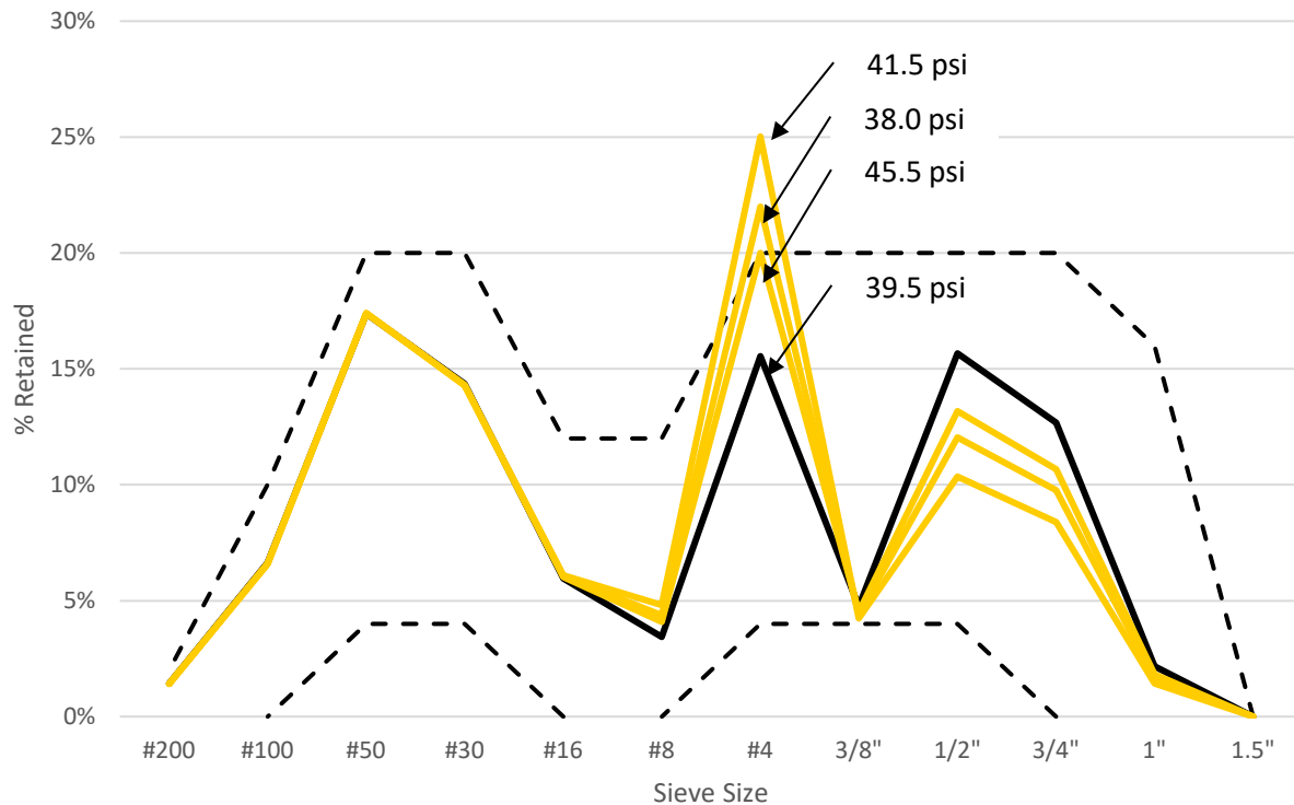
Figure 5-16 Sensor 2 pressures at 1500 rpm at 0 minutes per intermediate gradation. Desirable gradations are in black, undesirable are in yellow, and unacceptable are in red.
