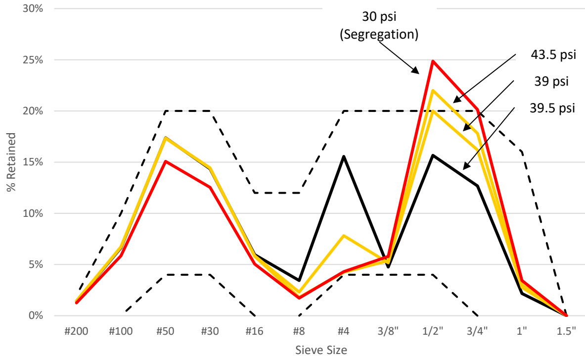
Figure 5-14 Sensor 2 pressures at 1500 rpm at 0 minutes per coarse gradation.
