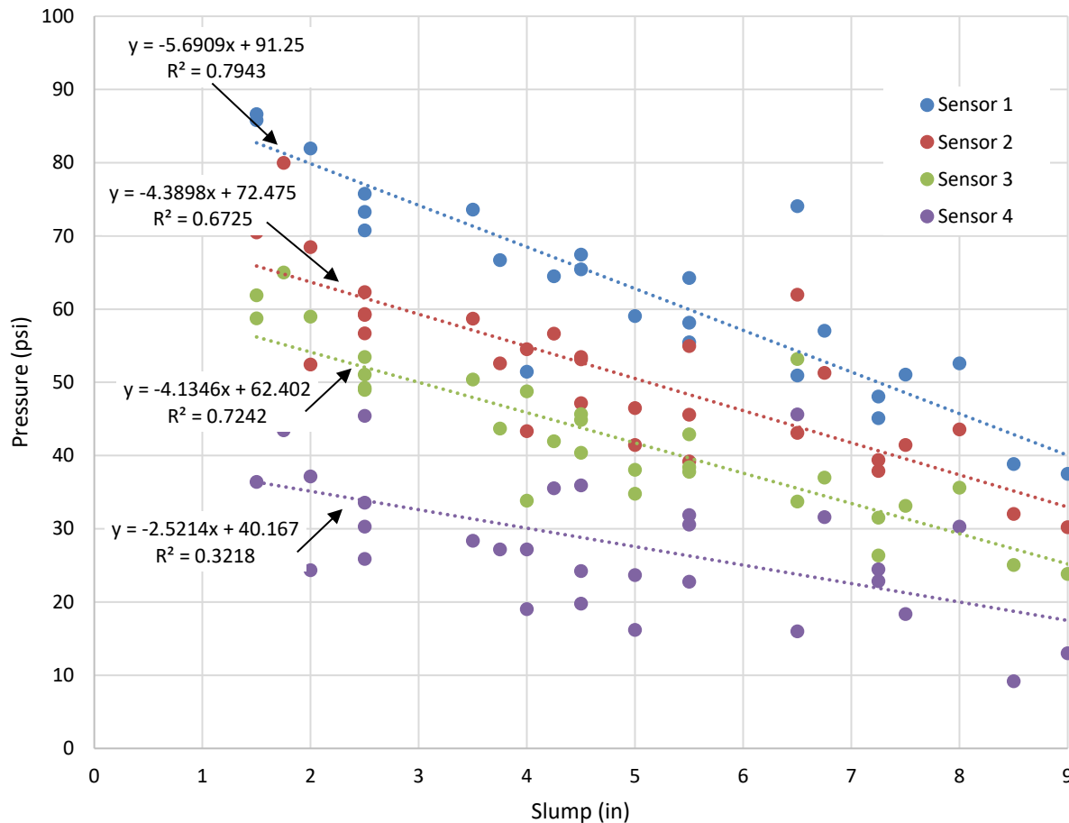
Figure 5-9: Pumping pressure versus slump.
