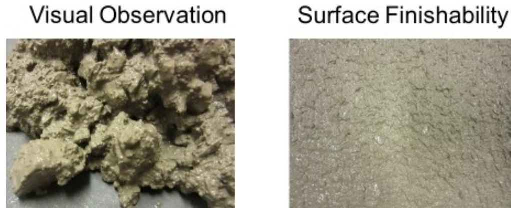
Figure 4-9: Pictures of mixtures with excessive amounts of #30 in mixture 27
