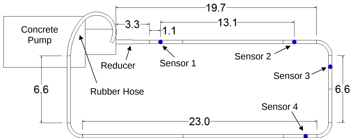
Figure 5-2: Plan view of the pump layout (units in feet).
