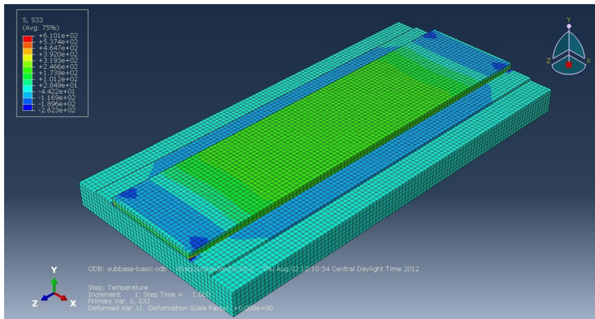
Figure 6.9 Distribution of normal stress in the longitudinal direction (S33)
