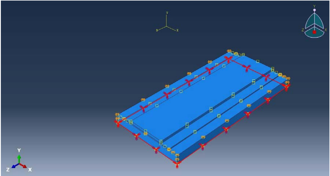
Figure 6.4 - Boundary conditions at the bottom of the subgrade
