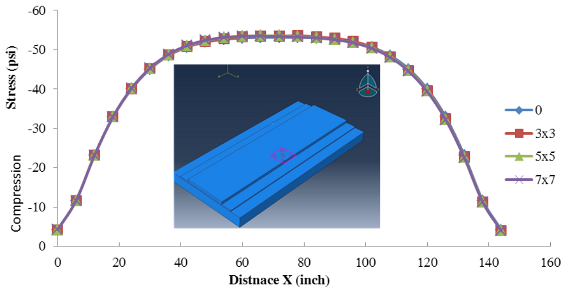
Figure 6.18 Distribution of S11 for changed friction areas placed halfway between two ends (FC-Area=1 and FC-Rest of the Pavement=20)
