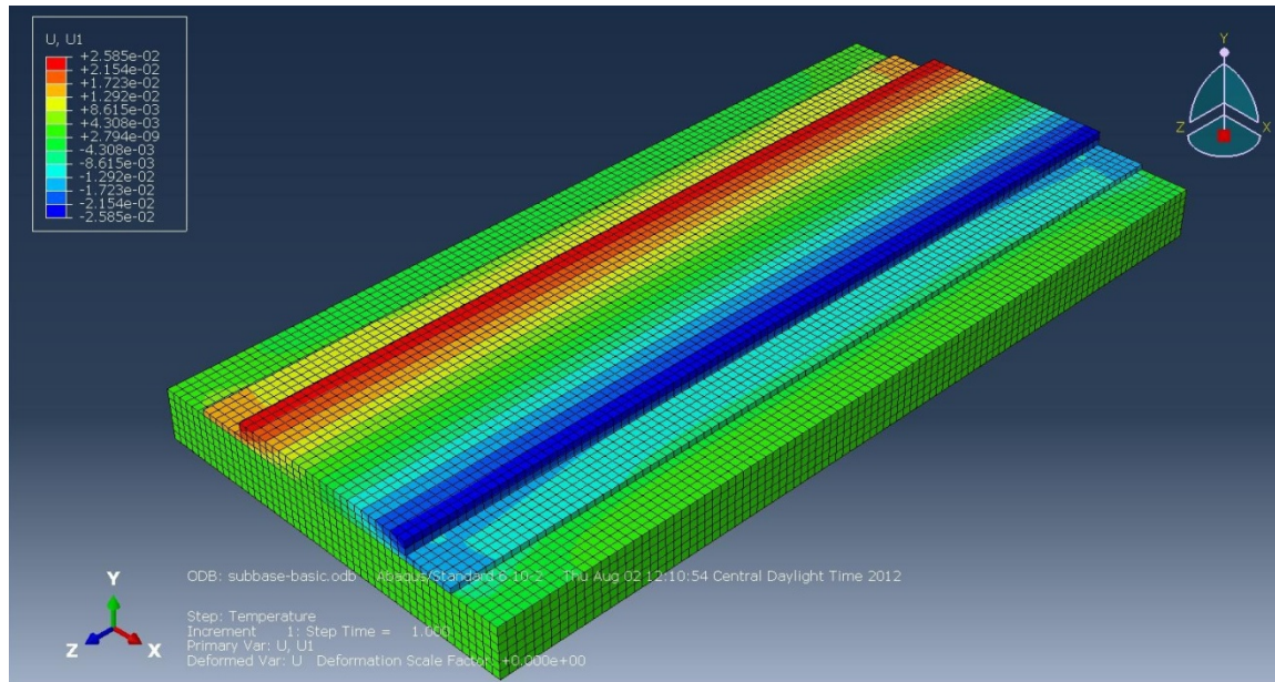
Figure 6.15 Color map of U1 in whole pavement model
