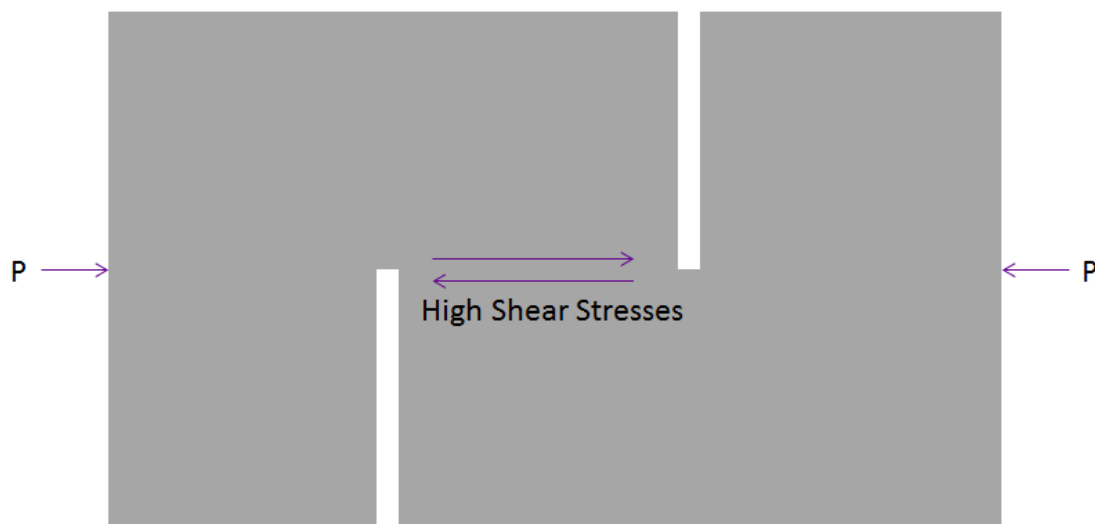
Figure 6.37 Schematic of Z-shaped concrete shear specimen
