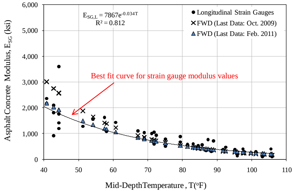
Figure 4-48 Back-calculated Modulus Values from Longitudinal Strain Gauges Versus Mid-Depth Temperature (on Linear Scale)
