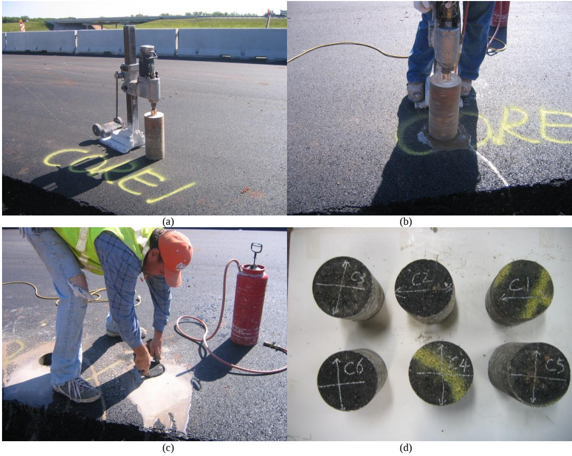
Figure 3-72 Extraction of Cores
