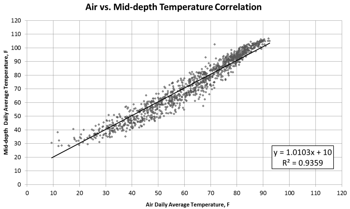
Figure 4-11 Air and Mid-depth Temperature Correlation
