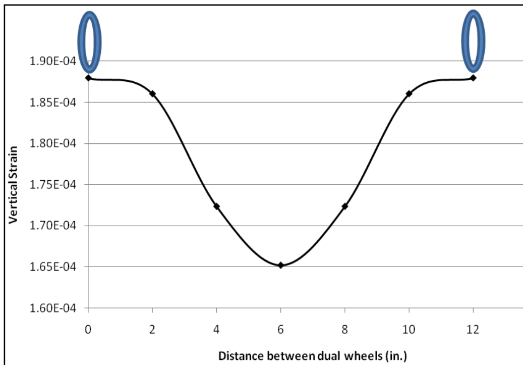
Figure 6-5 Vertical Strain Distribution for Dual Wheels of Tandem Axles
