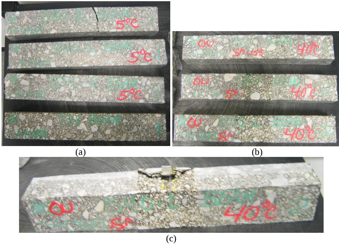
Figure 7-7 Four-Point Fatigue Beams (a) Tested at 5°C, (b) Tested at 40°C, and (c) Target Pulled Out of Beam at 40°C
