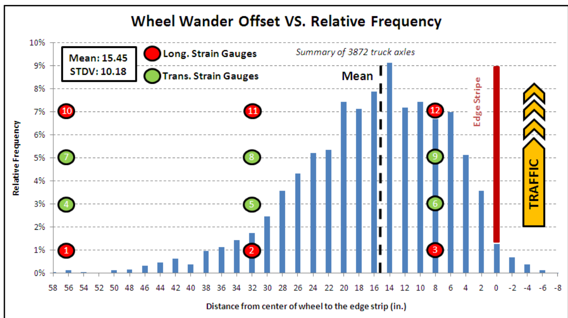
Figure 4-14 Statistical Distribution of Wheel Wander Data
