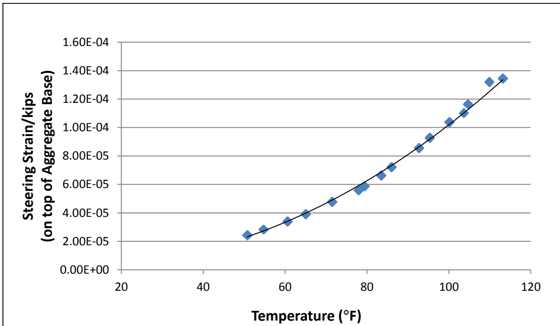
Figure 6-6 Vertical Strain-Temperature Correlation for Steering Axle
