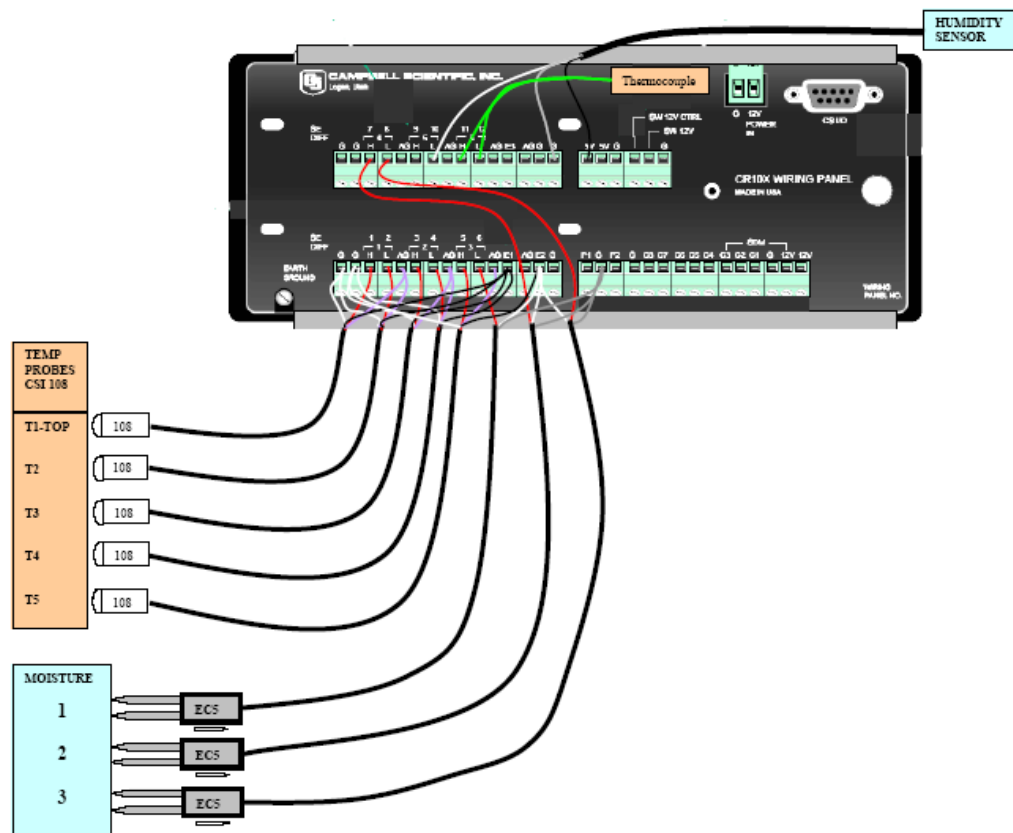
Figure 3-43 CR 10-X Wiring Diagram (Timm, 2007b)
