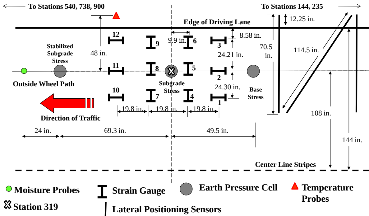
Figure 3-34 Instrumentation layout
