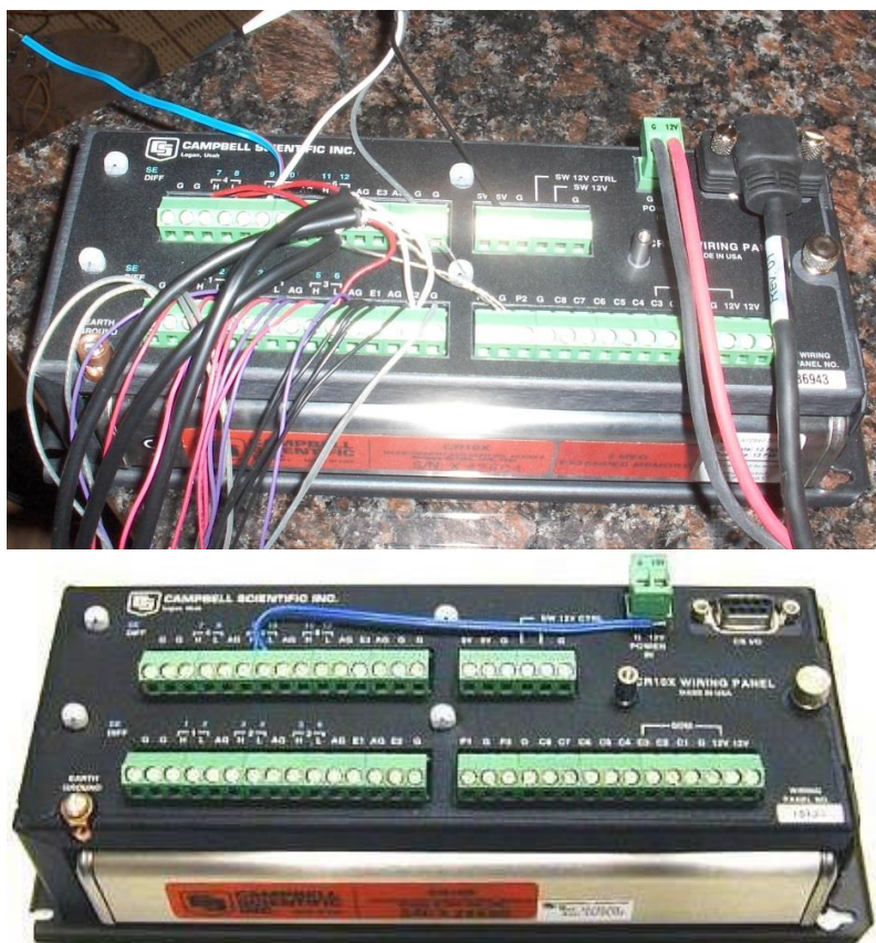
Figure 3-41 Campbell Scientific CR 10-X Environmental Data Acquisition System
