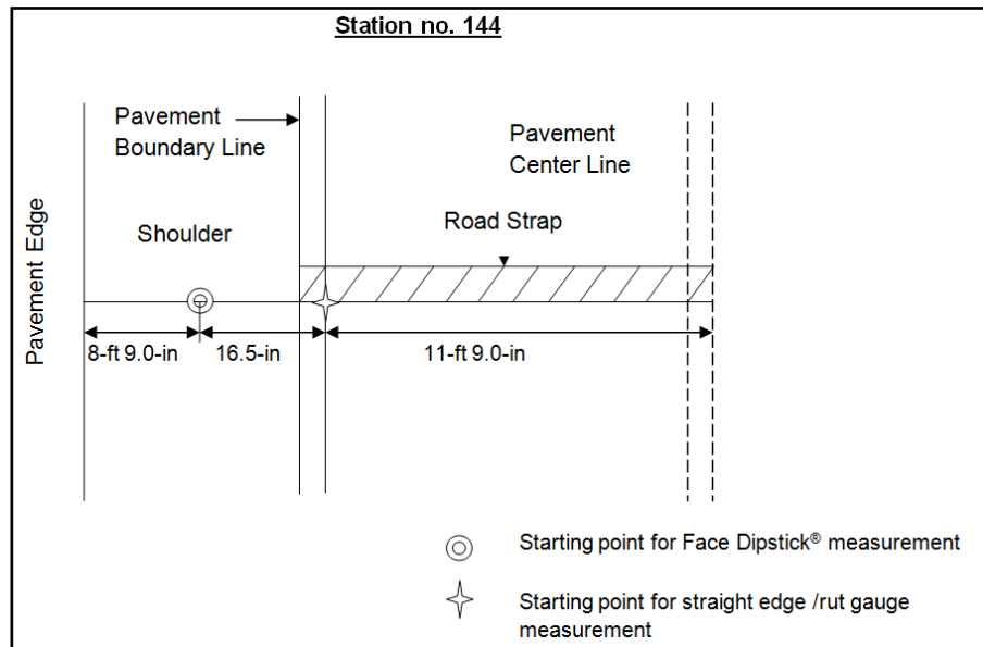
Figure 4-15 Rough Sketch of Pavement Section at Station 144
