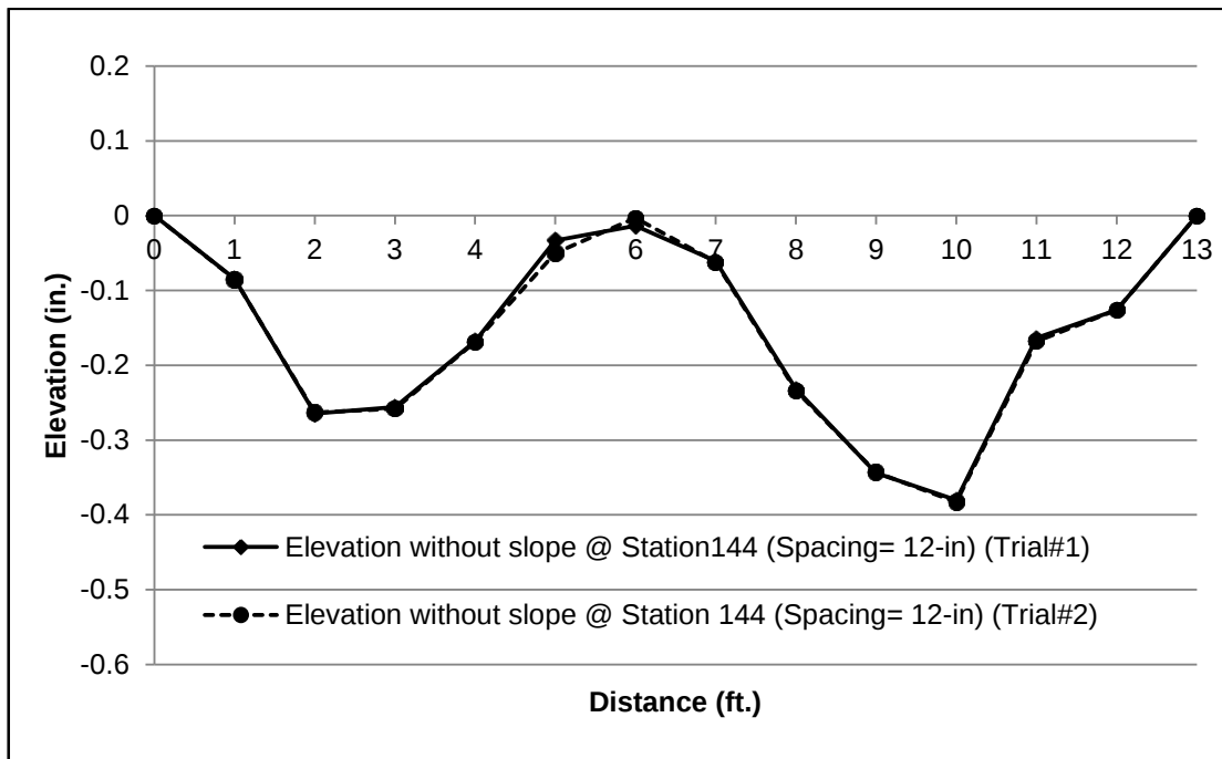
Figure 4-27 Pavement Profile without Slope at Station 144 (Moonfoot Spacing = 12-in.)
