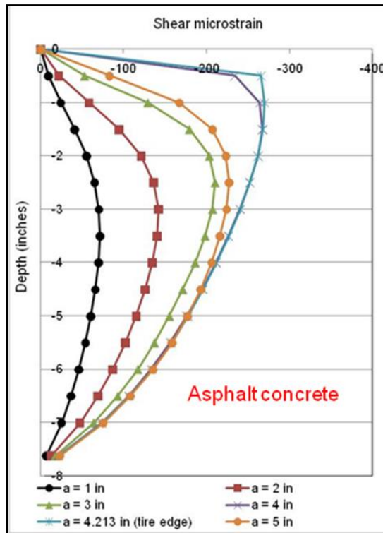
Figure 6-10 Typical Shear Strain Distribution in the HMA layer of the Test Section ( a = Distance from the Center of a Wheel Load)
