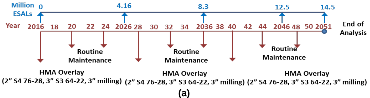
Figure 58 Two Suggested Rehabilitation Strategies, Alternatives a and b, for Flexible Pavements with 60 \leq \text{Structural Index} \leq 80
