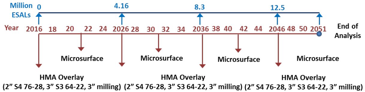
(III) Figure 66 Cost-effective Time-based Rehabilitation Strategies for Composite Pavements Sections with (I) Structural Index > 80, (II) 60 \leq Structural Index \leq 80 , (III) Structural Index < 60
