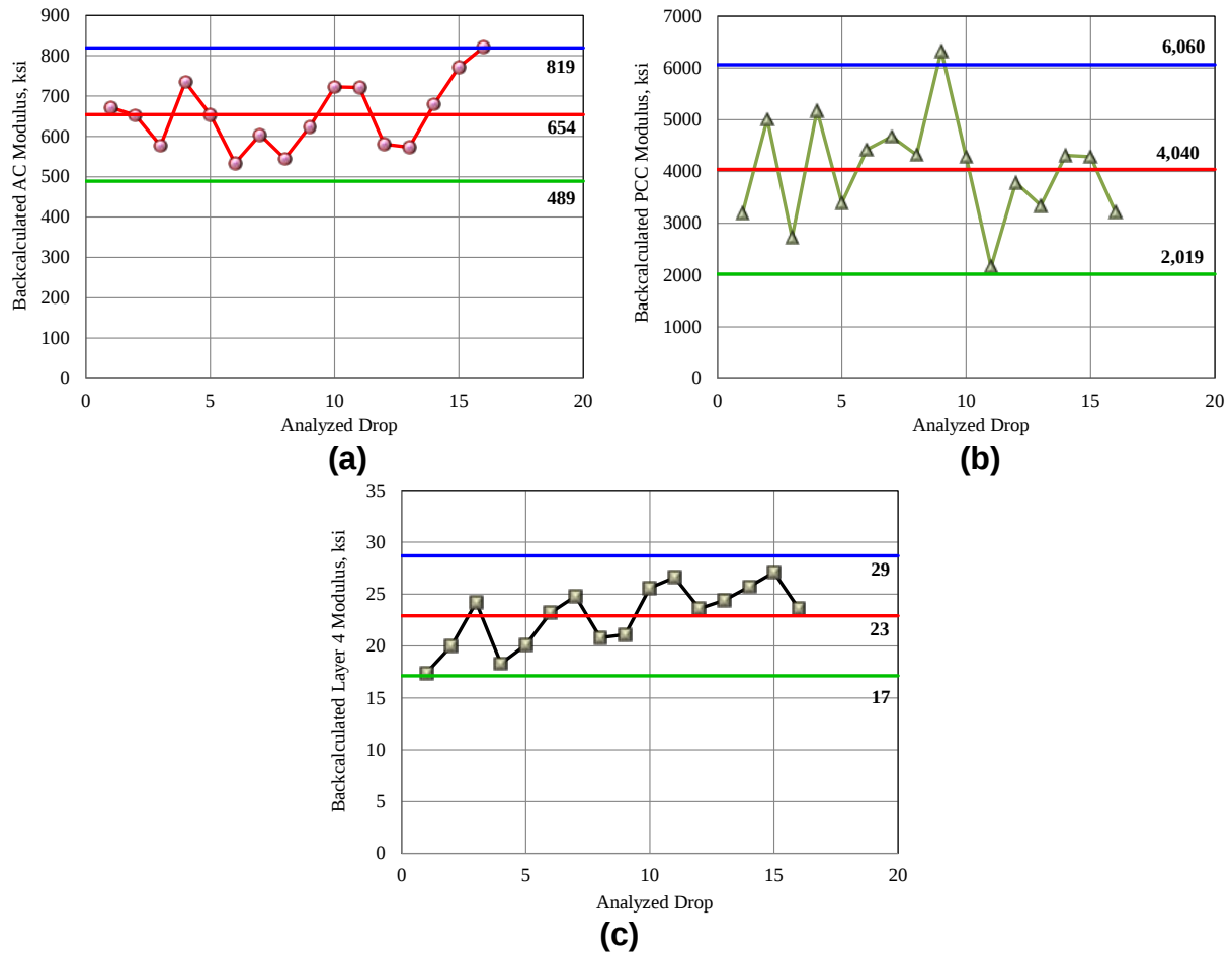
Figure 182 2010 Backcalculated (a) AC Layer, (b) Layer 2, and (c) Layer 3 Moduli for Control Section 25-46 MP 0, Direction 5.
