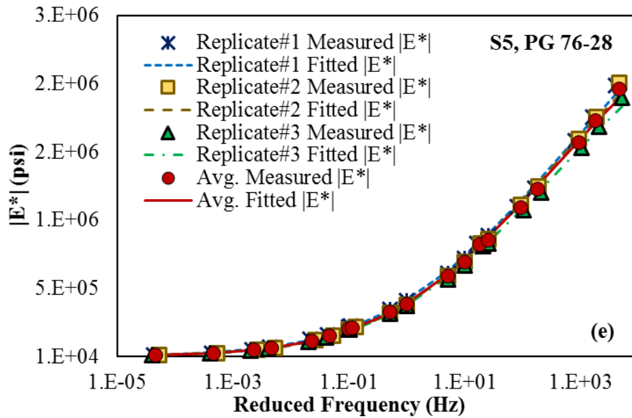
Figure 27 Dynamic Modulus Mastercurve for S5 PG 76-28 Specimens in Arithmetic Scale
