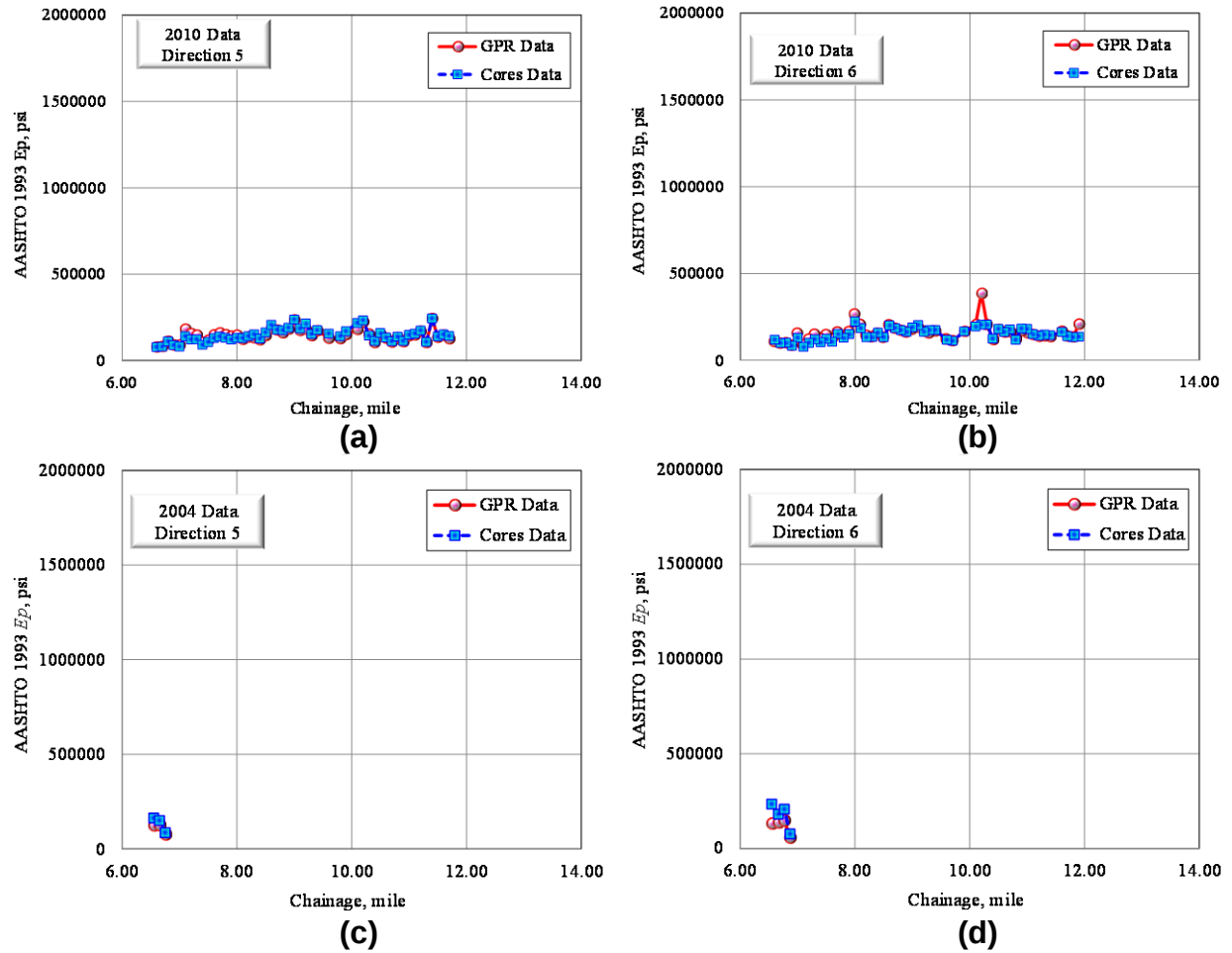
Figure 102 GPR and Core AASHTO 1993 Verified E_p Values Versus Distance for (a) 2010 Data in Direction 5, (b) 2010 Data in Direction 6, (c) 2004 Data in Direction 5, and (d) 2004 Data in Direction 6 for Control Section 55-68.
