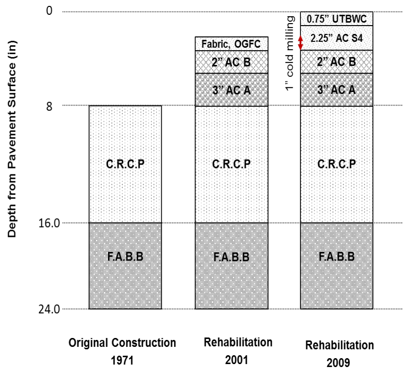
Figure 13 Structure Profile of Control Section 50-32 MP 0.0-6.54
