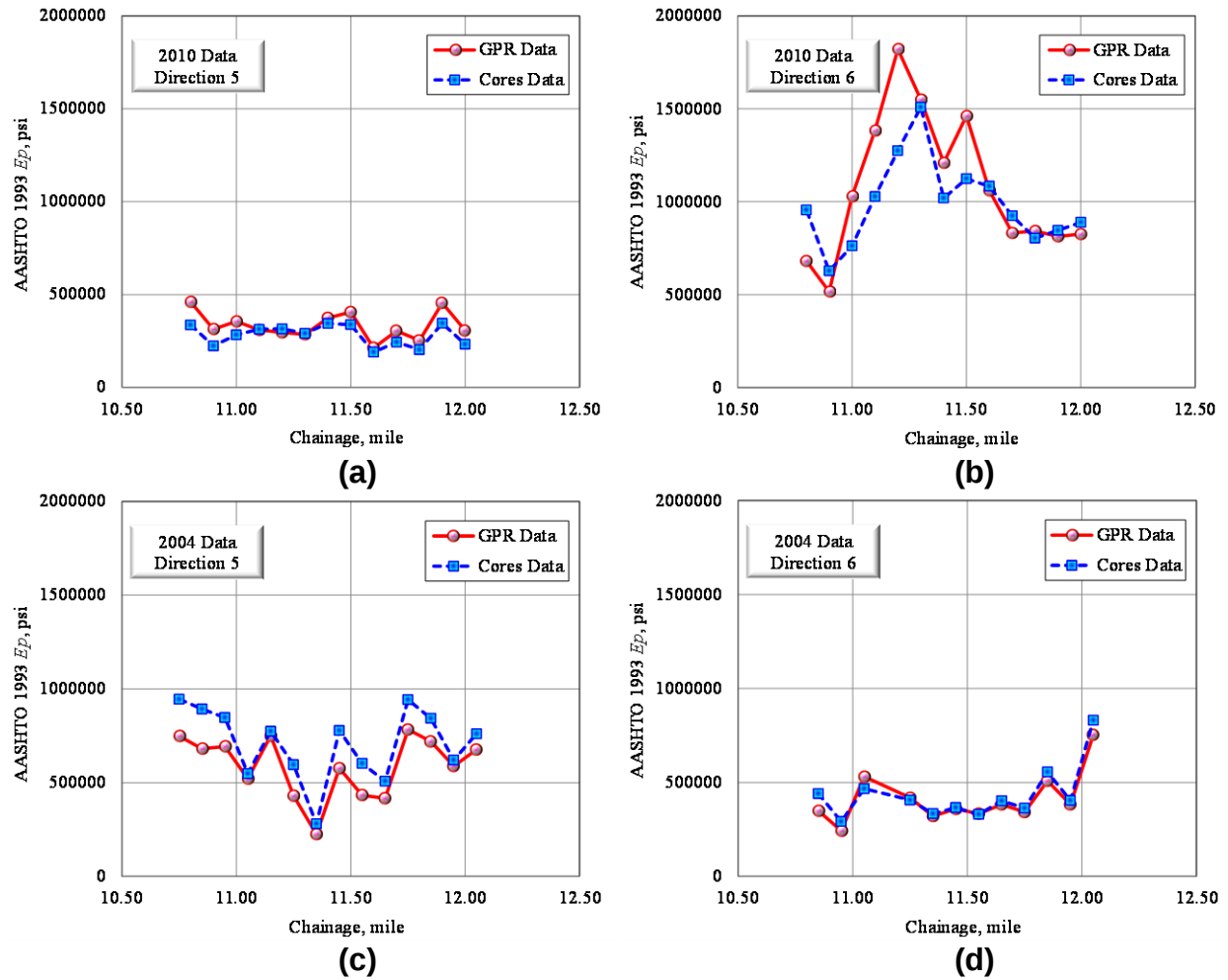
Figure 100 GPR and Core AASHTO 1993 Verified E_p Values Versus Distance for (a) 2010 Data in Direction 5, (b) 2010 Data in Direction 6, (c) 2004 Data in Direction 5, and (d) 2004 Data in Direction 6 for Control Section 44-05.
