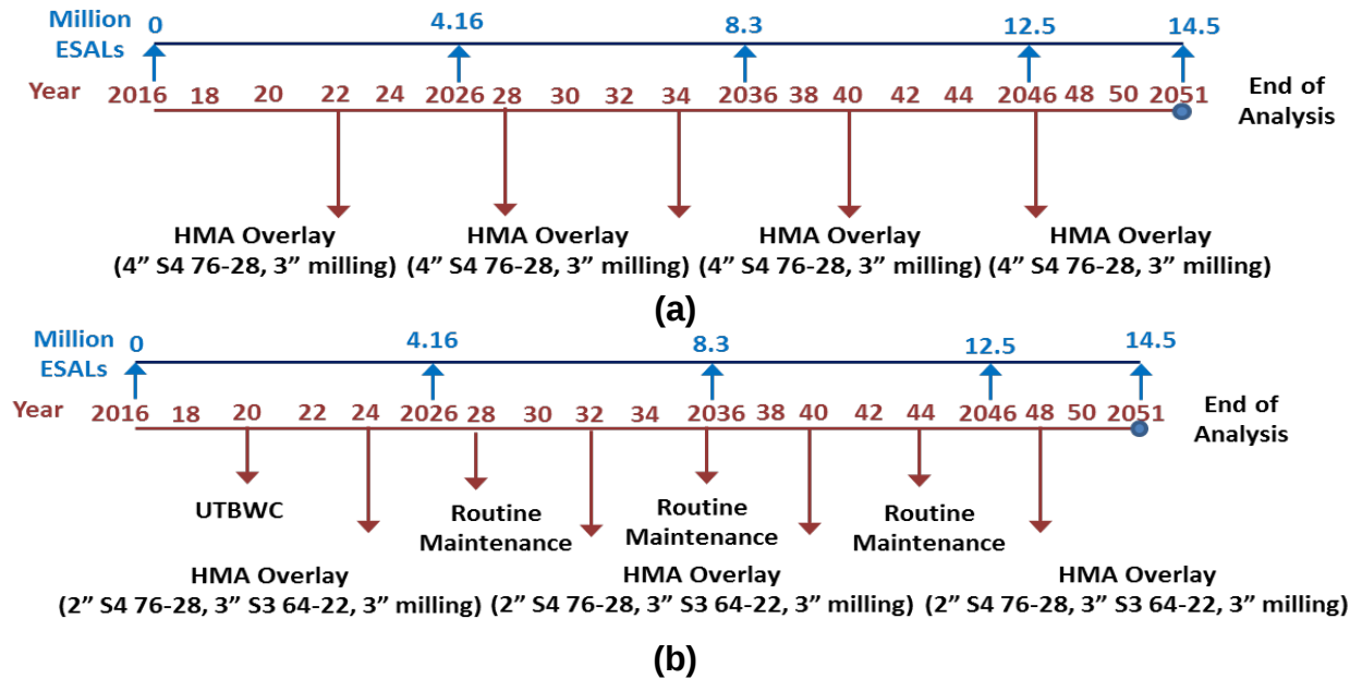
Figure 60 Two Suggested Rehabilitation Strategies for Composite Pavements with Structural index>80
