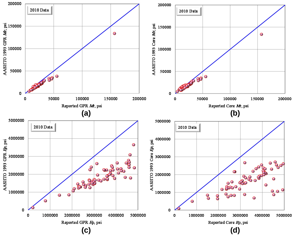
Figure 107 Comparison of 2010 Reported and AASHTO 1993 Verified Values of (a) M_r Based on GPR and (b) M_r Based on Core, (c) E_p Based on GPR and (d) E_p Based on Core for Control Section 42-30.
