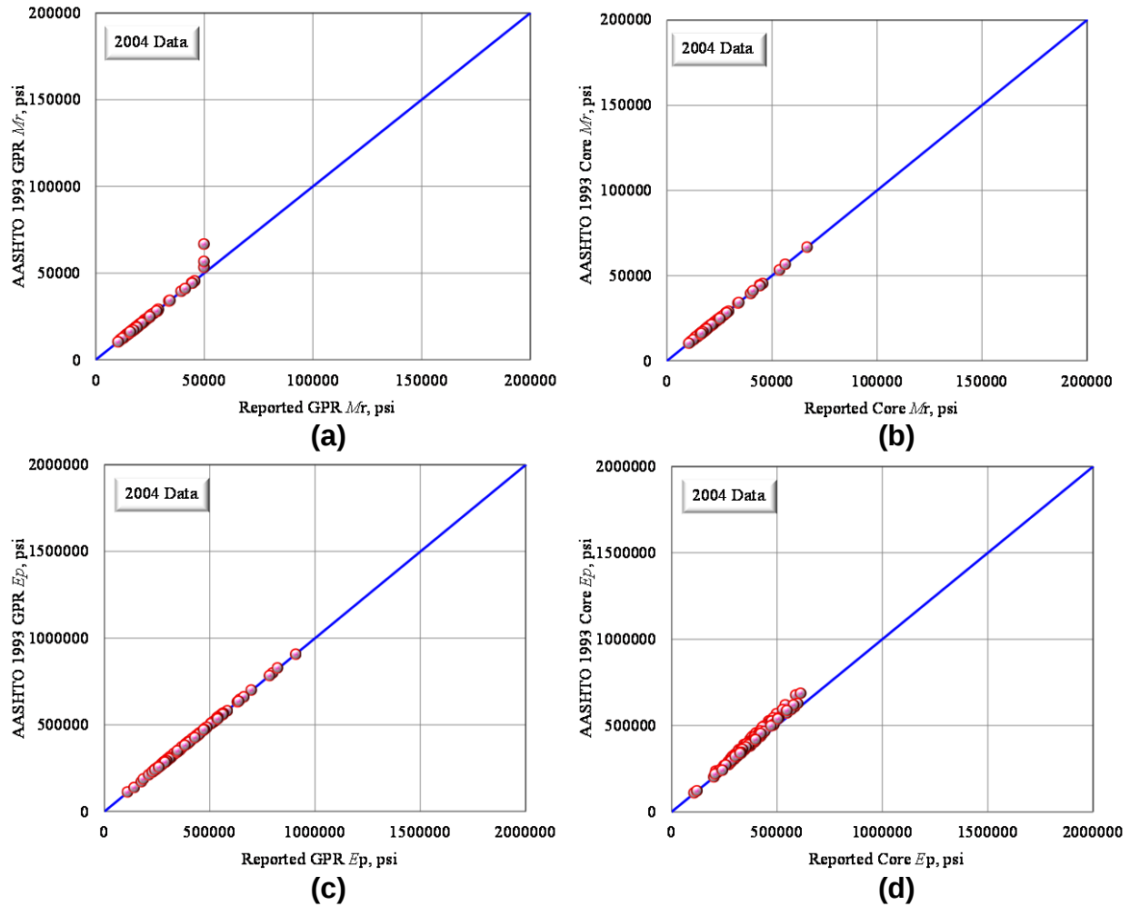
Figure 84 Comparison of 2004 Reported and AASHTO 1993 Verified Values of (a) M_r Based on GPR and (b) M_r Based on Core, (c) E_p Based on GPR and (d) E_p Based on Core for Control Section 09-05.
