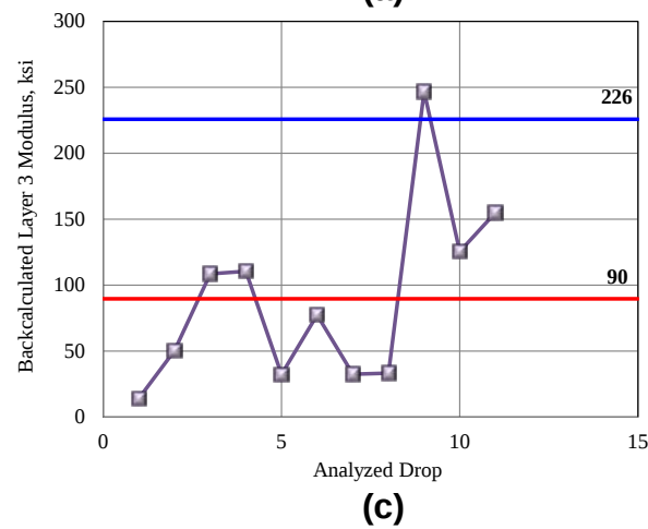
Figure 161 2010 Backcalculated (a) AC Layer, (b) Layer 2, (c) Layer 3 and (d) Layer 4 Moduli for Control Section 68-22, Direction 6.
