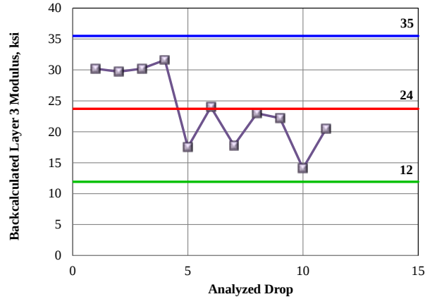
Figure 173 2010 Backcalculated (a) AC Layer, (b) Layer 2, and (c) Layer 3 Moduli for Control Section 44-05 MP 13.85, Direction 6.
