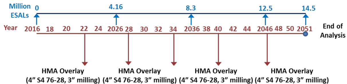
(III) Figure 65 Cost-effective Time-based Rehabilitation Strategies for Flexible Pavements Sections with (I) Structural Index > 80, (II) 60 \leq Structural Index \leq 80 , (III) Structural Index < 60
