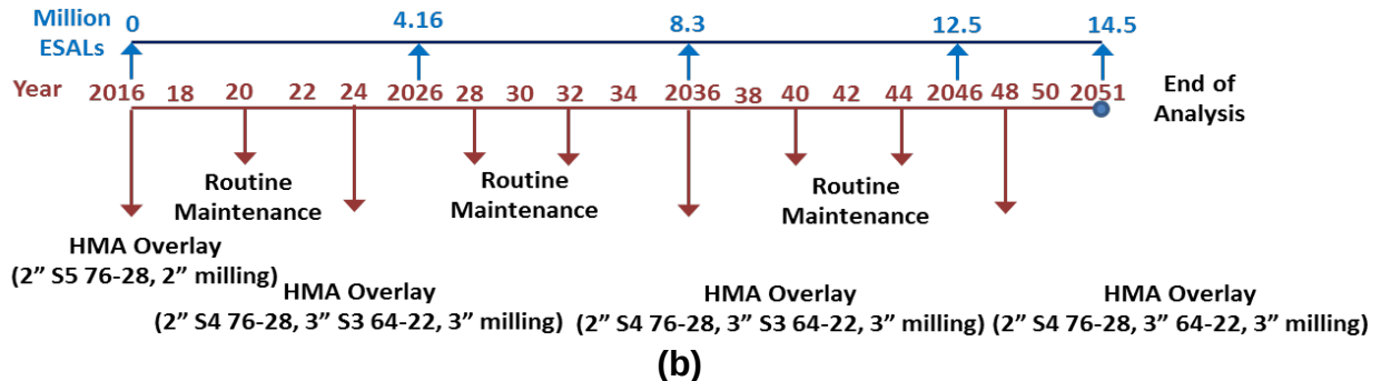
Figure 58 Two Suggested Rehabilitation Strategies, Alternatives a and b, for Flexible Pavements with 60 \leq \text{Structural Index} \leq 80
