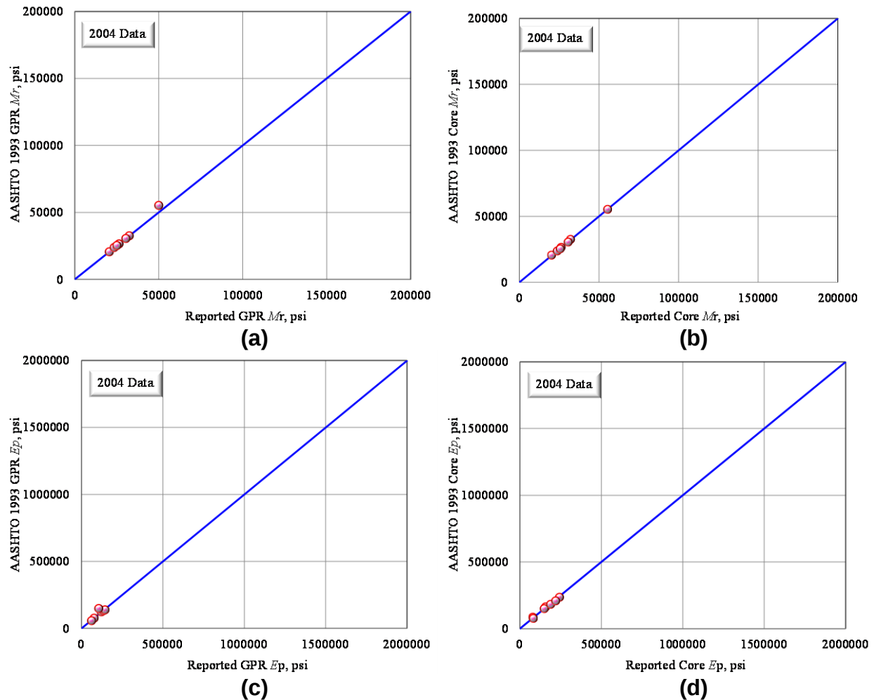
Figure 86 Comparison of 2004 Reported and AASHTO 1993 Verified Values of (a) M_r Based on GPR and (b) M_r Based on Core, (c) E_p Based on GPR and (d) E_p Based on Core for Control Section 55-68.
