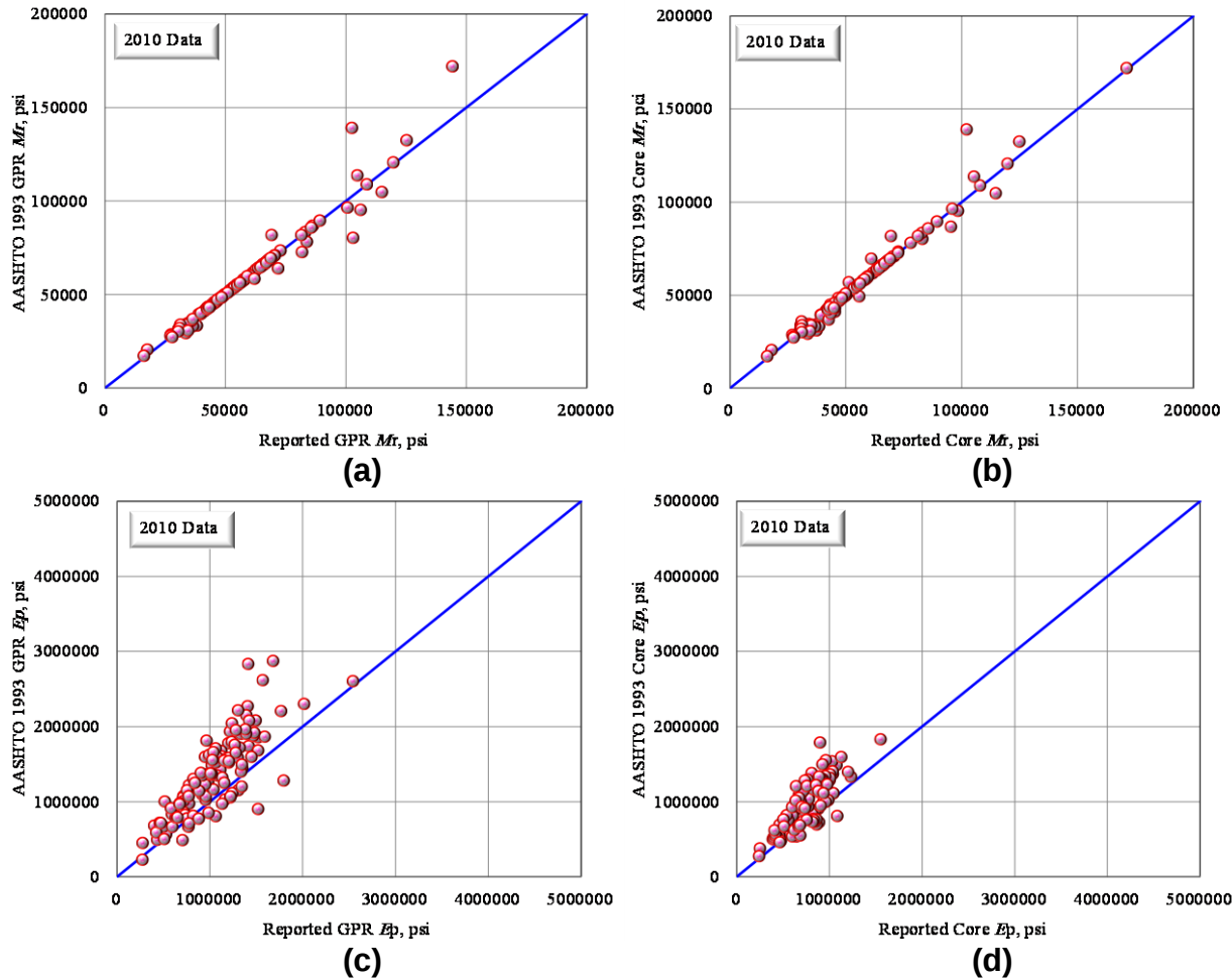
Figure 112 Comparison of 2010 reported and AASHTO 1993 Verified Values of (a) M_r Based on GPR and (b) M_r Based on Core, (c) E_p Based on GPR and (d) E_p Based on Core for Control Section 50-32.
