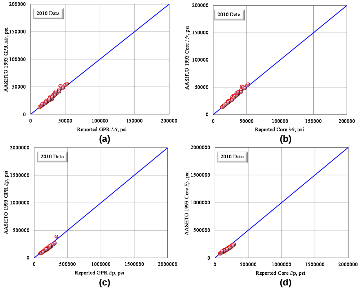
Figure 85 Comparison of 2010 Reported and AASHTO 1993 Verified Values of (a) M_r Based on GPR and (b) M_r Based on Core, (c) E_p Based on GPR and (d) E_p Based on Core for Control Section 55-68.
