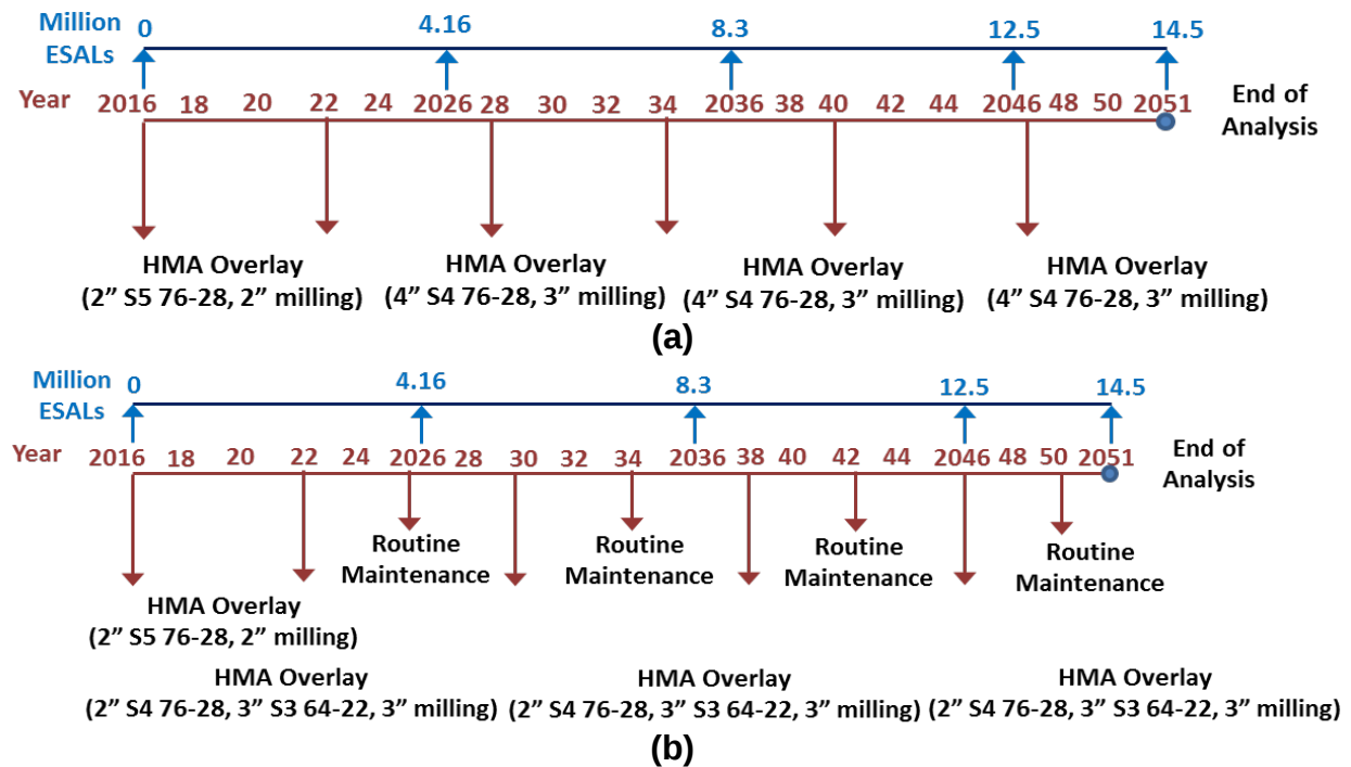
Figure 61 Two Suggested Rehabilitation Strategies for Composite Pavements with 60 \leq Structural Index \leq 80
