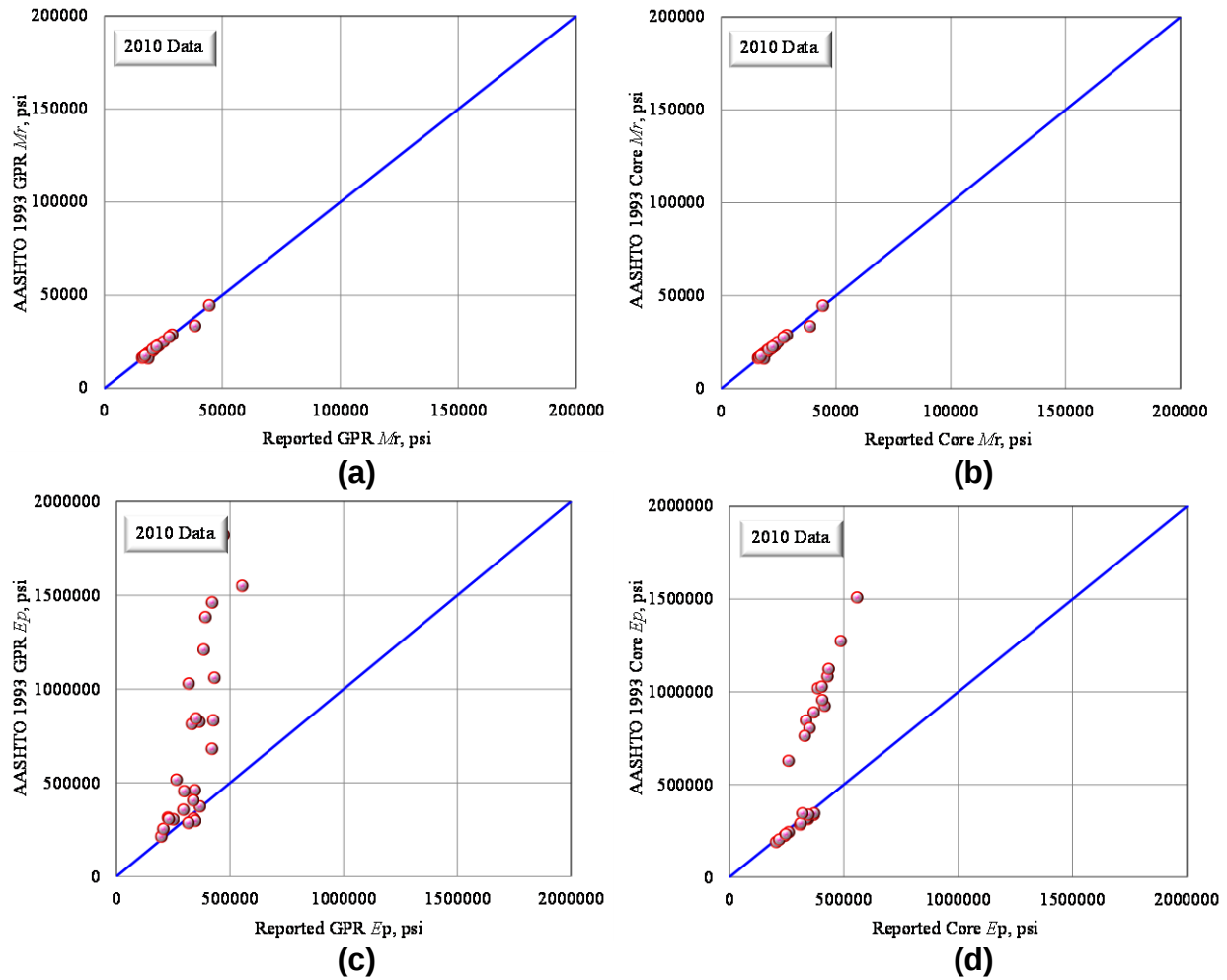
Figure 81 Comparison of 2010 Reported and AASHTO 1993 Verified Values of (a) M_r Based on GPR and (b) M_r Based on Core, (c) E_p Based on GPR and (d) E_p based on Core for Control Section 44-05.
