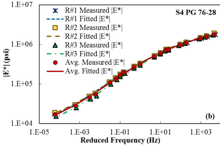
Figure 19 Dynamic Modulus Master-curve for S4 PG 76-28 Specimens in Logarithmic Scale
