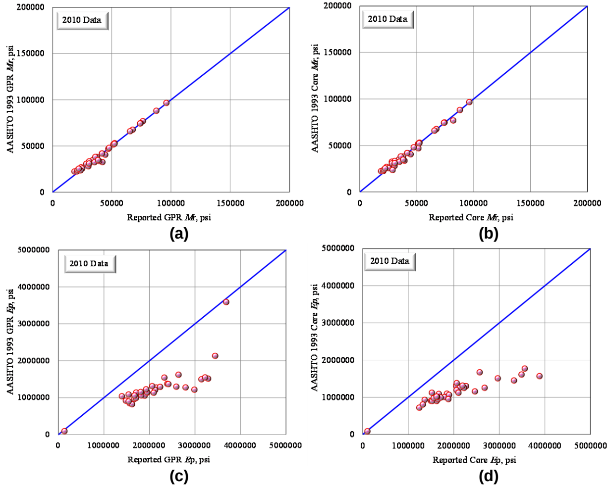
Figure 115 Comparison of 2010 reported and AASHTO 1993 Verified Values of (a) M_r Based on GPR and (b) M_r Based on Core, (c) E_p Based on GPR and (d) E_p Based on Core for Control Section 72-09.
