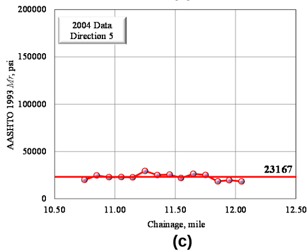
Figure 93 AASHTO 1993 Verified M_r Values Versus Distance for (a) 2010 data in Direction 5, (b) 2010 Data in Direction 6, (c) 2004 Data in Direction 5, and (d) 2004 Data in Direction 6 for Control Section 44-05.
