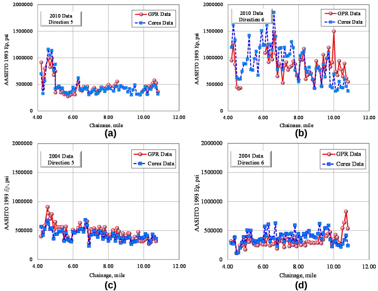
Figure 101 GPR and Core AASHTO 1993 Verified E_p Values Versus Distance for (a) 2010 Data in Direction 5, (b) 2010 Data in Direction 6, (c) 2004 Data in Direction 5, and (d) 2004 Data in Direction 6 for Control Section 09-05.
