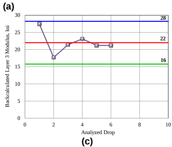
Figure 172 2010 Backcalculated (a) AC Layer, (b) Layer 2, and (c) Layer 3 Moduli for Control Section 44-05 MP 13.85, Direction 5.
