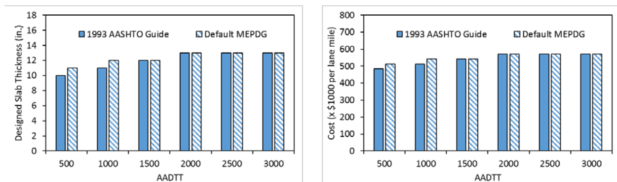
Figure 6.5 Comparison Analysis for CRCP over UAB
