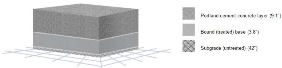
Figure 5.3 Pavement structure of LTPP Segment 40-4157
