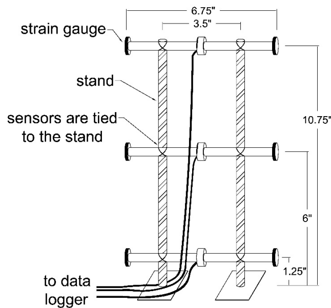
Figure 7.3 A strain gage tied to the steel bars
