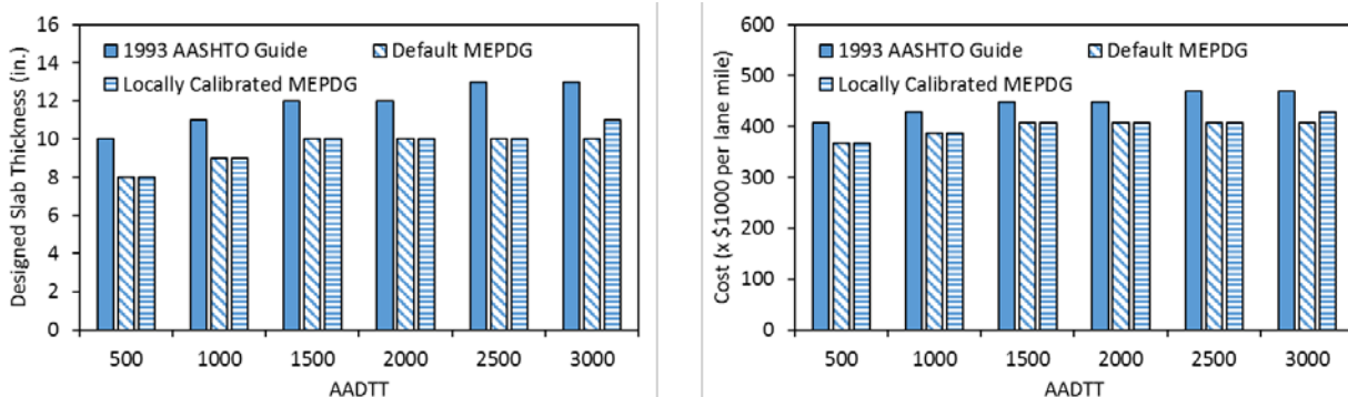
Figure 6.3 Comparison Analysis for JPCP over AC Base
