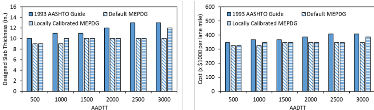
Figure 6.2 Comparison Analysis for JPCP over UAB
