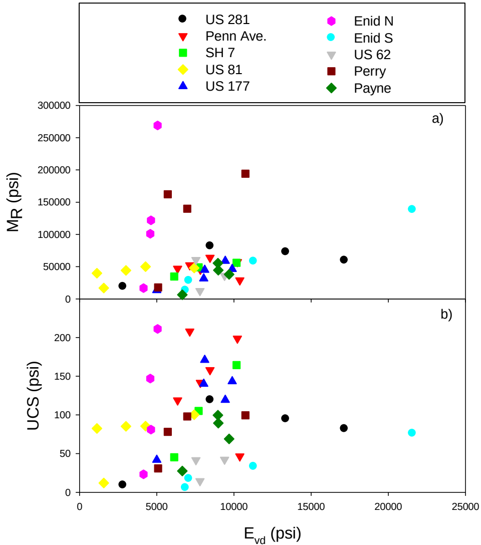
Figure 38: Comparison of Results of PFWD Field Tests with Laboratory Measurements of M_R and UCS at Similar Curing Times
