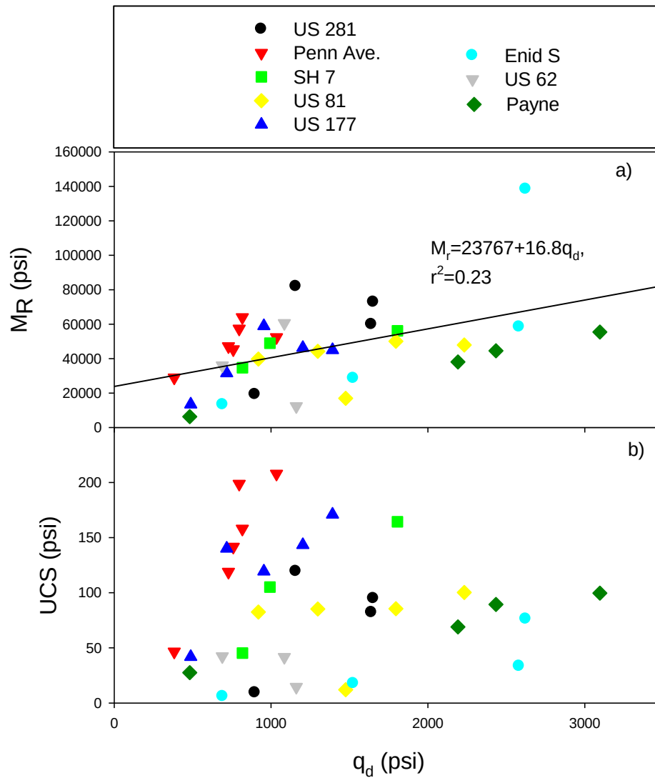
Figure 40: Comparison of Results of PANDA Penetrometer Field Tests with Laboratory Measurements of M_R and UCS at Similar Curing Times with Enid North and Perry Site Data Removed
