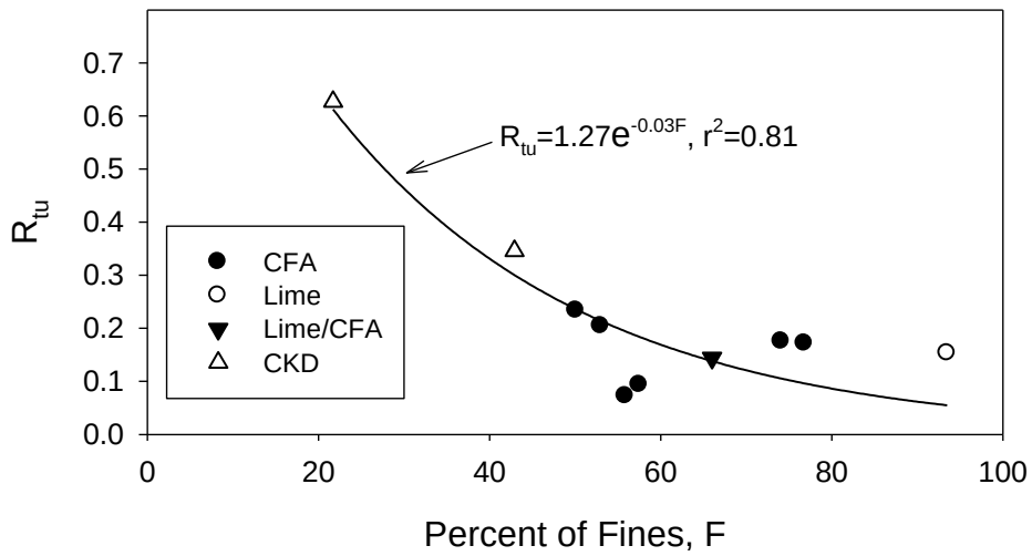
Figure 17: Power Model Parameter R_{tu} for UCS-Time Relationship versus Percent of Fines
