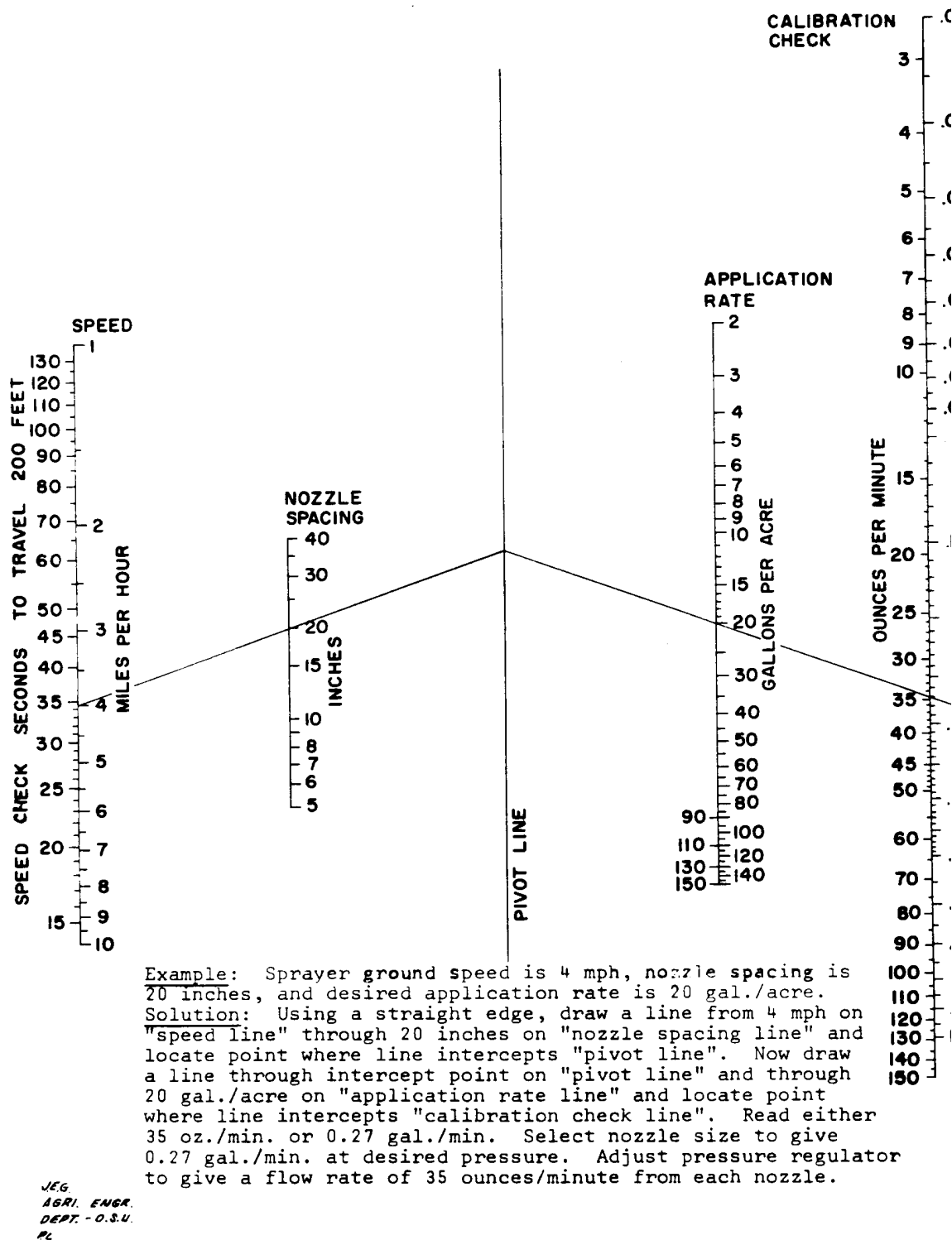
Figure 11.2. Nomograph for Calibrating Boom-Type Sprayers.
