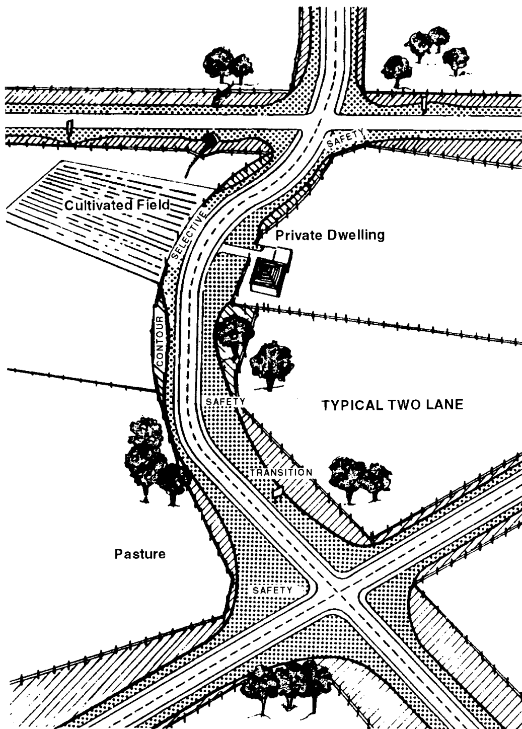
Figure 2.10. Safety, Contour, Selective And Transition Mowing On Rural Two-Lane Facilities.
