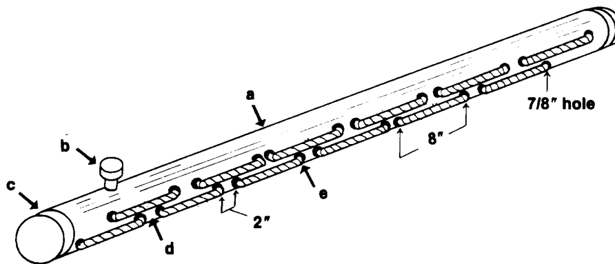
Figure 11.3. Typical ropewick applicator showing the components assembled. Materials are (a) 3-inch PVC pipe; (b) capped fill spout – PVC; (c) end cap – PVC; (d) wick of \frac{1}{2} -inch diameter soft braided nylon marine rope; (e) rubber bushing (for \frac{1}{2} -inch rope) with compression cap.
