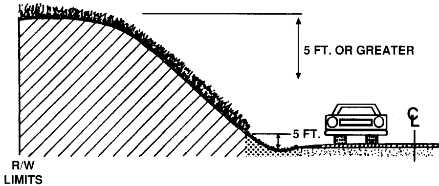
Figure 2.4. Normal Mowing Limits for a Ditch With Depth of Five Feet or Greater.
