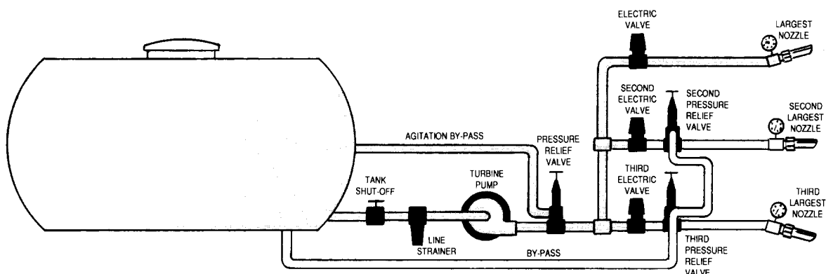
Figure 10.17. A System Using Three Different Boom Buster Tips Allows For Flexibility.
