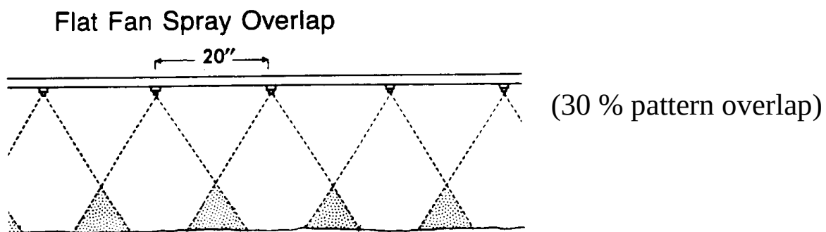
Figure 10.11. Spray Patterns From Adjacent Nozzles Must Be Overlapped To Produce Uniform Spray Coverage [Above].
