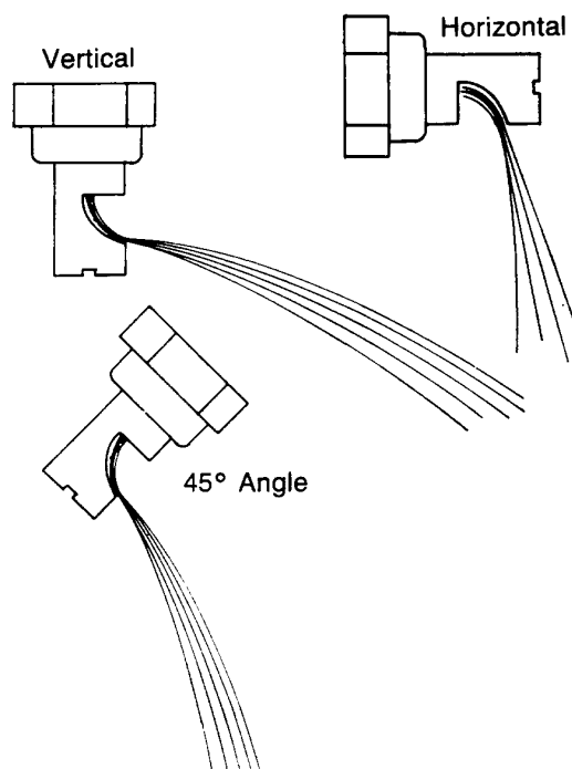
Figure 10.14. Flooding Nozzle Operating Positions of Vertical, Horizontal and 45 Degree Angle.
