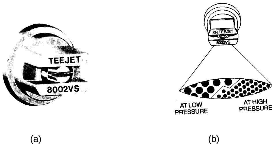
Figure 10.10. A Regular Flat-Fan Spray Tip (a) Produces A Flat Pattern Tapered At The Edges (b) [Above].
