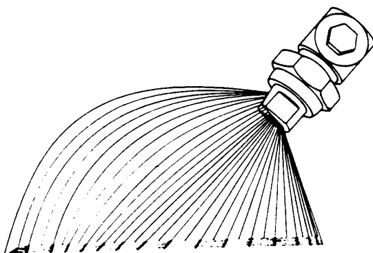
Figure 10.19. The Off-Center Nozzle Is Used For Making Boomless Broadcast Herbicide Applications.
