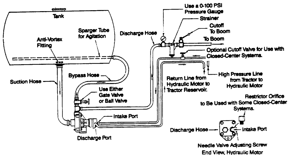
Figure 10.2. Basic Spraying System With Hydraulic Motor Driven Centrifugal Pump.
