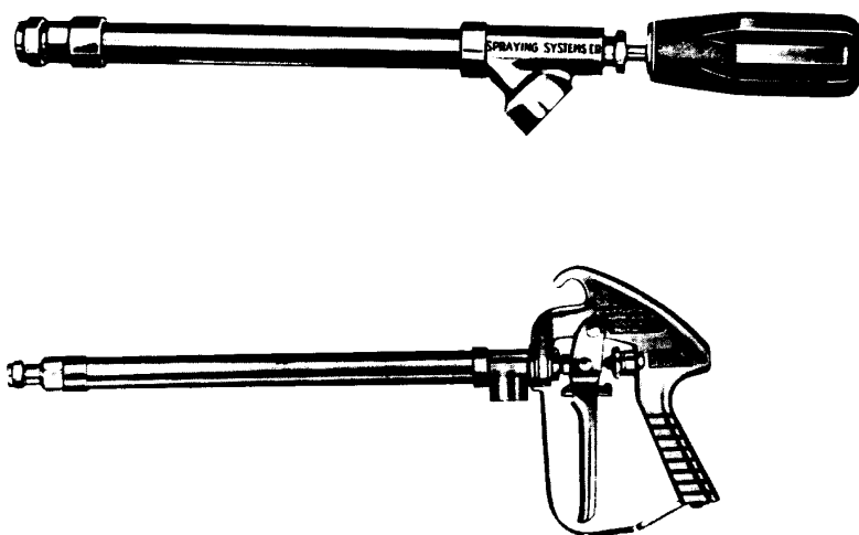
Figure 10.8. Commonly Used Hand Spray Guns For Applying High Volume Herbicide Treatments.
