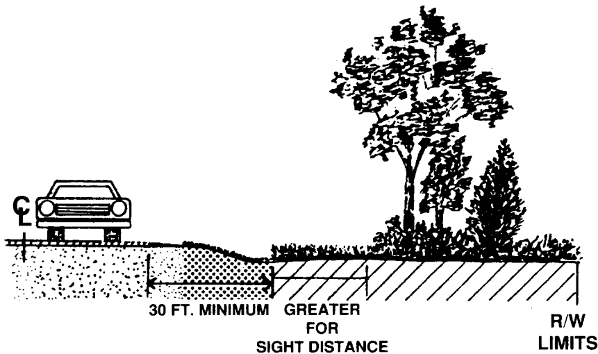
Figure 2.6. Mowing Limits On Flat Areas.
