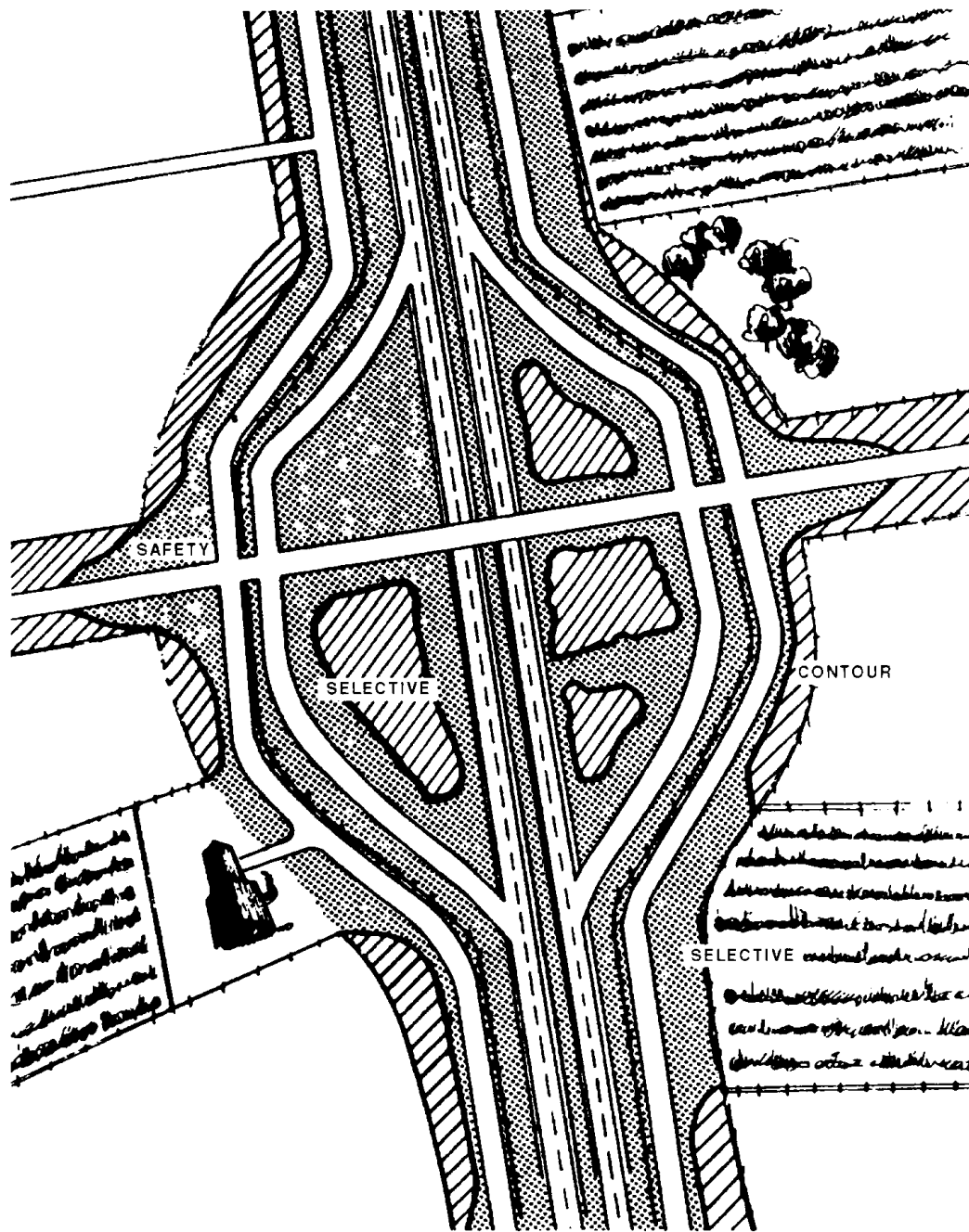
Figure 2.9. Safety, Selective And Contour Mowing At Multi-Lane Interchanges.
