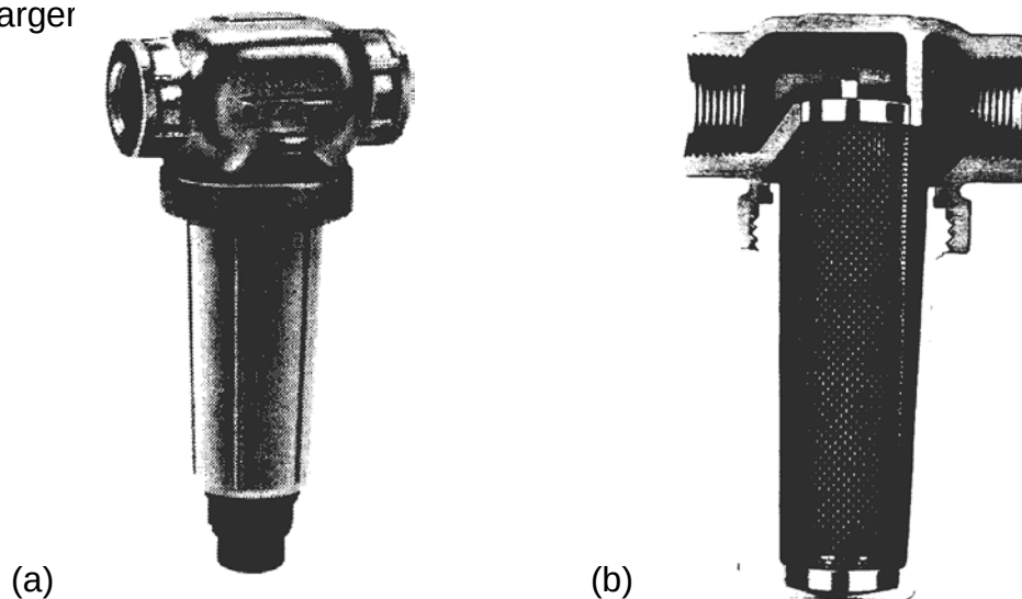
Figure 10.4. Spray System Strainer; (a) Exterior View and (b) Cut-Away View Showing Strainer Mesh.
