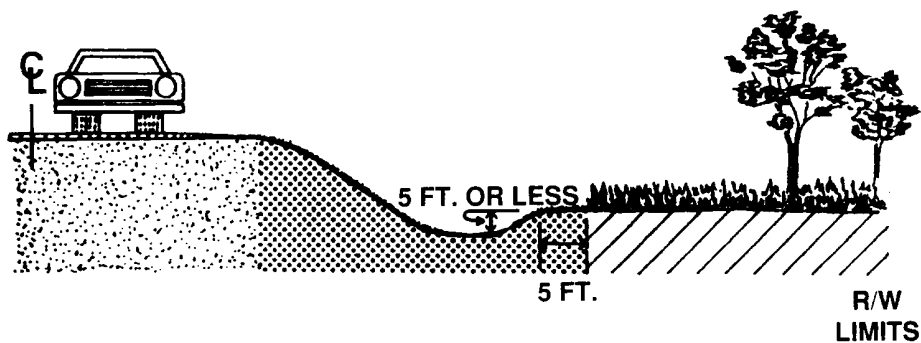
Figure 2.3. Normal Mowing Limits For A Ditch Less Than Five Feet Deep.
