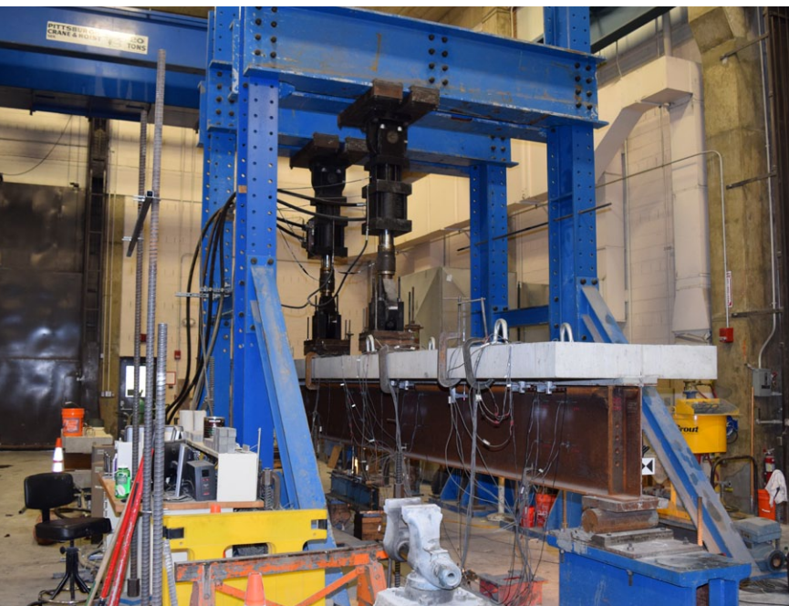
Testing bridge components at the Turner Fairbank Highway Research Center
