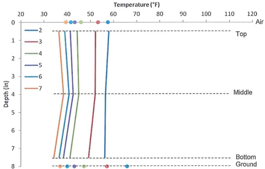
Figure 5. 53 November 30, 2011 no cure temperature differentials
