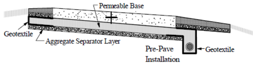
Figure 3.1 Typical cross-section of subsurface drainage system (FHWA 1994)
