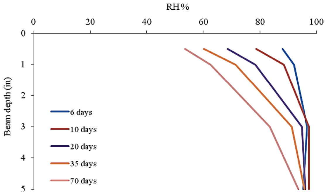
Figure 5.34 RH profiles for 6, 10, 20, 35 and 70 days after exposure for concrete beam C3-D
