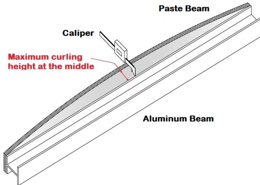
Figure 5.3 Measuring the curling height using a caliper
