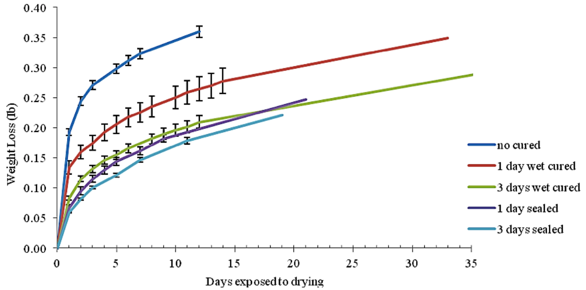
Figure 5.10 Weight loss vs. age of the paste specimen
