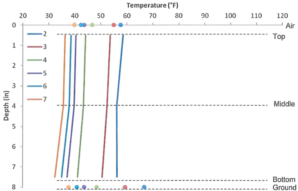
Figure 5. 57 November 30, 2011 single layer curing compound temperature differentials
