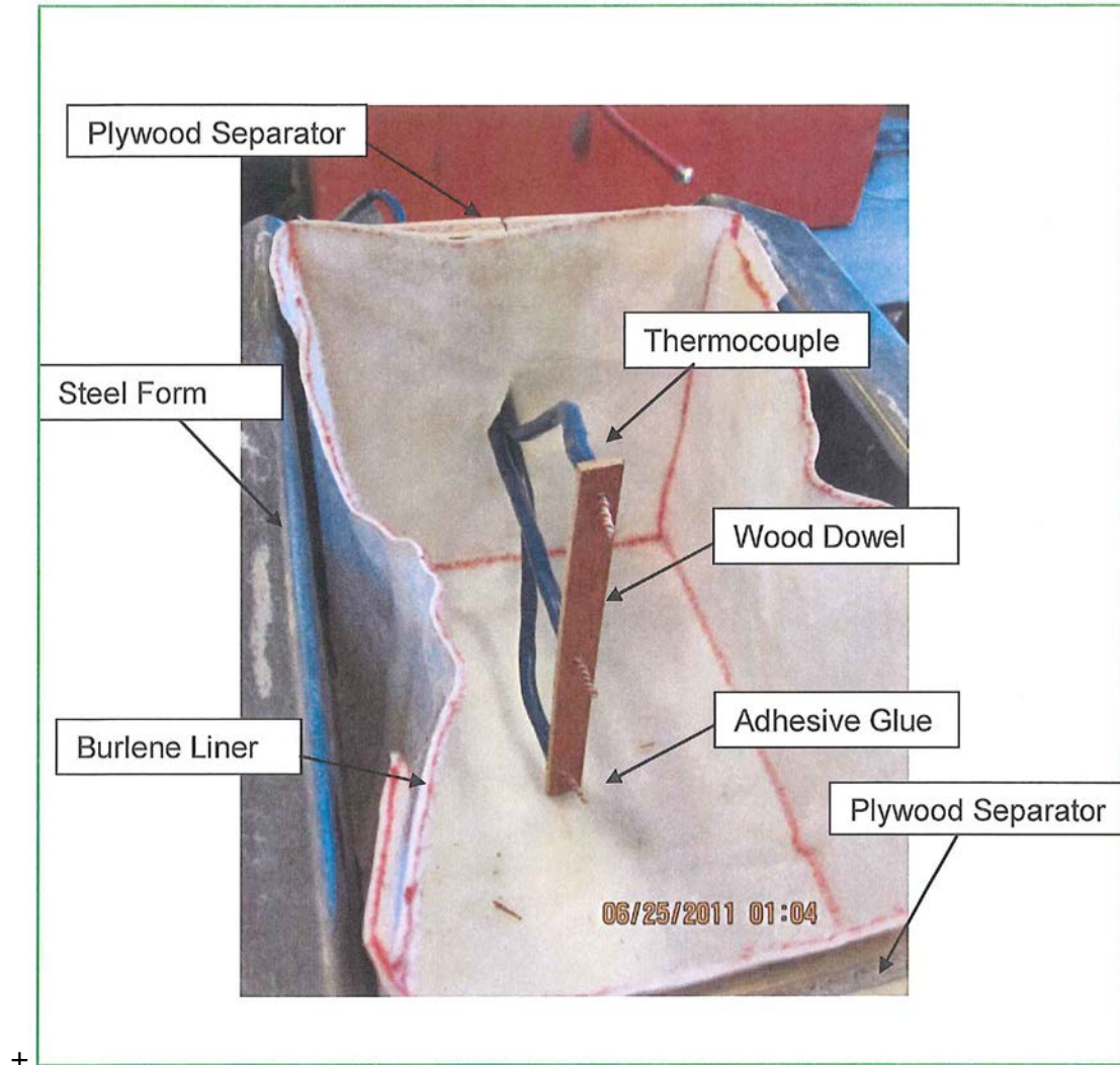
Figure 5.39 Assembled thermocouple, dowel, liner & form
