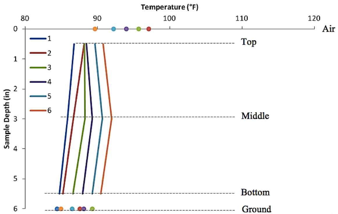
Figure 5.47 Six layers of dry burlap temperature gradients
