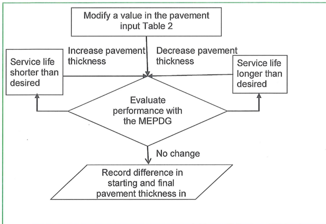
Figure 2.2 Flowchart showing the steps to find out the resulting change in the design thickness for a change of a given variable
