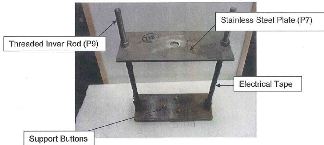
Figure 6.6 Assembled rigid frame with labels
