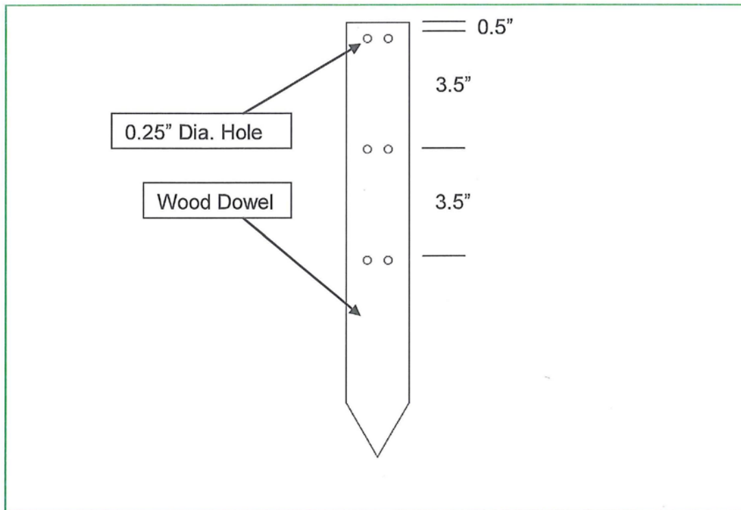
Figure 5.49 Wood dowel with dimensions
