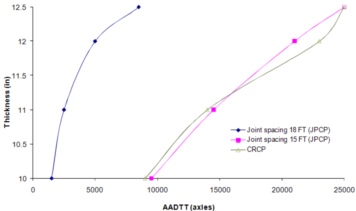
Figure 2.3 A plot of the required design thickness for JPCP and CRCP with different AADTTs.
