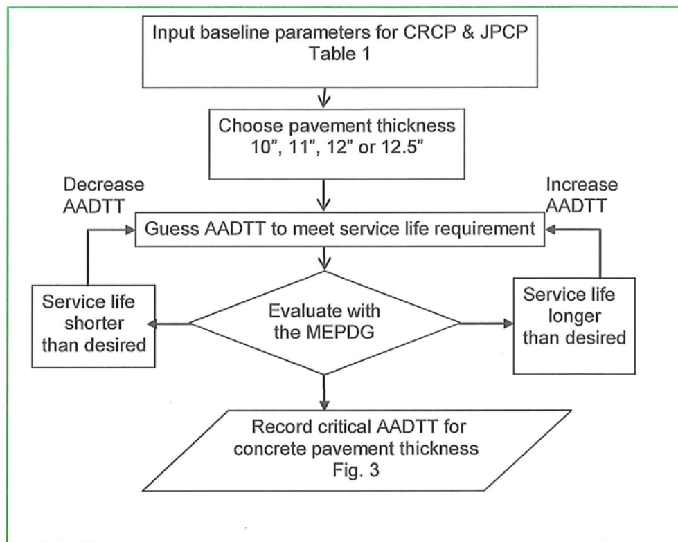
Figure 2.1 Flowchart showing the steps to find the critical AADTT for a typical pavement design.
