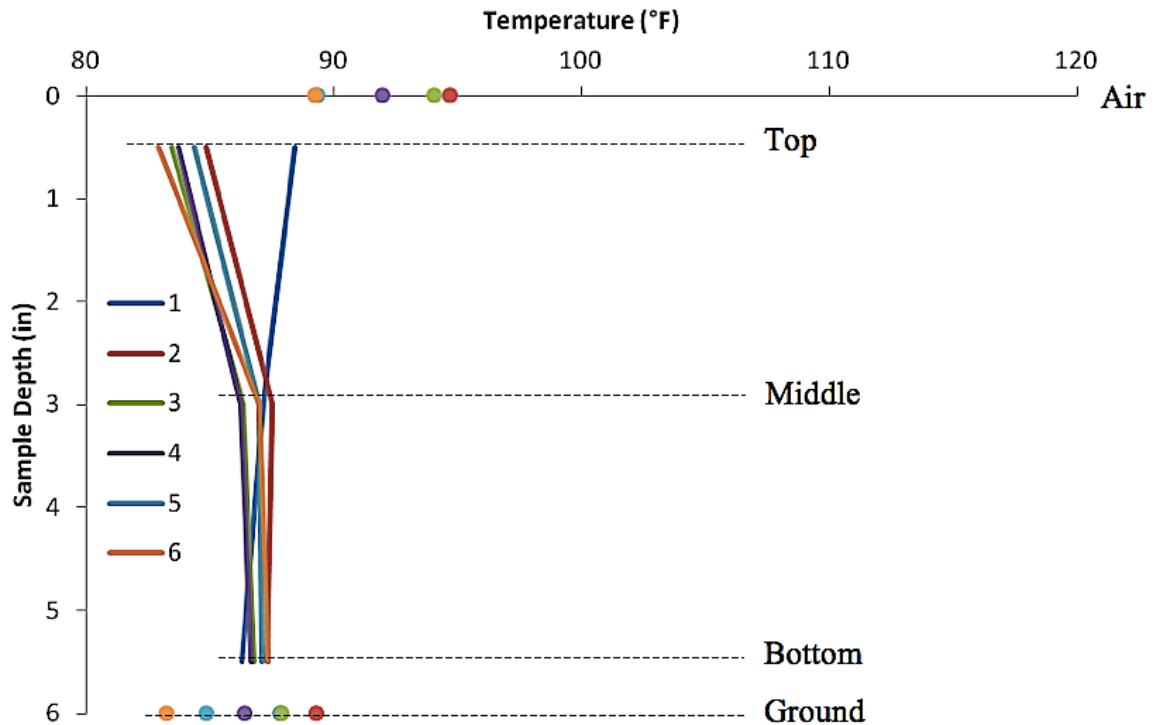
Figure 5.43 Two layers wet burlap temperature gradients
