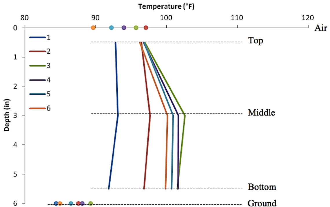
Figure 5.40 No-cure temperature gradients
