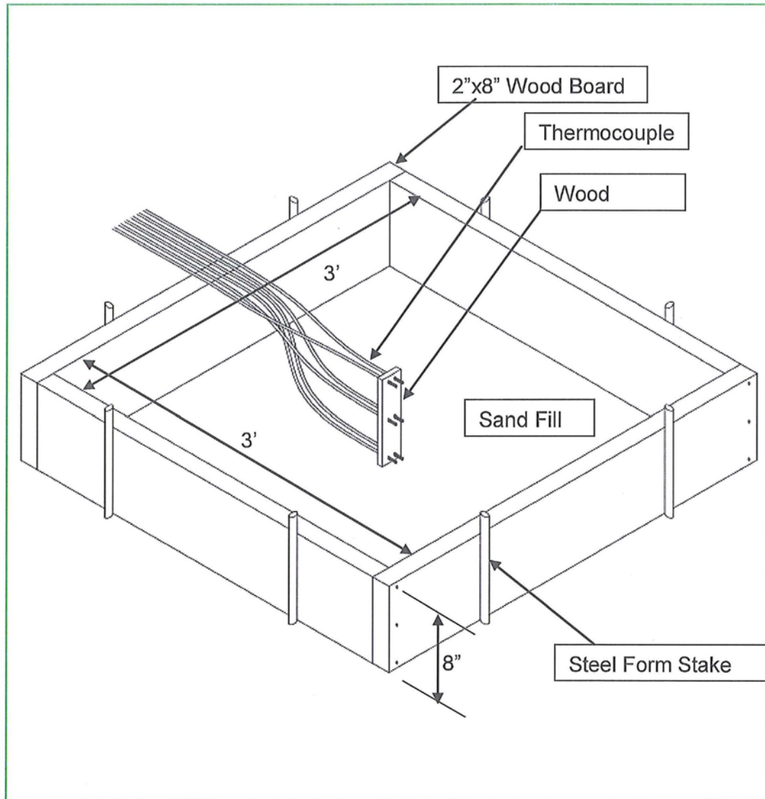
Figure 5.50 Assembled thermocouple, dowel, liner & form
