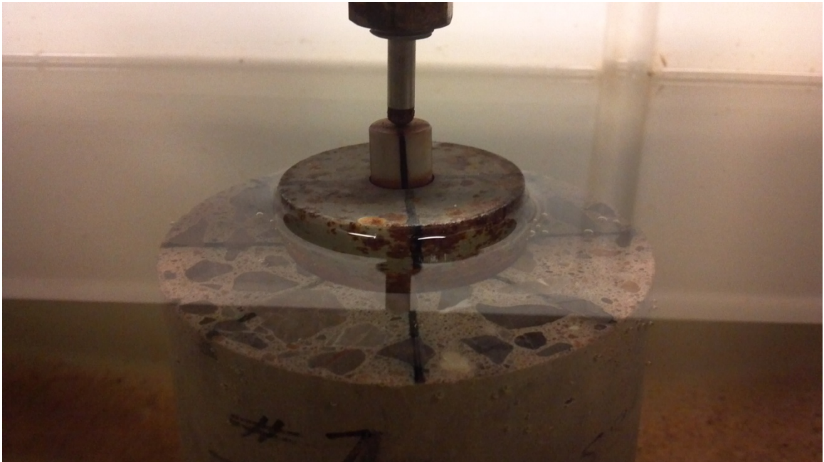
Figure 6.18 Aligned LVDT, Ceramic Spacer, Invar Spacer And Sample In The Holding Tank
