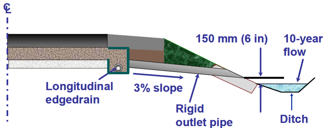
Figure 3.4 Recommended design for edge drain outlet (FHWA-NHI-08-030)
