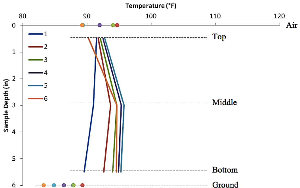
Figure 5.46 Two layers of dry burlap temperature gradients
