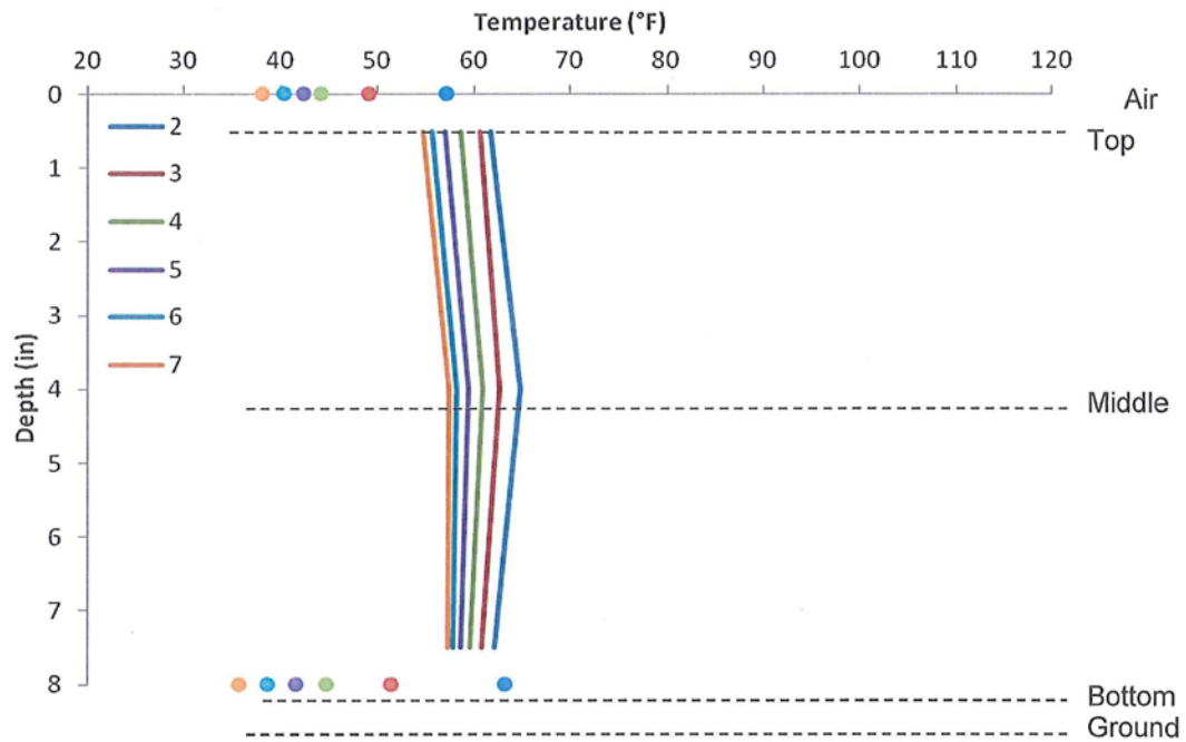
Figure 5. 60 November 30, 2011 temperature differential for one layer of wet burlap and clear plastic
