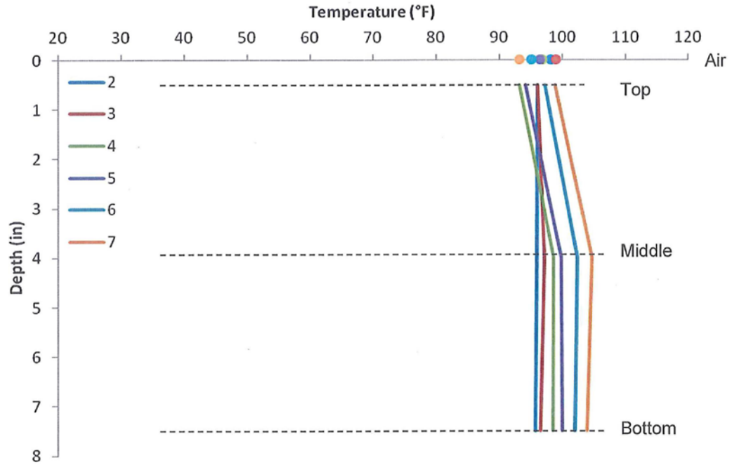
Figure 5. 51 August 29, 2011 no cure temperature differentials
