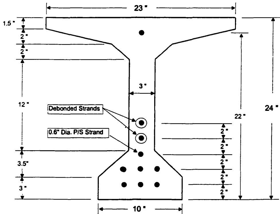
Figure 6.4. Cross-section of Girder 4.
