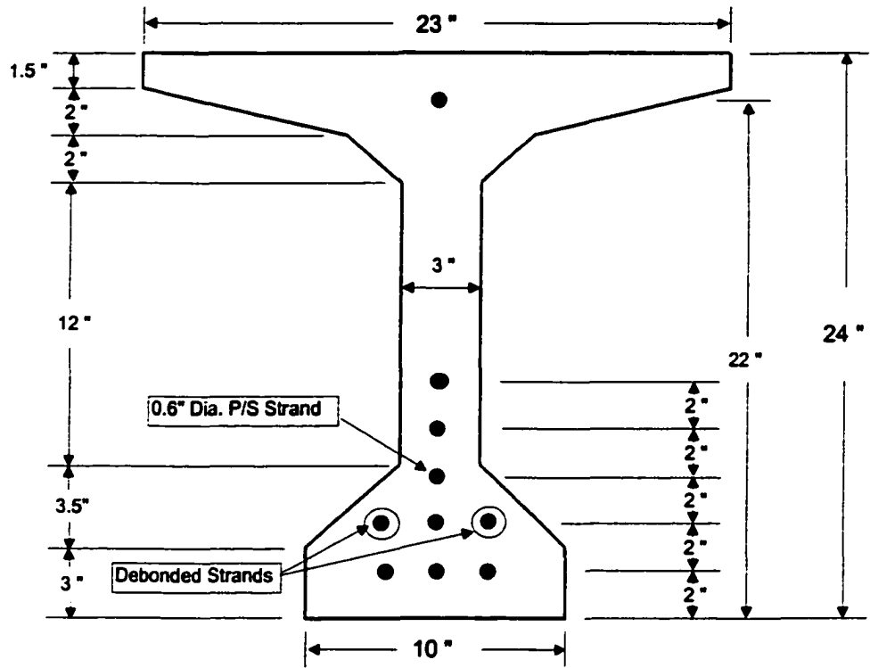
Figure 6.3. Cross-section of Girder 3.
