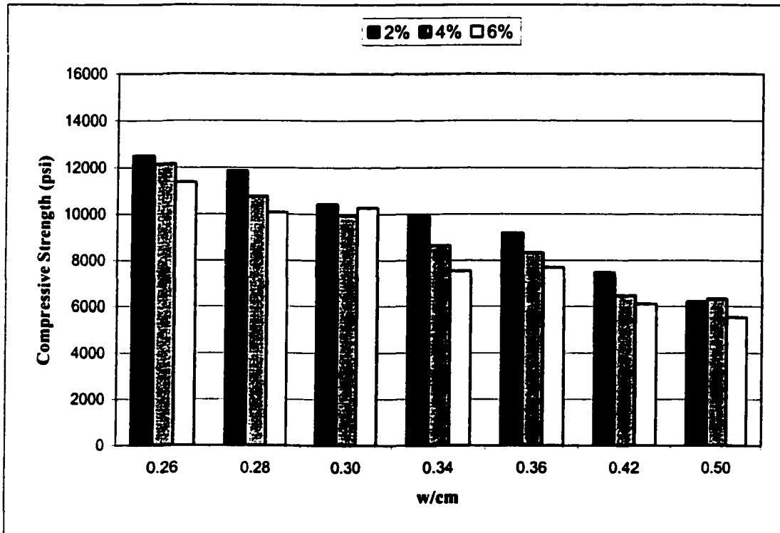
Figure 3.5. Compressive Strength Results at 28 Days.
