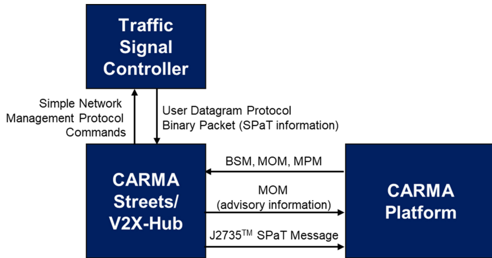
Figure 4. Graphic. CARMA design and architecture for adaptive traffic signal optimization use case for automation Level 3, cooperation Class D. (3-10)
