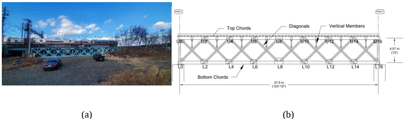
Figure 4: Span 3 of Cos Cob Bridge: (a) Picture, (b) elevation view drawing [14]
