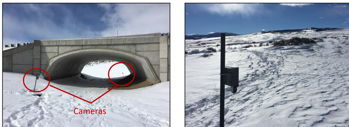
Figure 3. Two cameras were positioned at each underpass at opposite corners (left). Habitat camera placed 50-100 feet in front of a structure, facing out into the adjacent habitat (right).
