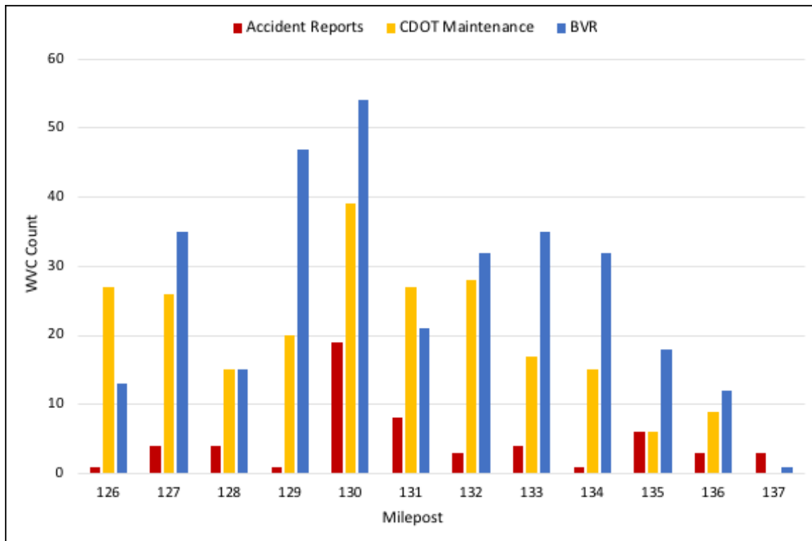
Figure 25. Comparison of WVC data from Accident Reports, CDOT Maintenance carcass reports and BVR/CPW by milepost for five years pre-construction and one year pre-completion.
