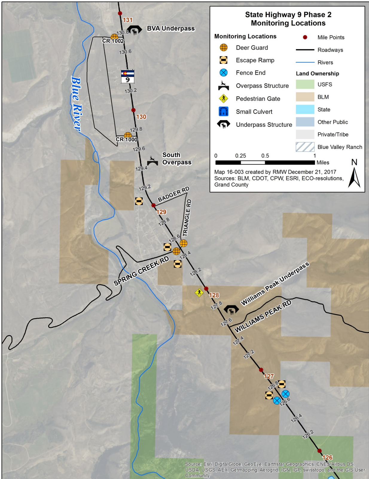
Figure 2. Phase 2 (south segment, MP 126 – 131) monitoring locations.
