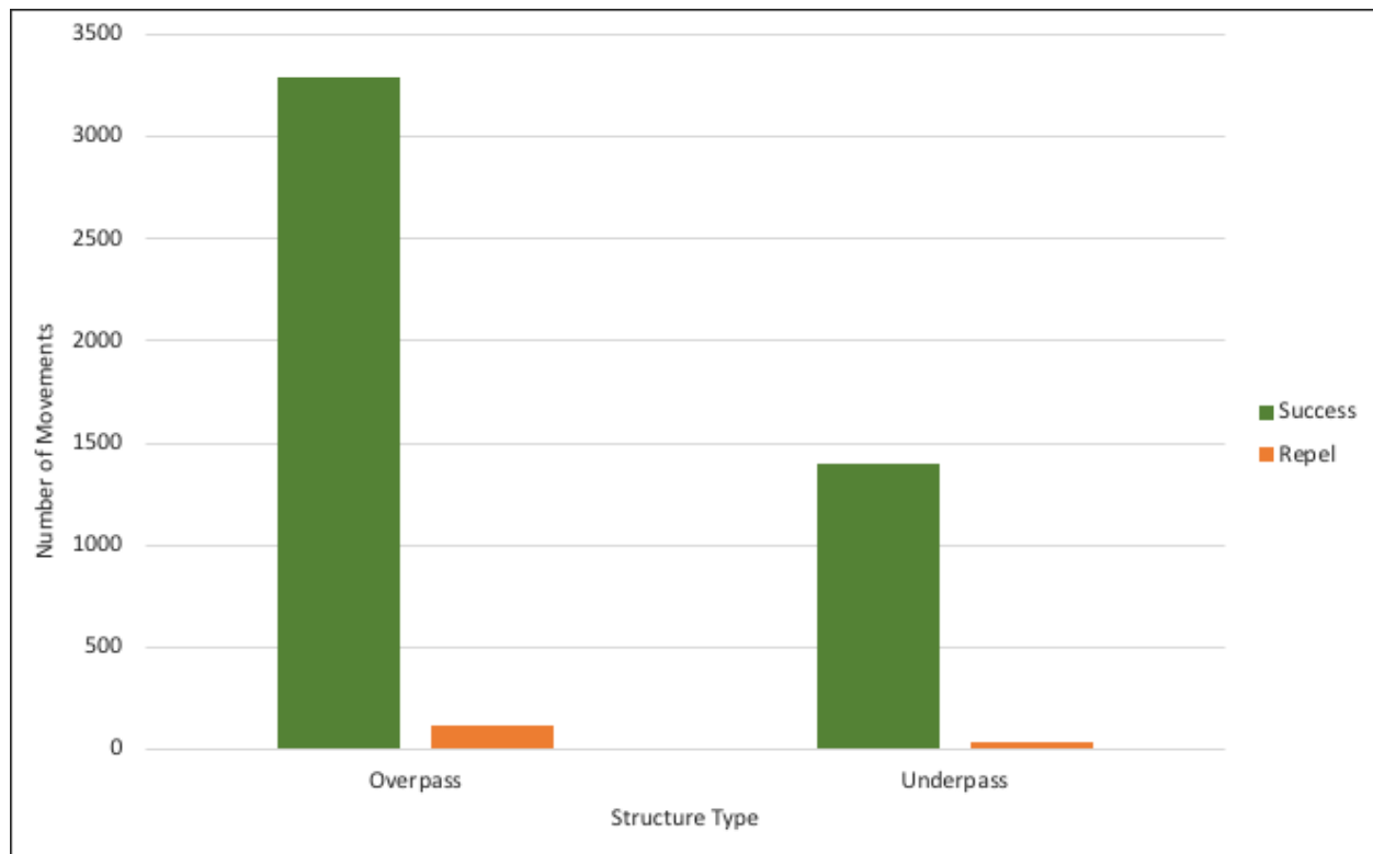
Figure 5. Average number of success and repel movements for mule deer at overpass versus underpass structures during Winter 2016-17.
