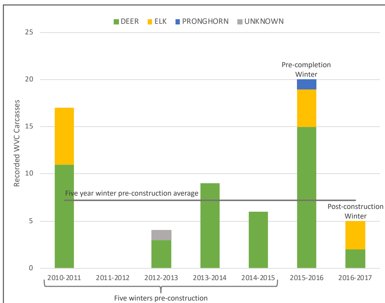
Figure 26. Ungulate carcass counts recorded by CDOT Maintenance on US 40 east and west of Kremmling for five winters prior to mitigation construction, one winter following the construction of the Phase 1 segment (pre-completion) and one year post-construction. The solid line represents the five-year pre-construction average number of carcasses (7.2).
