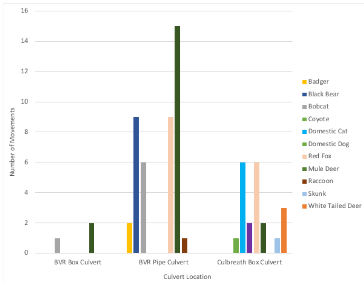
Figure 15. Species presence at small culverts, including success, repel and parallel movements.
