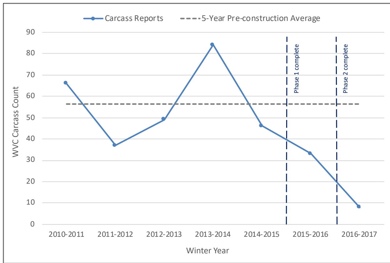
Figure 2. Mule deer and elk carcass counts recorded by Blue Valley Ranch and Colorado Parks and Wildlife pre-construction to post-construction compared to the 5-year pre-construction average of 56.4 carcasses per year.
