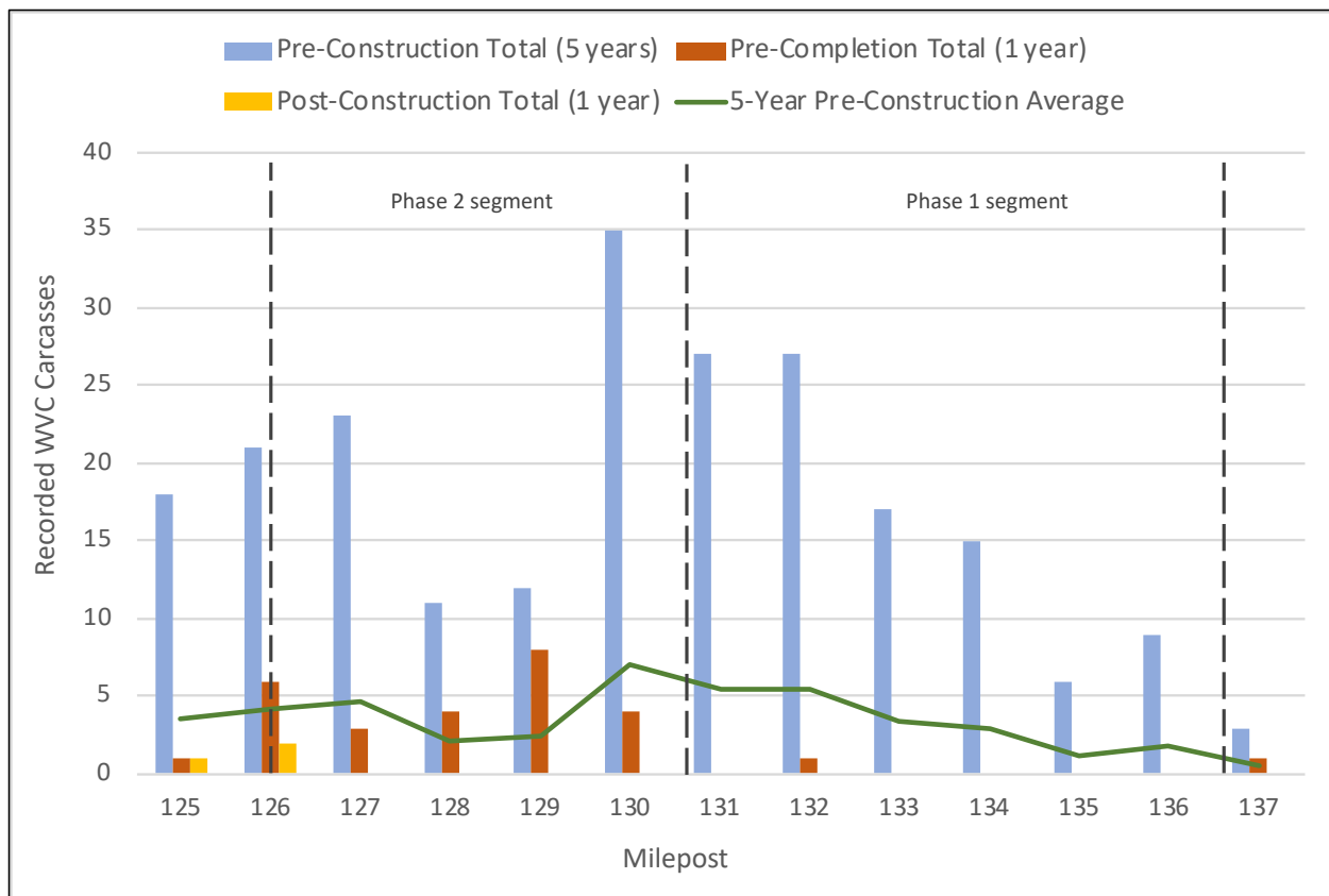
Figure 22. Mule deer and elk carcass counts recorded by CDOT Maintenance by milepost. Pre-construction totals comprise 5 years; pre-completion and post-construction totals comprise 1 year each. The 5-year pre-construction average was calculated for each one-mile segment.
