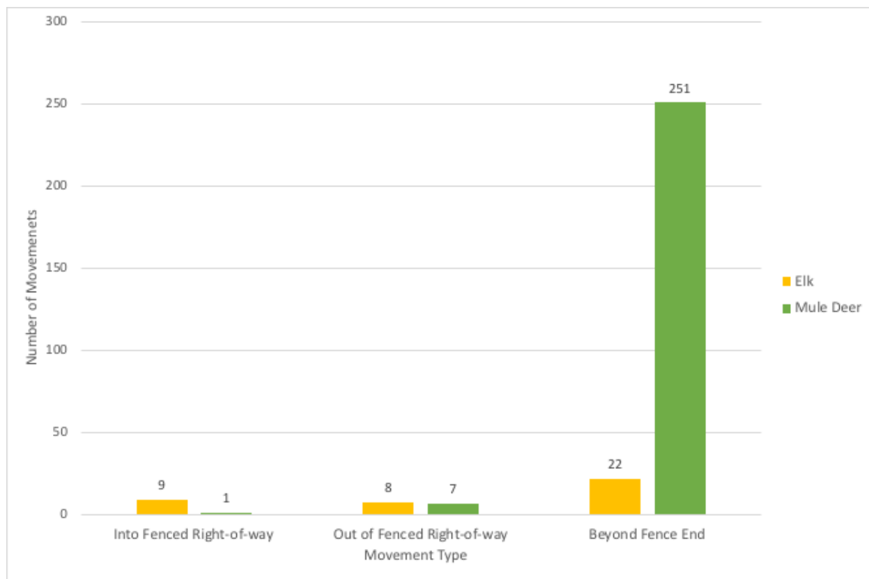
Figure 19. Elk and mule deer movements at the south fence end.
