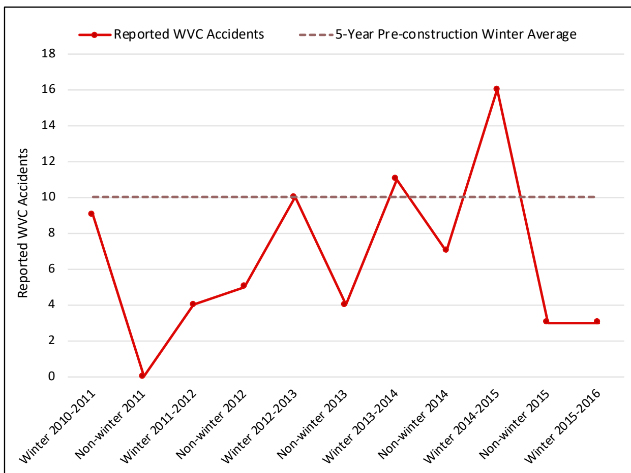
Figure 23. Accidents reported to law enforcement involving mule deer or elk relative to the 5-year pre-construction average.
