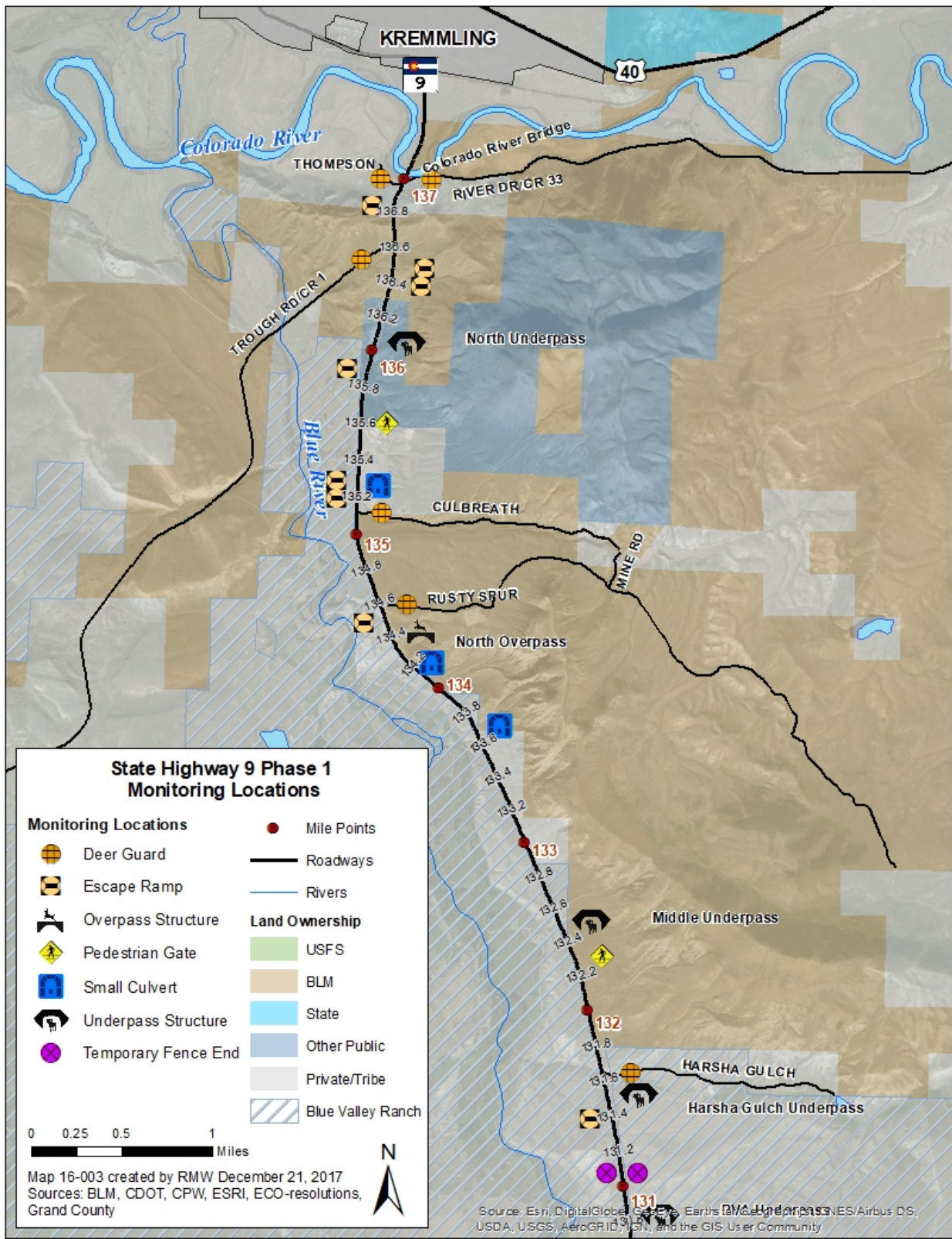
Figure 1. Phase 1 (north segment, MP 131 – 137) monitoring locations.
