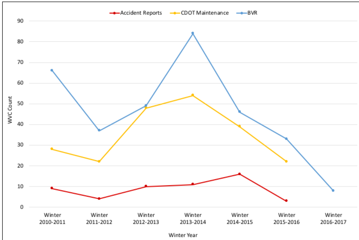
Figure 24. Comparison of WVC data from Accident Reports, CDOT Maintenance carcass reports and BVR/CPW carcass reports. Accident data for 2017 were not available at the time of this analysis.
