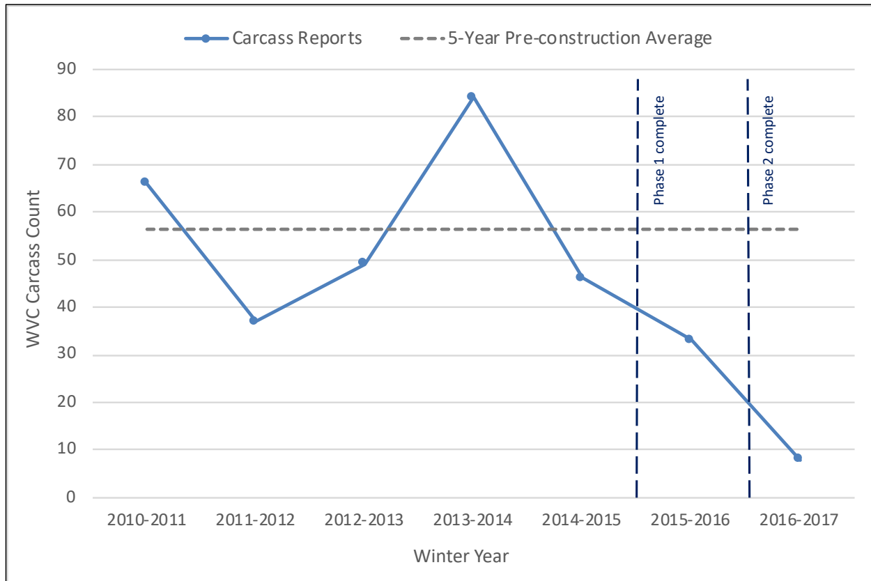
Figure 20. Mule deer and elk carcass counts recorded by BVR and CPW during winter, pre-construction to post-construction.
