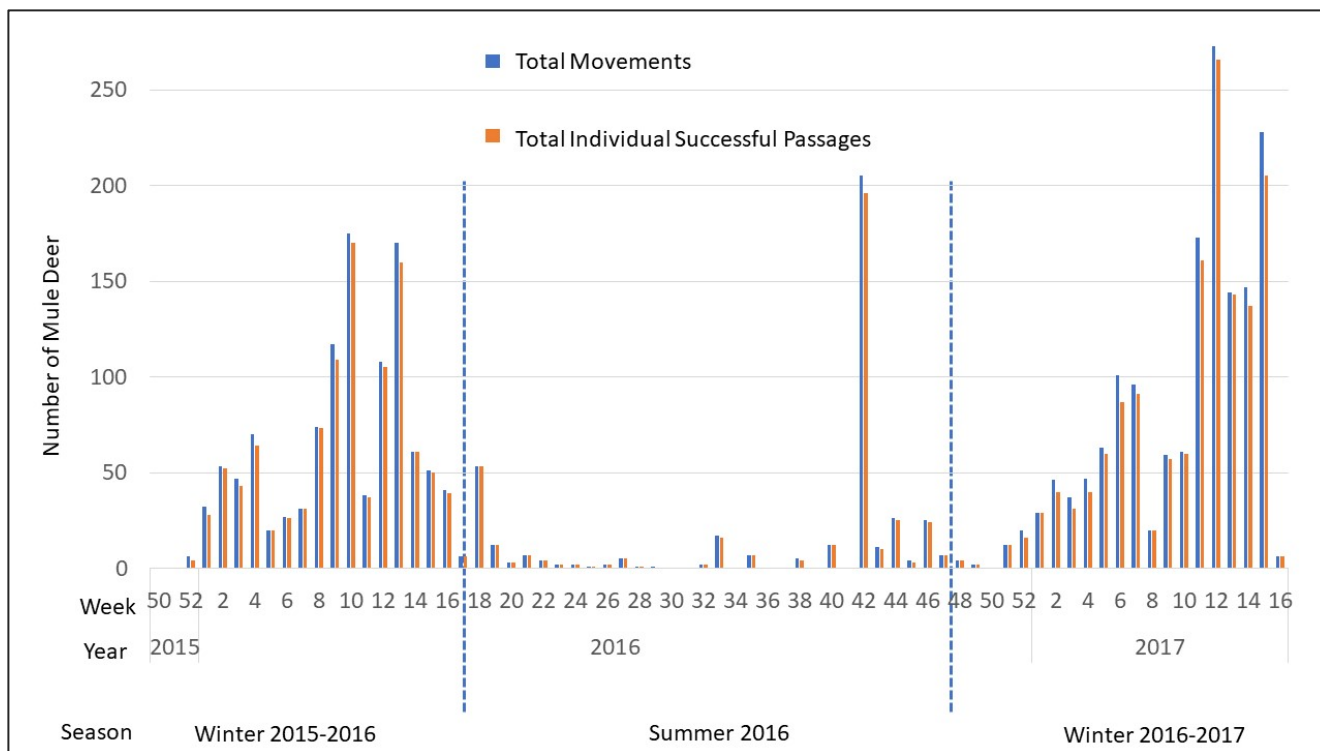
Figure 8. Mule deer total movements and success movements by weeks of the year at the Middle Underpass (MP 132.5). Note y-axis scale is 0-250.
