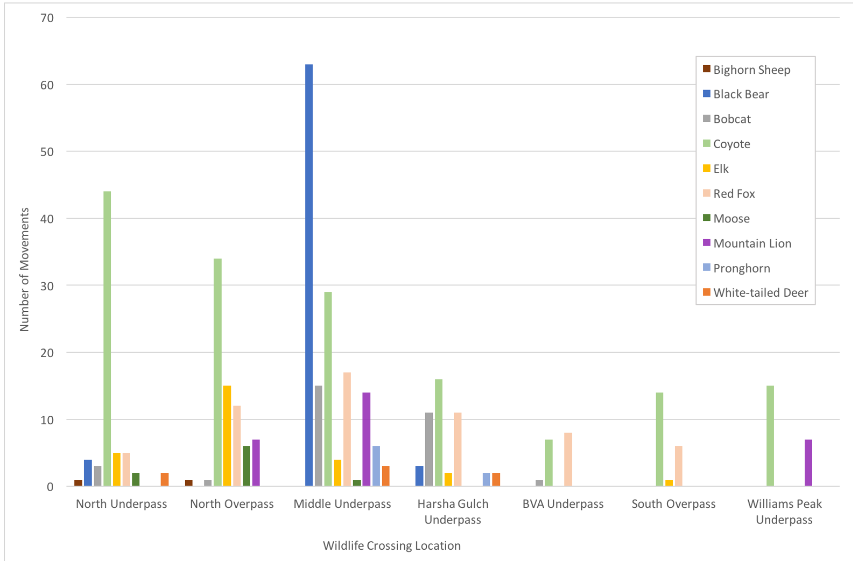
Figure 13. Success movements by non-mule deer species at each wildlife crossing structure from the onset of pre-completion monitoring in December 2015 through April 2017.
