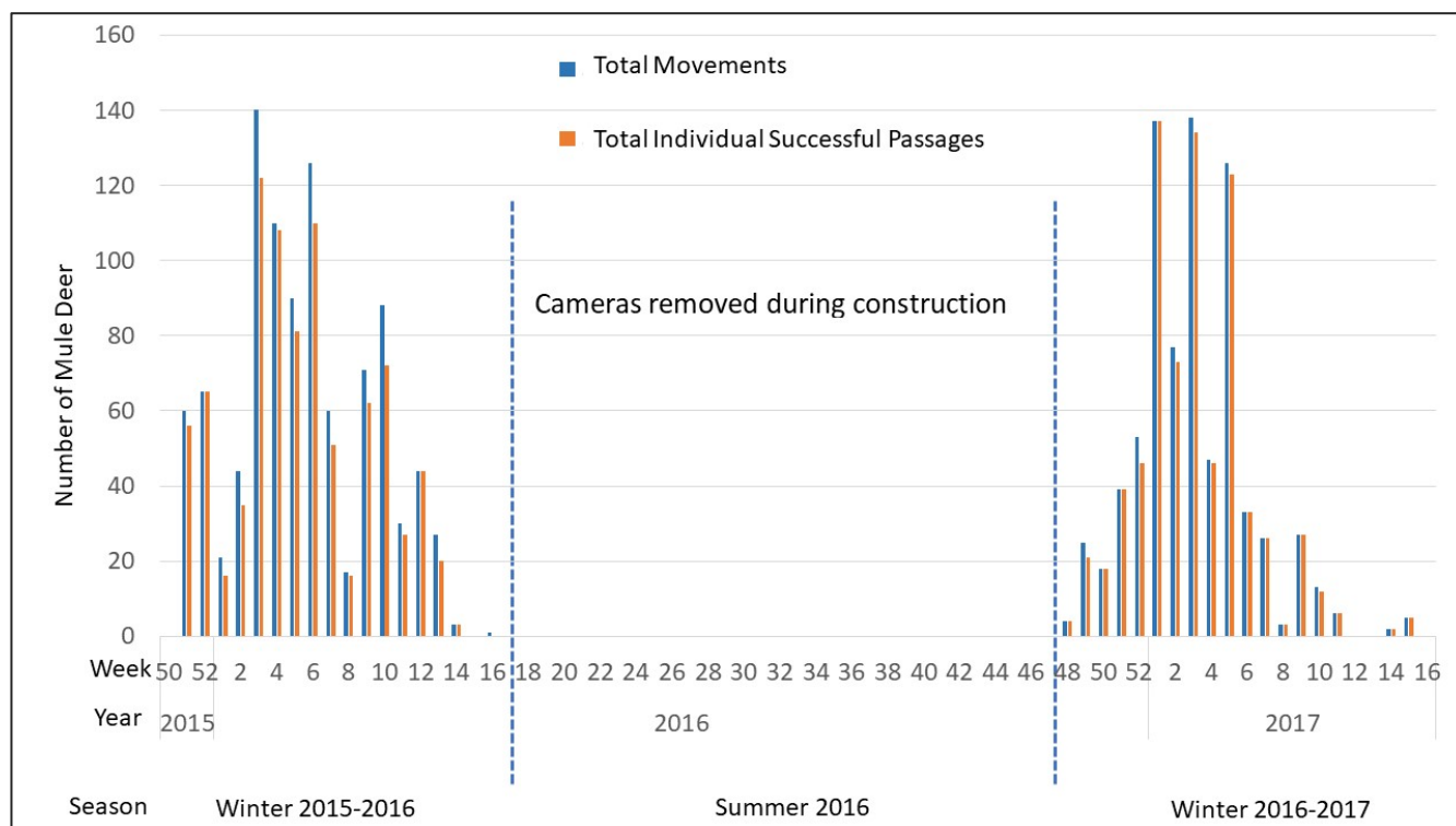
Figure 9. Mule deer total movements and success movements by weeks of the year at Harsha Gulch Underpass (MP 131.6). Note y-axis scale is 0-160.
