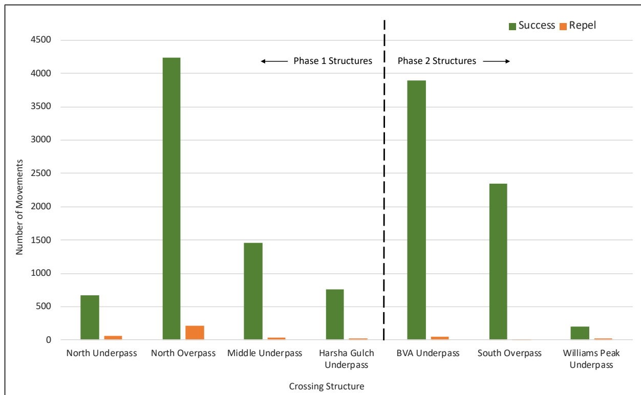
Figure 1. Total number of mule deer success movements and repel movements at each crossing structure location during Winter 2016-17.
