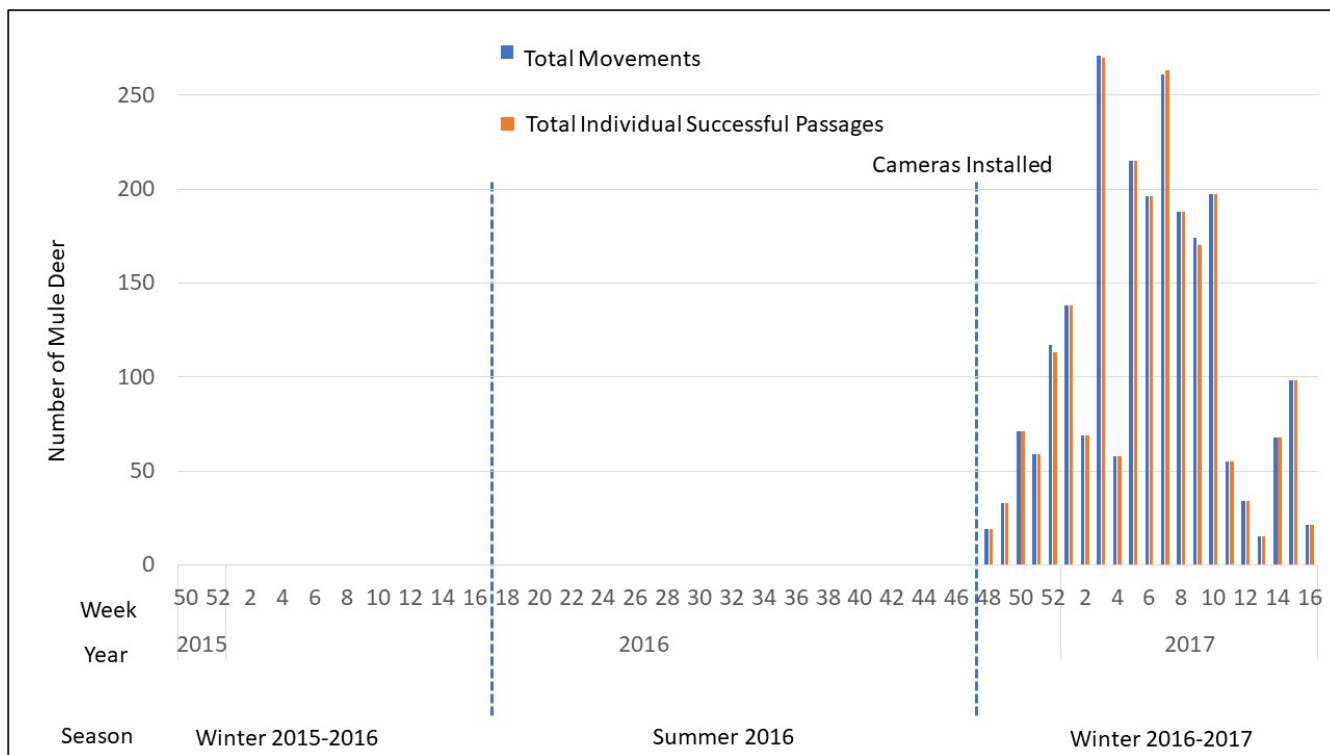
Figure 11. Mule deer total movements and success movements by weeks of the year at the South Overpass (MP 129.5). Note y-axis scale is 0-250.
