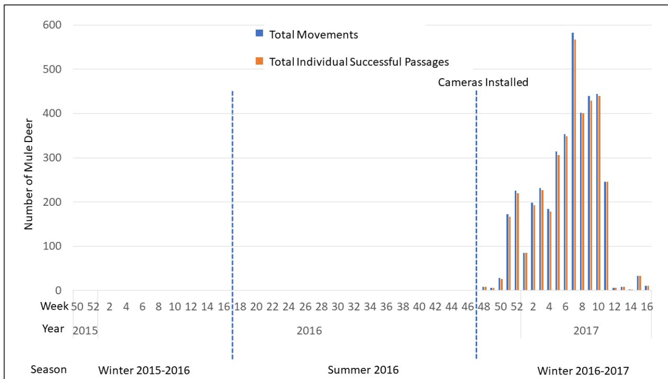
Figure 10. Mule deer total movements and success movements by weeks of the year at the BVA Underpass (MP 130.8). Note y-axis scale is 0-600.
