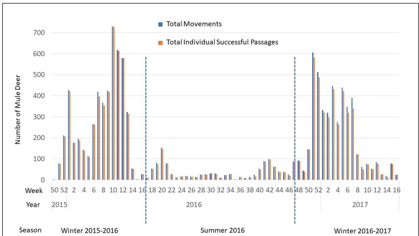
Figure 7. Mule deer total movements and success movements by weeks of the year at the North Overpass (MP 134.3). Note y-axis scale is 0-700.
