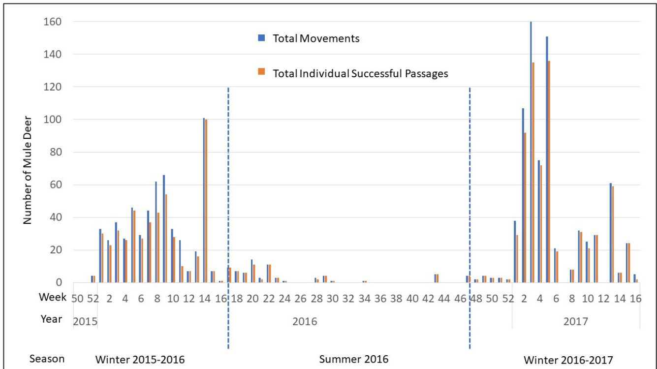
Figure 6. Mule deer total movements and success movements by weeks of the year at the North Underpass (MP 136). Note y-axis scale is 0-160.
