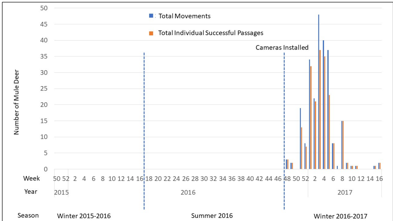
Figure 12. Mule deer total movements and success movements by weeks of the year at the Williams Peak Underpass (MP 127.7). Note y-axis scale is 0-50.
