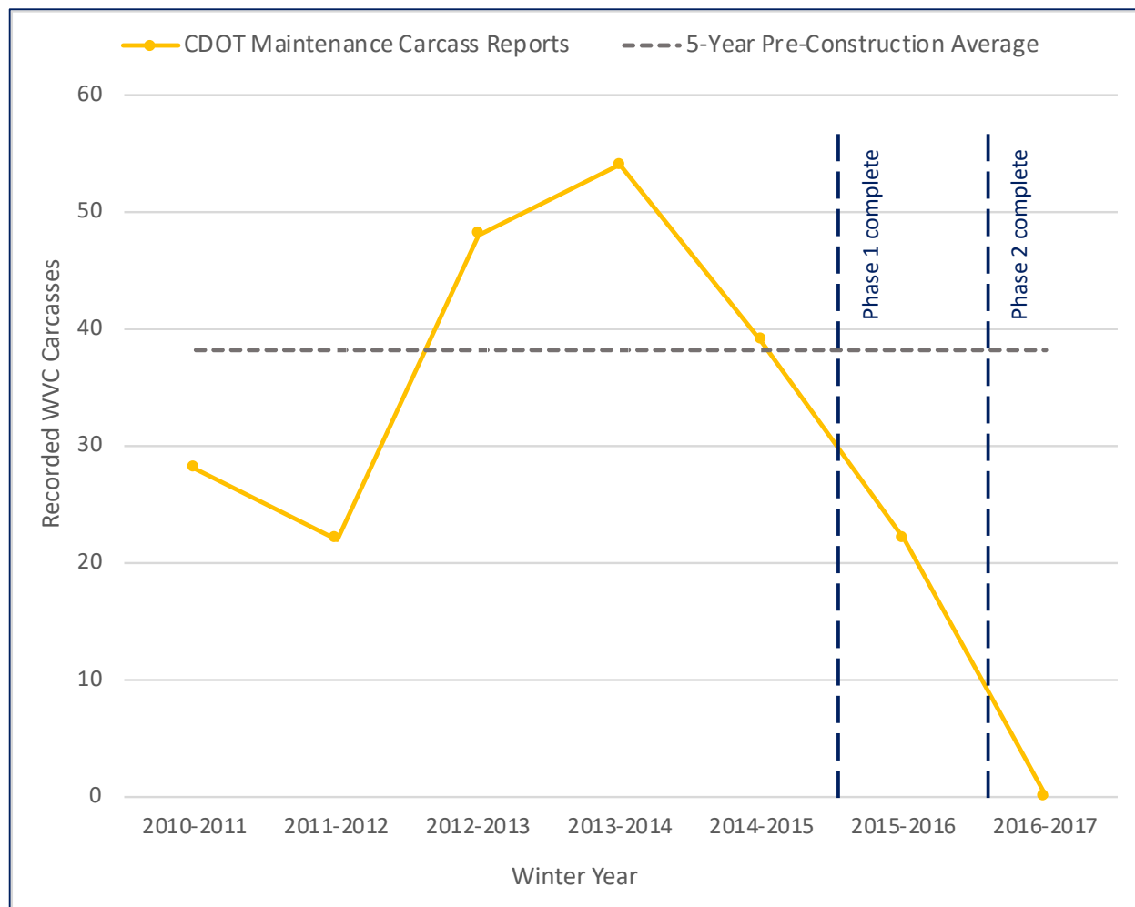
Figure 21. Mule deer and elk carcass counts recorded by CDOT Maintenance pre-construction to post-construction.
