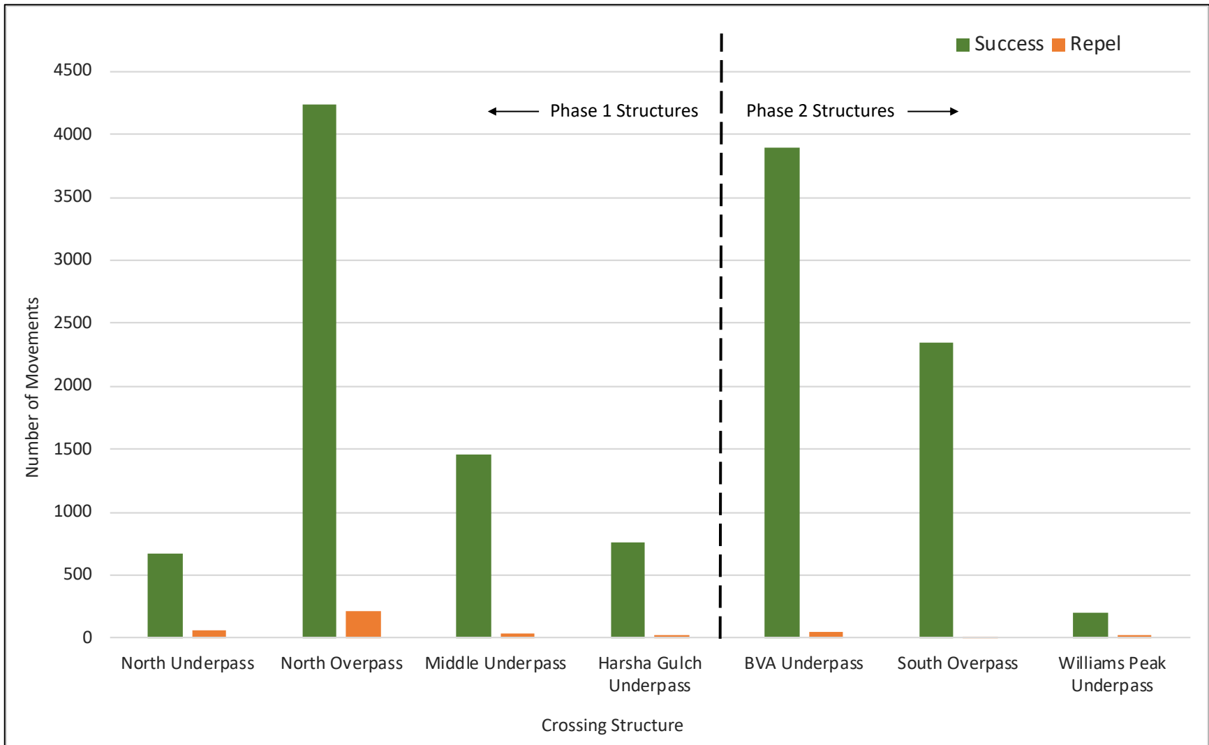
Figure 4. Total number of mule deer success and repel movements at each crossing structure location during Winter 2016-17.
