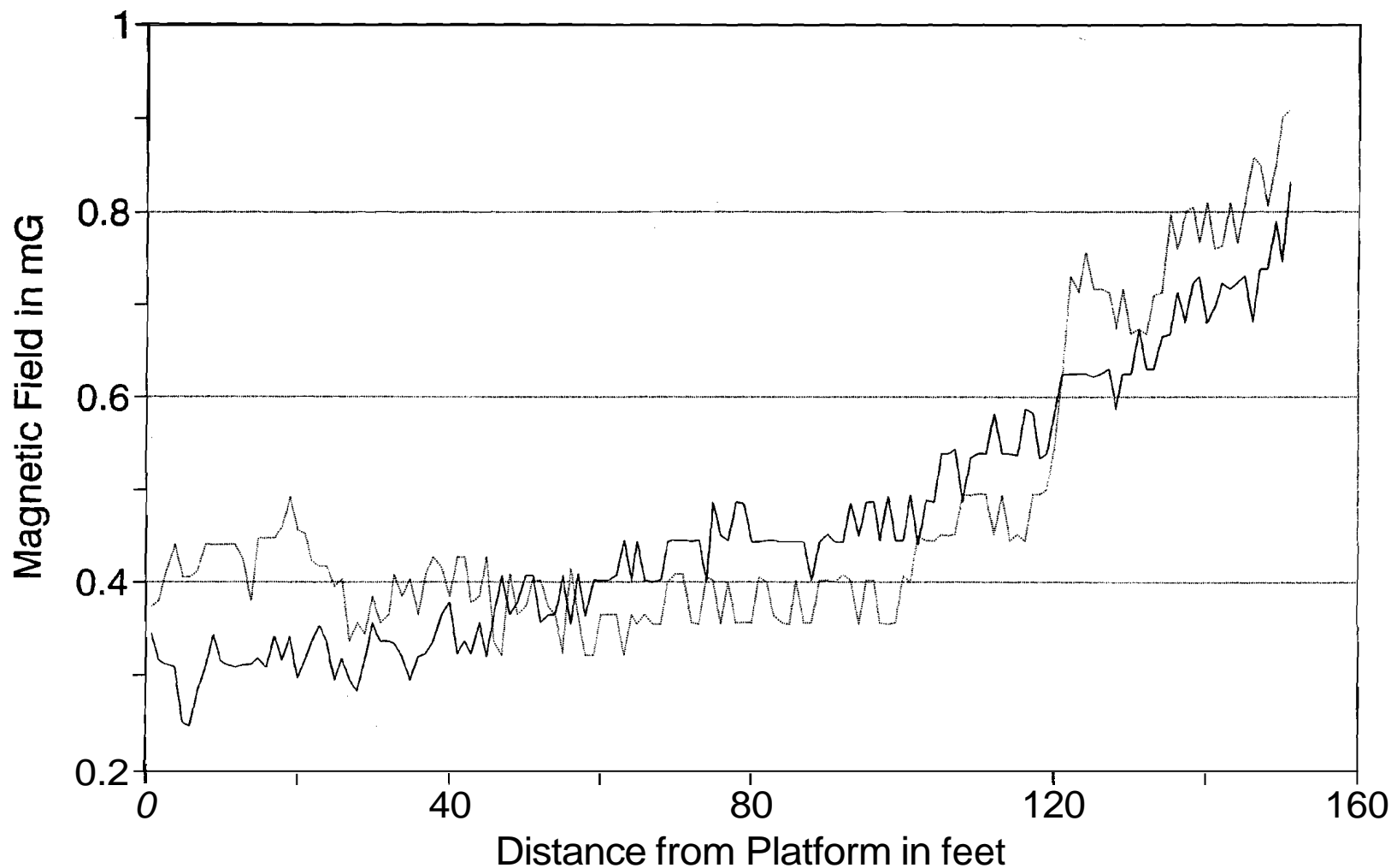
FIGURE 7-5. MAGNETIC FIELD AS A FUNCTION OF DISTANCE FROM THE STATION PLATFORM ALONG PROFILE LINE 3, 30.5 M (100 FT) OUTSIDE THE SUBSTATION FENCE AT THE MT. VERNON SUBSTATION
