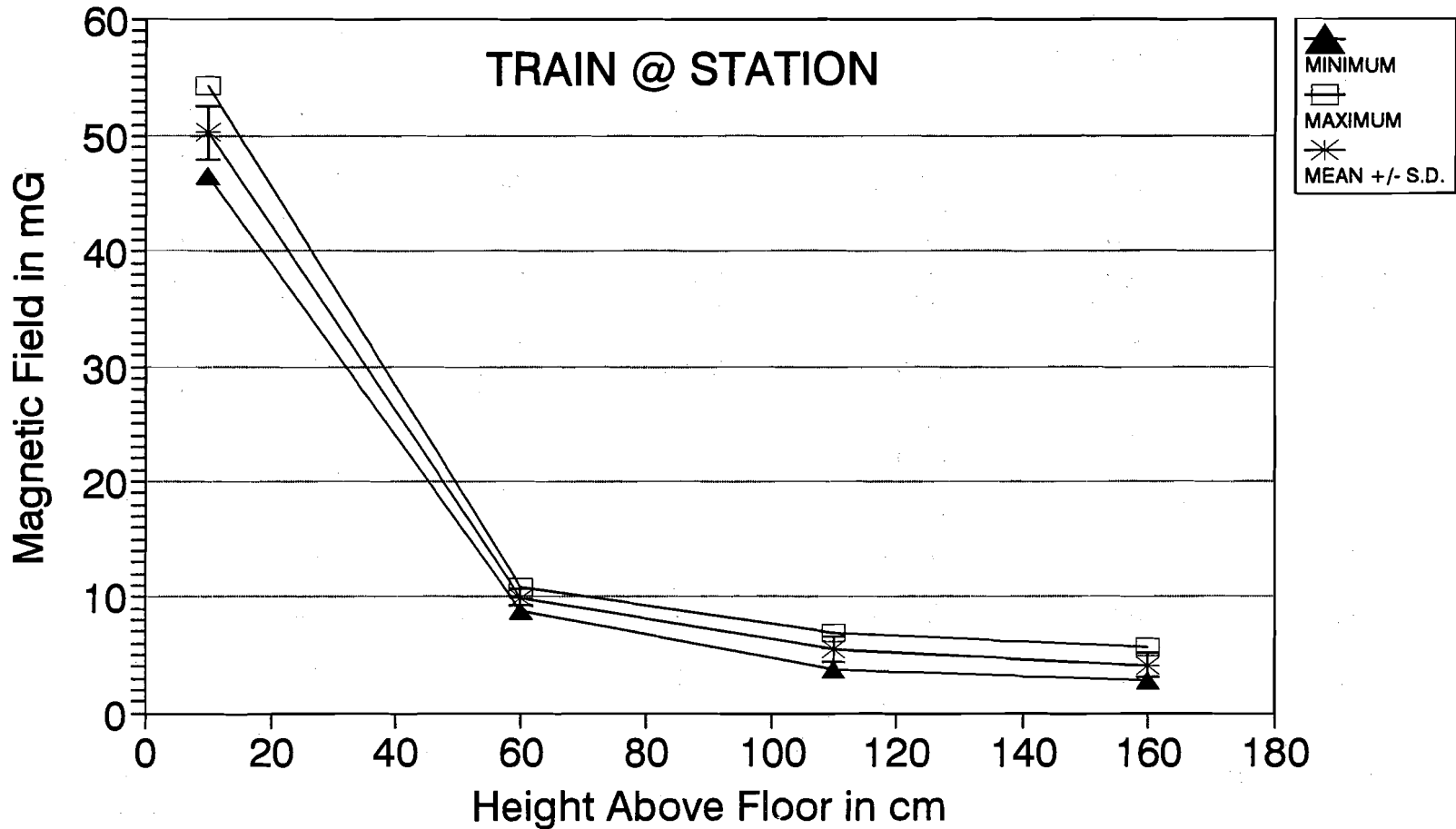
FIGURE 4-16. VERTICAL PROFILE OF THE POWER FREQUENCY MAGNETIC FIELD STRENGTH IN THE REAR CAB OF A LOCOMOTIVE STANDING AT THE LONG BRANCH STATION ON THE 60 HZ SECTION OF THE NORTH JERSEY COAST LINE
