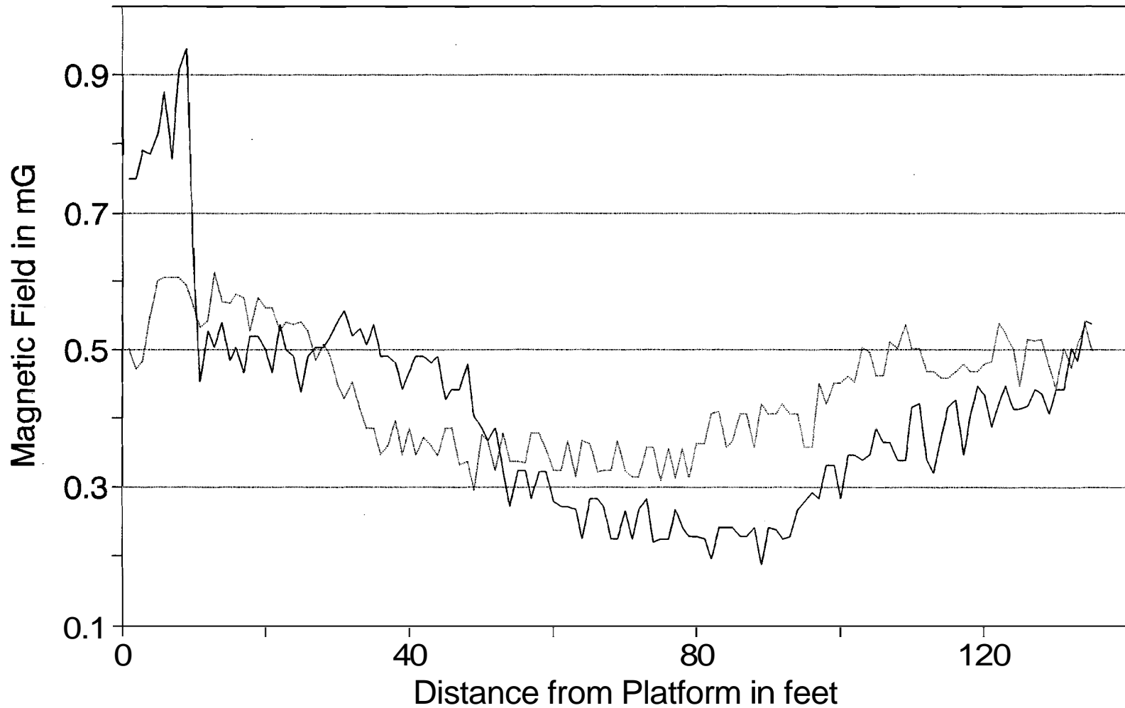
FIGURE 7-4. MAGNETIC FIELD AS A FUNCTION OF DISTANCE FROM THE STATION PLATFORM ALONG PROFILE 1, 1.5 M (5 FT) OUTSIDE THE SUBSTATION FENCE AT THE MT. VERNON SUBSTATION
