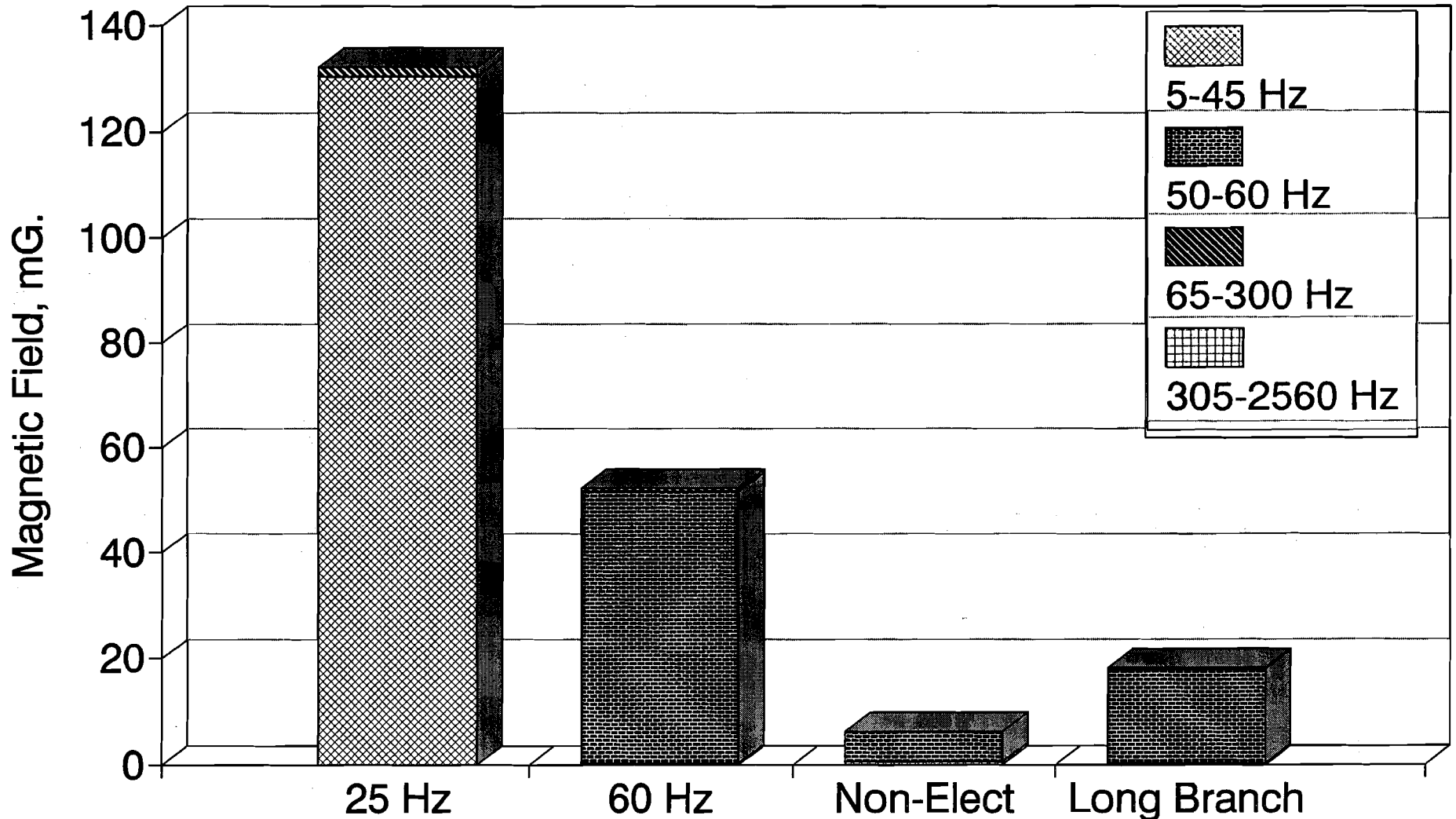
FIGURE 3-24. COMPARISON OF THE AVERAGE TIME-VARYING MAGNETIC FIELD LEVELS IN COACHES ON VARIOUS SECTIONS OF THE NEC AND ON THE NORTH JERSEY COAST LINE AND THEIR PRINCIPAL COMPONENT FREQUENCY RANGES
