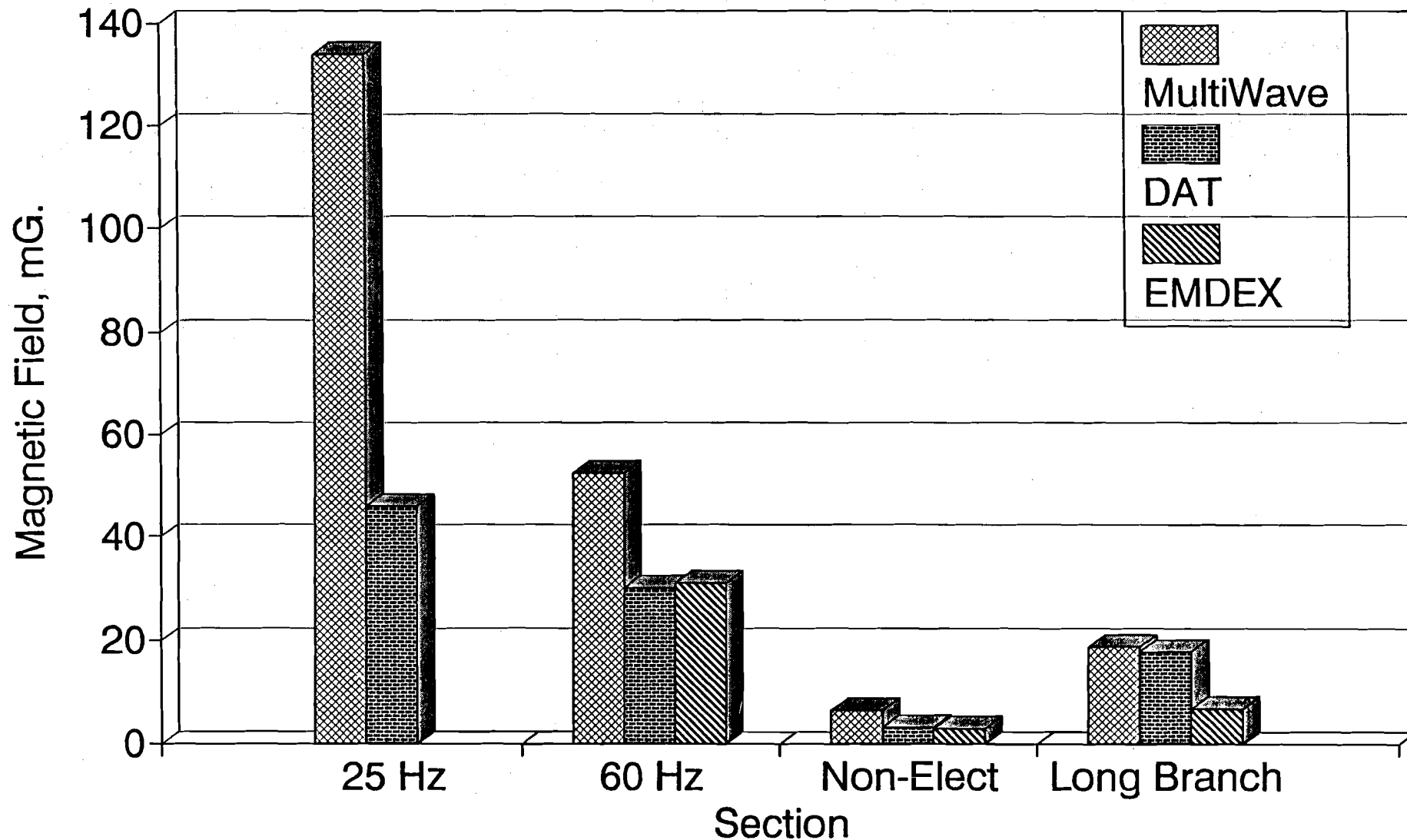
FIGURE 1-2. COMPARISON OF THE AVERAGE TIME-VARYING MAGNETIC FIELD LEVELS IN COACHES OPERATING ON VARIOUS SECTIONS OF THE NEC AND THE NORTH JERSEY COAST LINE MEASURED IN DIFFERENT WAYS
