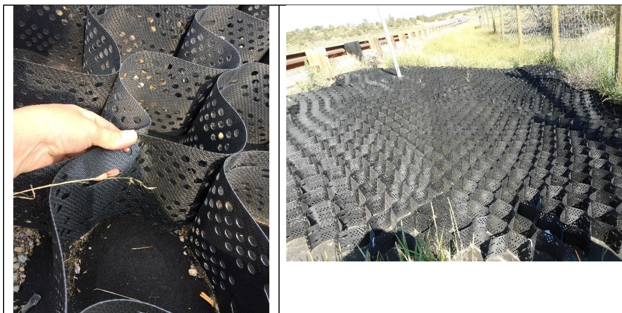
Figure 4. The EnviroGrid® Geocell Up Close (left), and In-Place at the East Fence End.
