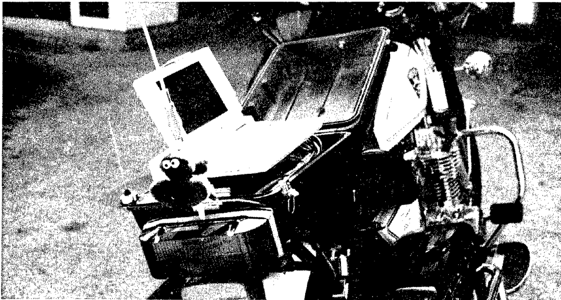
Figure 13. Santa Cruz Police Department's motorcycle-mounted laptop computer system.
