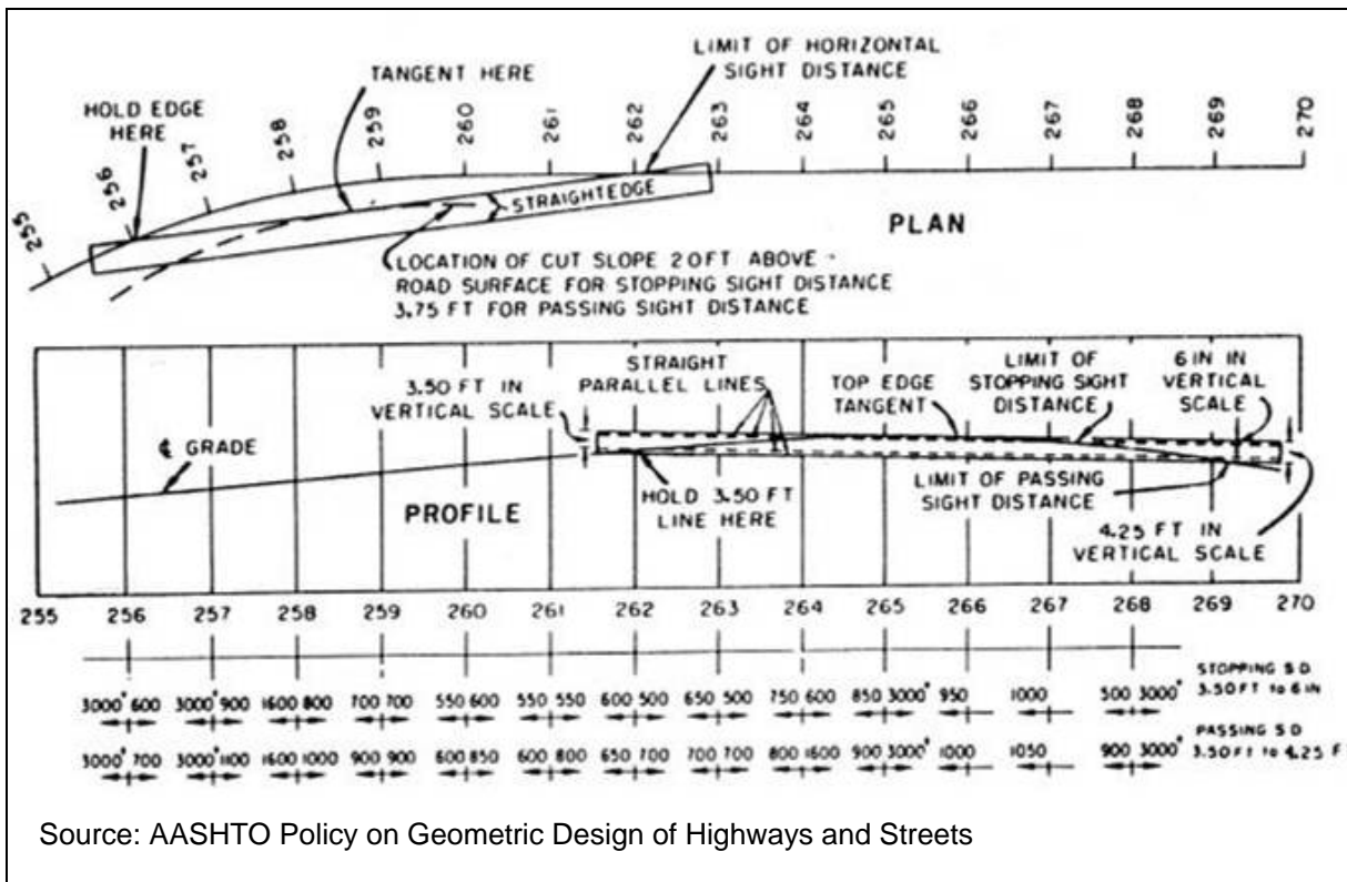
Figure 7-3. AASHTO Method for Scaling and Recording Sight Distance on Plans.
