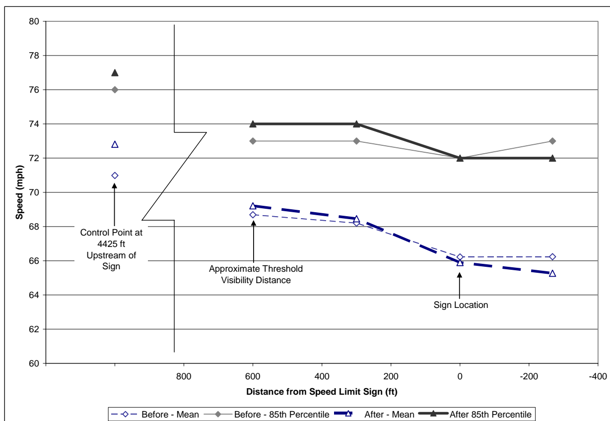
Figure 4-19. FM 36, Milano—Mean and 85th Percentile Speeds before and after Red Border Installation, Passenger Vehicles, Day Data Only.
