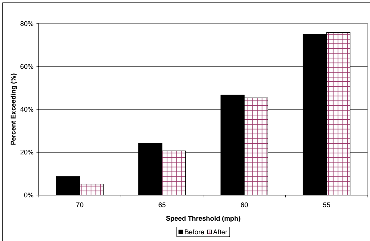
Figure 4-18. FM 60, Snook—Percent of Passenger Vehicles during Night Exceeding Speed Thresholds Downstream of Speed Sign before and after the Installation of the Red Border.
