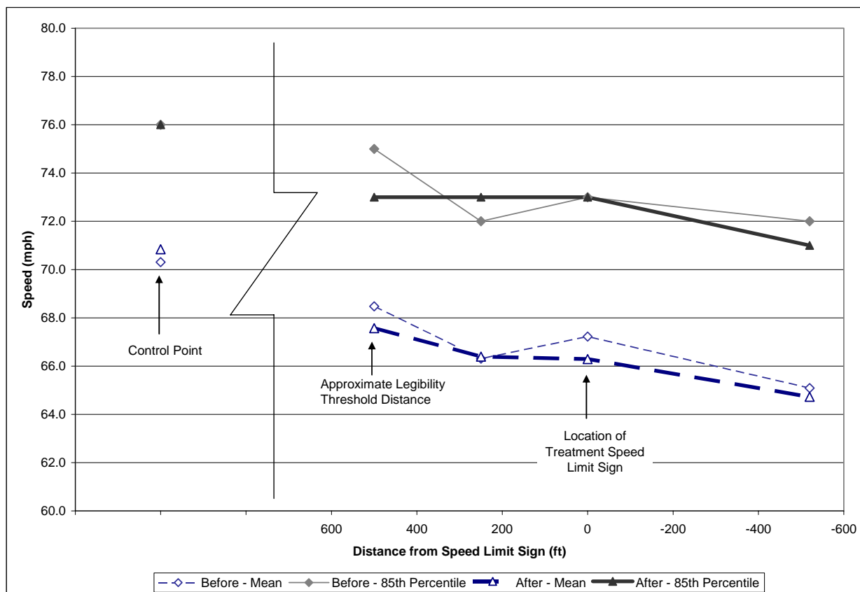
Figure 4-14. FM 60, Snook—Mean and 85th Percentile Speeds before and after Red Border Installation, Passenger Vehicles, Day Data Only.
